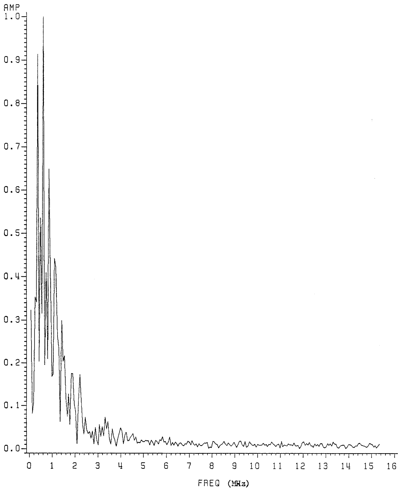
Fig. 18. Amplitude vs. Frequency for 50 Degrees.
