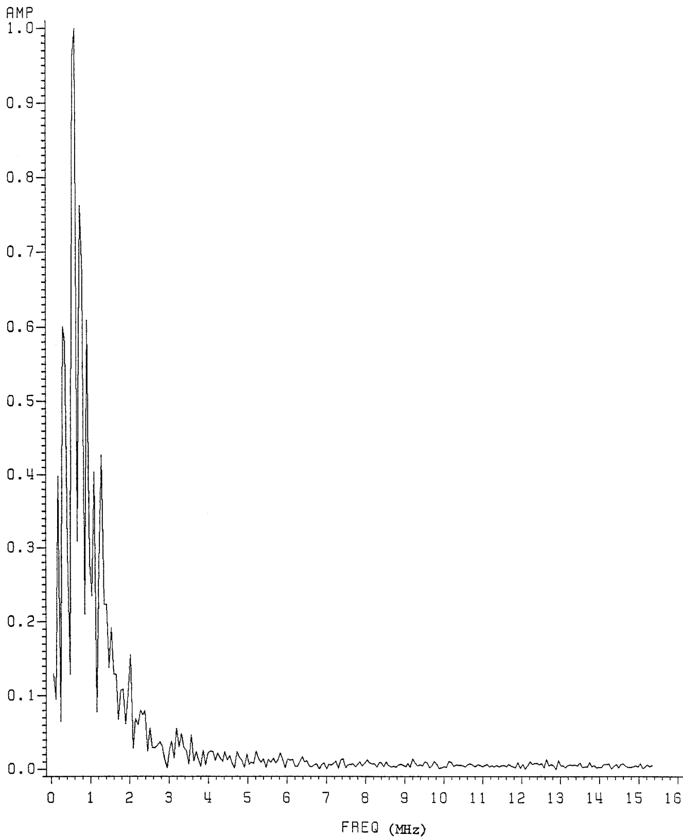
Fig. 16. Amplitude vs. Frequency for 30 Degrees.
