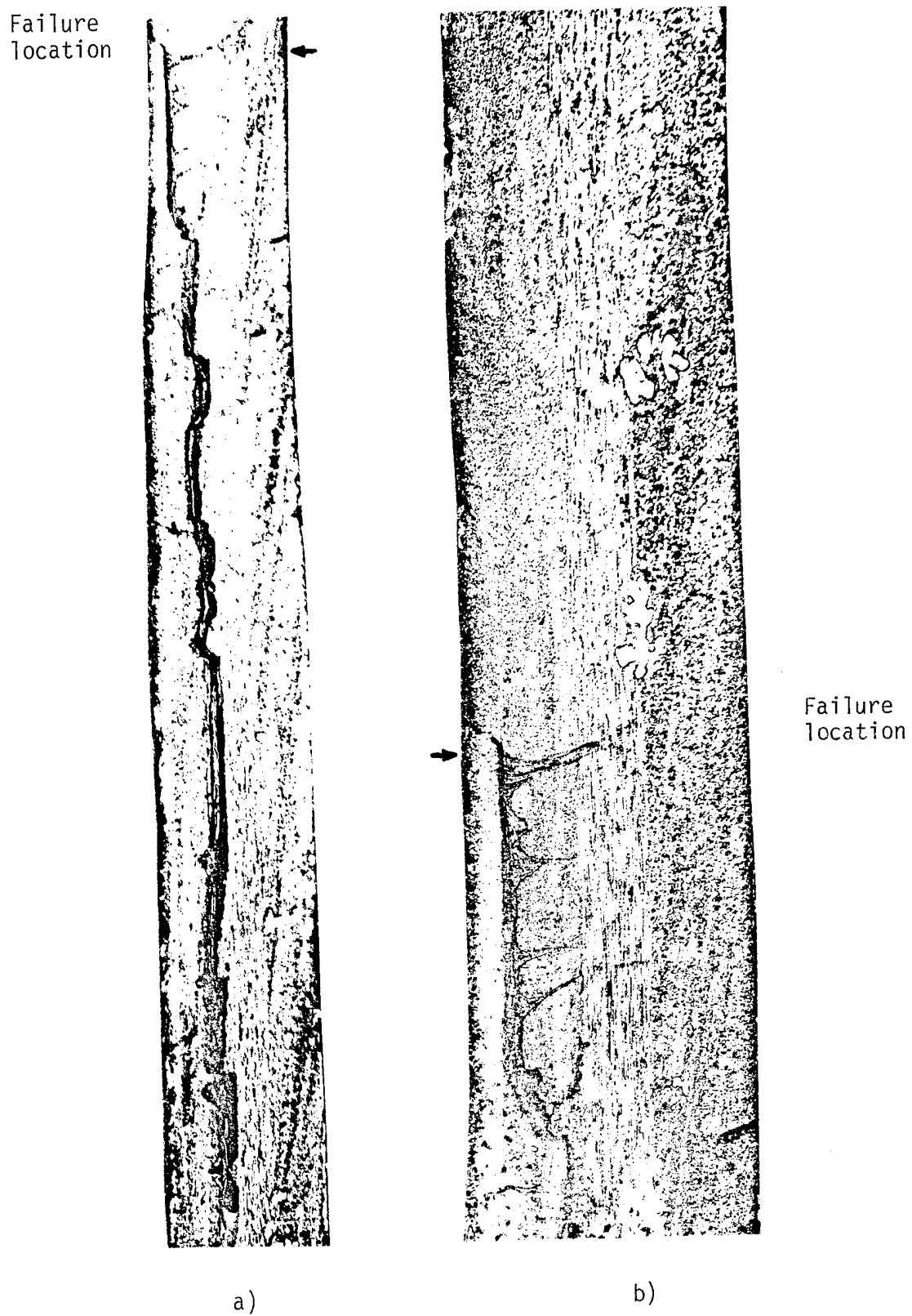
Fig. 13. Edge replicas of specimen #2 after loading close to the failure load. a) 20X b) 40X magnification.
