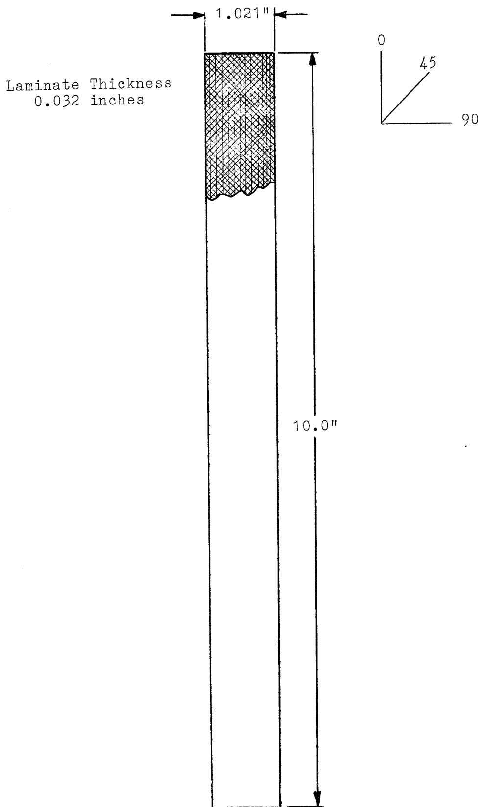
Fig. 1. Specimen configuration.
