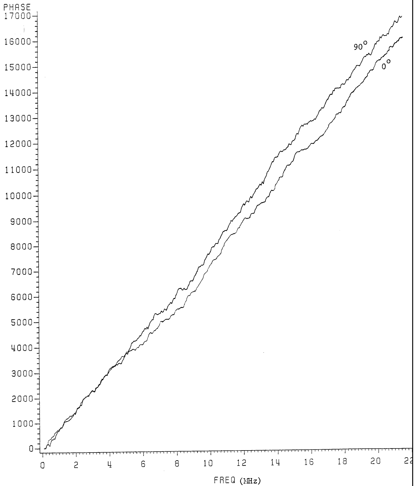
Fig. 12b. Phase Angle vs. Frequency for 0 and 90 Degrees.
