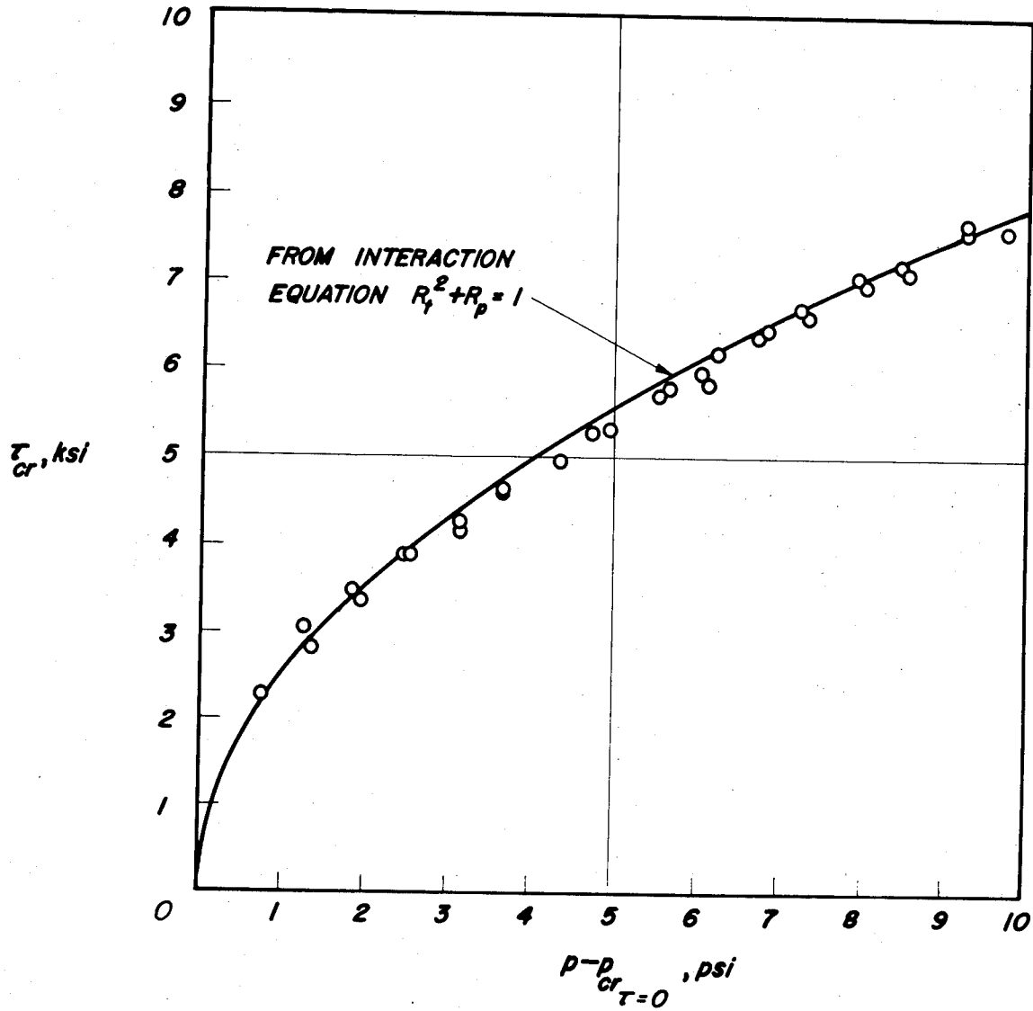
Figure 33.- Effect of internal pressure on torsional-buckling stress of long cylinders. Test results are from reference 43.
