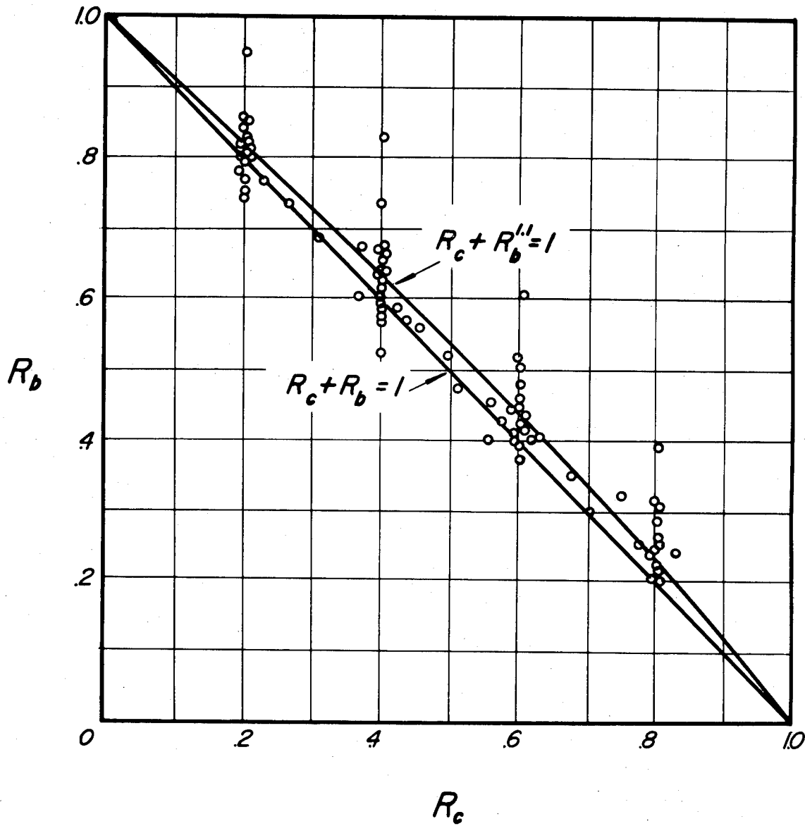
(a) Combined bending and compression.
