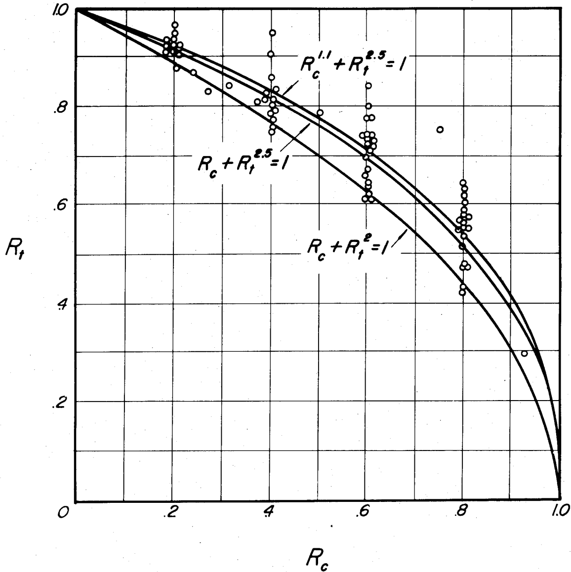
(b) Combined compression and torsion.
