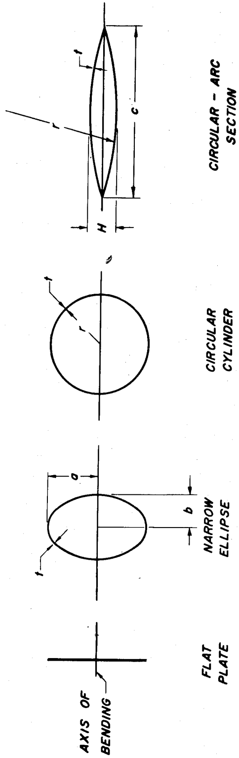
Figure 14.- Elliptic-cylinder geometry.
