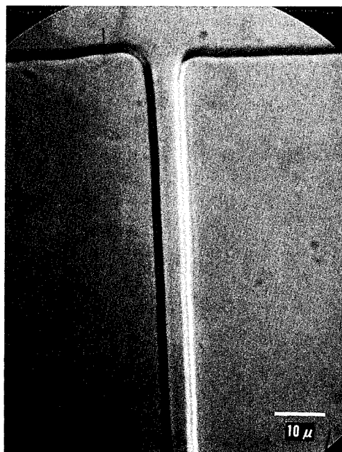
FIG. 9. A 5- \mu m wide light guide in PPS film; 1040X.
