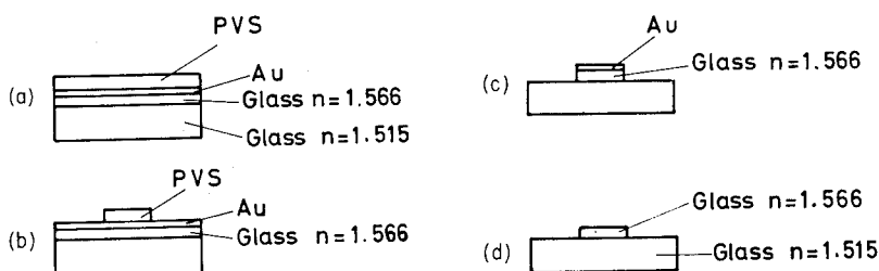
FIG. 6. Procedure for manufacturing optical waveguide in a glass of n = 1.566 : (a) PVS coating; (b) irradiation and development; (c) ion sputter etching; (d) Au removal.
