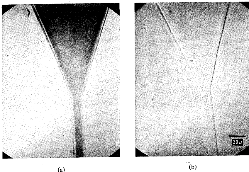
FIG. 7. A 10- \mu m wide light guide in a glass of n = 1.566 : (a) after exposure and heating of PVS; (b) after backspattering.
