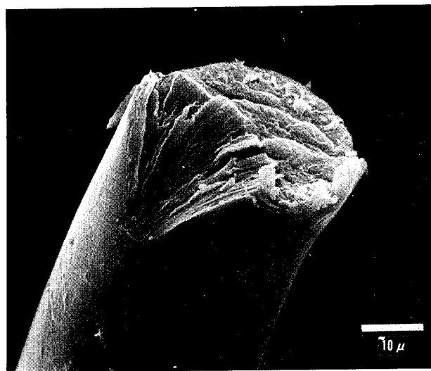
FIG. 1. Typical example of failure through ductile crack growth.
