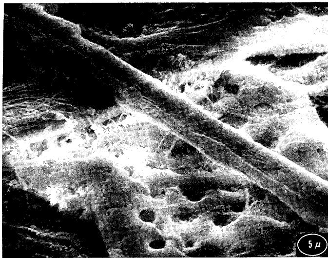
FIG. 7. Felt side of conventional paper; 2,000X.
