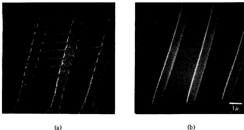
FIG. 9. Gold patterns on oxidized silicon produced by "lift-off" technique with 3% crosslinked PMMA resist: (a) 7000X and 65°; (b) 7000X and 45°.
