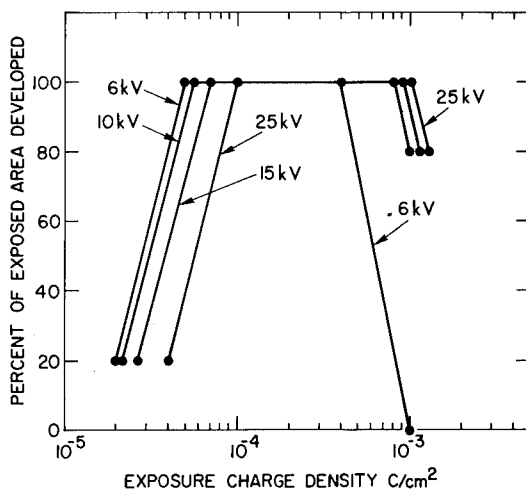
FIG. 1. Exposure characteristics of PMMA resist. Layer thickness = 8000\text{ \AA} . Development was carried out in 3:1 isopropyl alcohol-methyl isobutyl ketone for 2 min at 23^\circ\text{C} .
