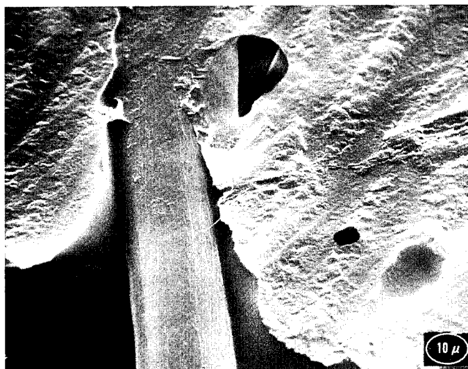
FIG. 2. SEM micrograph of Papylon poly(vinyl alcohol) paper; 1,000X.
