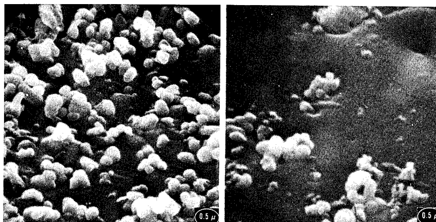
FIG. 10. Titanium dioxide particles chalking out of surface of paint no. 10 at 20,000X; (a) represents general surface area, (b) raised ring with low pigment density.
