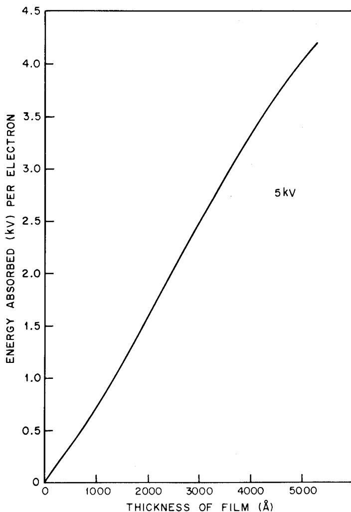
FIG. 6. Energy absorbed per electron as a function of film thickness.
