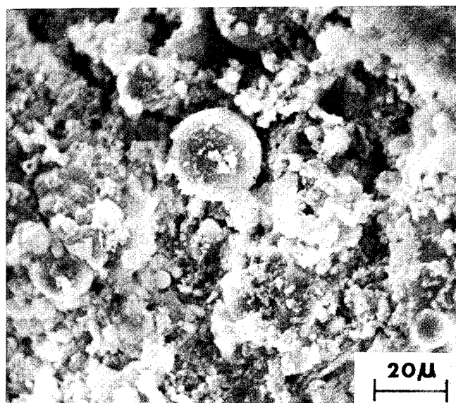
FIG. 9. SEM micrograph of underside of a paint chip peeled from a concrete surface, showing cement particulates.
