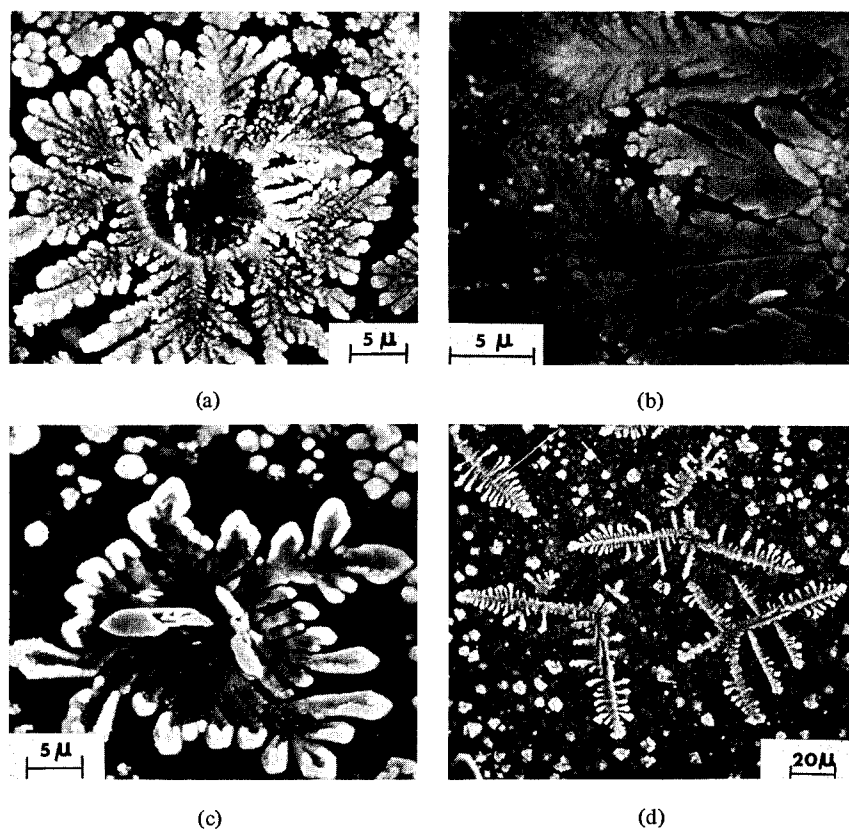
FIG. 13. SEM micrographs of the laboratory-induced discolored areas of a mirror by exposure to HCl vapor: (a) through (c) exposed for 116 hr using 0.1N HCl solution; (d) exposed for 20 hr using 1N HCl solution.
