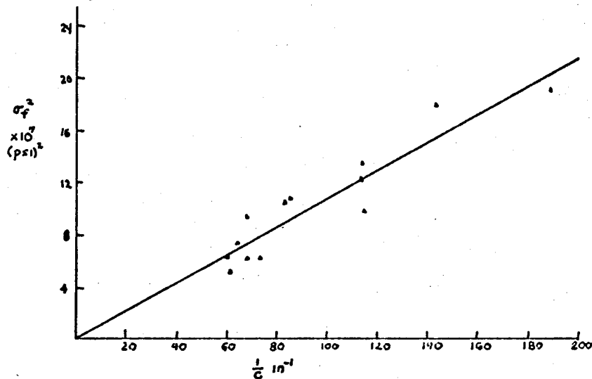
Figure IV-2. (\text{Strength})^2 - reciprocal of the flaw radius curve for the epoxy matrix material.
