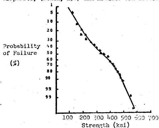
Figure I-3. Boron filament strength distribution.
