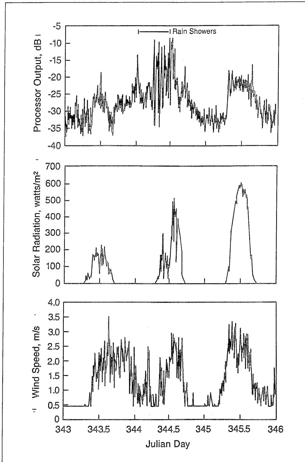
Figure 38. Processor output, solar radiation, and wind speed measured during the 72-hr monitoring period at the BBTS with the TR1 cable deployed on the surface
