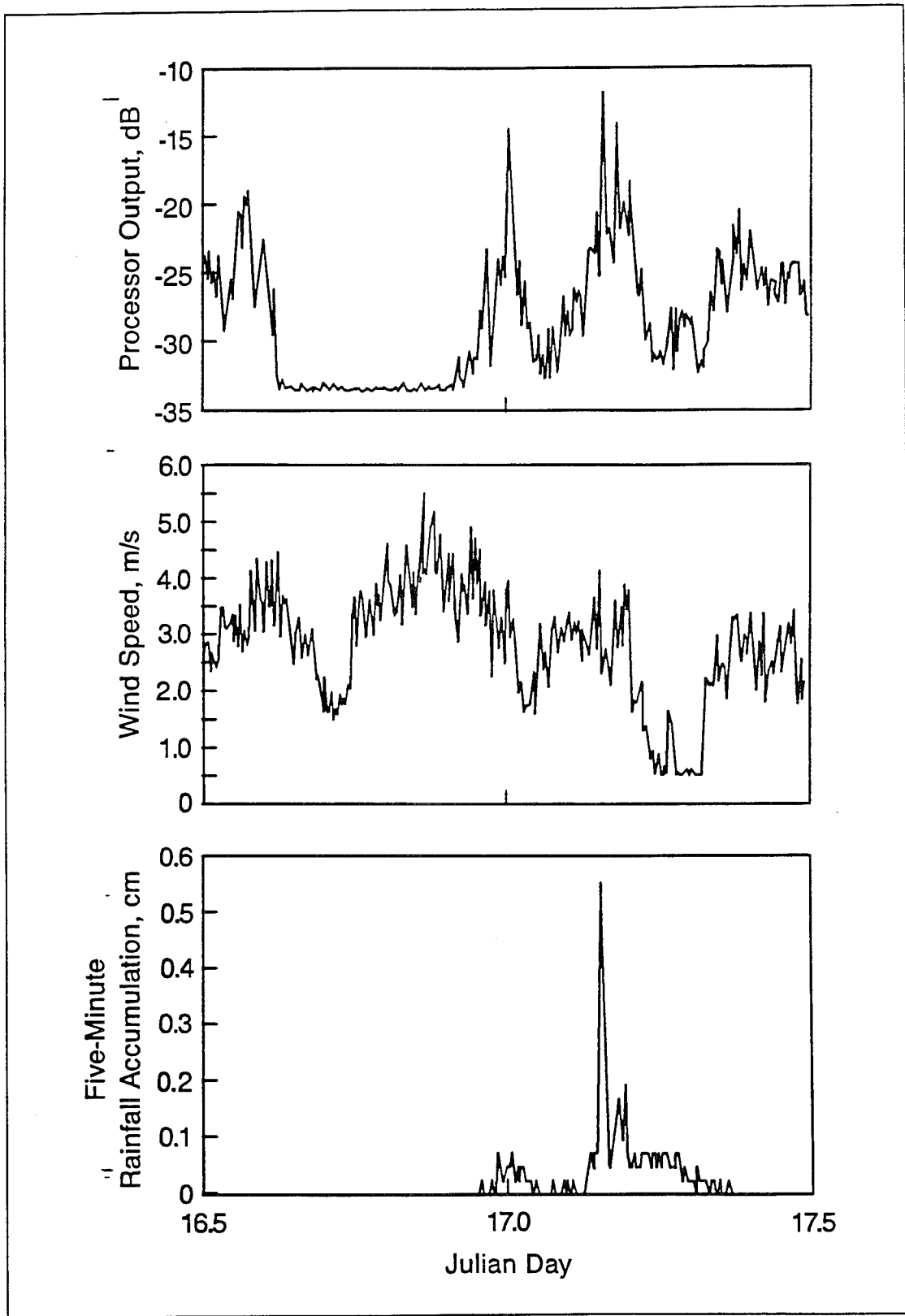
Figure 29. Processor output, wind speed, and rainfall during one 24-hr period at the BBTS
