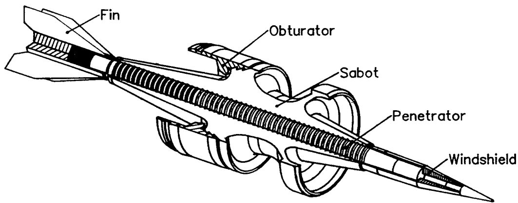
Figure 1. Typical KE projectile.
