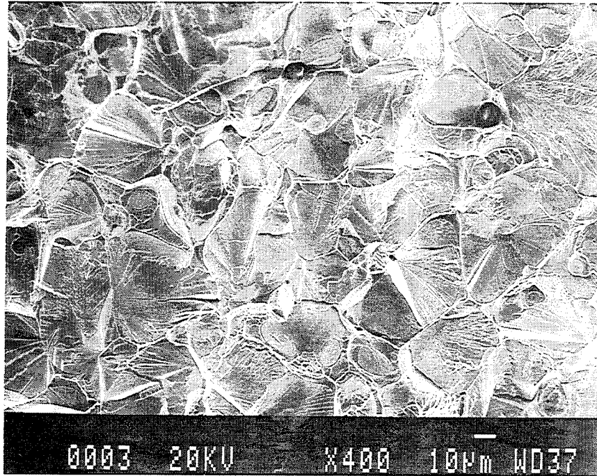
Figure 12. SEM fractograph of swaged and aged 93W-4.9Ni-2.1Fe at \dot{\epsilon} = 10^{-4} \text{ s}^{-1} .
