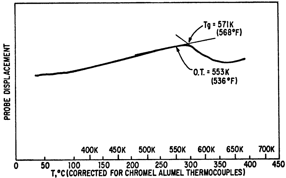
FIGURE 5 TMA CURVE OF ADHESIVE BOND LINE FROM SAMPLE 24 TABLE VII
