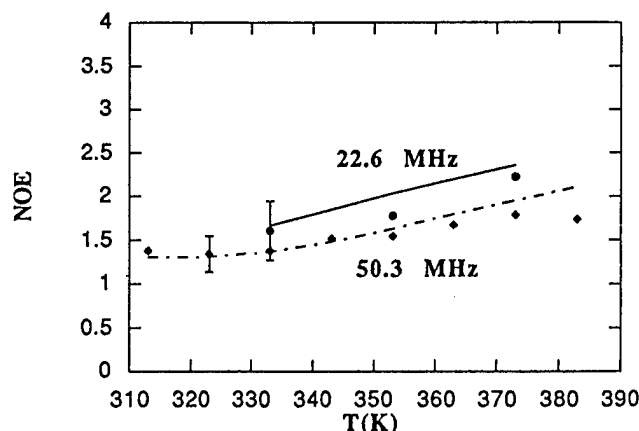
Figure 1. NOE vs Temperature at 22.6 MHz and 50.3 MHz. Lines correspond to the fit for the DLM autocorrelation function. Fits from other models are comparable to the fit shown for the DLM model.
