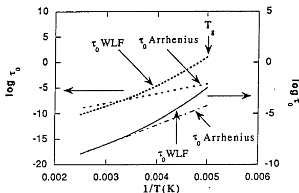
Figure 6. Comparison of the temperature dependence of \tau_0 from the Hall-Helfand model combined with restricted anisotropic rotational diffusion assuming first WLF and then Arrhenius behavior. The lower two curves compare the Arrhenius and the WLF temperature dependence of \tau_0 produced by fitting T_1 when c_1^0 was floated ( c_1^0 = 5 ); the two curves coincide at high temperatures. The upper two curves show the Arrhenius and the WLF temperature dependence of \tau_0 produced from fitting T_1 when c_1^0 was kept constant and equal to a literature value 1 ( c_1^0 = 8.61 ); the two curves do not coincide at high temperatures and it was impossible to produce an acceptable fit.
