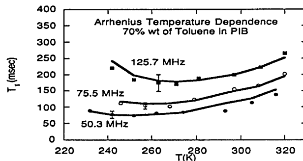
Fig. 2. Spin-Lattice relaxation times of the methylene carbon of PIB as a function of temperature and Larmor frequency. The concentration of toluene is about 70% wt. The solid lines represent fitting from the Hall-Helfand model combined with a restricted anisotropic rotational diffusion. An Arrhenius temperature dependence was given to the correlation times.
