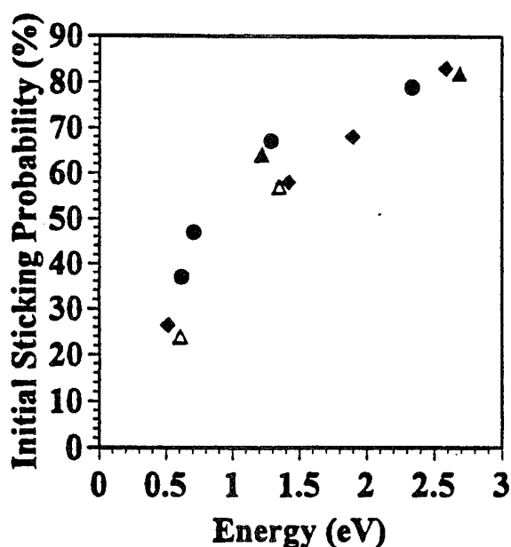
Fig. 14 Upper limit of Cl 2 and Cl sticking probabilities ( S_0 ) vs. kinetic energy. (●) and (◆) Two different runs using velocity-selected kinetic energies of Cl 2 . (▲) Two different average energies using the full kinetic energy distribution of Cl 2 (not velocity selected). (△) Two different average energies of Cl atom using the full kinetic energy distribution (not velocity selected).
