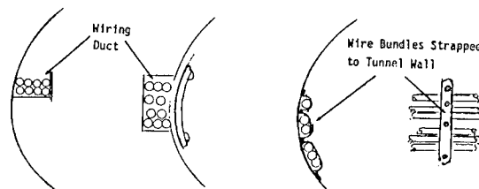
FIGURE 2-5. METHODS OF INSTALLING WIRE AND CABLE IN TUNNELS
