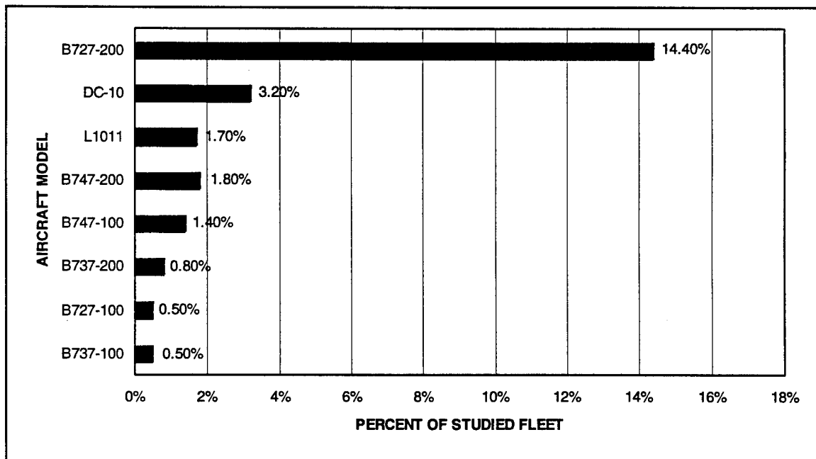
FIGURE 4. COCKPIT LAYOUT OF STUDIED FLEET - ANALOG, THREE-PERSON CREW
