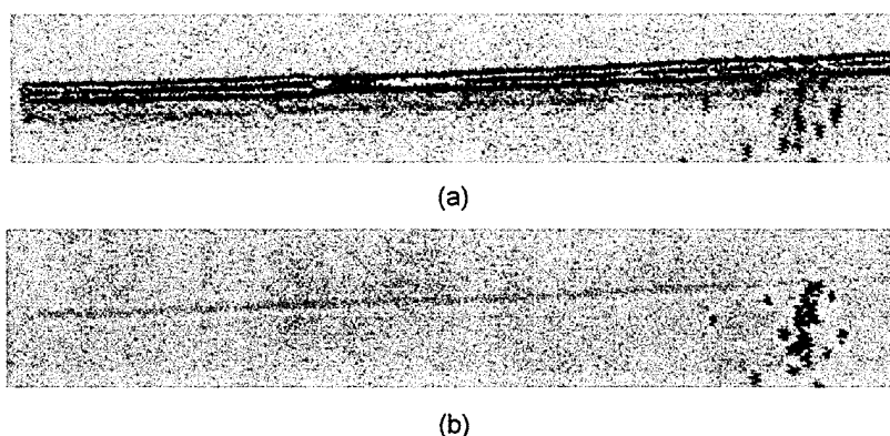
Figure 3-54. Ultrasonic image from Ti-14Al-21Nb/SiC sample which was consolidated by vacuum hot pressing + HIPing (Panel A) -- (a) oblique-incidence (24°) shear wave, and (b) normal-incidence longitudinal wave.
