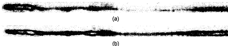
Figure 3-55. Ultrasonic images from Ti-14Al-21Nb/SiC single fiber composite (Panel B) using shear wave interrogation with different angles of wave front incidence: (a) 18° and (b) 24°.
