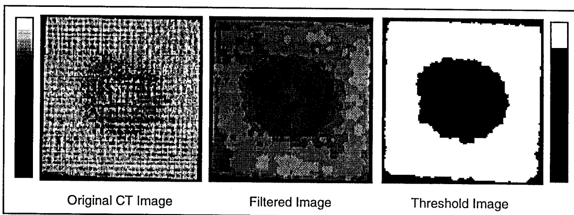
Figure 27. Damage evaluation process on impact panels
