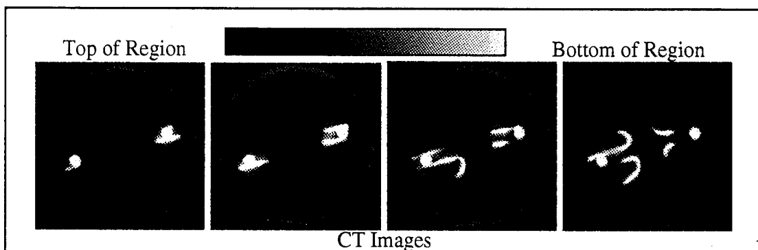
Figure 43. DR and CT images of a crystal oscillator
