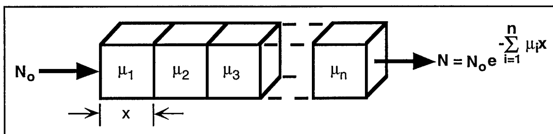
Figure A1. X-ray attenuation
