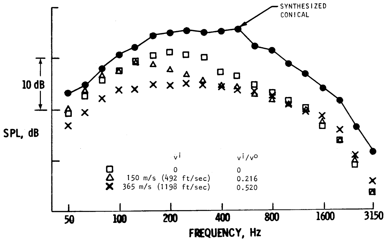
Figure 5.- Typical inverted conannular plug nozzle spectral characteristics. 732 m (2400 ft) sideline; data scaled to .33 \text{ m}^2 ( 513 \text{ in}^2 ); v^0 = 701 \text{ m/s} ( 2300 \text{ ft/sec} ); T_T = 967 \text{ K} ( 1740^\circ \text{ R} ); \theta_I = 130^\circ ; configuration No. 3; A_R = .53 .
