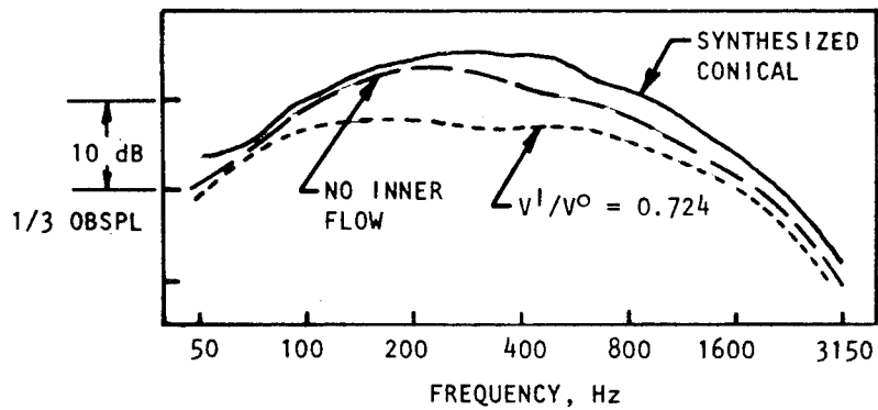
Figure 6.- Additional typical inverted coannular plug nozzle spectra. 732 m (2400 ft) sideline; data scaled to .33 \text{ m}^2 ( 513 \text{ in}^2 ); \theta_I = 130^\circ ; v^o = 701 \text{ m/s} ( 2300 \text{ ft/sec} ).
