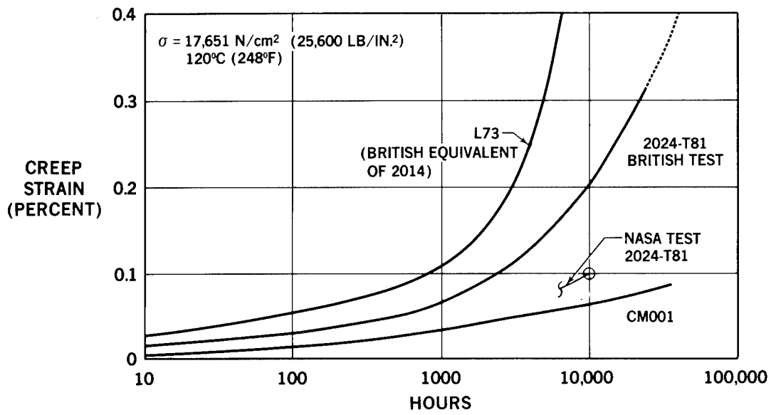
Figure 6.- Creep strain of aluminum materials.
