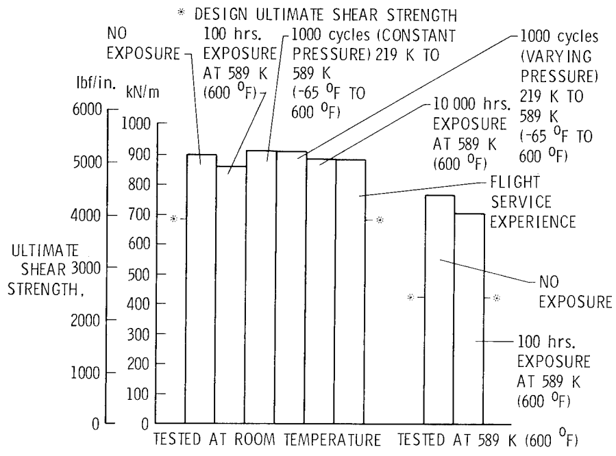
Figure 8.- Weldbraced panel shear test results.
