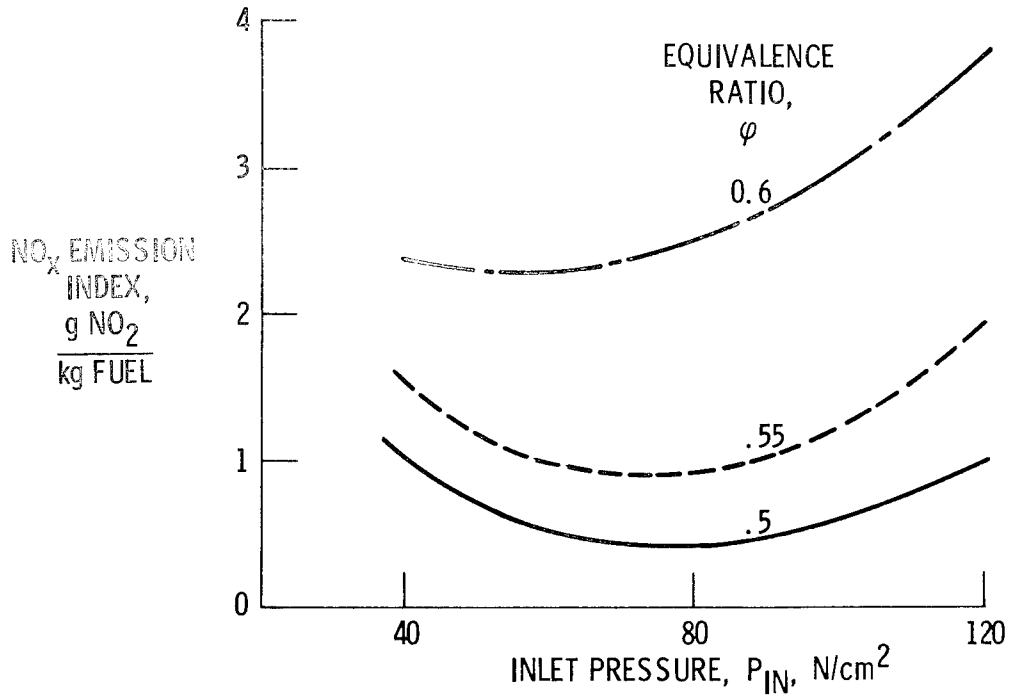
Figure 13.- Effect of inlet pressure and equivalence ratio on NO x emissions from GASL experiment. Inlet temperature, 900 K; Jet-A fuel.
