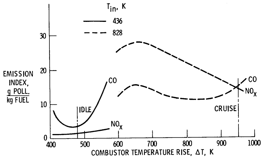
Figure 8.- Effect of optimized idle equivalence ratio on cruise emissions of fixed geometry configuration of SOLAR VAB concept. Inlet pressure, 14 \text{ N/cm}^2 ; Jet A-1 fuel.
