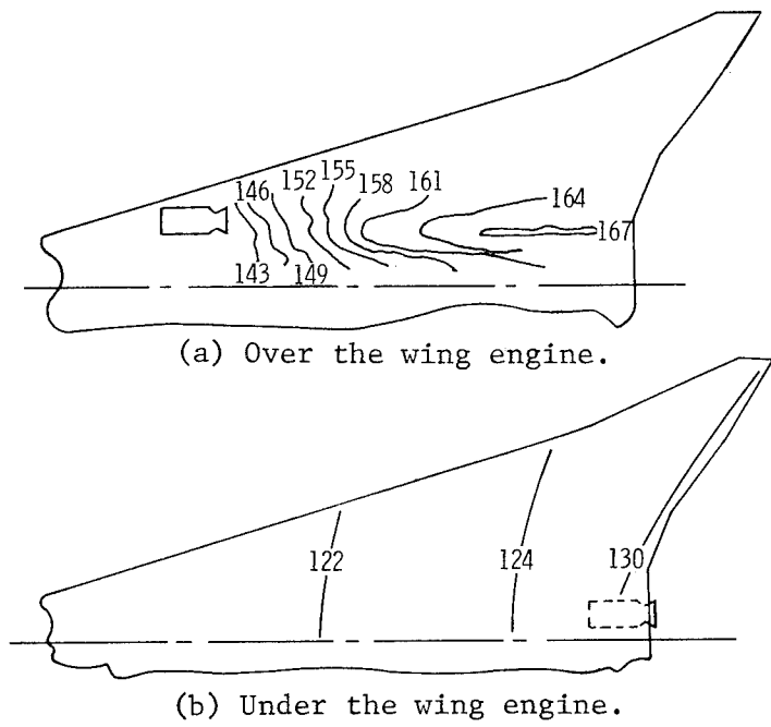
Figure 6.- Fluctuating pressure contours, dB.
