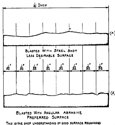
FIGURE 4: The less desirable smooth "rolling hill" type of profile produced by shot as compared to the preferred roughness showing distinct anchorages as made by an angular abrasive.
