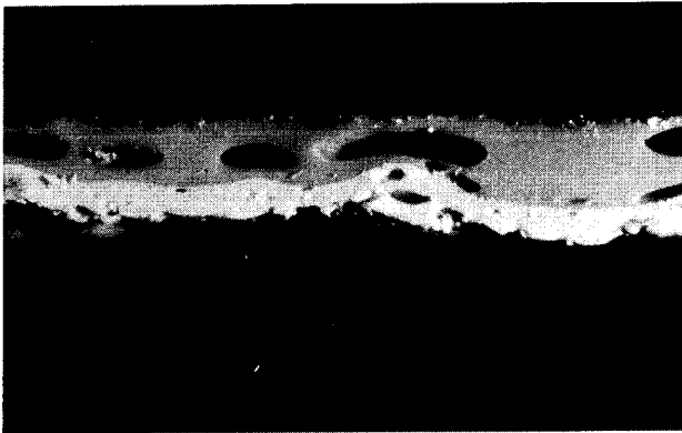
FIGURE 13: Photomicrograph of the cross-section of a Saran film taken from a submarine tank. The same type of porosity is present as indicated for normal spraying.
