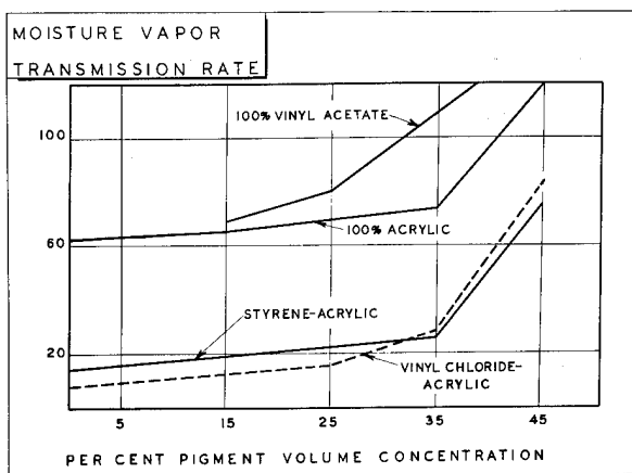
FIGURE 3: Effect of Pigment Volume Concentration on the M.V.T.R. of Latex Polymers - M.V.T.R. in Grams/100 in. 2 /24 hours - General Foods Cabinet.
