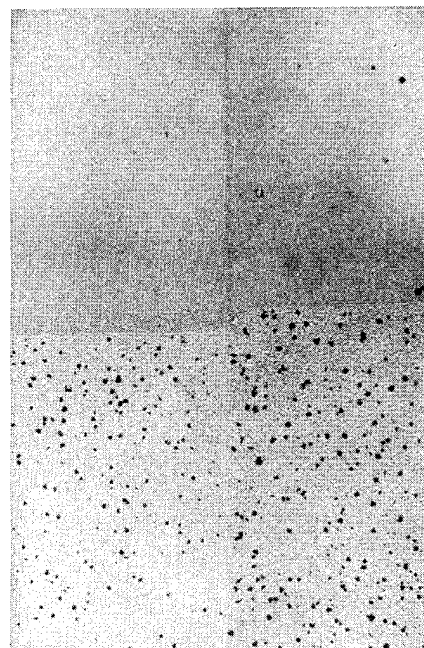
FIGURE 6: Preferential atmospheric corrosion of plated surfaces of varying profiles. The roughest area, No. 4, has greater moisture condensing surface and occluded sand to promote maximum corrosion.
