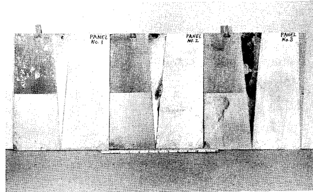
FIGURE 14: Cathodic protection evaluation test panels with the "V" holiday bare steel area, showing degrees of protection of inorganic zinc coatings. #117 wash primer and #119 red lead vinyl are evaluated also as a top coat system.
