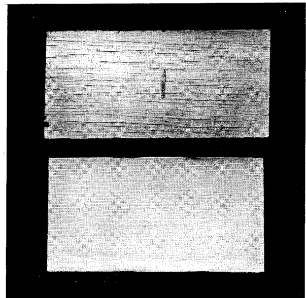
FIGURE 4: 25 Cycle Boil Test – Conventional Commercial Finish (top) Versus EC-167 Coated Bare Plywood (bottom).
