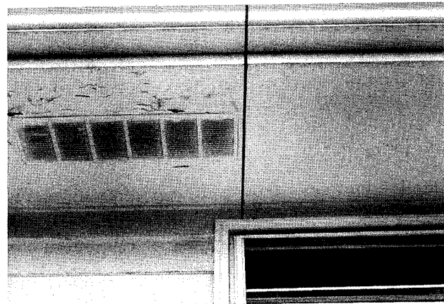
FIGURE 2: Close-Up of Paint Under Eaves - A Smooth, Hydrophobic Surface. Left-hand portion - Vinyl Acetate - 45% Alkyd - Eave Failure. Right-hand portion - Vinyl Chloride - Acrylic - 45% Alkyd - No Eave Failure.
