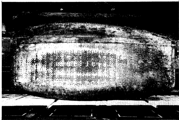
FIGURE 11: Typical wear of the vinyl coating on the stainless steel sonar dome on the USS ISHERWOOD after 2 years of service. The wear is only down to vinyl primer.
