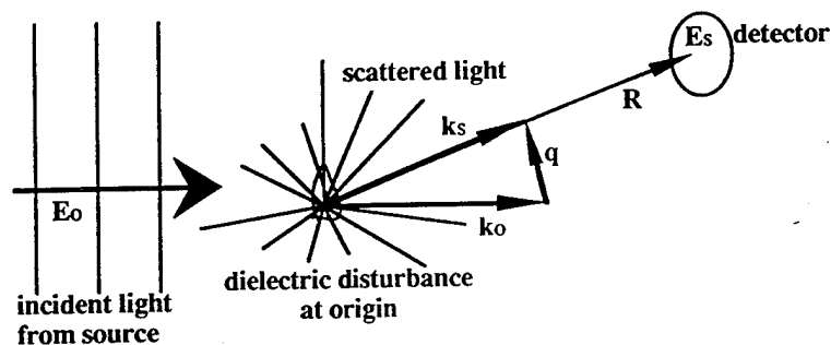
Figure 4-1 Scattering geometry for equation 4-1.
