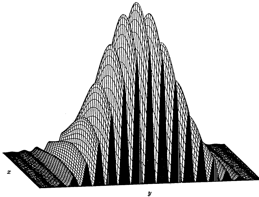
Figure 4-3 Sample crosssection in the plane z = 0 of the electric field intensity grating caused by the intersection of two Gaussian beams, as in Figure 4-2.
