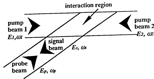
Figure 2-1 Schematic diagram of a common DFWM geometry. The pump beams counterpropagate through the medium. The probe and signal beams intersect these beams at a small angle. The interaction region is defined by their intersection.
