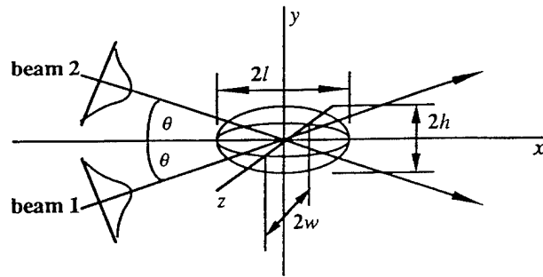
Figure 4-2 Geometry of the intersection region used in this analysis.
