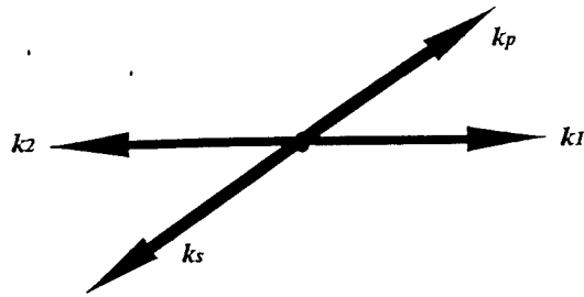
Figure 2-2 Vector diagram of momentum conservation or phase-matching for DFWM with the geometry shown in Figure 1.
