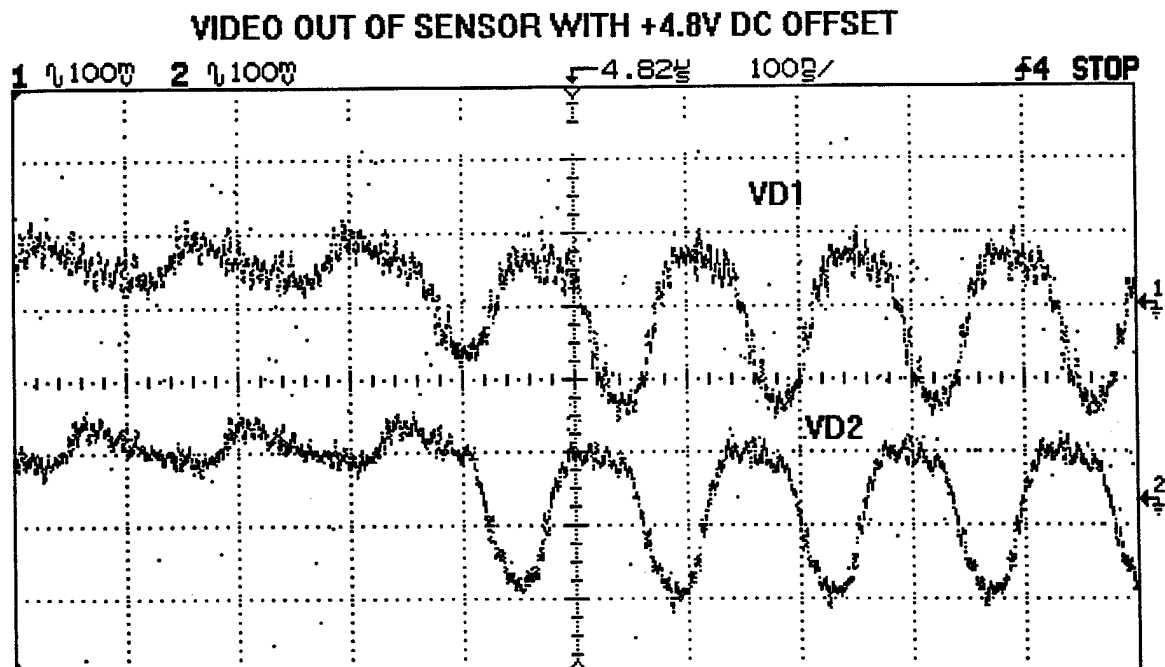
Fig. 8.5 - Normal video out of CCD at 7.2MHz.
