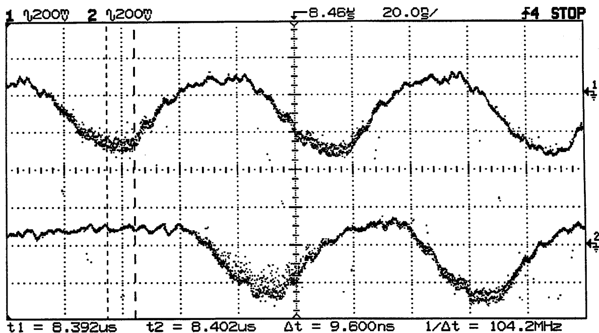
Fig. 8.6 - Video out at 13.3MHz.
