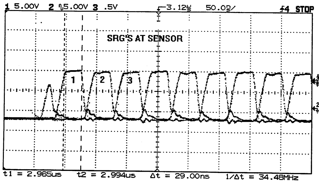
Fig. 8.3 - SRGS at normal pixel rate of 7.2MHz per channel.
