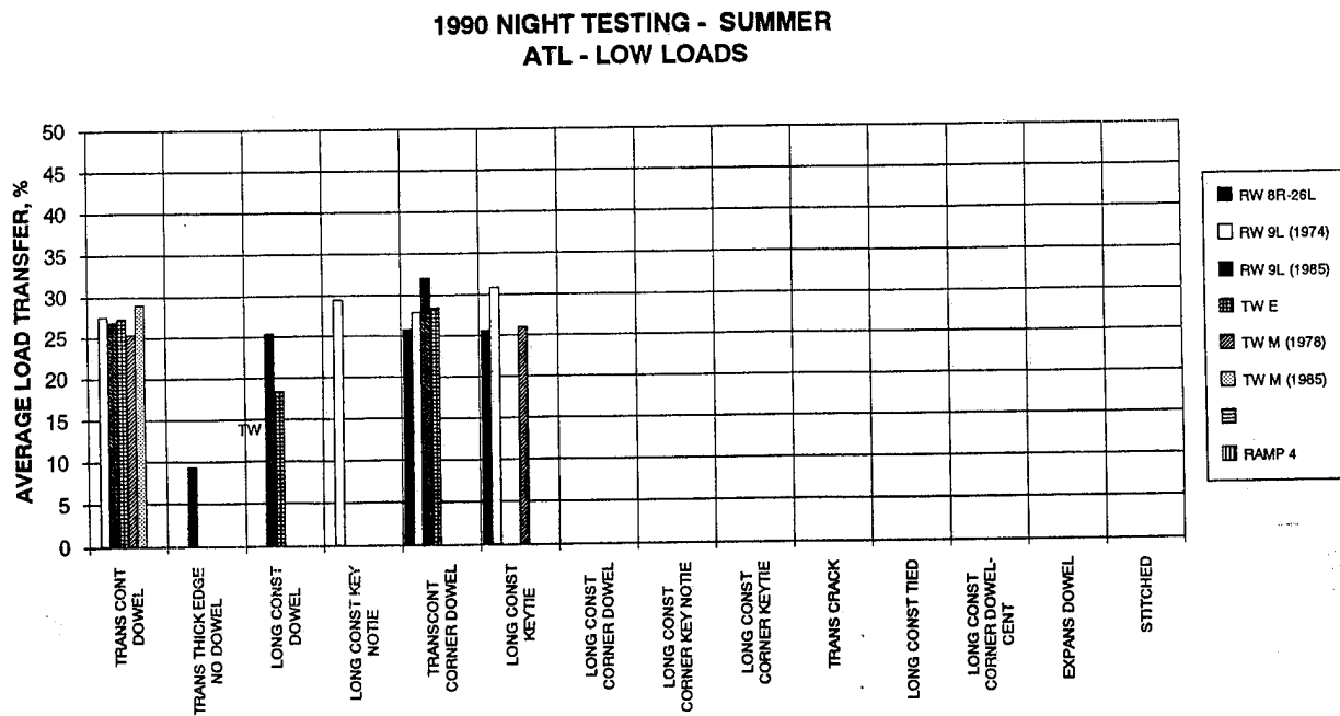
FIGURE 24. SUMMARY OF LOW-LOAD TESTS, 1990 NIGHT TESTING, SUMMER CONDITIONS, ATLANTA
