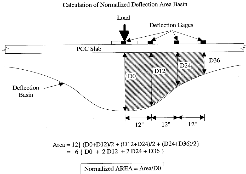
FIGURE 14. DETERMINATION OF AREA FROM MIDSLAB DEFLECTION BASIN
