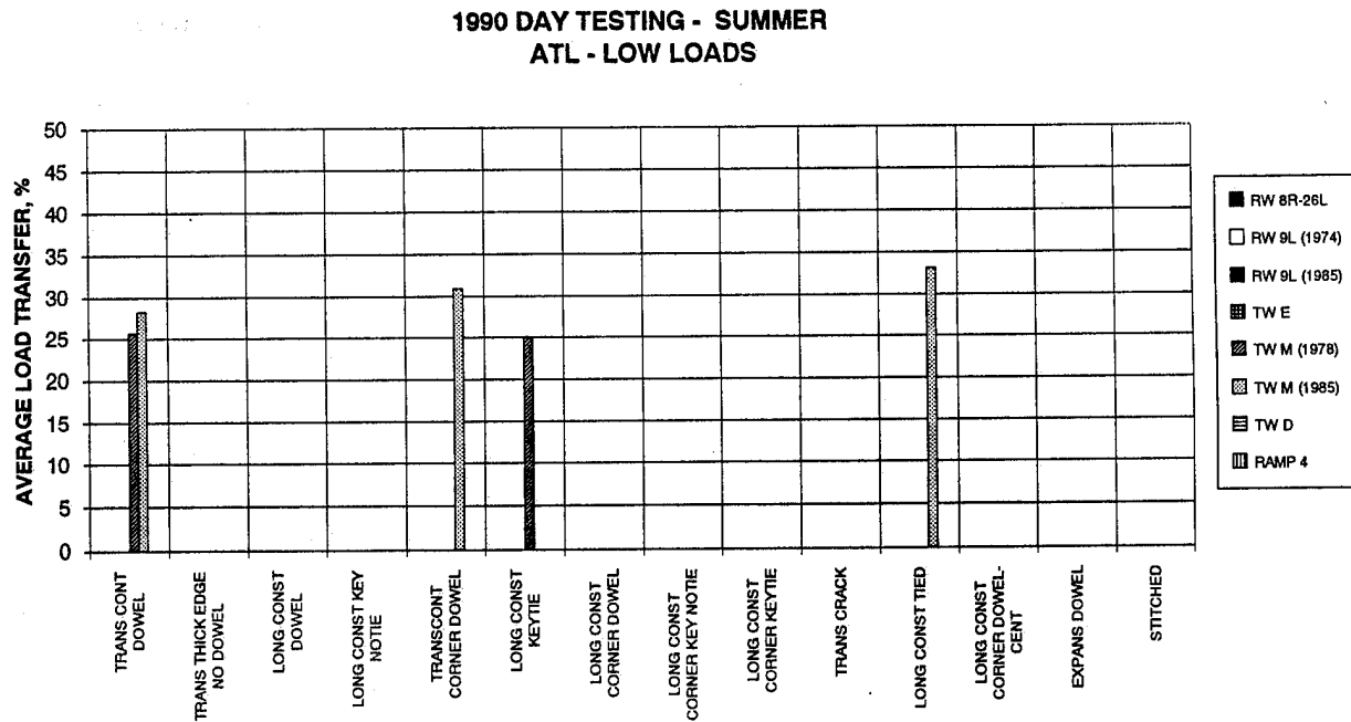
FIGURE 23. SUMMARY OF LOW-LOAD TESTS, 1990 DAY TESTING, SUMMER CONDITIONS, ATLANTA
