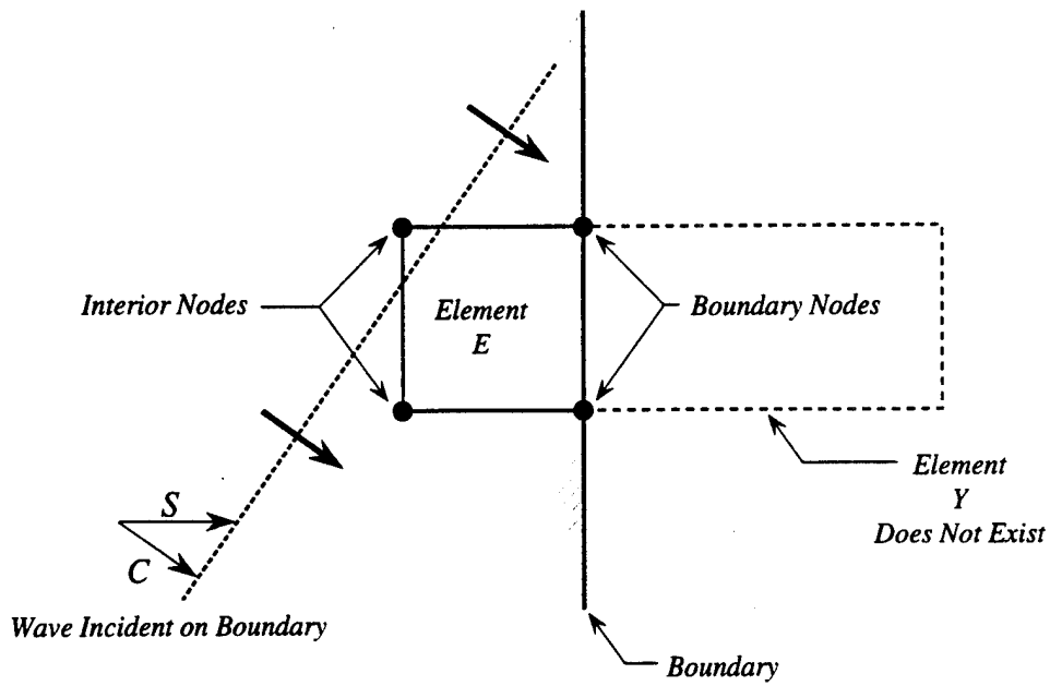
Figure 3-1. Arrival of a wave at the boundary of a finite element grid.
