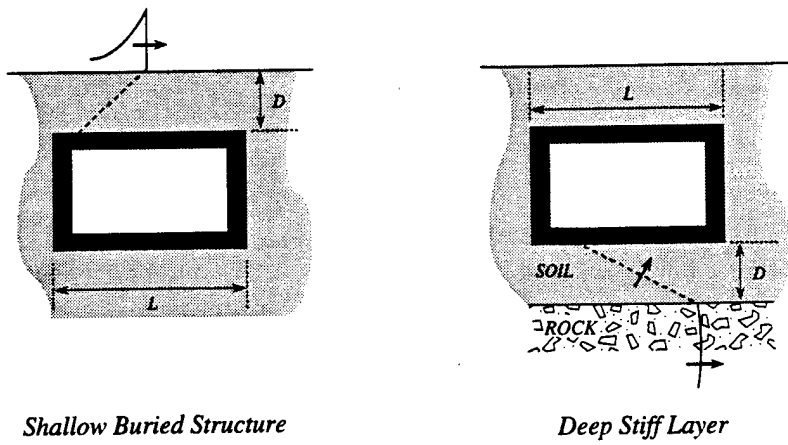
Figure 5-1. Examples for which the free field solution is a poor choice of datum problem.
