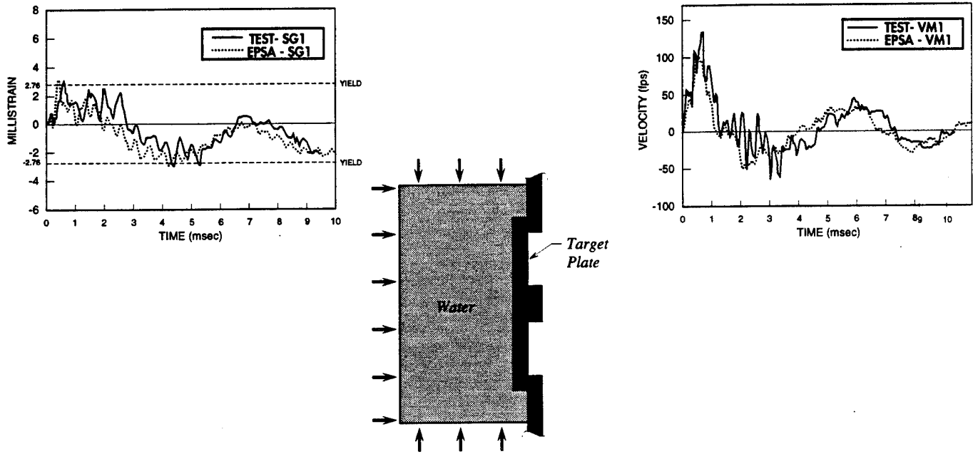
Shock is Applied at Boundary of Hexahedral Mesh and Propogates through Water to Target Plate
