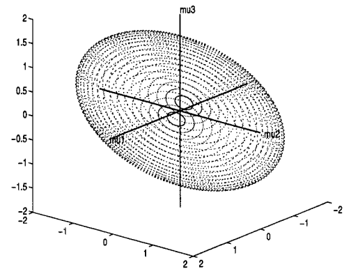
Figure 3.5 Wheel Momenta Ellipsoid (Pyramidal Wheels)
