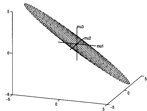
Figure 3.7 Wheel Momentum Ellipsoid (Nearly Co-planar Wheels)
