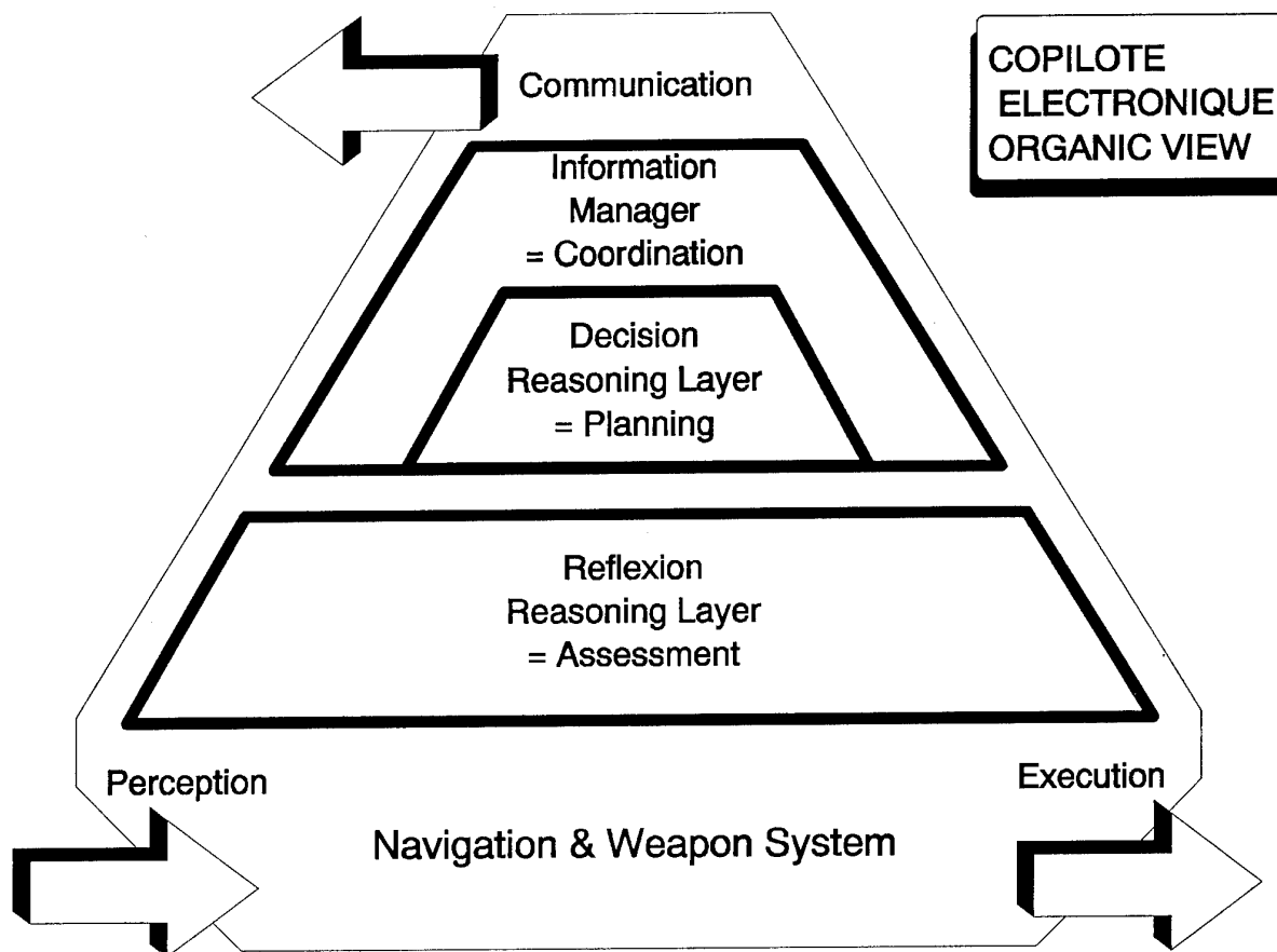
Figure 4 : Copilote Electronique Organic View
