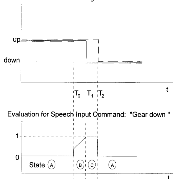
Pilot's Model of Gear Setting
