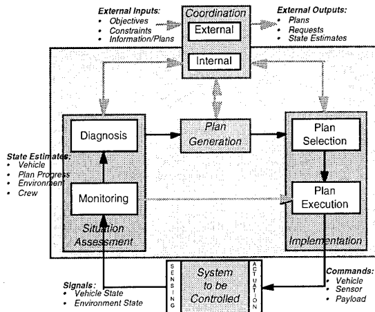
Figure 1.3b Knowledge-Based Guidance and Control System
