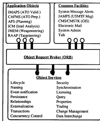
Figure 3. CTAPS ORB Architecture
