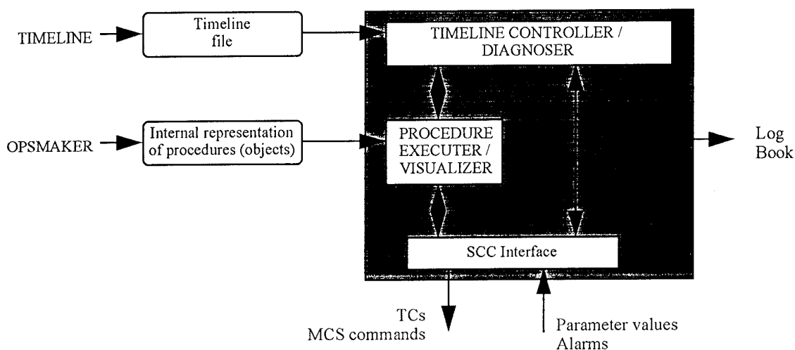
FIGURE 6.1 - OPSEXCUTER ARCHITECTURE
