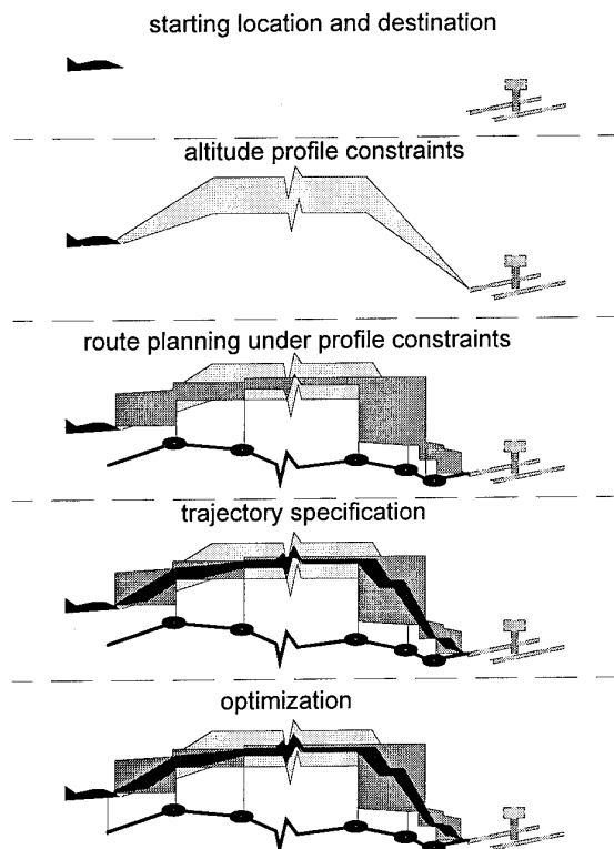
Figure 9. Trajectory Planning
