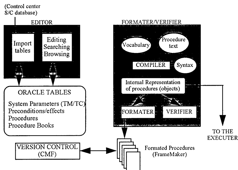
FIGURE 4/2 - OPSMAKER ARCHITECTURE
