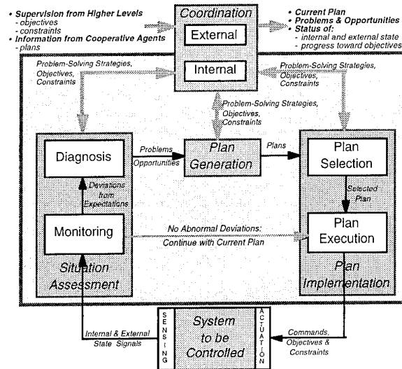
Figure 1.3a Detailed Decomposition
