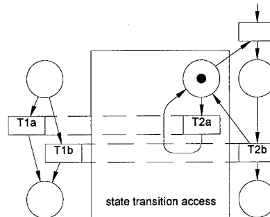
Figure 11. Coupling mechanisms
