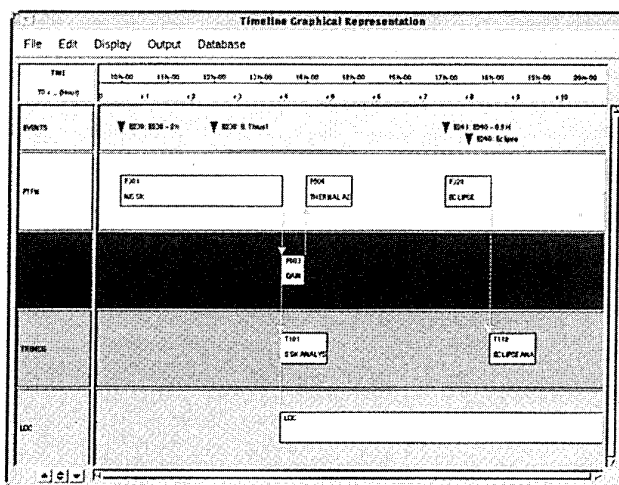
FIGURE 5/1 - A PART OF THE TIMELINE USER INTERFACE
