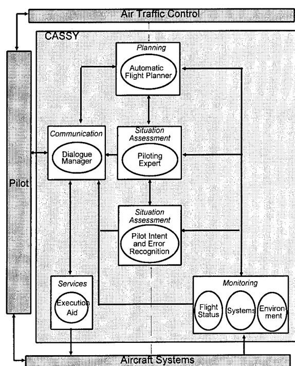
Figure 5. CASSY structure
