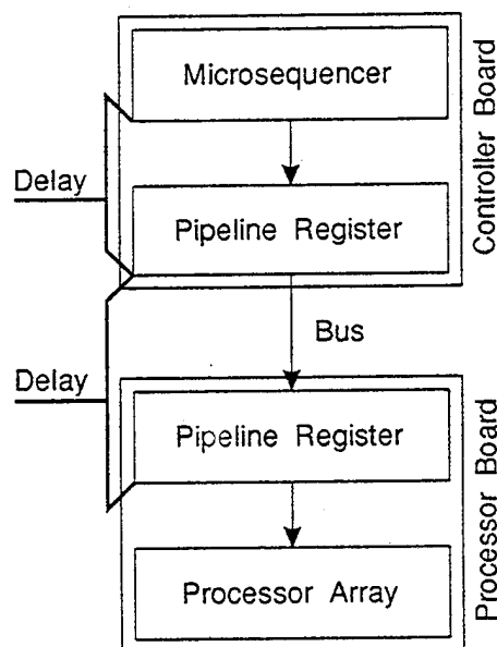
Figure 6.6: Gauss Machine Pipeline Delay Model
