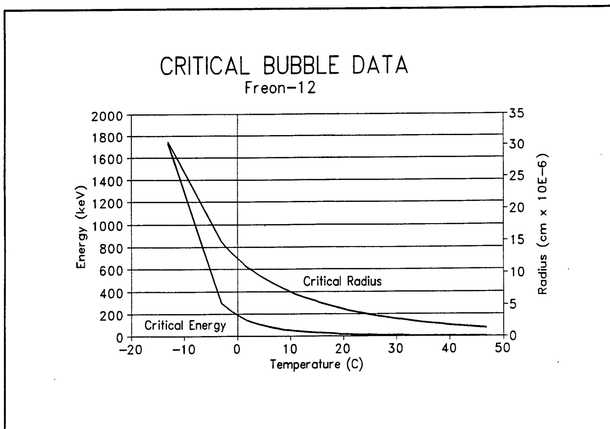
FIGURE A-1. Critical energy and bubble radius for Freon-12 as a function of temperature at 1 atmosphere.
