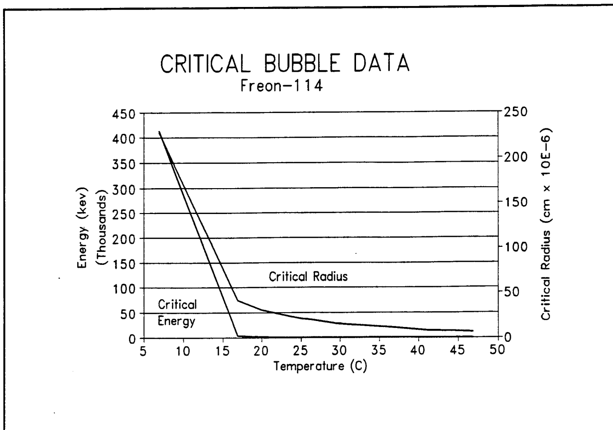
FIGURE A-5. Critical energy and bubble radius for Freon-114 as a function of temperature at 1 atmosphere.
