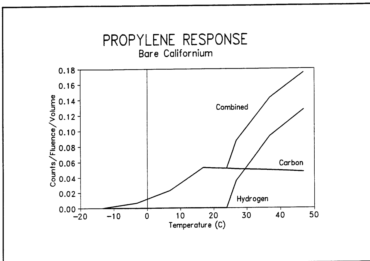
FIGURE 3-14. Theoretical model's predicted response for propylene ( C_3H_6 ) to bare Californium neutron spectrum at 1 atmosphere.
