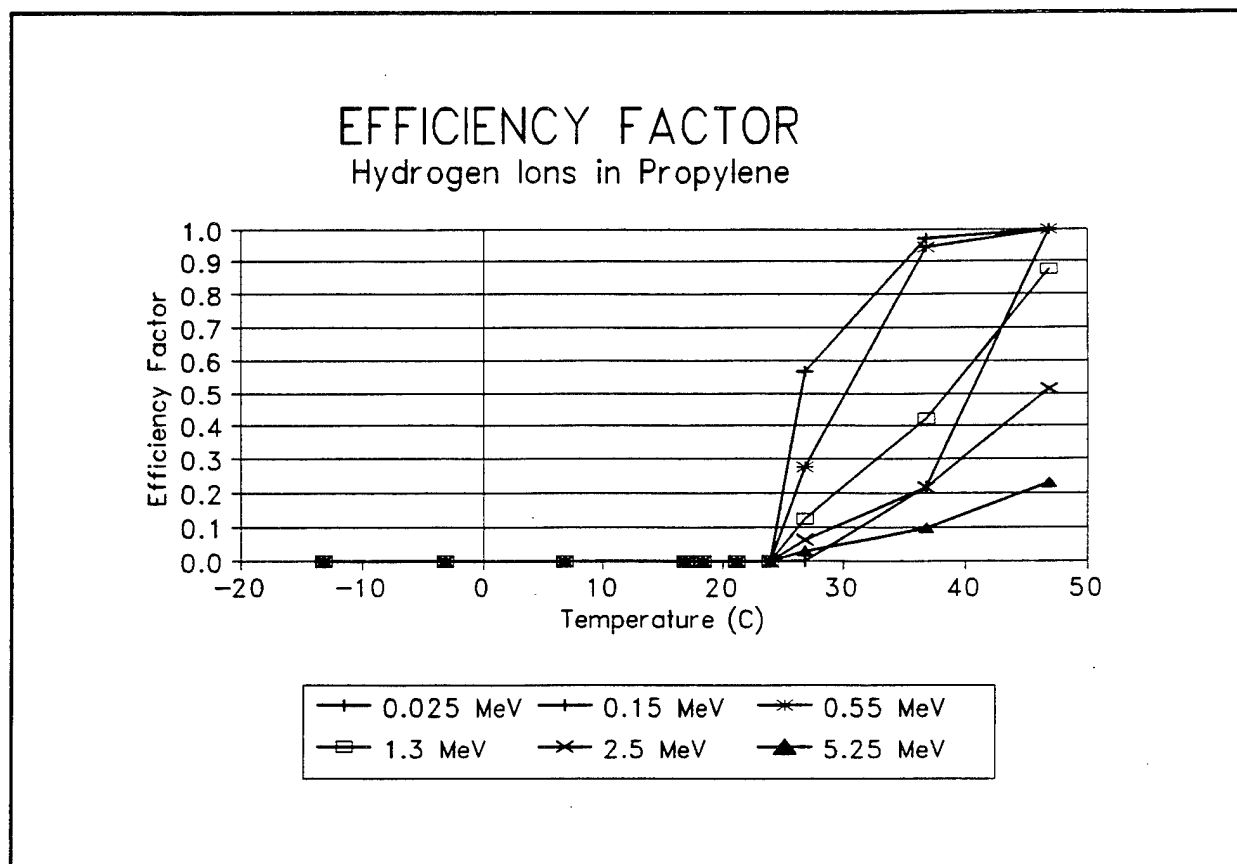
FIGURE 3-13. Efficiency factor F(E_n, T) for hydrogen ions in propylene as a function of temperature.
