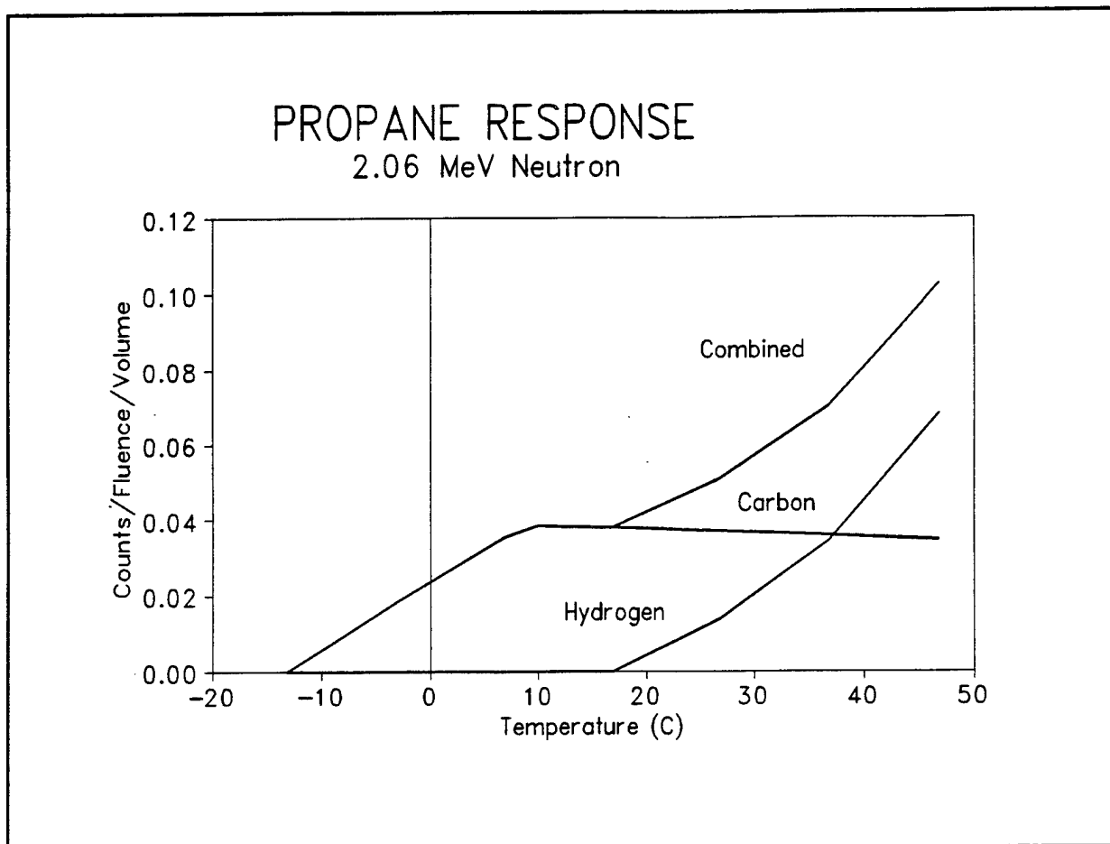
FIGURE 3-15. Theoretical model's predicted response for propane ( C_3H_8 ) to bare Californium neutron spectrum at 1 atmosphere.
