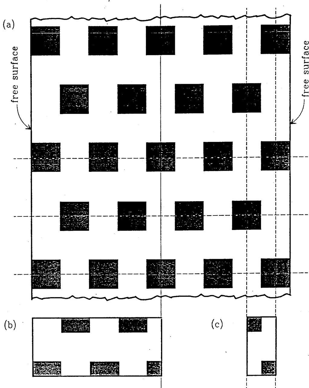
Figure 3.1-2 Ordered array with 25% soft grains (shaded). (a) The infinite strip with two free surfaces, shown here with a width of 9 grains. It is symmetrical about the center line. (b) The minimum cell required to represent the array in (a). (c) The minimum cell to represent the infinite, surface-free version of (a). The horizontal dashed lines denote representative planes of symmetry in the strip and infinite space, and the vertical dashed lines denote additional symmetry planes in the infinite space.
