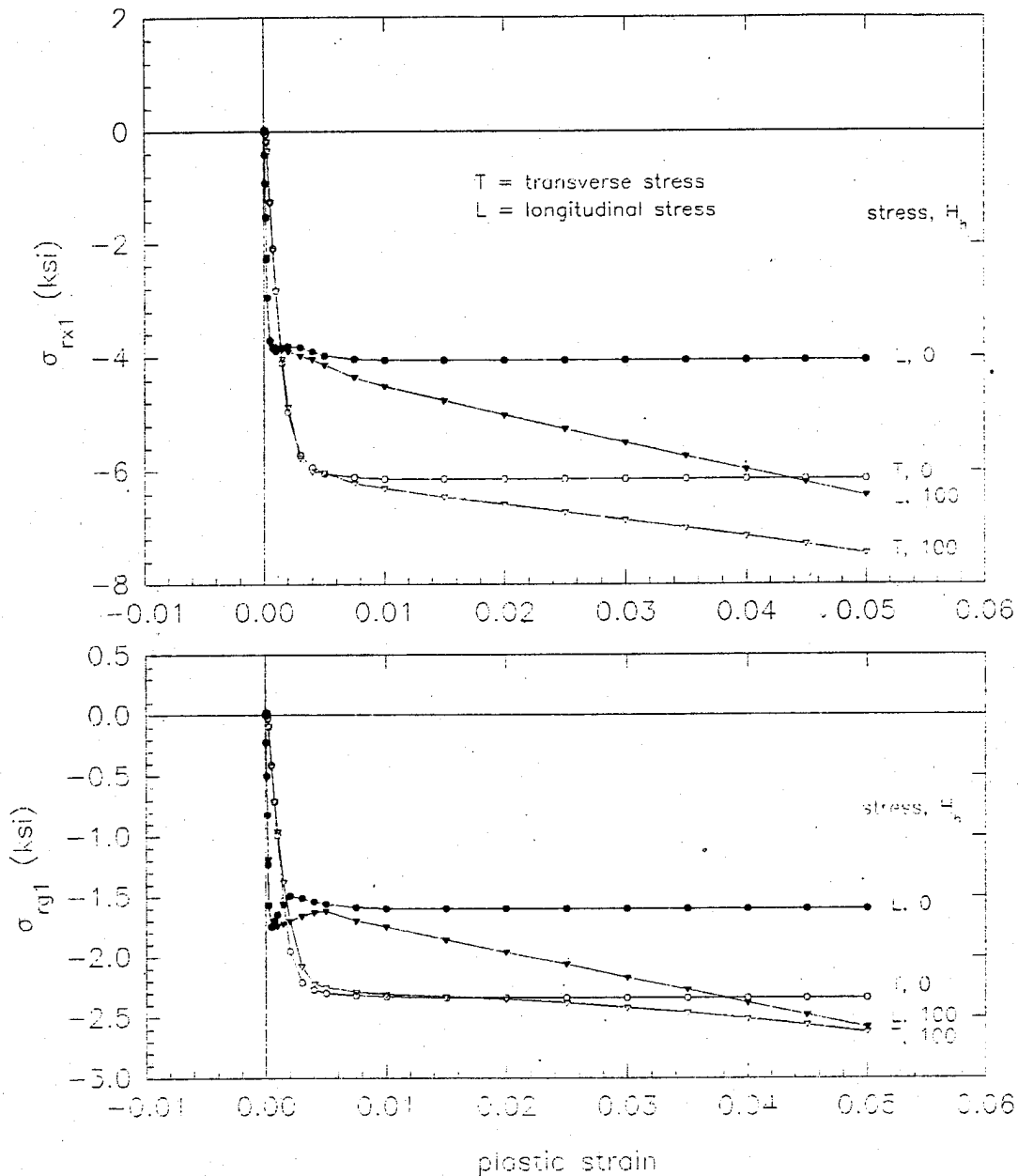
Figure 4.2.2.9-14. The transverse x-ray-averaged residual stress ( \sigma_{Tx1} ) and the transverse surface-grain-averaged residual stress ( \sigma_{Tg1} ) versus plastic strain for models under generalized plane strain for a yield point spread of 15 ksi, with and without hard grain hardening. The corresponding residual longitudinal stresses are also shown for comparison. ( f_s = 0.33 , E = 30,000 ksi, \nu = 0.29 , \sigma_{ys} = 15 ksi, \sigma_{yh} = 30 ksi, H_h = 0 or 100 ksi, H_s = 0 ksi.)
