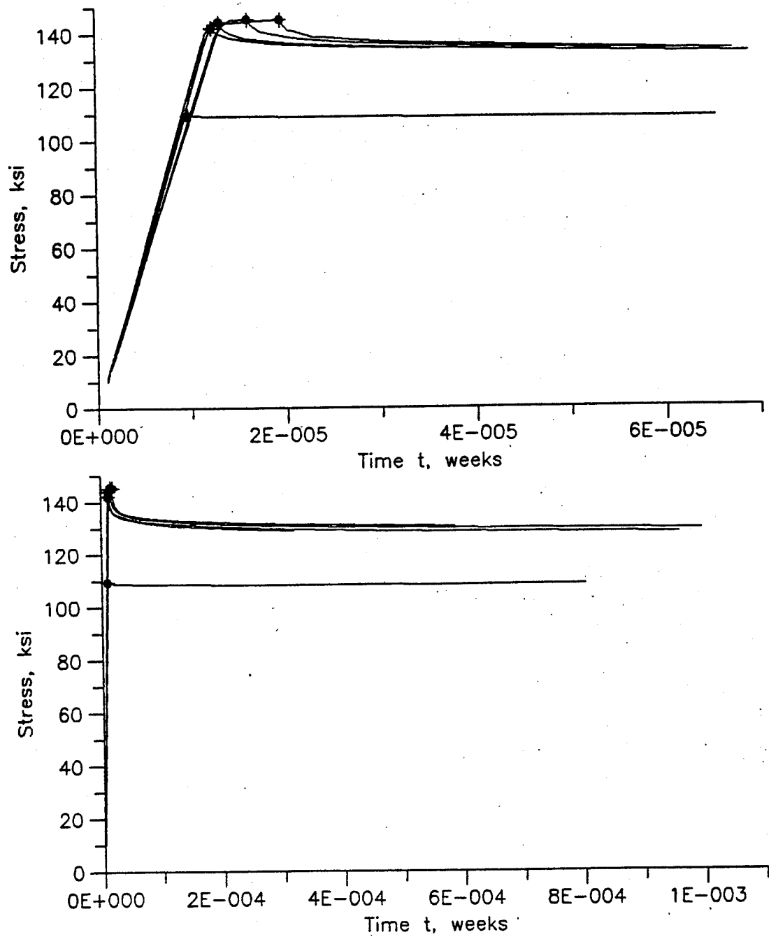
Figure 17. Static relaxation Ti-6Al-4V initial transients.
