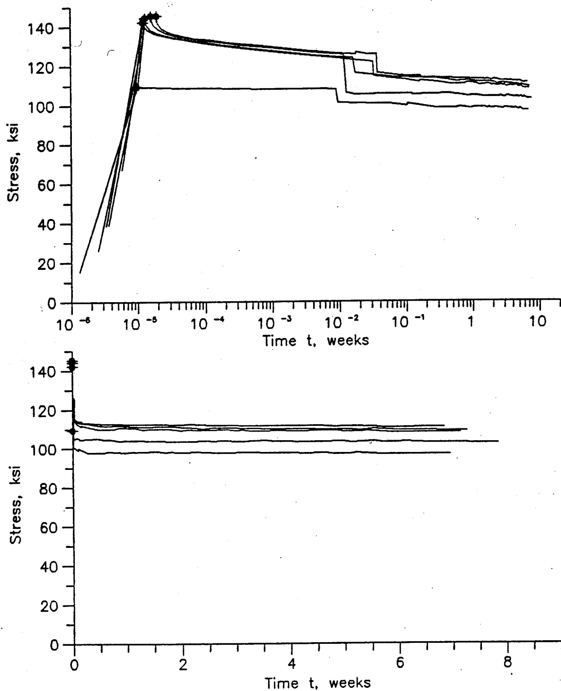
Figure 16. Static relaxation Ti-6Al-4V for test duration.
