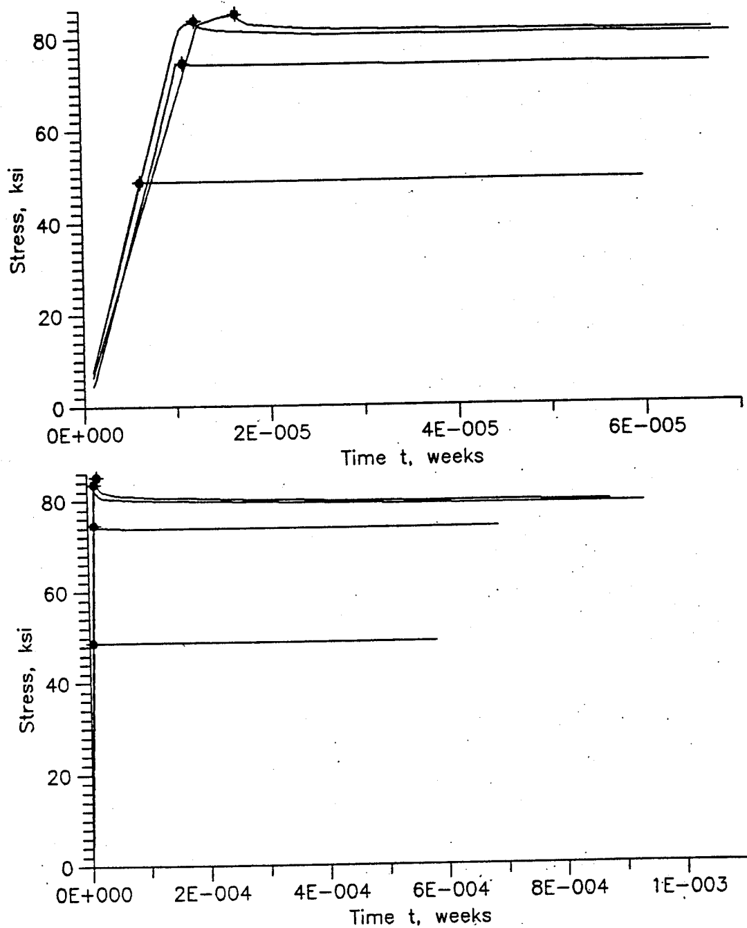
Figure 15. Static relaxation 7475-T651 initial transients.
