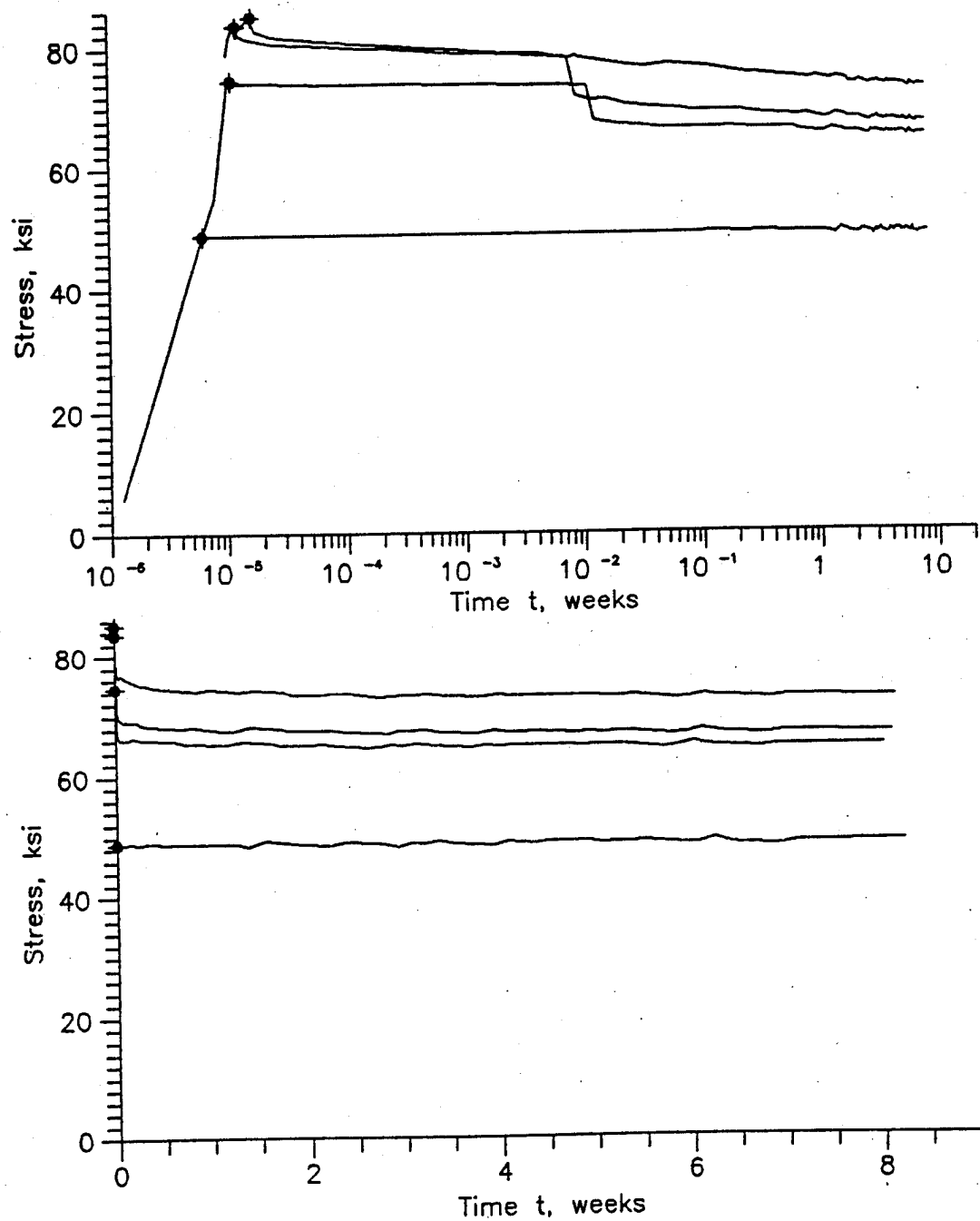
Figure 14. Static relaxation 7475-T651 for test duration.
