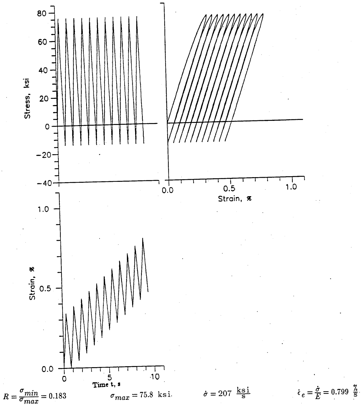
Figure 3. Computer simulated stress control including time/cycle dependent material transients.
