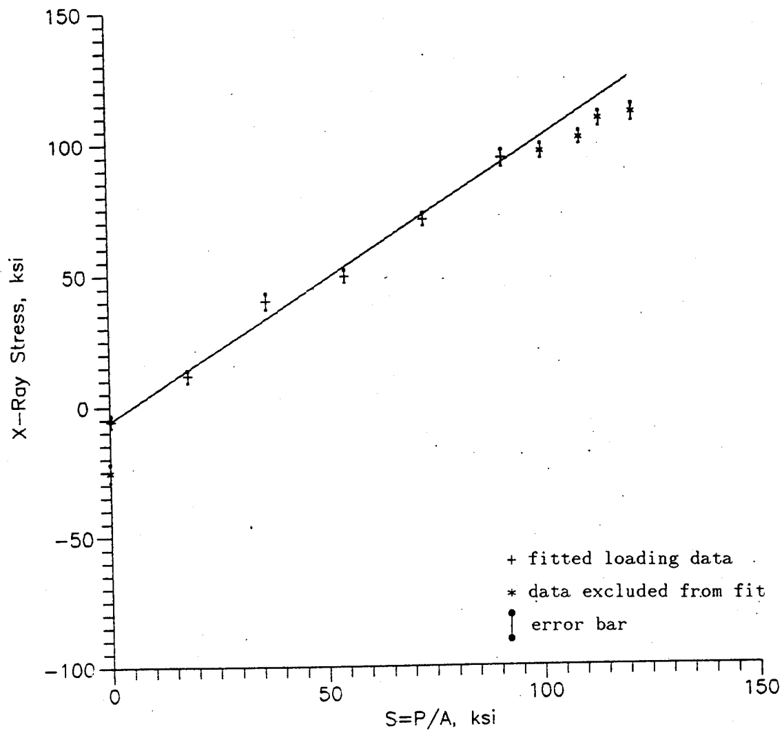
Figure 19. Agreement of x-ray with P/A for unnotched Ti-6Al-4V, specimen T1S02.
