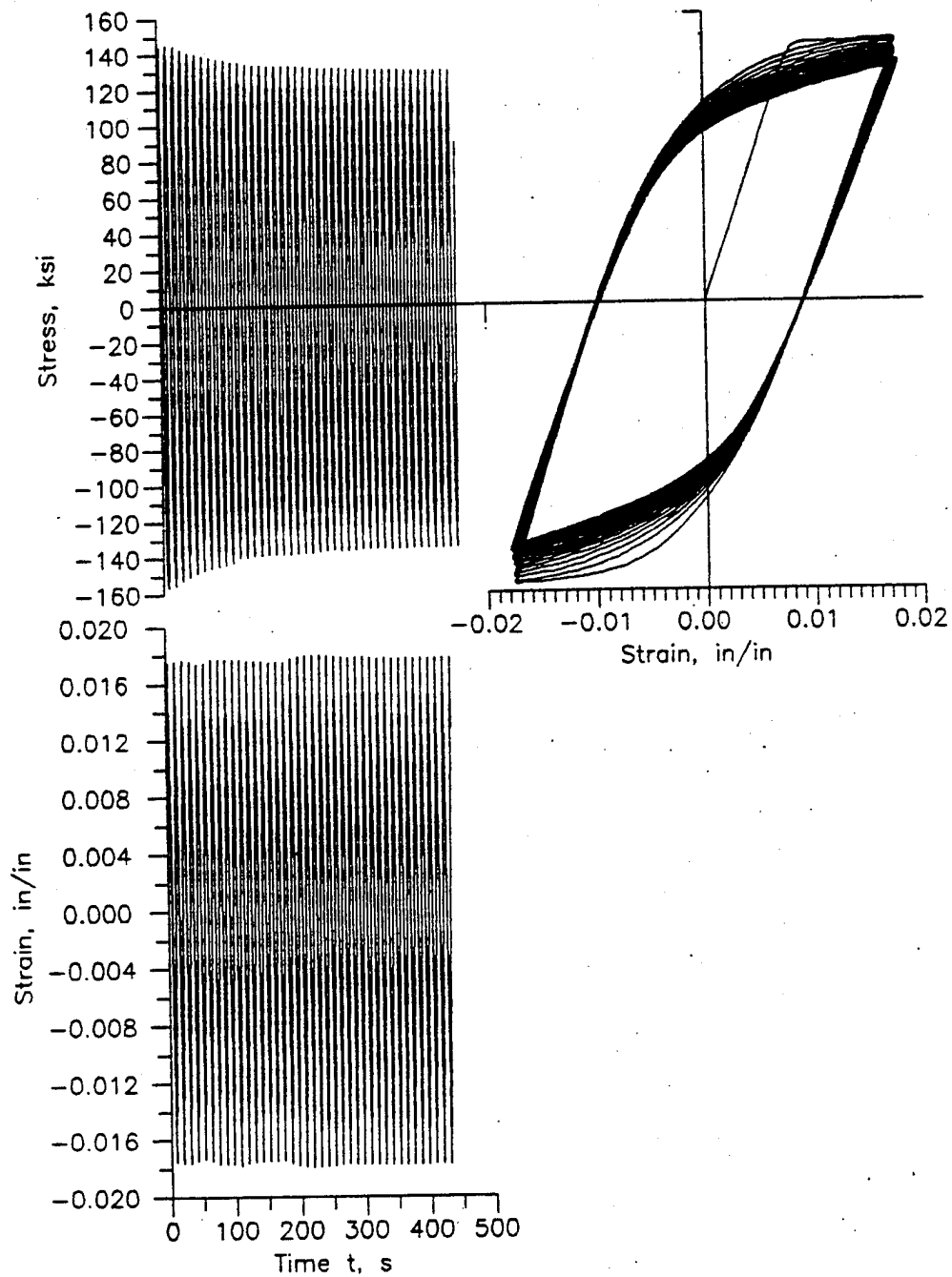
Figure 2. Cyclic softening Ti-6Al-4V. uniaxial strain control test. specimen T1A05A.
