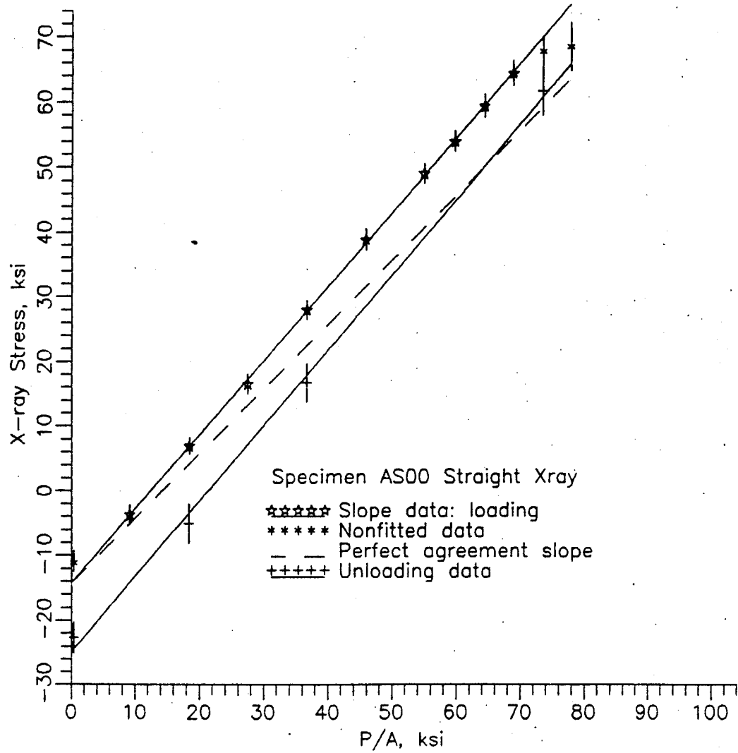
Figure 20. Agreement of x-ray stress with P/A for unnotched 7475-T651 Al.
