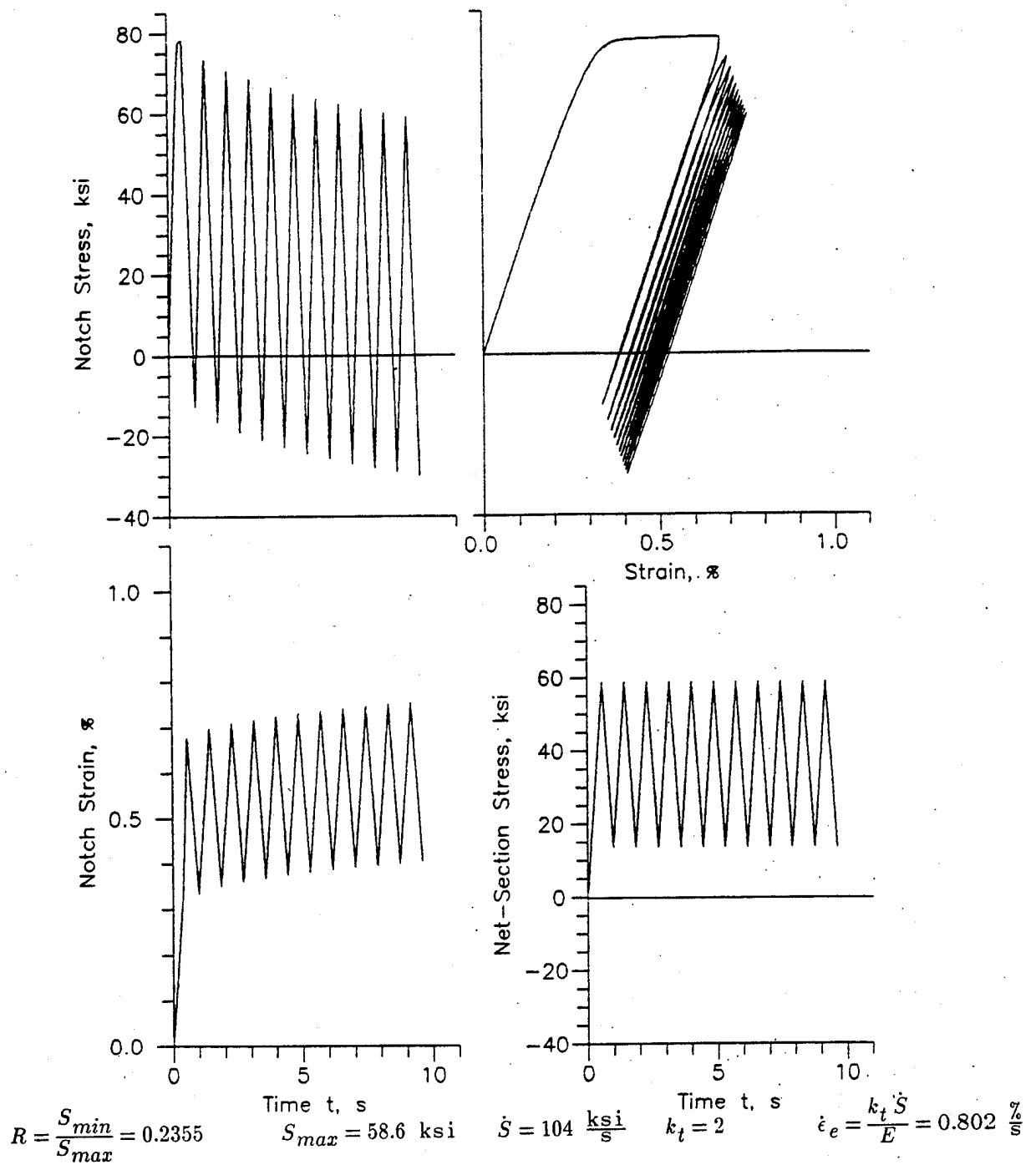
Figure 5. Computer simulated Neuber control including time/cycle dependent material transients.
