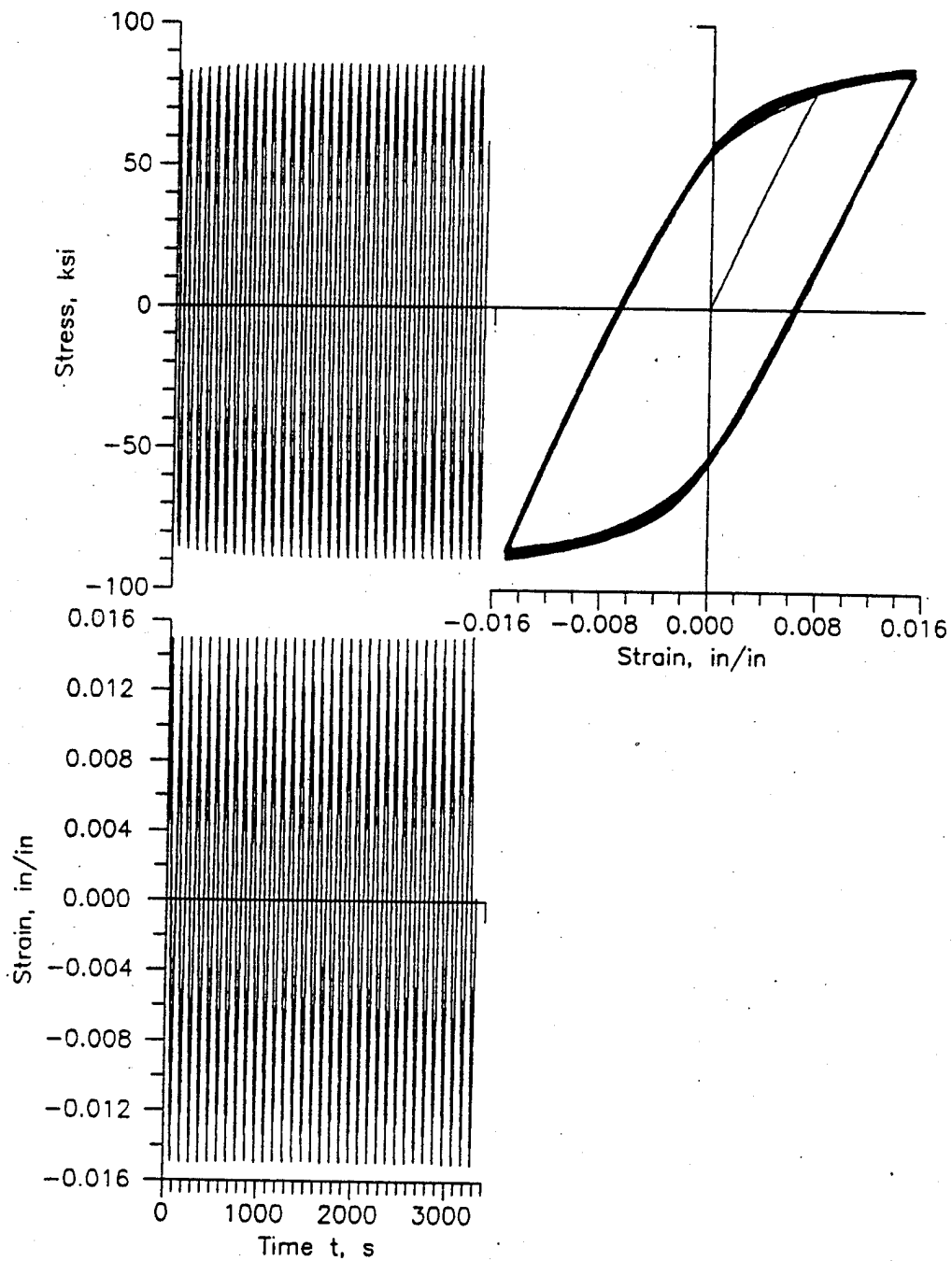
Figure 1. Cyclic hardening 7475-T651 Al. uniaxial strain control test. specimen A2A06C.
