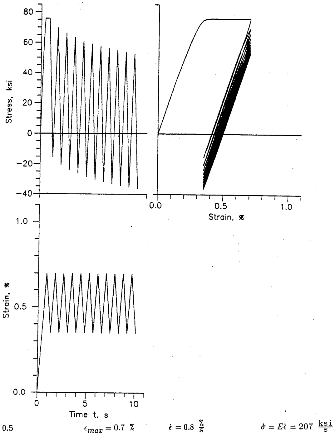
Figure 4. Computer simulated strain control including time/cycle dependent material transients.
