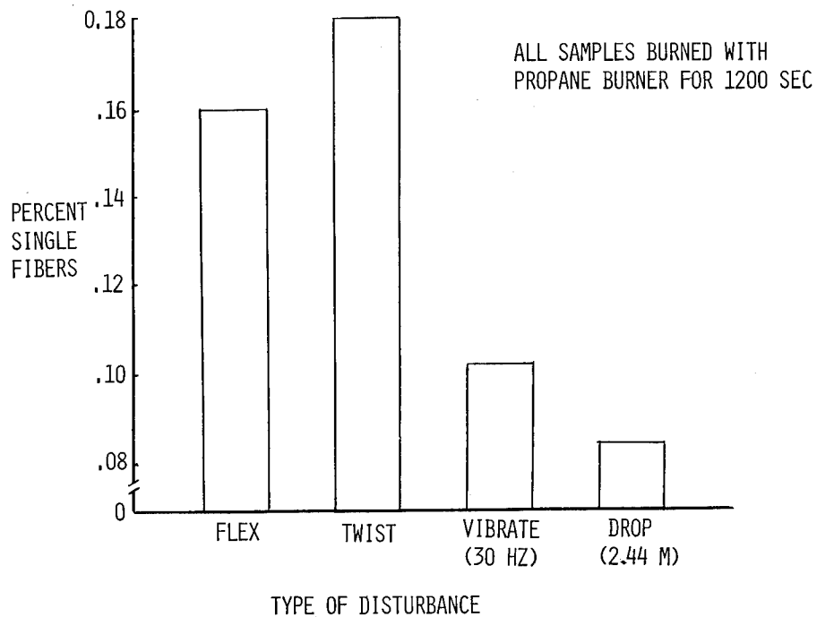
Figure 10.- Effects of internal disturbances on single fiber release (Navy/Dahlgren chamber).
