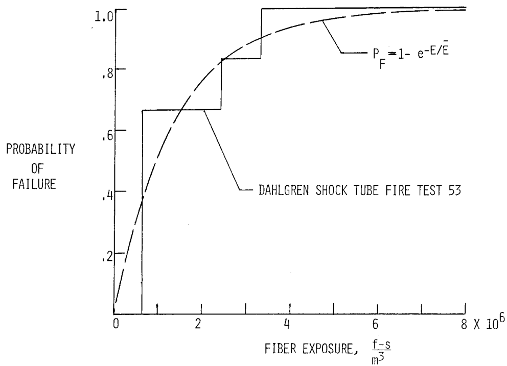
Figure 10.- Probability of electronic equipment failures from exposure to fire-released carbon fibers and to virgin carbon fibers.
