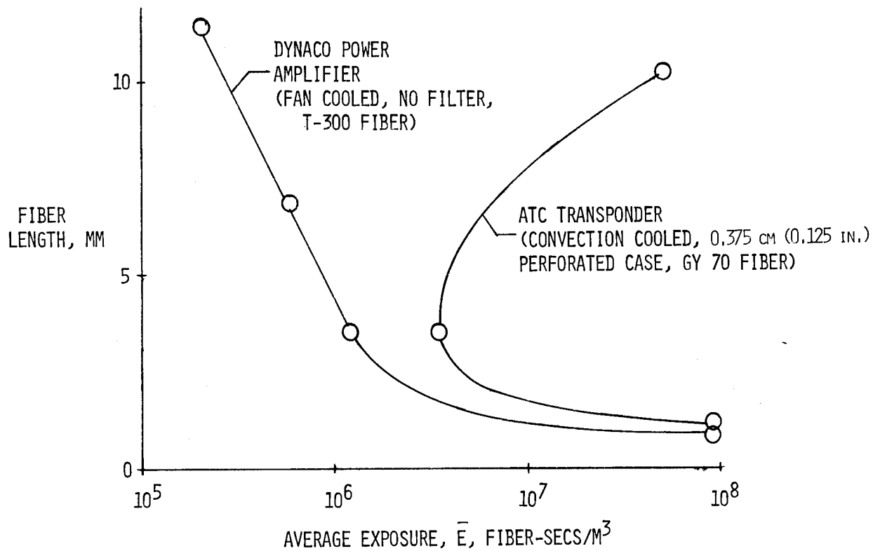
Figure 5.- Fiber length effect on equipment vulnerability.
