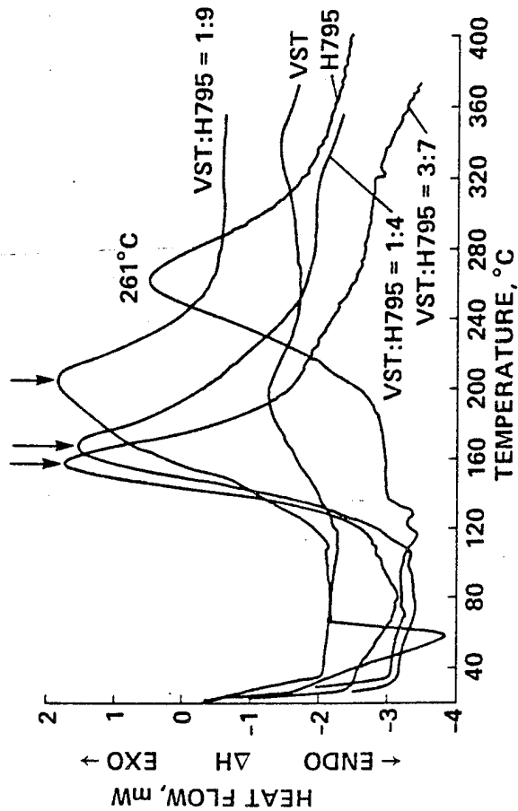
Fig. 13 DSC OF BISMALEIMIDE (H795), VST AND VST/H795 BLENDS
