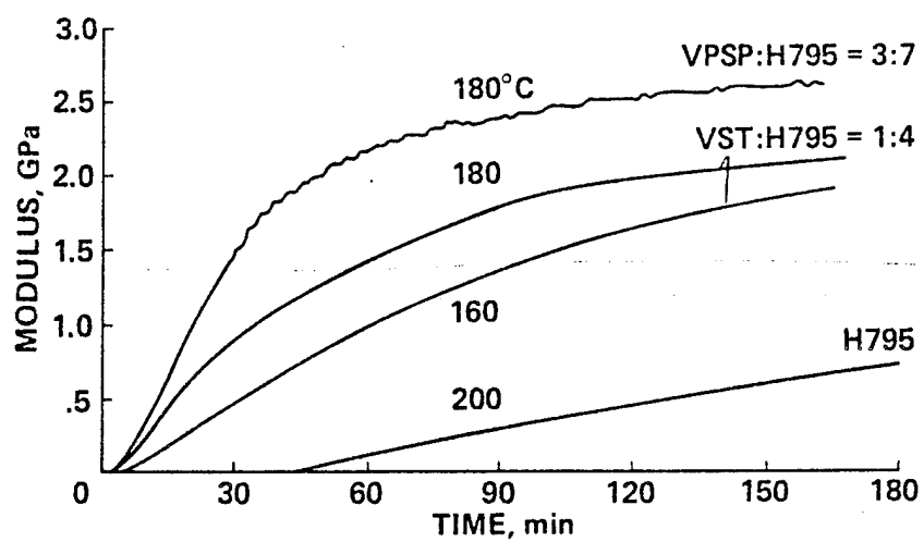
Fig. 19 ISOTHERMAL DMA OF MODIFIED AND UNMODIFIED BISMALEIMIDE PREPREG
