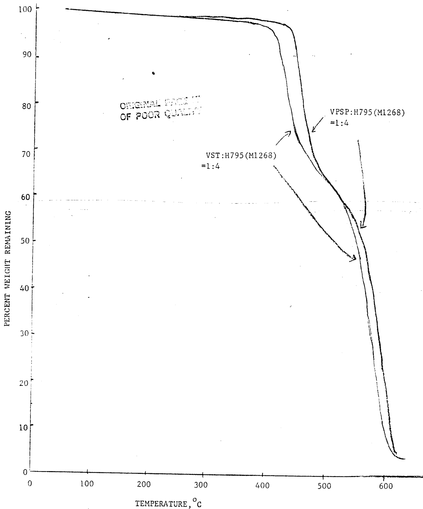
FIG. 18 TYPICAL THERMOGRAVIMETRIC ANALYSIS OF VINYLSTYRYLPYRIDINE MODIFIED BISMALIMIDE IN AIR ( 10^{\circ}\text{C}/\text{min} )
