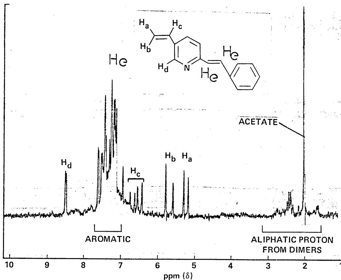
FIG. 4 NMR OF 5 VINYL-2-STIL BAZOLE (VST)
