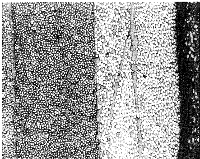
B. VIEW OF SECTION NORMAL TO ZERO-DEGREE FIBERS
