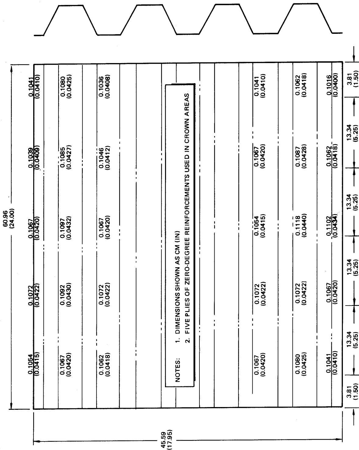
Figure 29. Thicknesses Measured on the Second 0.61m Test Panel
