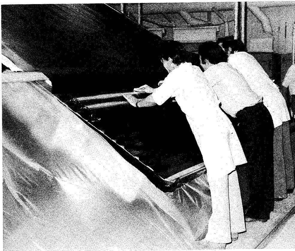
Figure 40. Contouring the Bottom \pm 45 -Deg Preplid Sheet to the Mold
