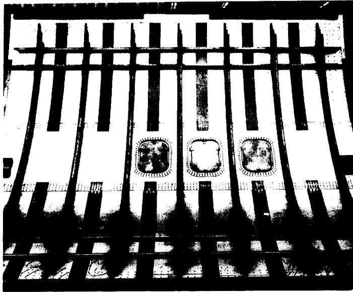
Figure 11. - Typical window installation.
