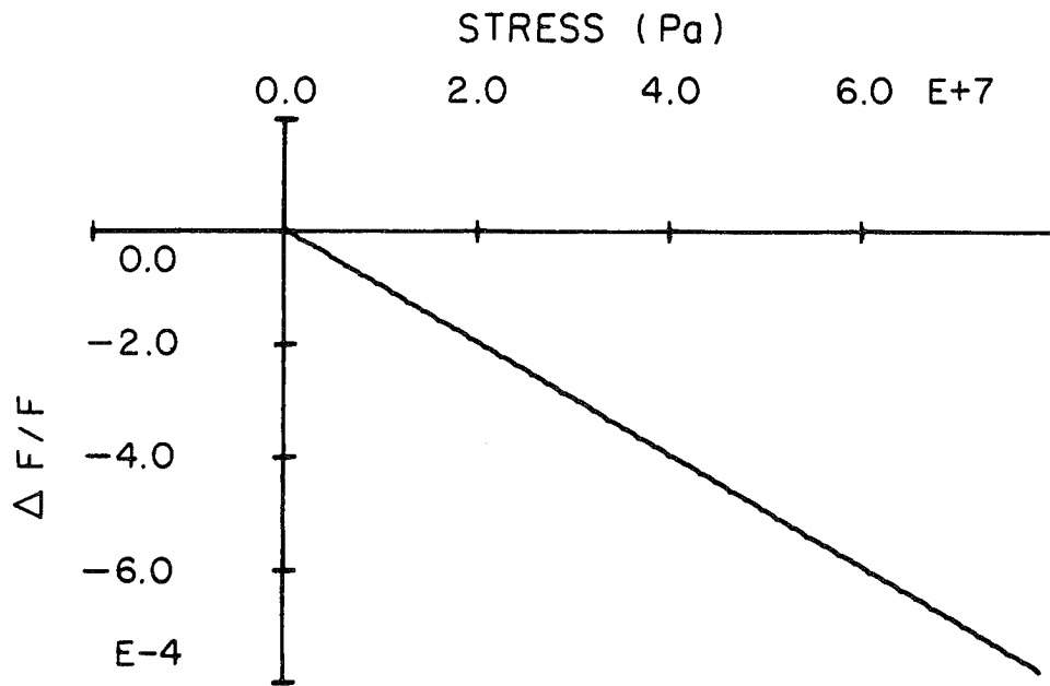
Figure 3.15 - Delta F/F versus stress for a shear wave propagating along x_2 polarized along x_3 with stress applied along x_3 .
