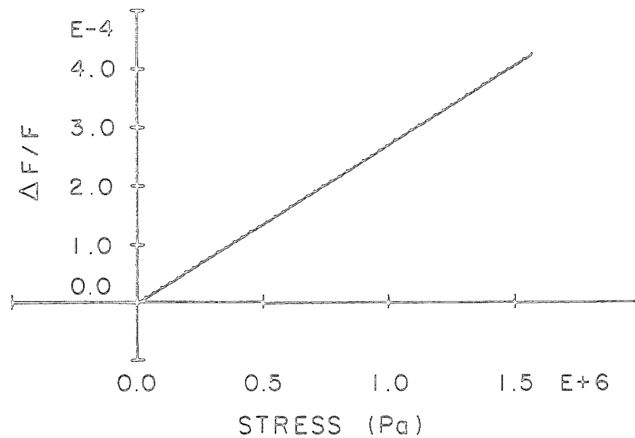
Figure 3.27 - Delta F/F versus pressure for a shear wave propagating along x_2 polarized along x_3 .
