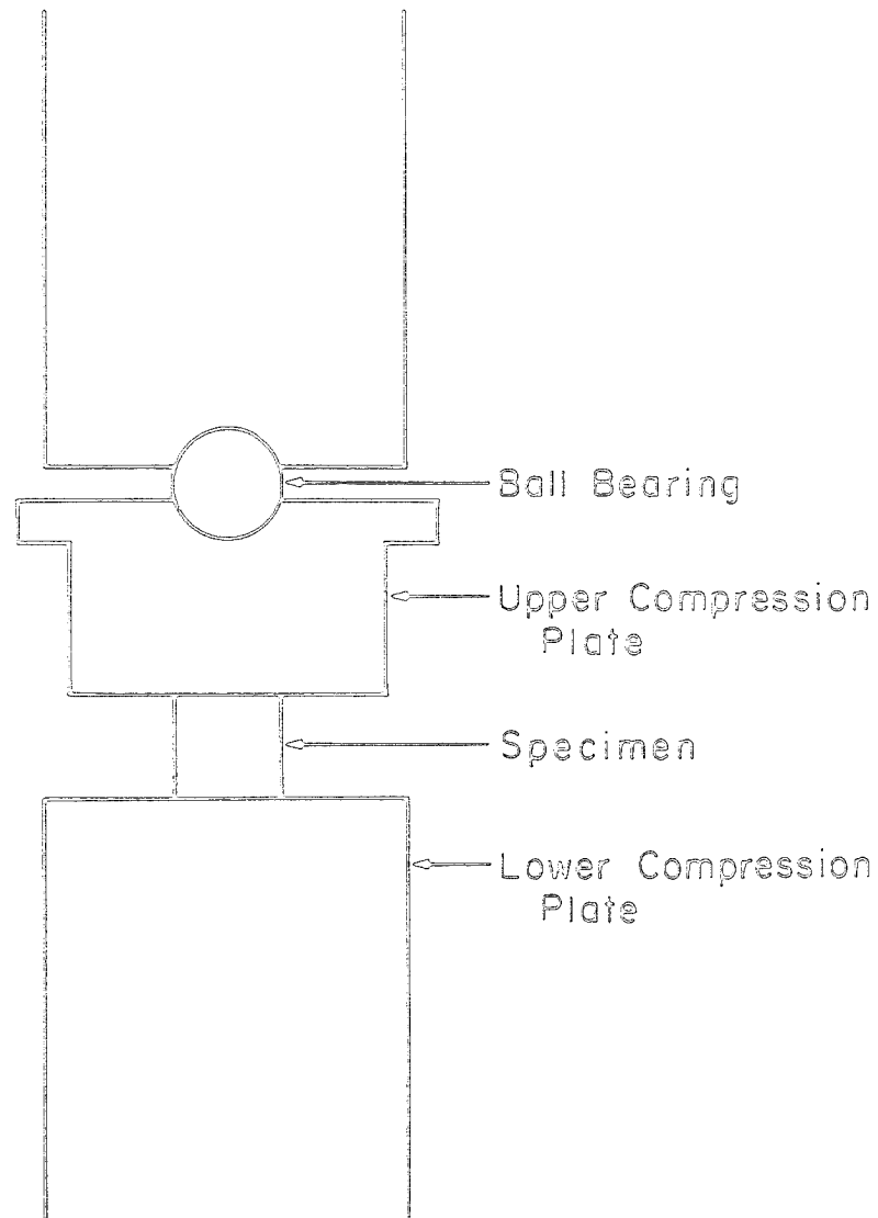
Figure 2.15 - Diagram of the compression fixture used during the static loading for the measurement of the elastic compliance moduli and the uniaxial stress acoustic constants.
