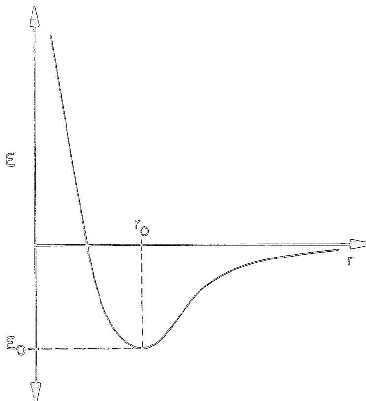
Figure 1.4 - Potential Energy ( E ) - Separation distance ( r ) curve for interatomic bonding.
