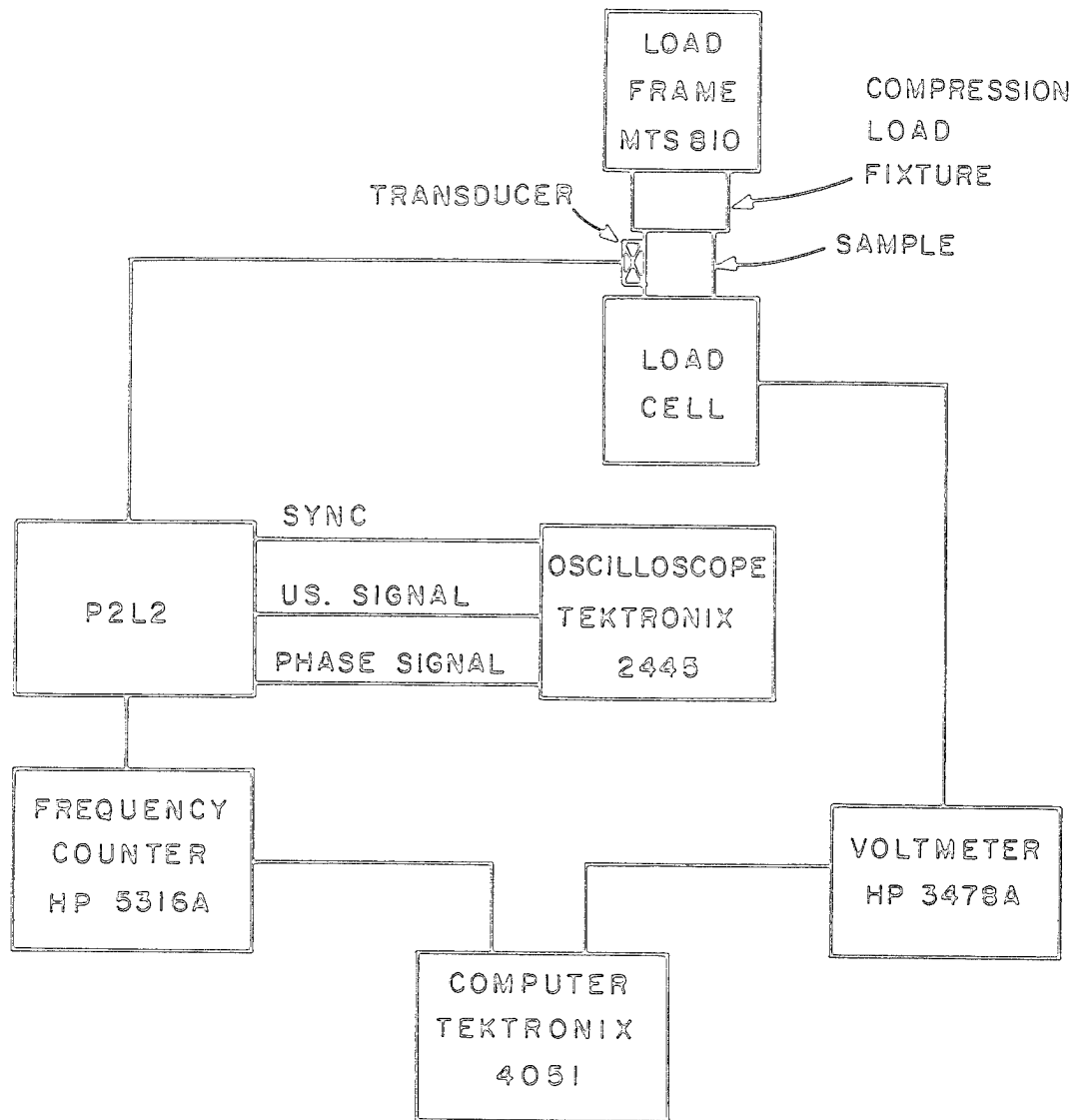
Figure 3.2 - Block diagram of uniaxial stress acoustic constant measurement apparatus.
