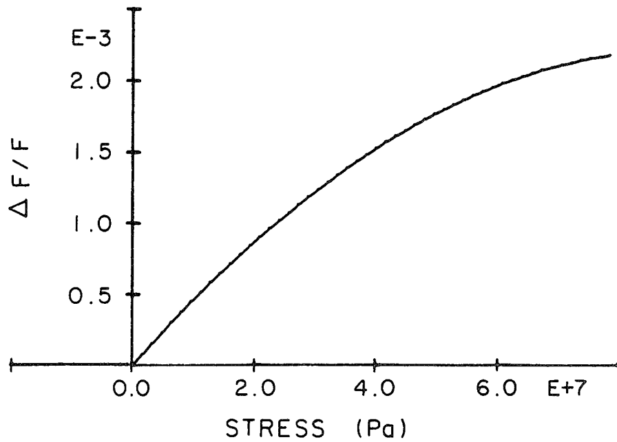
Figure 3.7 - Delta F/F versus stress for a longitudinal wave propagating along x_2 with stress applied along x_1 .
