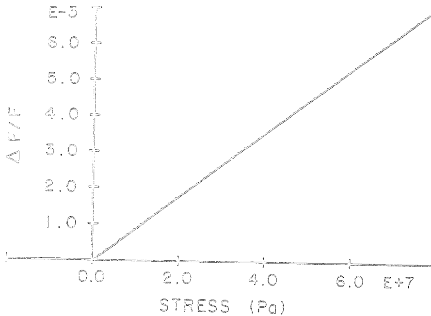
Figure 3.9 - Delta F/F versus stress for a shear wave propagating along x_2 polarized along x_1 with stress applied along x_1 .
