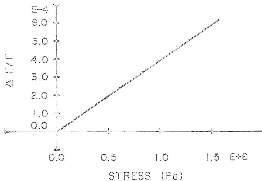
Figure 3.22 - Delta F/F versus pressure for a longitudinal wave propagating along x_1 .
