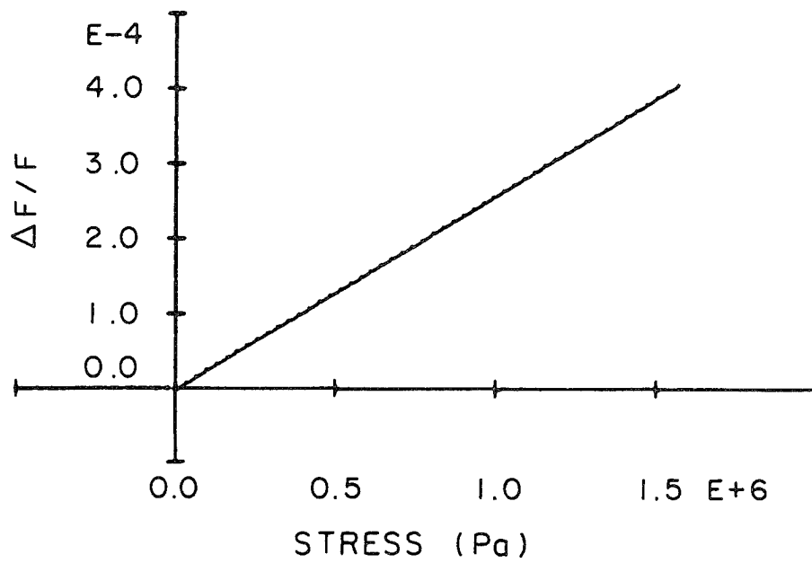
Figure 3.24 - Delta F/F versus pressure for a shear wave propagating along x_1 polarized along x_2 .
