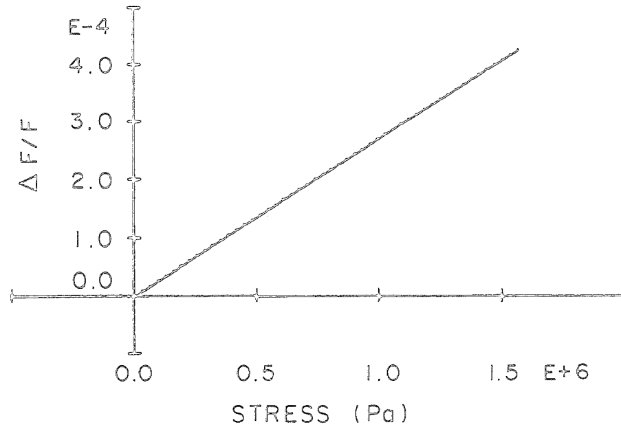
Figure 3.26 - Delta F/F versus pressure for a shear wave propagating along x_1 polarized along x_3 .
