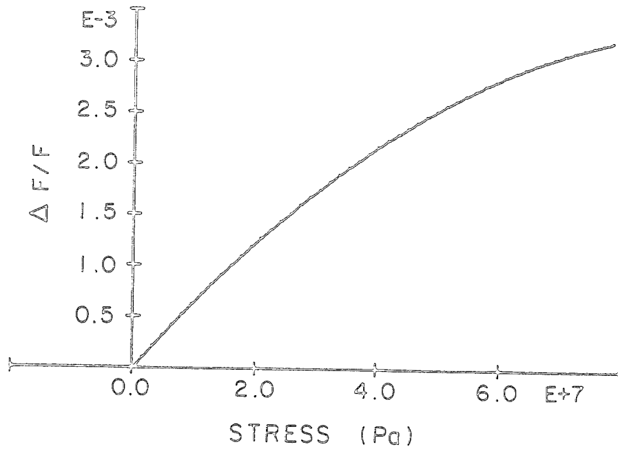
Figure 3.13 - Delta F/F versus stress for a shear wave propagating along x_2 polarized along x_3 with stress applied along x_1 .
