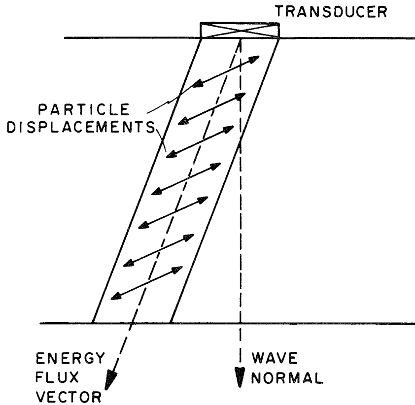
Figure 2.6 - Diagram of a quasitransverse elastic wave undergoing energy flux deviation illustrating the directions of particle displacements, wave normal, and energy flux vector.
