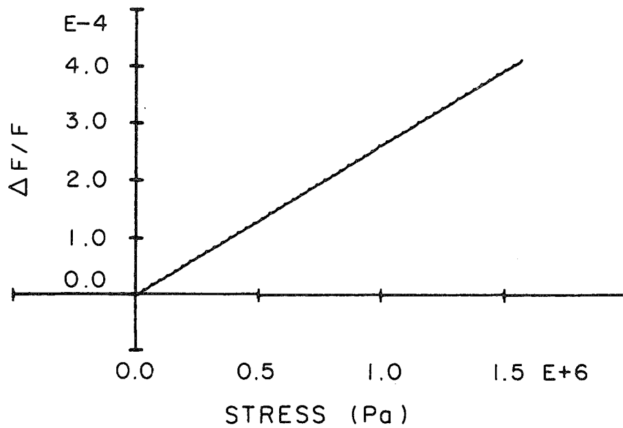
Figure 3.25 - Delta F/F versus pressure for a shear wave propagating along x_2 polarized along x_1 .
