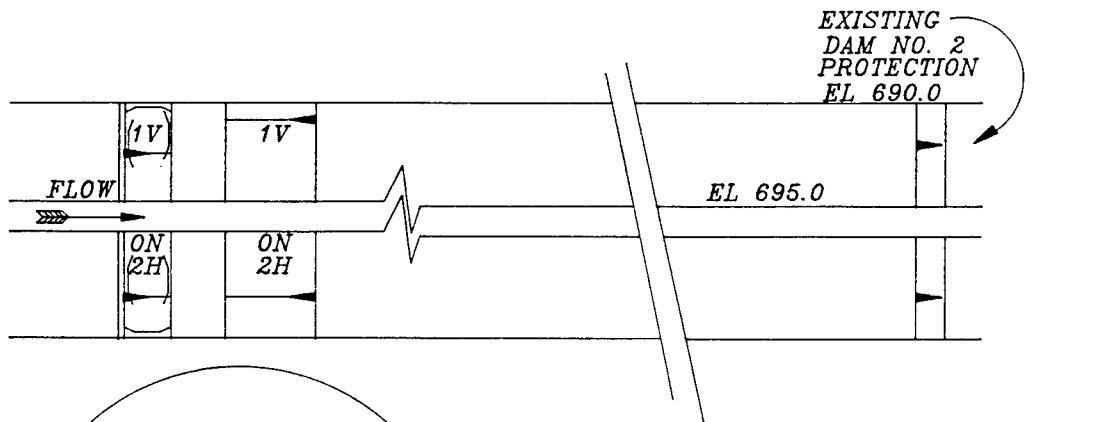
PLAN VIEW
