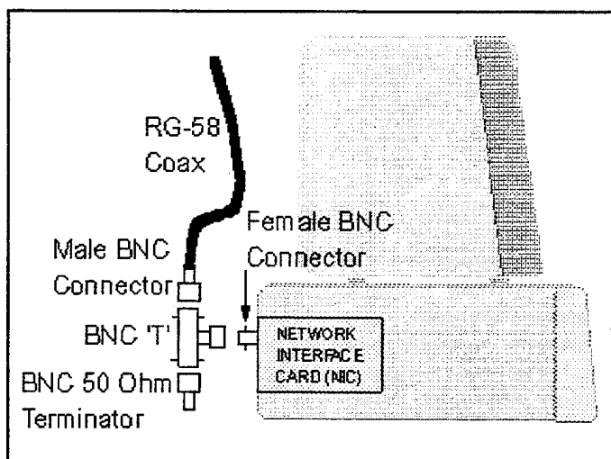
Figure 5.4 BNC "T" connection to node.
