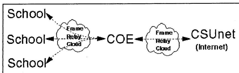
Figure 6.7 County Office of Education (COE)-centric WAN design with a potential single point of failure at the COE.
