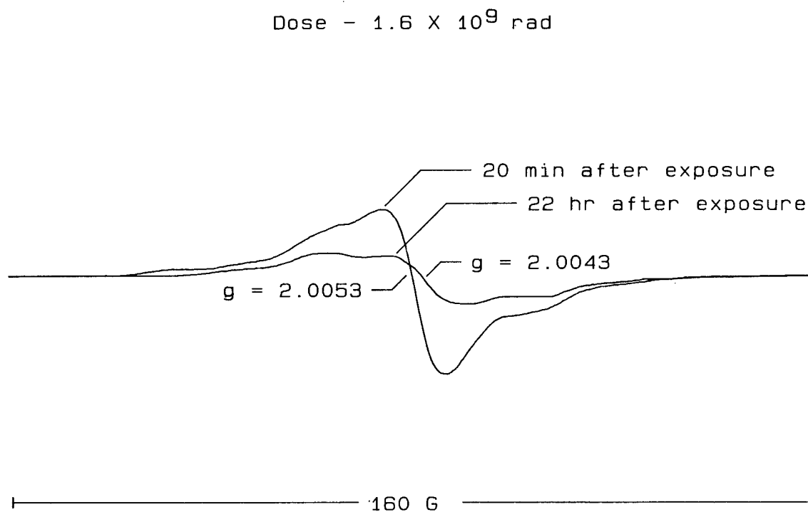
Figure 18.- Relative decay in vacuum at 22°C of radicals in irradiated Ultem, 1.6 \times 10^9 rad dose.
