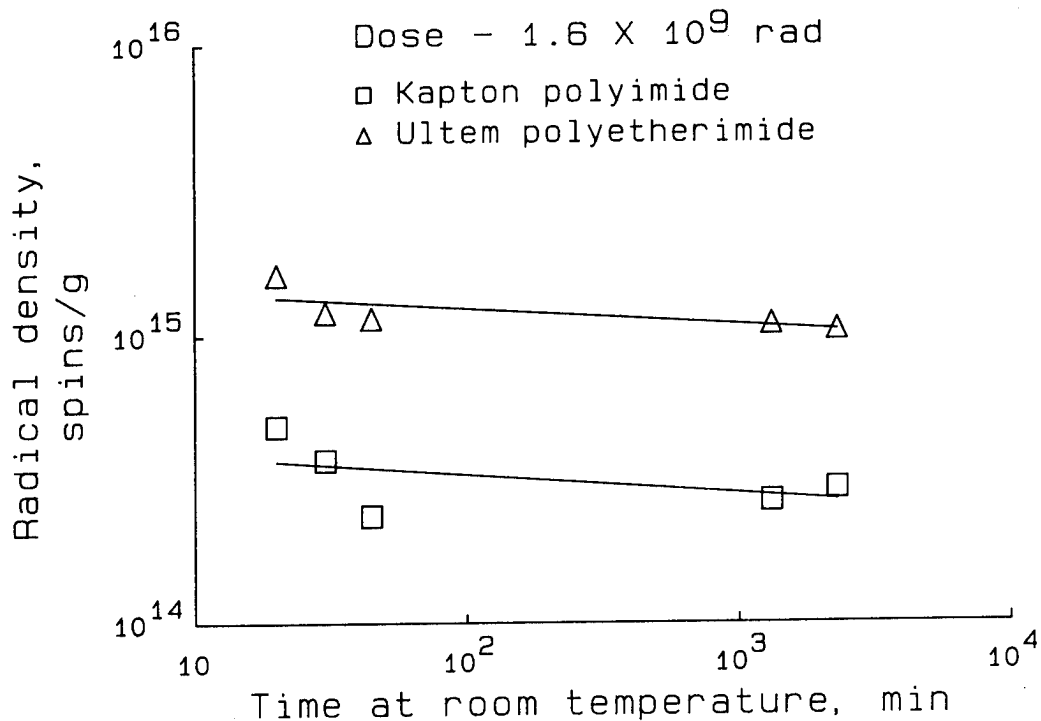
Figure 17.- Radical decay at 22°C in vacuum for irradiated Ultem and irradiated Kapton.
