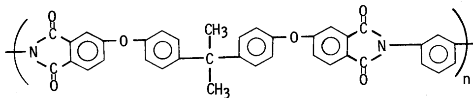
Figure 2.- Molecular structure of nonirradiated Ultem.
