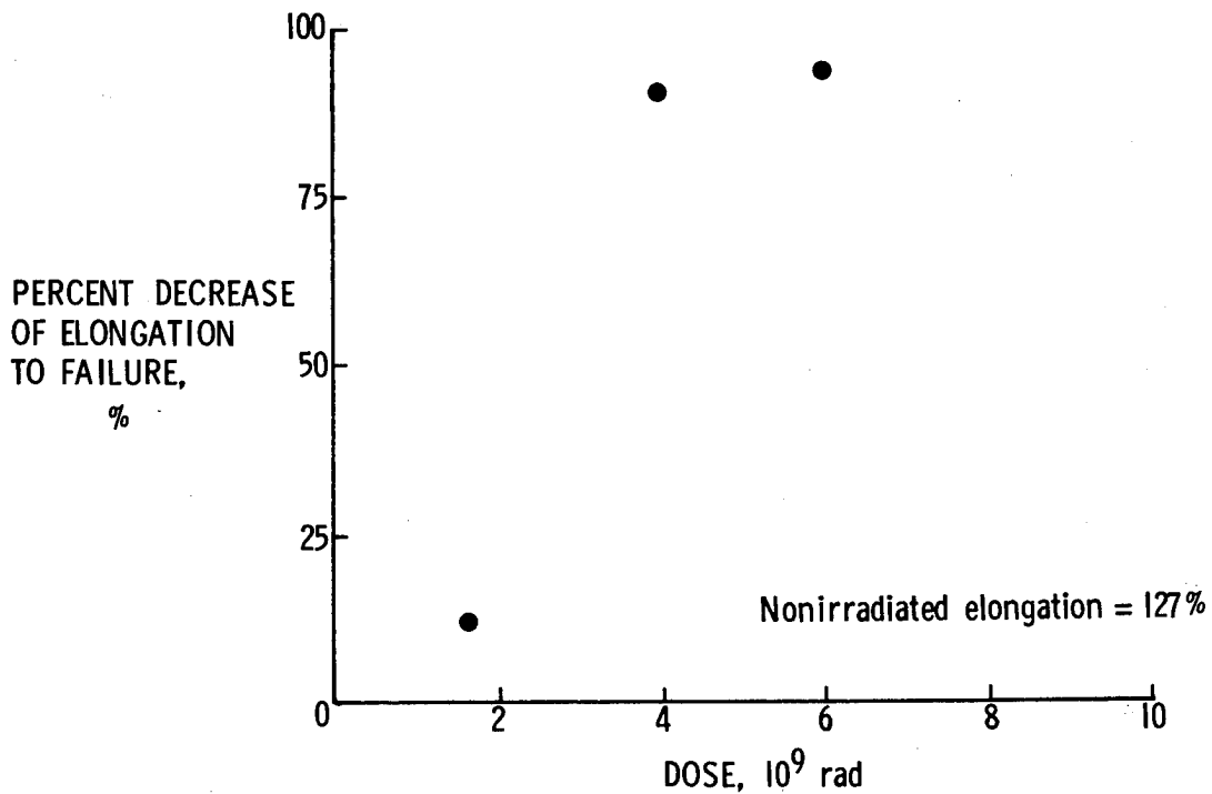
Figure 28.- Change in elongation to failure of Ultem with radiation.
