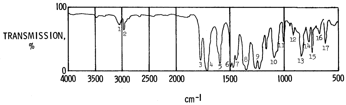
Figure 23.- Infrared spectrum for nonirradiated Ultem.
