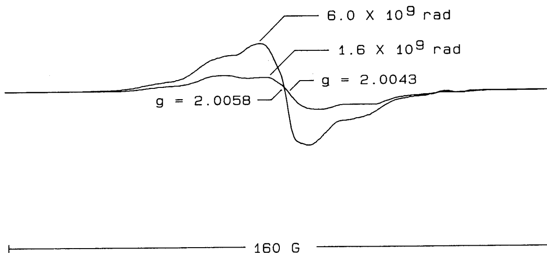
Figure 21.- Comparison for two radiation doses of the radical distribution in Ultem after one day of decay in vacuum at 22°C.
