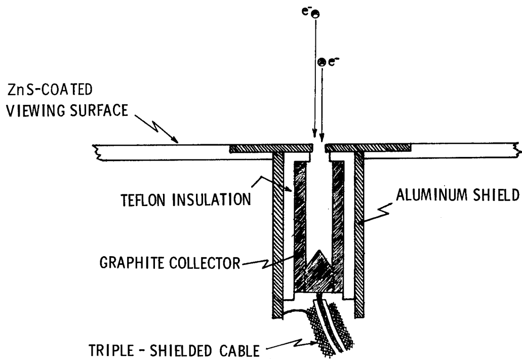
Figure 1.- Cross-sectional drawing of Faraday cup.
