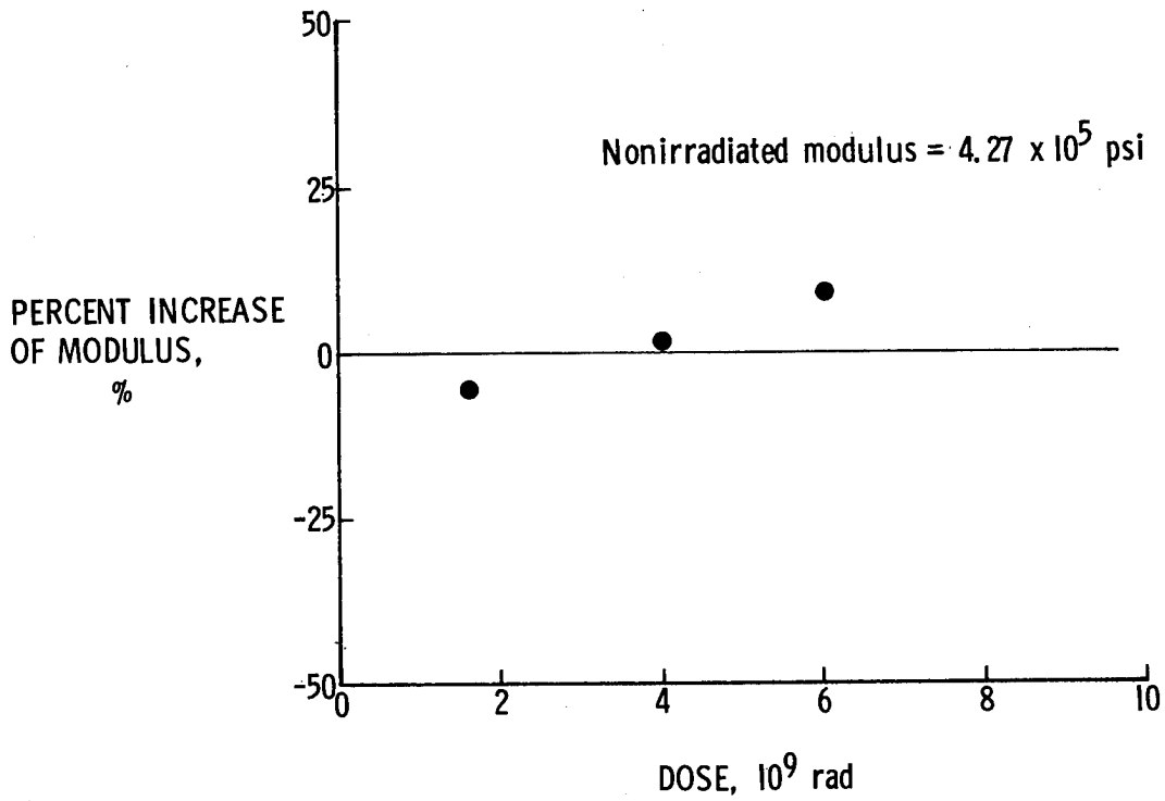
Figure 27.- Change in tensile modulus of Ultem with radiation.
