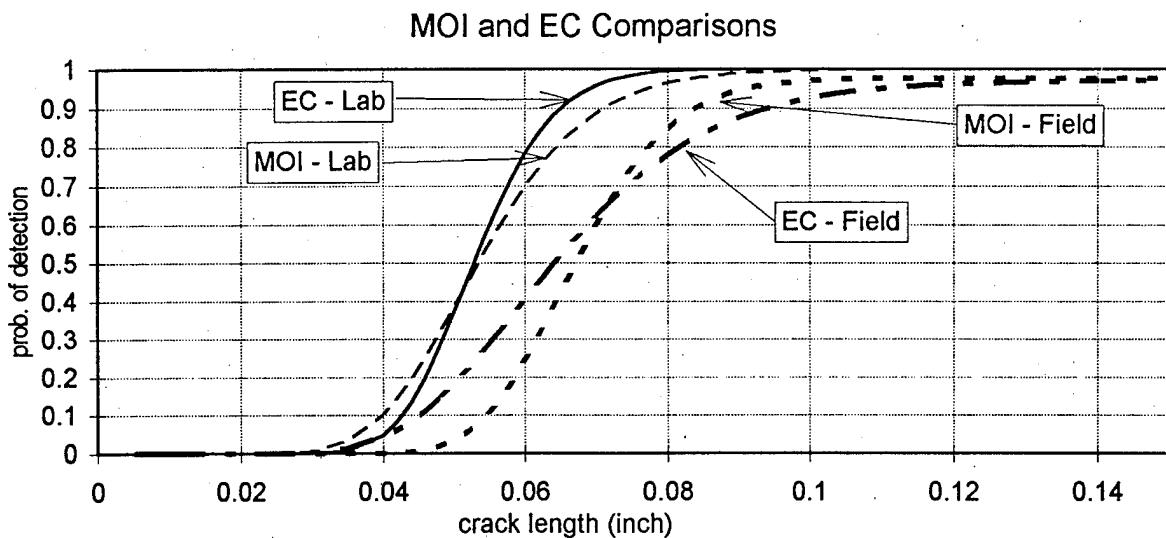
FIGURE 2.8 COMPARISON OF PROBABILITY OF DETECTION CURVES
