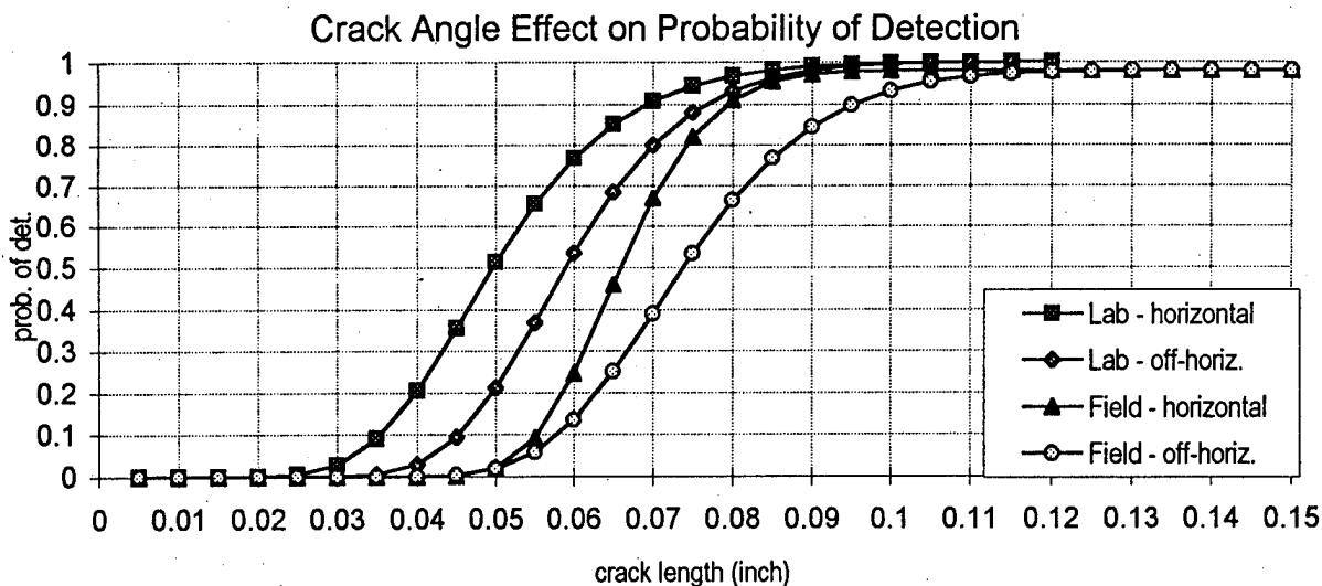
FIGURE 2.7 EFFECT OF CRACK ORIENTATION
