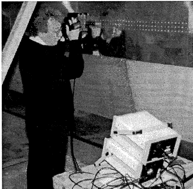
FIGURE 1.1 THE MOI BEING USED IN A SIMULATED LAP SPLICE INSPECTION
