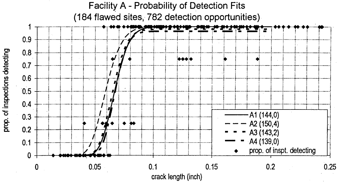
FIGURE 2.4 PoD FITS TO FACILITY A INSPECTIONS. Legend shows (total number of detects, total number of false calls).
