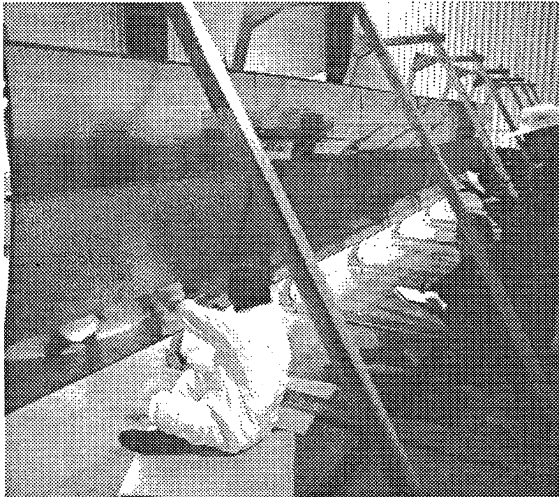
FIGURE 2.2 PRESENTATION OF LAP SPLICE SKIN SPECIMENS. (Inspector is shown inspecting bottom row with eddy-current equipment.)
