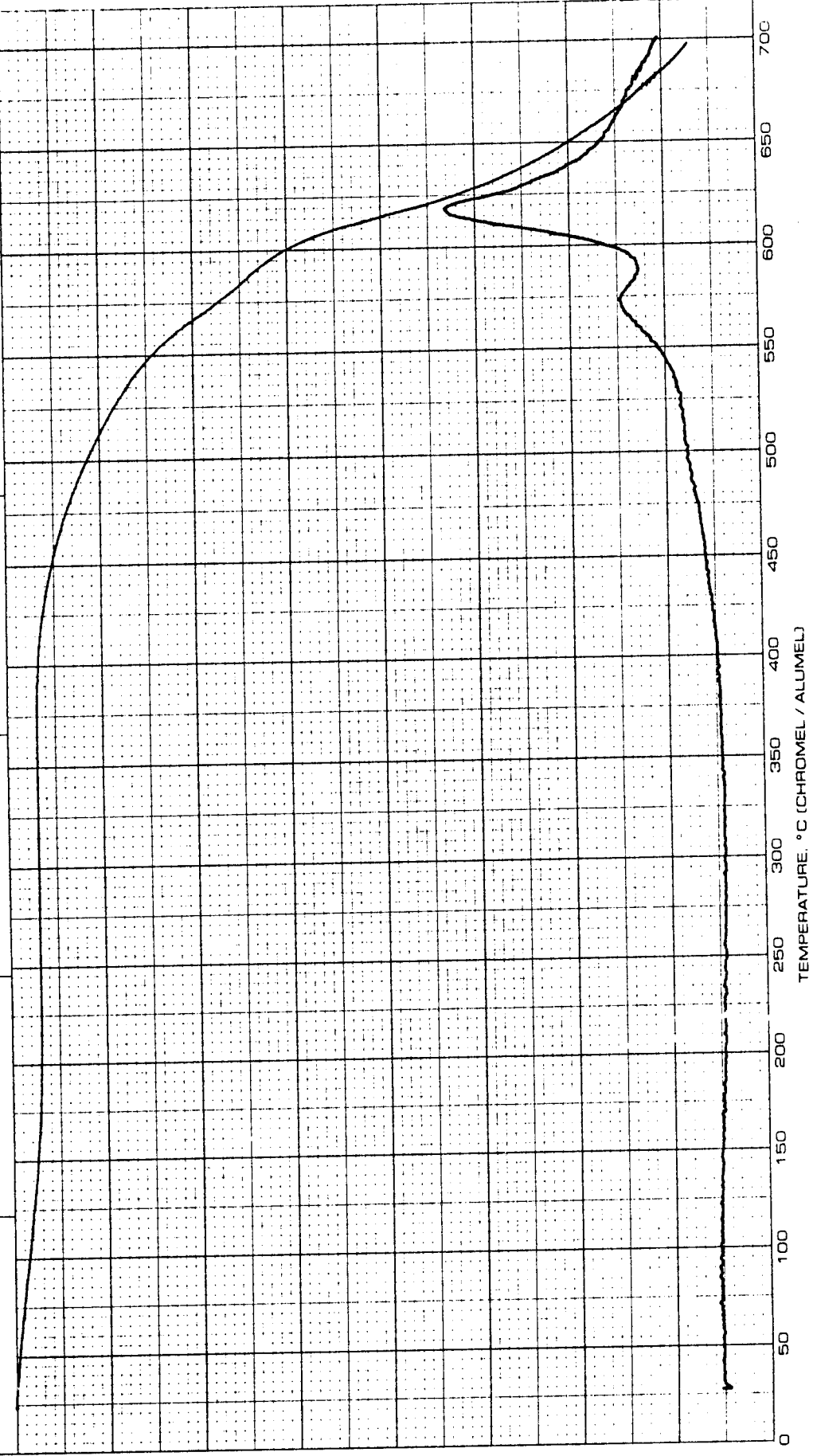
Figure 7: TGA Scan of Post Cured-Humidity Exposed BTDE/MDA/NE Resin (in Air)
