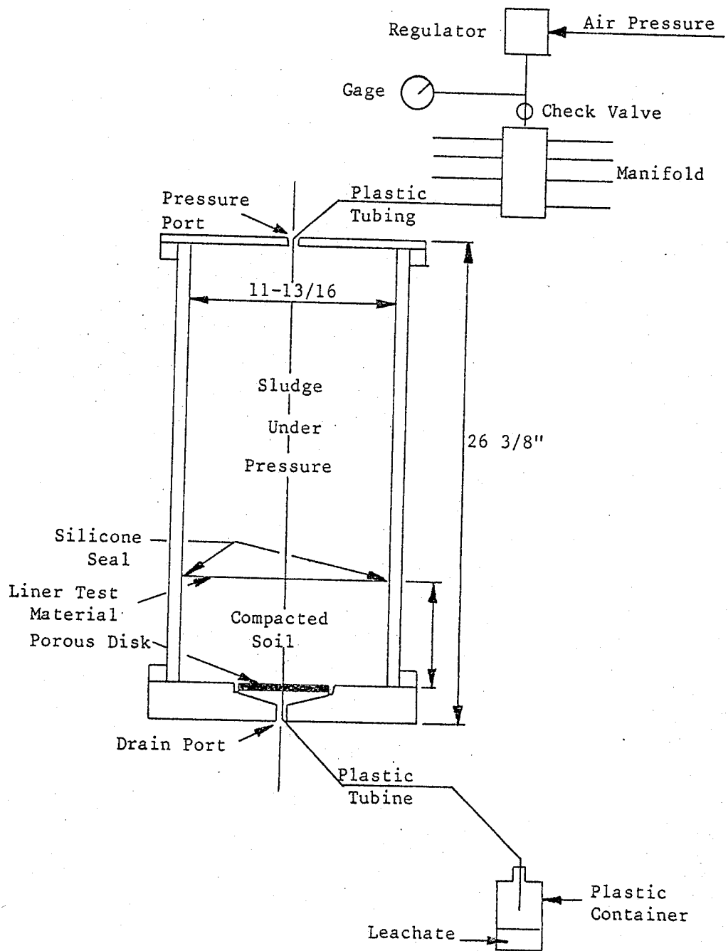
Figure 10. Schematic of a Test Cell Apparatus for Membrane Liners (Styron and Fry, 1979).
