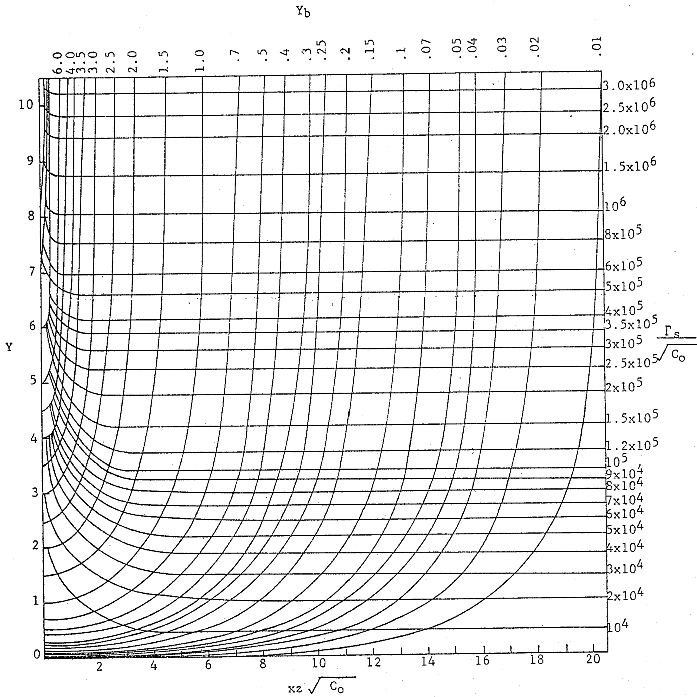
Figure 16. Scaled Potential as a Function of Solution Concentration, Distance From, and Charge Density of Mineral Surfaces (Kemper and Quirk, 1970).
