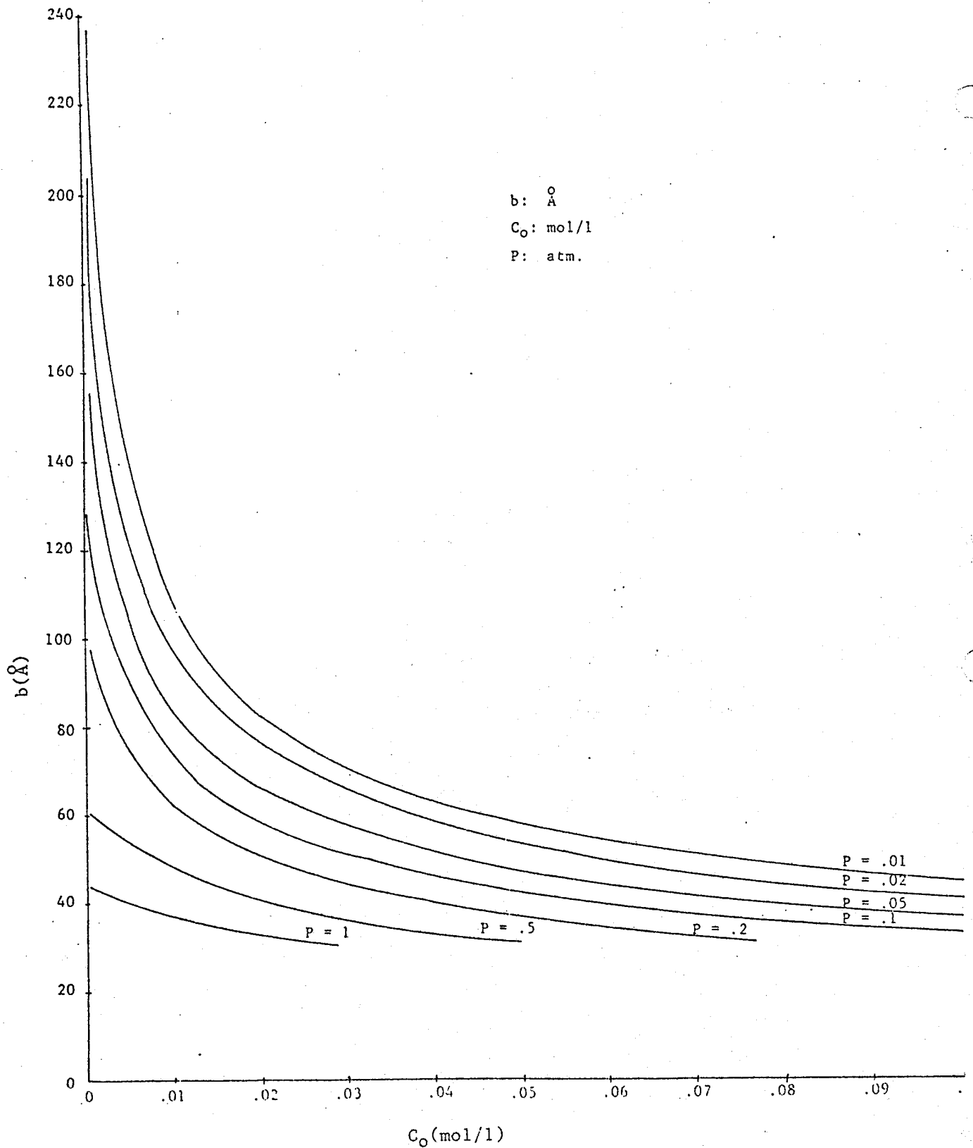
Figure 17. Interparticle Distances as a Function of NaCl Concentration at Several Applied Pressures.
