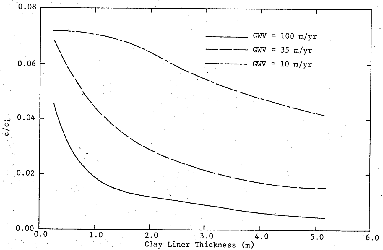
Figure 5. Effect of Clay Liner Thickness on Ionic Concentration ( c/c_i ) in an Aquifer with Various Ground Water Velocities (GWV) (Staub and Triage, 1978). Waste Pit = 1067 m x 224 m x 18 m. Distance From Pit = 10,000 m.
