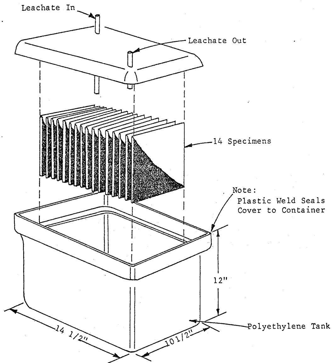
Figure 11. Individual Polyethylene Immersion Tank for Liner Compatibility Tests (Haxo, 1979). Showing method of holding membrane specimens and the inlet and outlet for the leachate.
