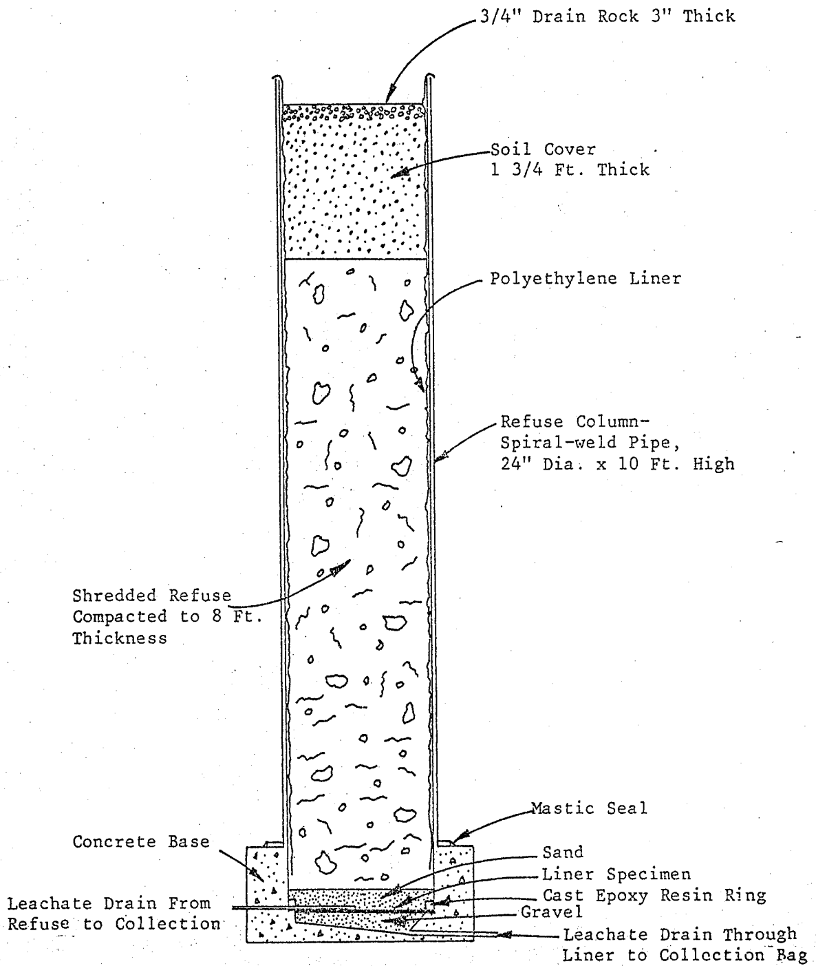
Figure 12. Schematic Drawing of Leachate Generator and Cell in Which the Liner Materials Were Exposed to Leachate Under Conditions Simulating Sanitary Landfills (Haxo, 1979).
