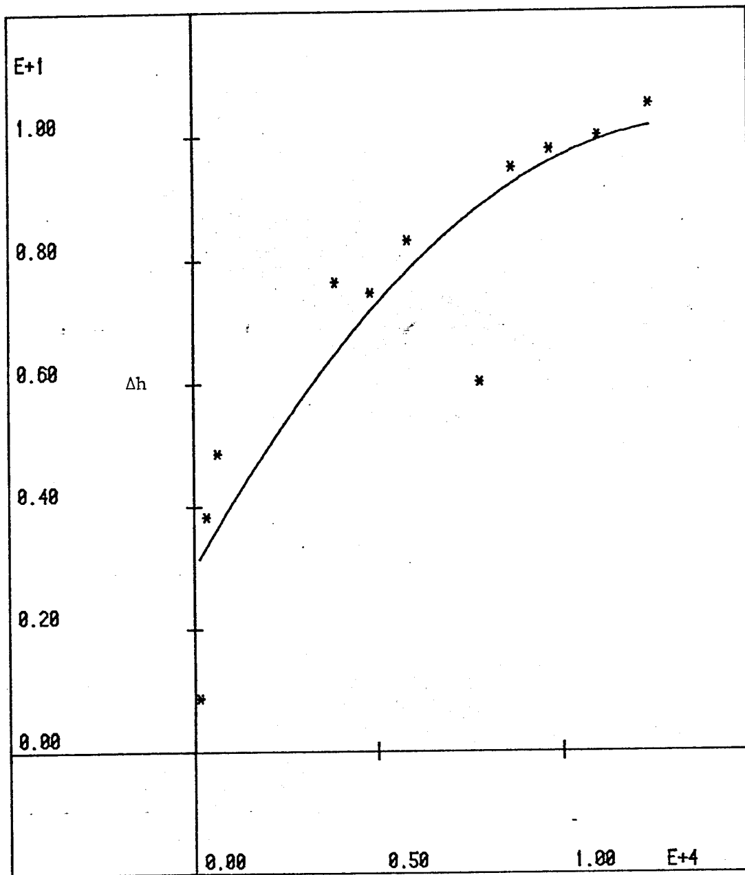
FIGURE 7 GRAPH OF HEAD CHANGE VERSUS TOTAL RECHARGE FOR BORE "B" INITIAL
