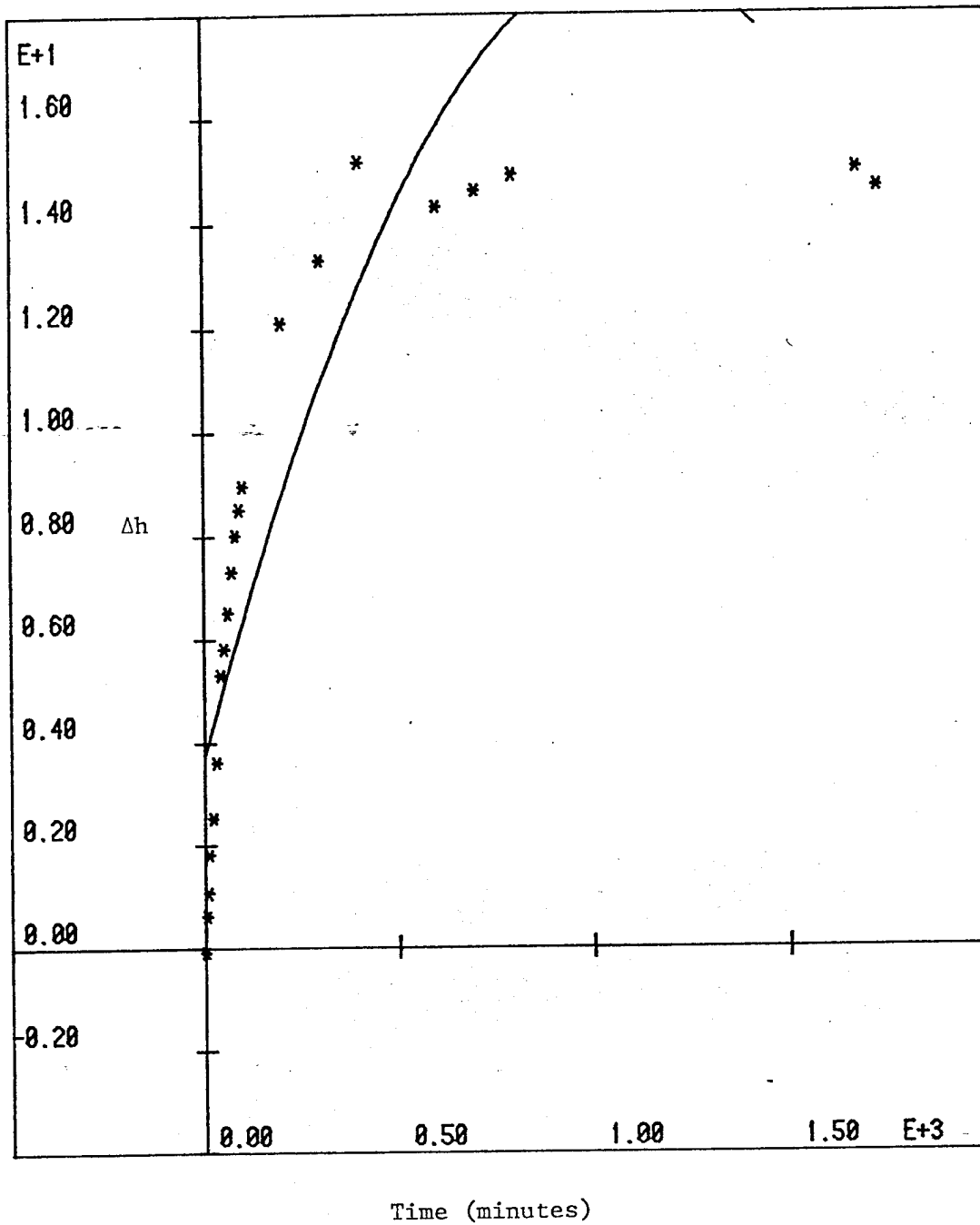
FIGURE 6 GRAPH OF HEAD CHANGE VERSUS TIME FOR BORE "C" INITIAL
