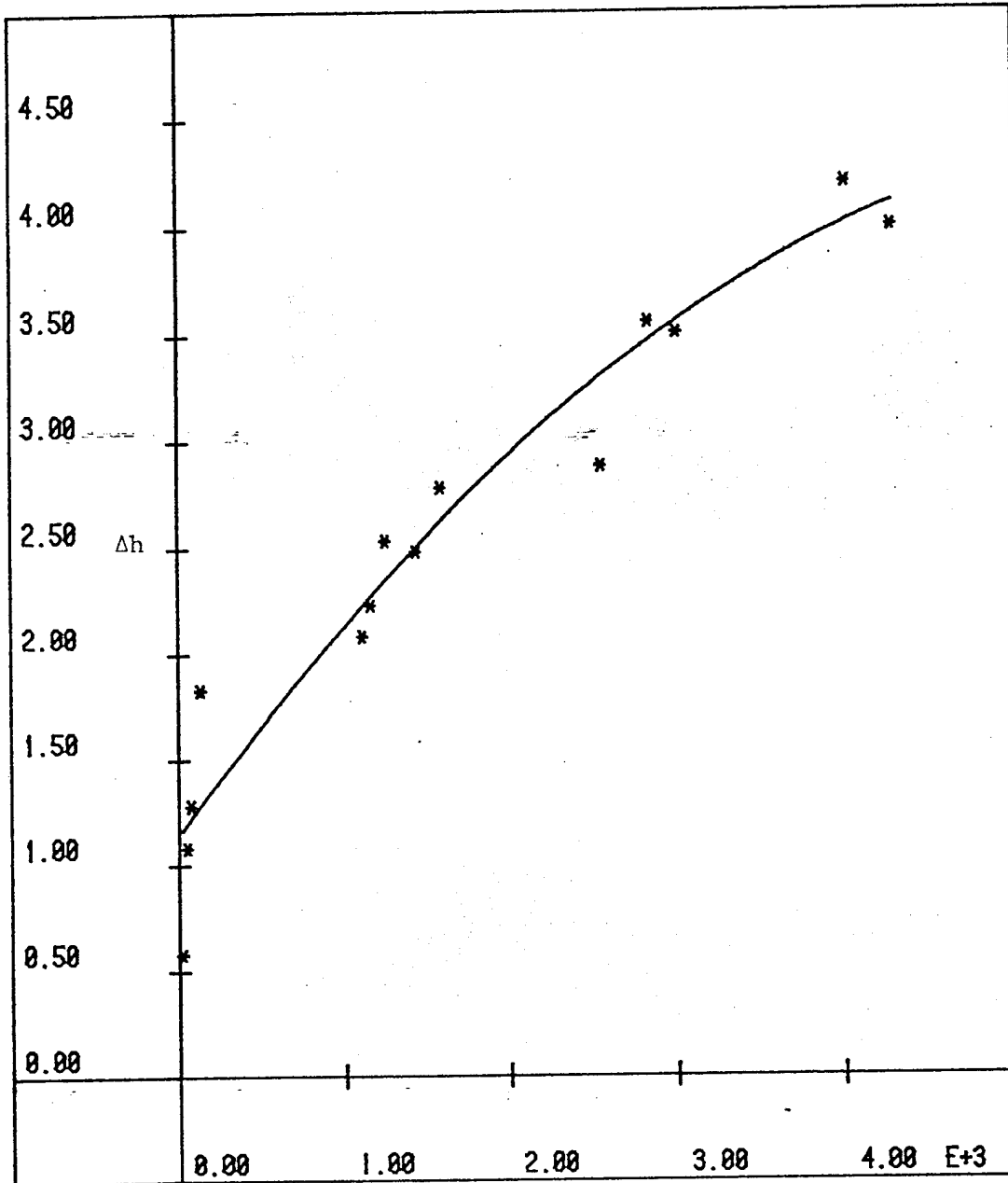
FIGURE 11 GRAPH OF HEAD CHANGE VERSUS TIME FOR CLEANED TRENCH
