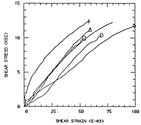
914 EPOXY 82C DRY TORSION
