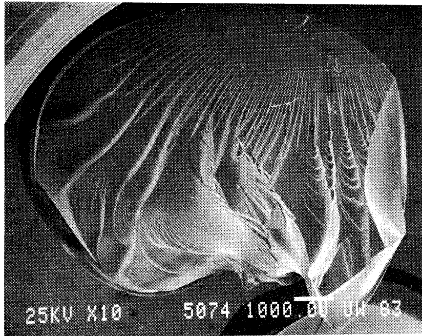
Figure D19. 3502 Neat Epoxy Torsional Shear, 54°C, Moisture-Saturated.
