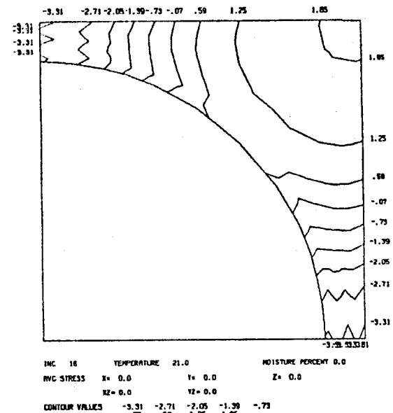
c) Maximum Principal Stress (ksi) d) Minimum Principal Stress (ksi)
