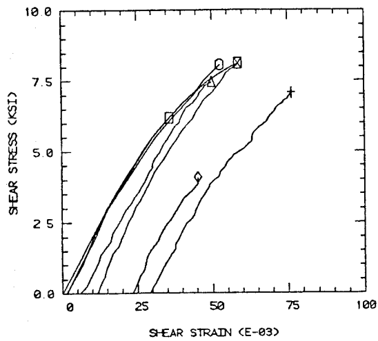
3502 EPOXY 54C WET TORSION
