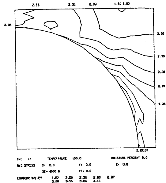
f) Intermediate Principal Stress (ksi)
