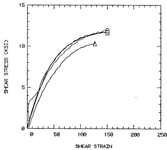
2220-1 EPOXY 82C DRY TORSION
