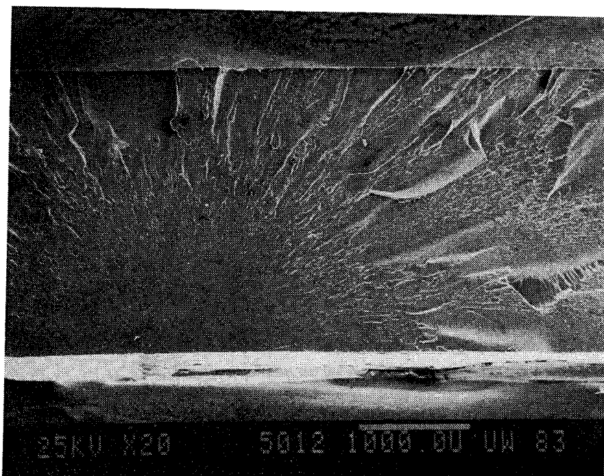
Figure D6. Fibredux 914 Neat Epoxy Tension, Specimen No. LTDB2X, 54°C, Dry.
