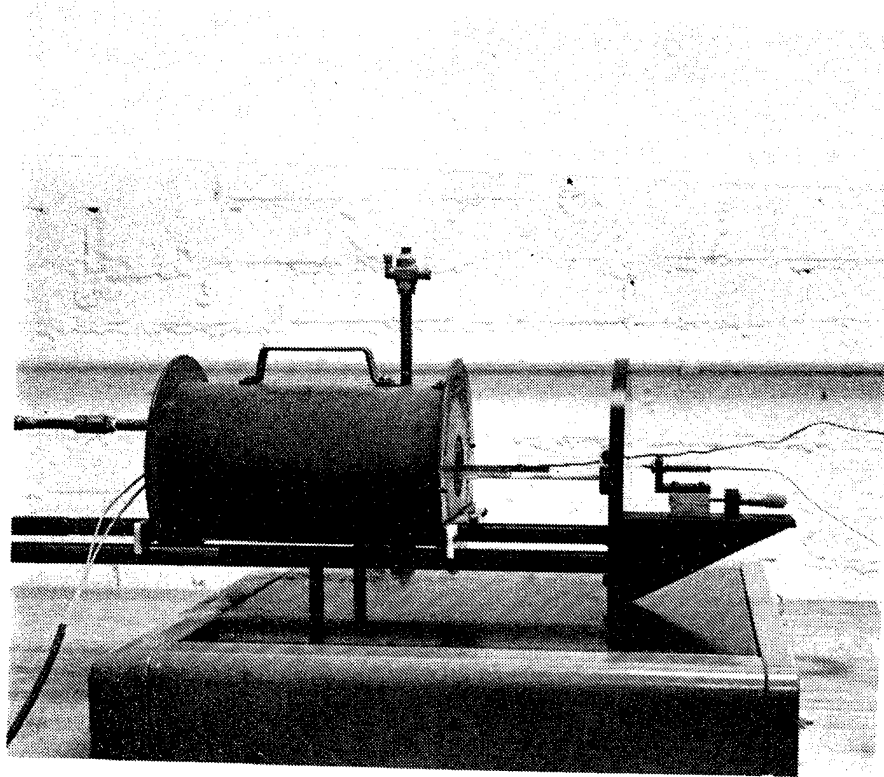
Figure B5. Coefficient of Thermal Expansion Test Apparatus.
