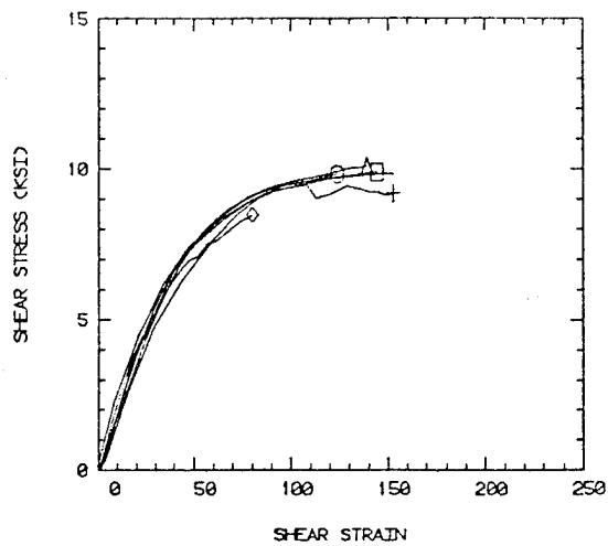
2220-1 EPOXY 54C WET TORSION
