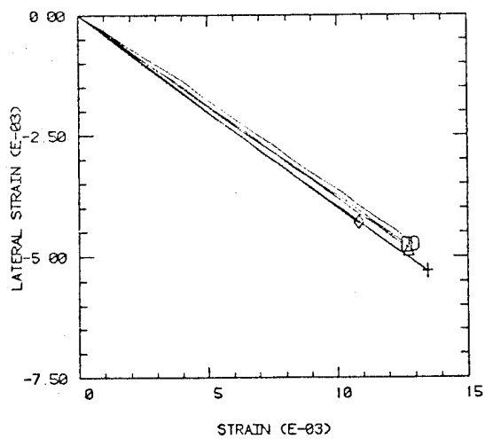
2220-1 EPOXY 23C DRY TENSION
