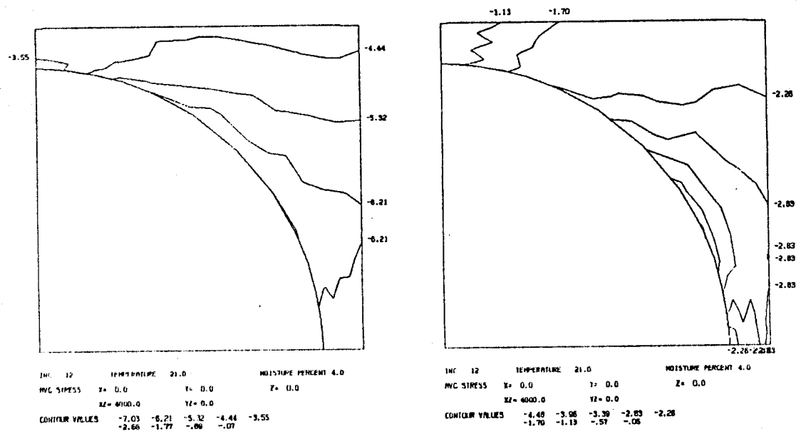
c) Minimum Principal Stress (ksi)
