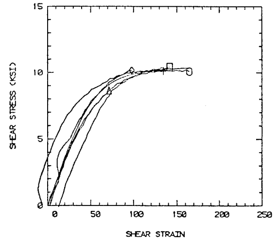
2220-3 EPOXY 82C DRY TORSION
