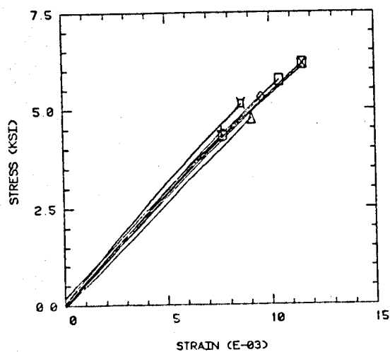
3502 EPOXY 23C DRY TENSION
