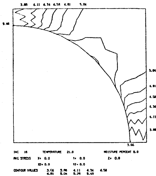
c) Maximum Principal Stress (ksi) d) Minimum Principal Stress (ksi)
