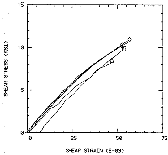
3502 EPOXY 82C DRY TORSION
