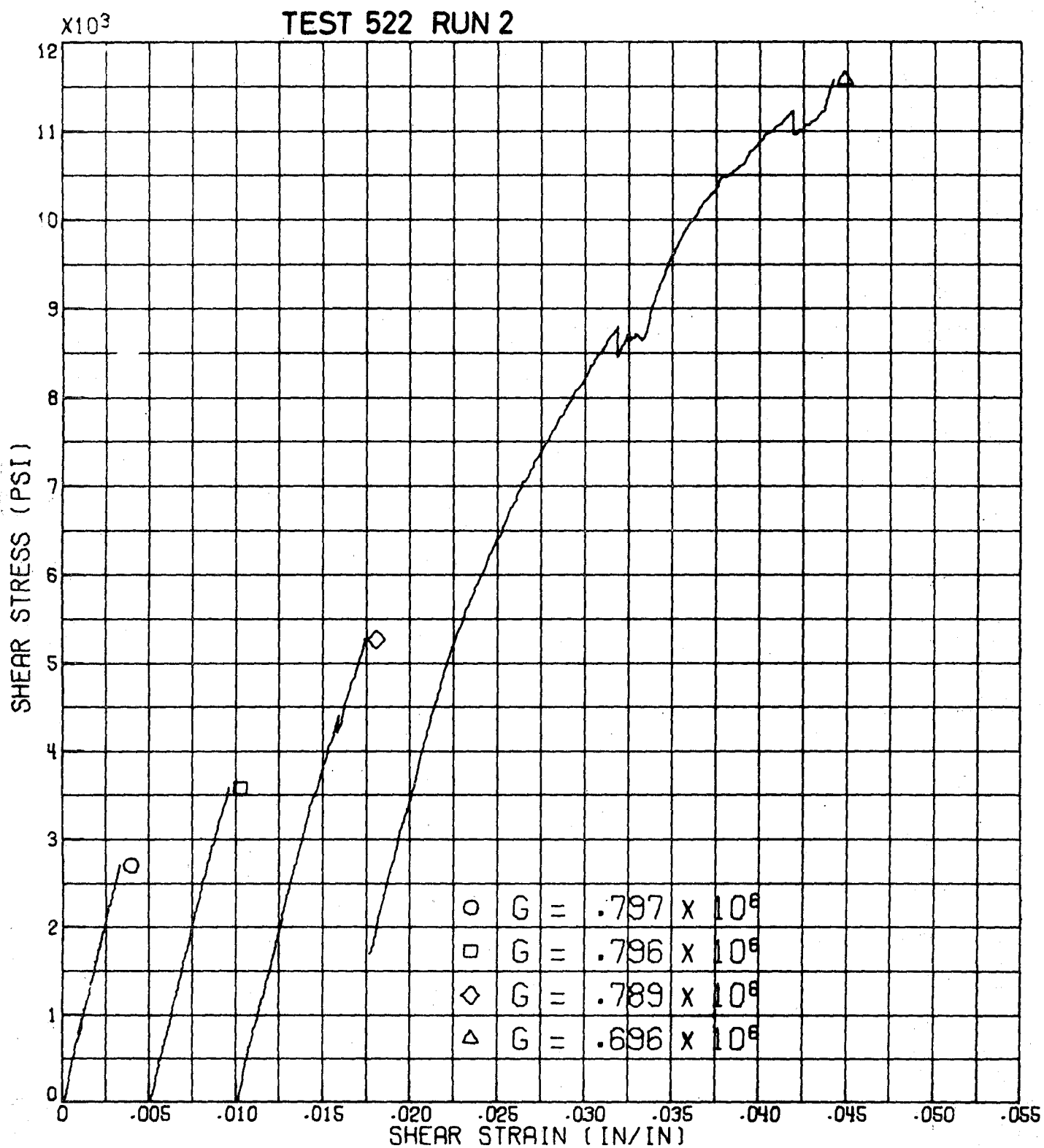
FIG. APA 41 - INFLUENCE OF LOADING AND UNLOADING ON RESPONSE OF SHEAR TUBES-CO/90J GR/EP 77
