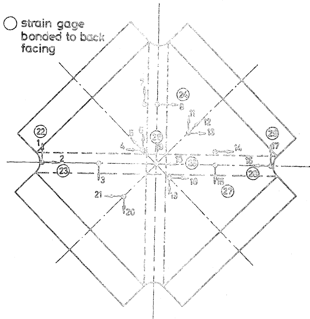
FIG. 3B SHEAR PANEL-STRAIN GAGE LOCATION (TEST 516/RUNS 1,2,4-6 & TEST 517/RUNS 1-10)
