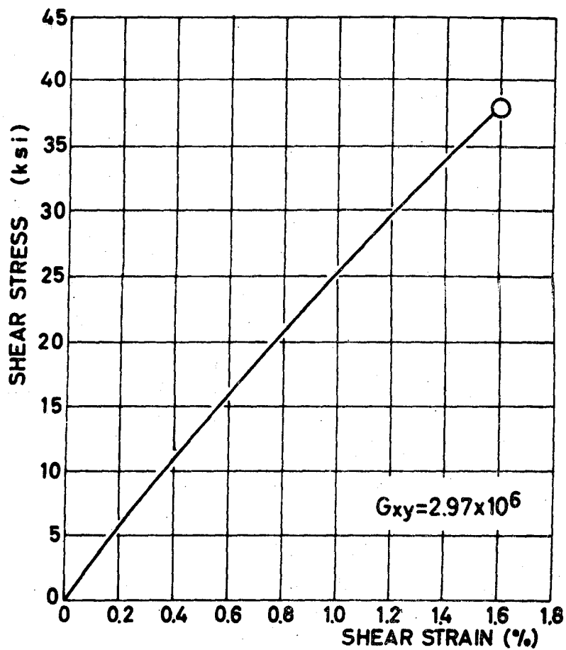
FIG. 15 A SHEAR RESPONSE OF PLANAR SPECIMENS \pm 15^\circ B/EP
