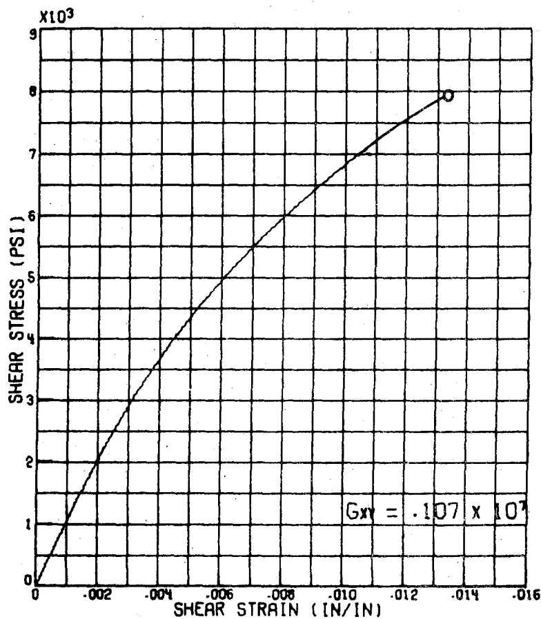
FIGURE 14B:--SHEAR RESPONSE OF TUBULAR SPECIMENS-[90°] B/EP
