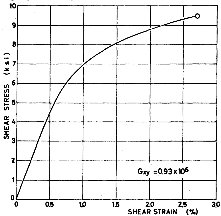
FIG. 14A SHEAR RESPONSE OF PLANAR SPECIMENS 0° B/EP
