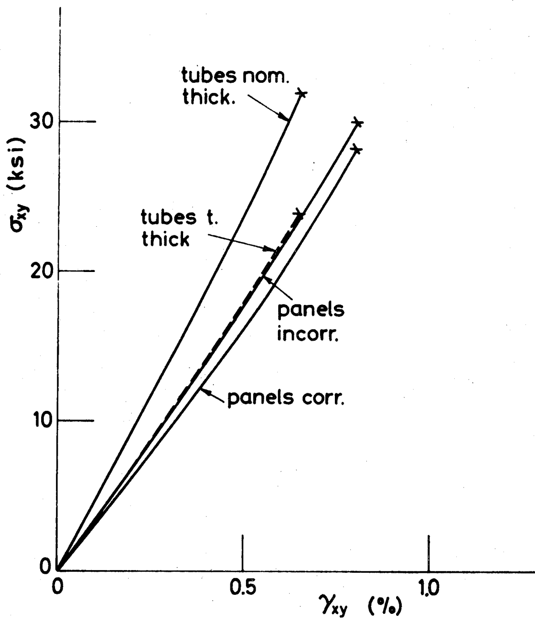
FIG. 10C SHEAR RESPONSE OF \pm 30^\circ 3M SP-286T3 GRAPHITE-EPOXY LAMINATES
