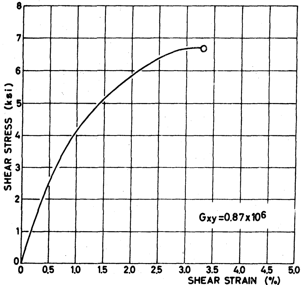
FIG. 18B SHEAR RESPONSE OF TUBULAR SPECIMENS 0/90° B/EP
