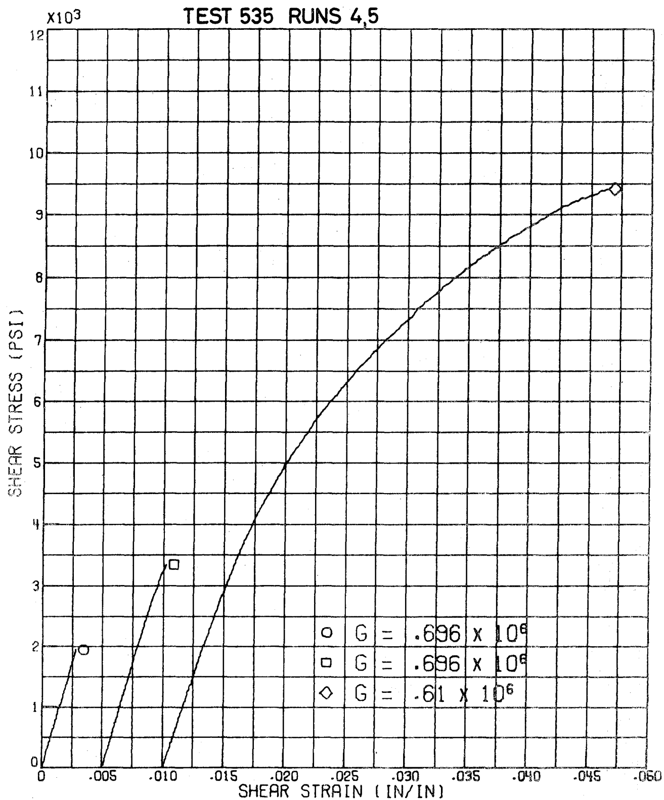
FIG. APA 4 II - INFLUENCE OF LOADING AND UNLOADING ON RESPONSE OF SHEAR TUBES-CO/90J GR/EP 78
