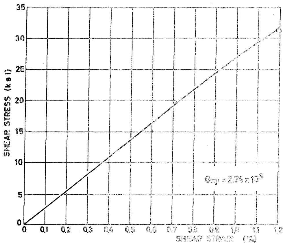
FIG. 13A SHEAR RESPONSE OF PLANAR SPECIMENS 0R45/30° GR/EP
