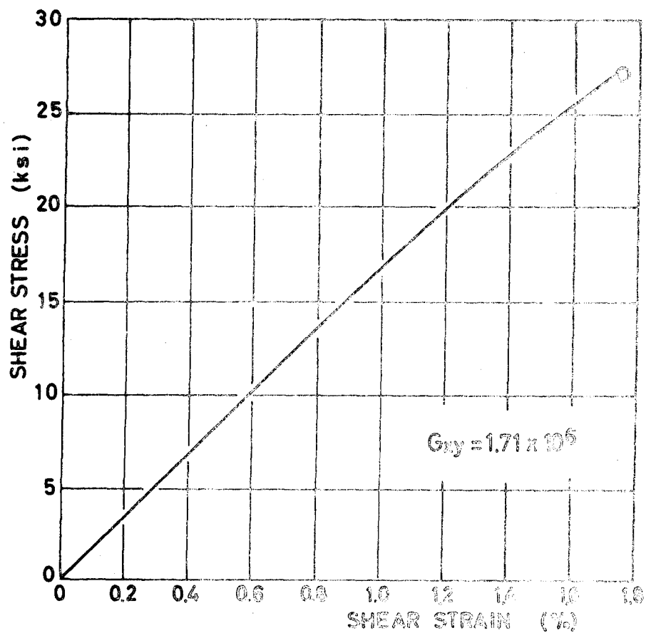
FIG. 9A SHEAR RESPONSE OF PLANAR SPECIMENS \times 10^6 GR/EP
