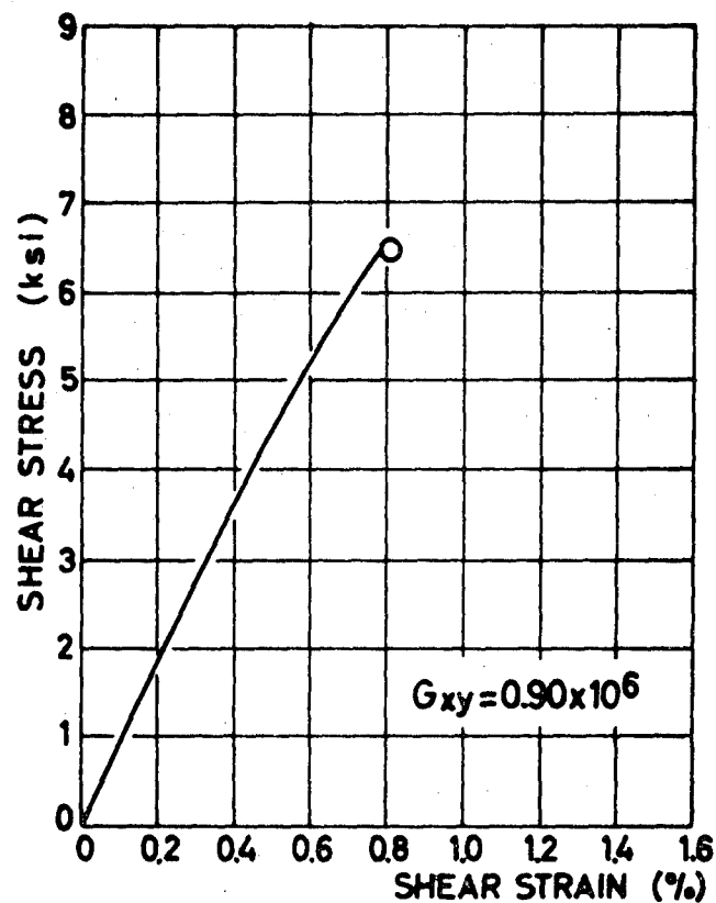
FIG. 8A SHEAR RESPONSE OF PLANAR SPECIMENS 0° GR/EP
