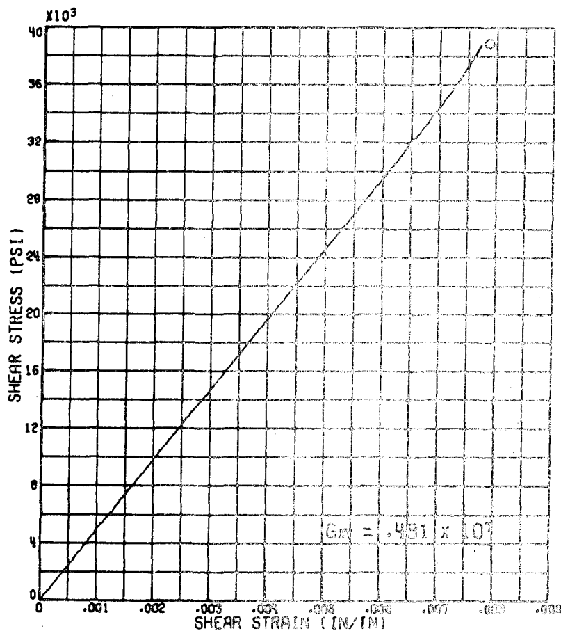
FIGURE 10B:-SHEAR RESPONSE OF TUBULAR SPECIMENS-E*309 GR/EP
