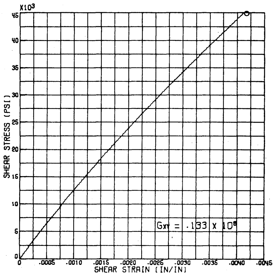
FIGURE 17B :-SHEAR RESPONSE OF TUBULAR SPECIMENS-[ \pm 45^\circ ] B/EP
