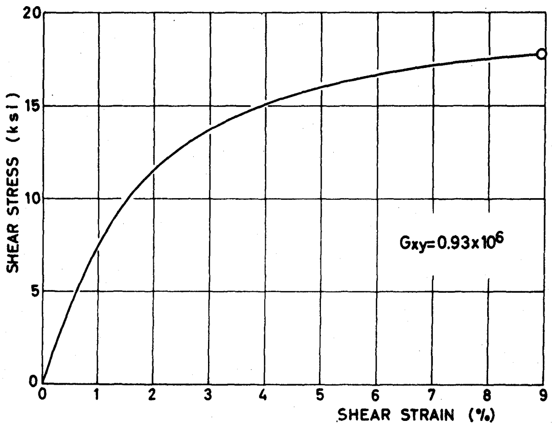
FIG. 12A SHEAR RESPONSE OF PLANAR SPECIMENS 0/90° GR/EP
