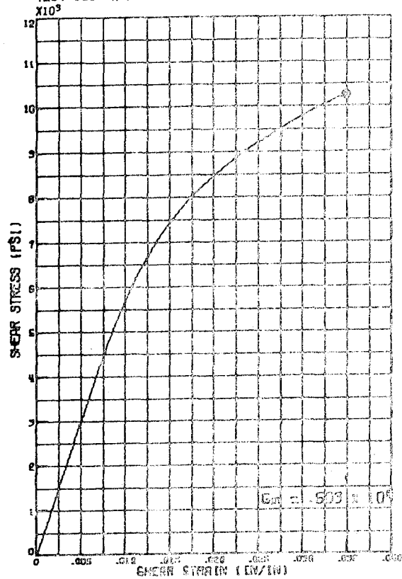
FIGURE 12B:-SHEAR RESPONSE OF TUBULAR SPECIMENS-CO/50 GR/EP
