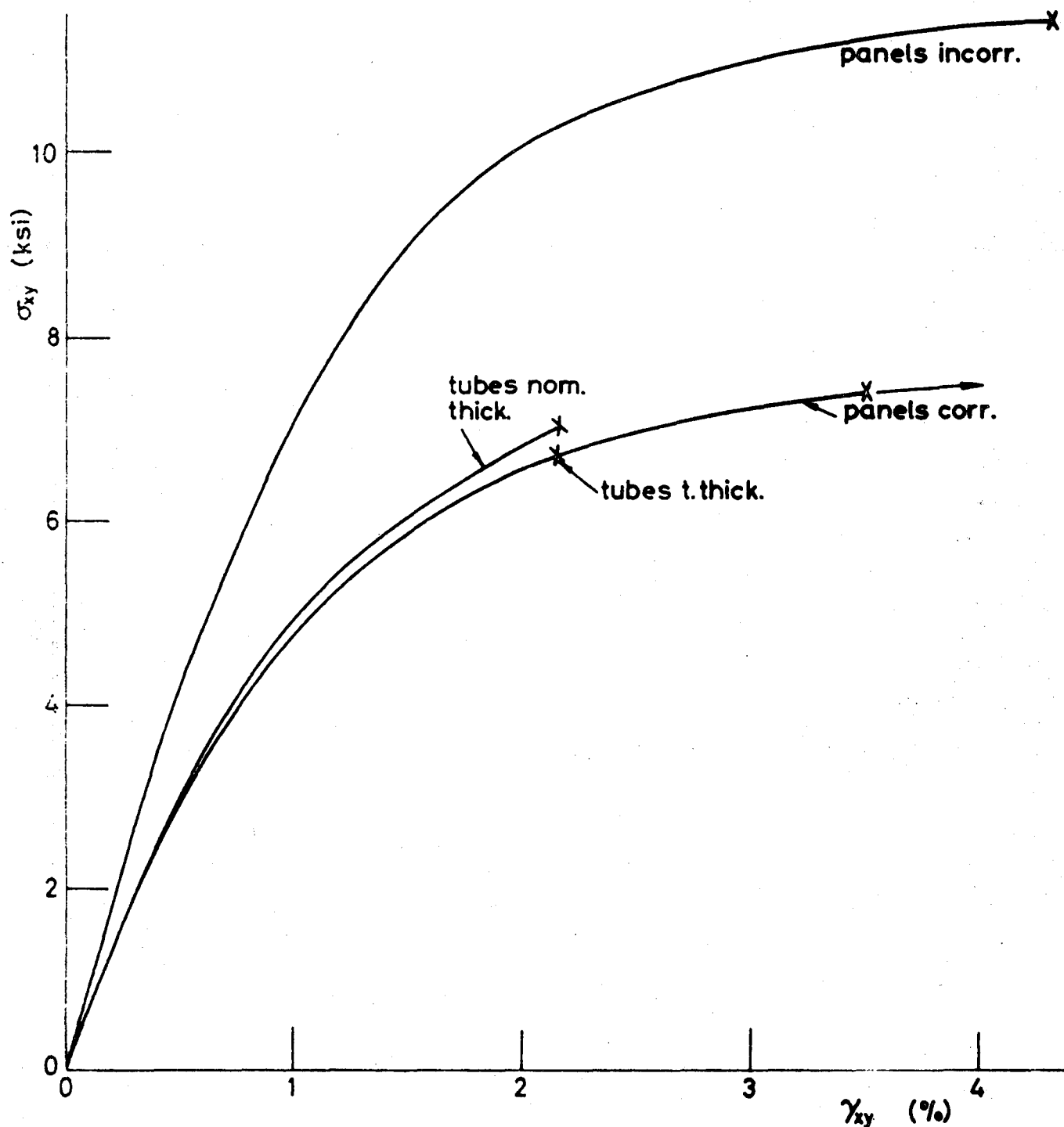
FIG. 18C SHEAR RESPONSE OF Q/90° AVCO 5505/5.6 MIL. BORON-EPOXY LAMINATES
