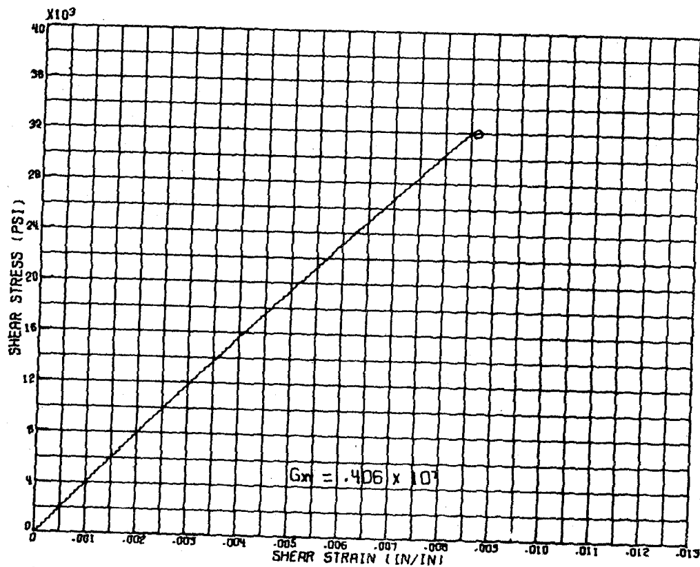
FIGURE 15B:-SHEAR RESPONSE OF TUBULAR SPECIMENS-[±15°] B/EP
