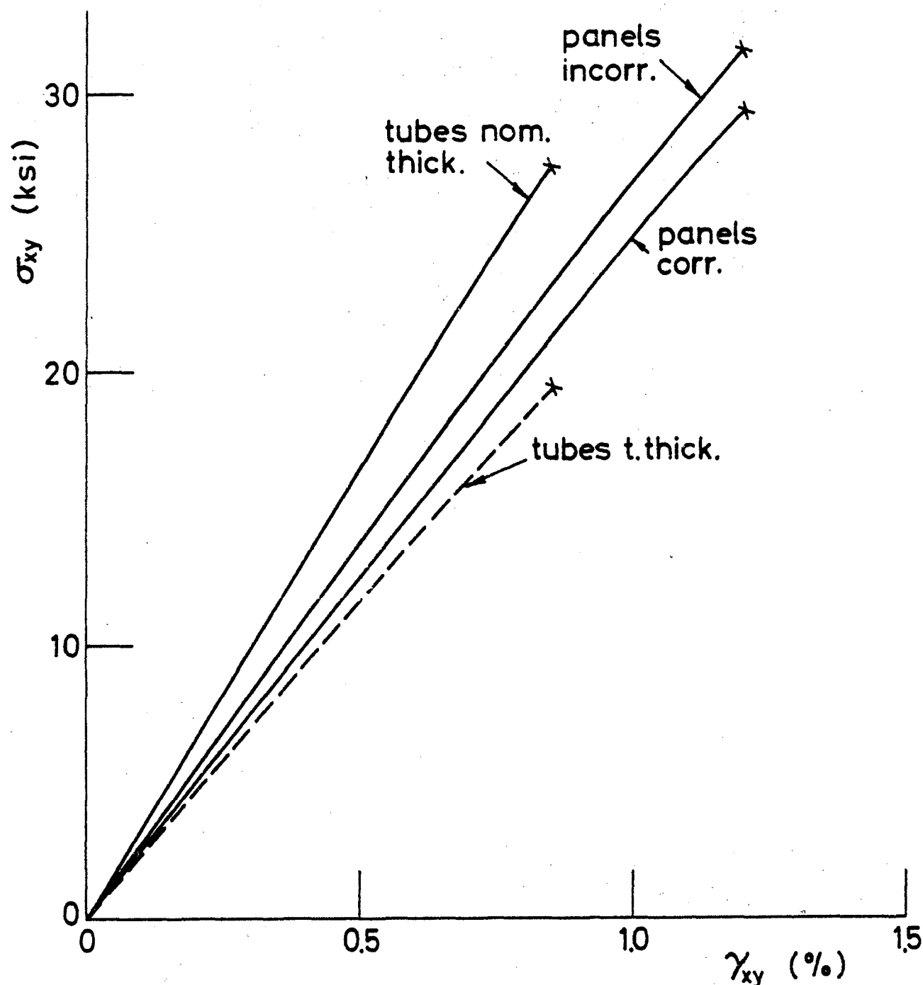
FIG. 13C SHEAR RESPONSE OF 0/±45/90° 3M SP-286T3 GRAPHITE-EPOXY LAMINATES
