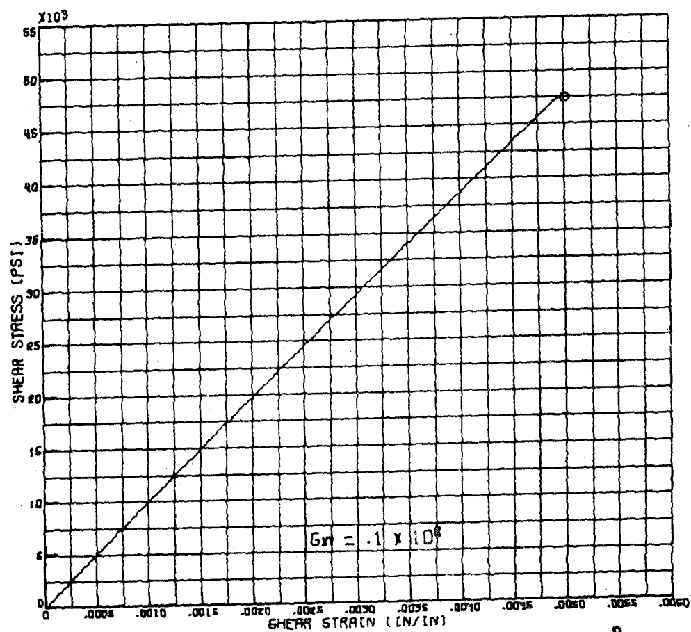
FIGURE 168 -- SHEAR RESPONSE OF TUBULAR SPECIMENS - C±30° B/EP
