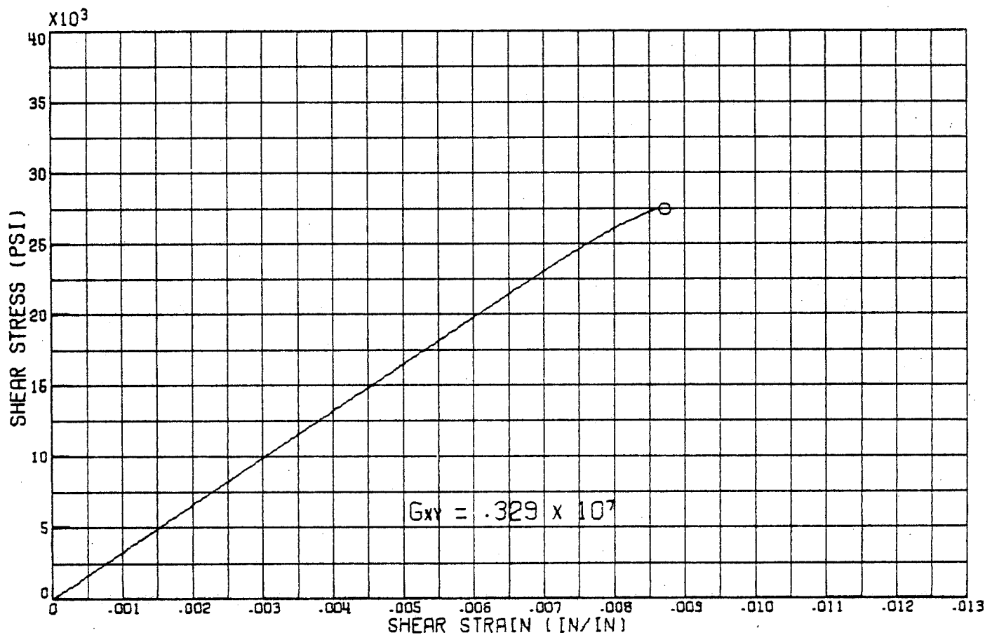
FIGURE 13B ;--SHEAR RESPONSE OF TUBULAR SPECIMENS-[0/±45/90] GR/EP
