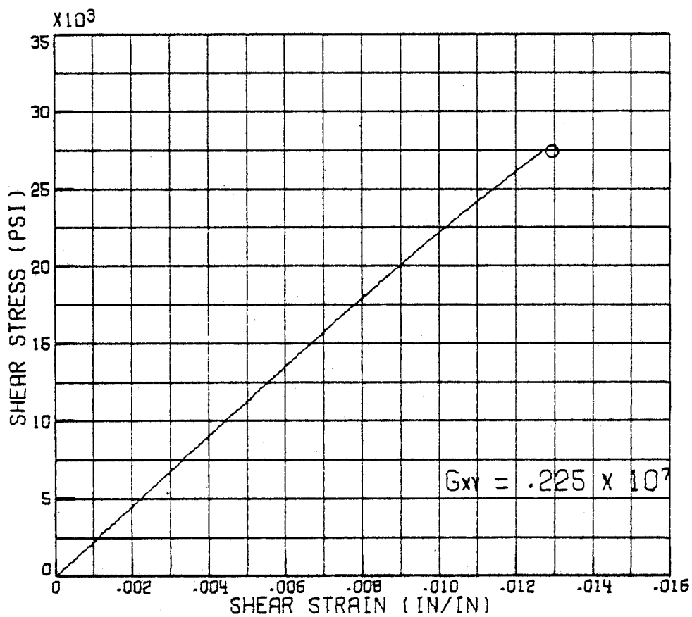
FIGURE 9B ; -SHEAR RESPONSE OF TUBULAR SPECIMENS. [±15°] GR/EP
