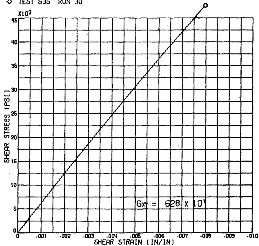
FIGURE 11B :-SHEAR RESPONSE OF TUBULAR SPECIMENS-[C±45] GR/EP
