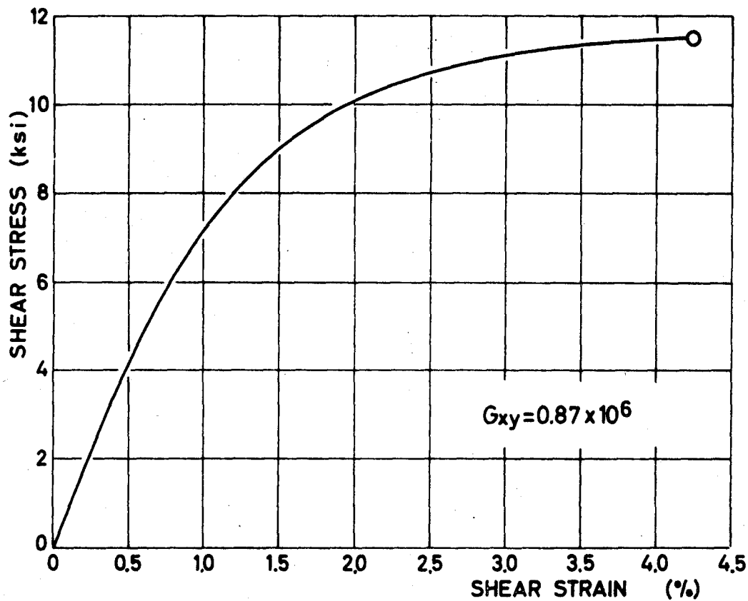
FIG. 18A SHEAR RESPONSE OF PLANAR SPECIMENS 0/90° B/EP
