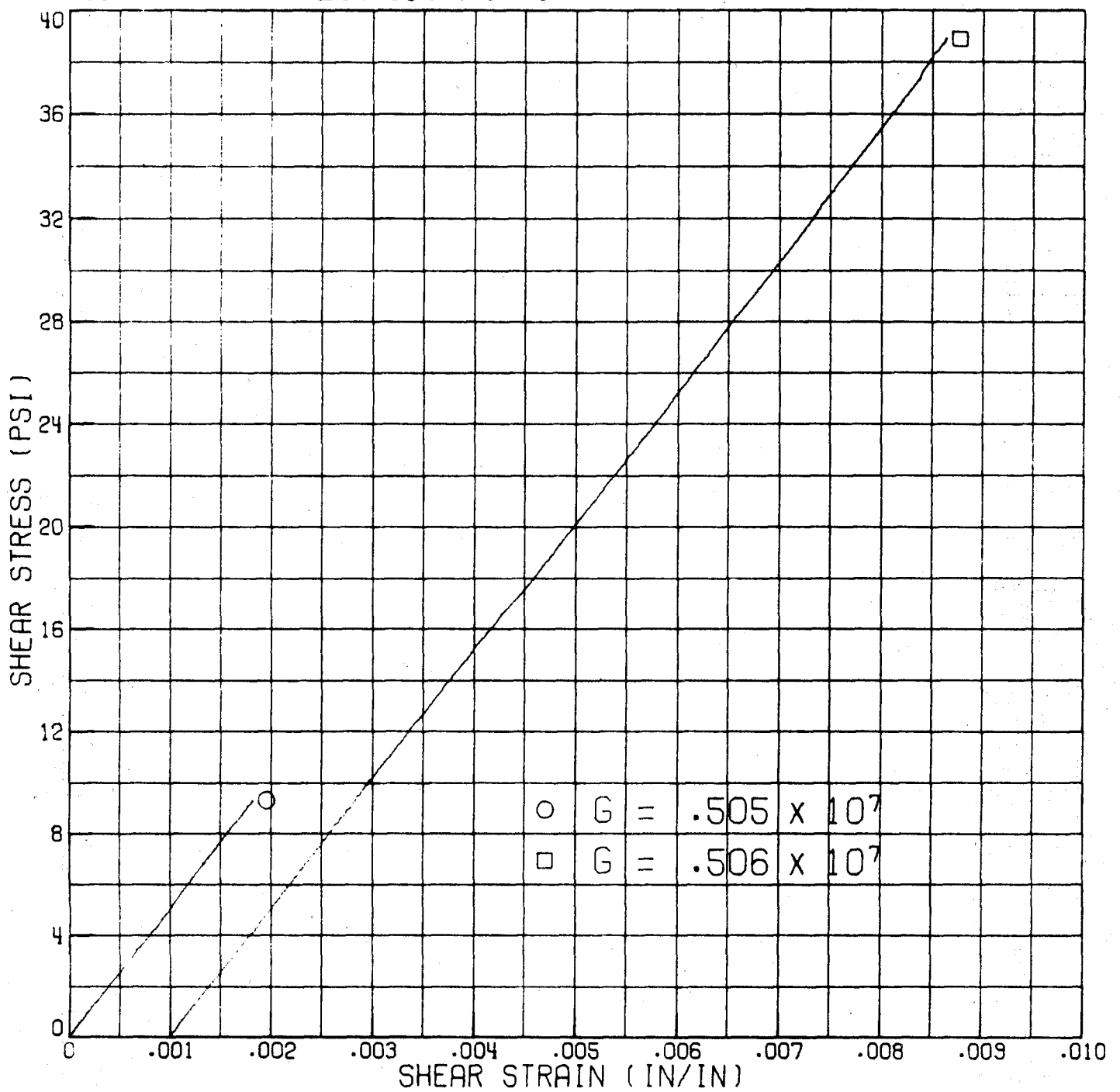
FIG. APA 21 -INFLUENCE OF LOADING AND UNLOADING ON RESPONSE OF SHEAR TUBES-[±30] GR/EP
