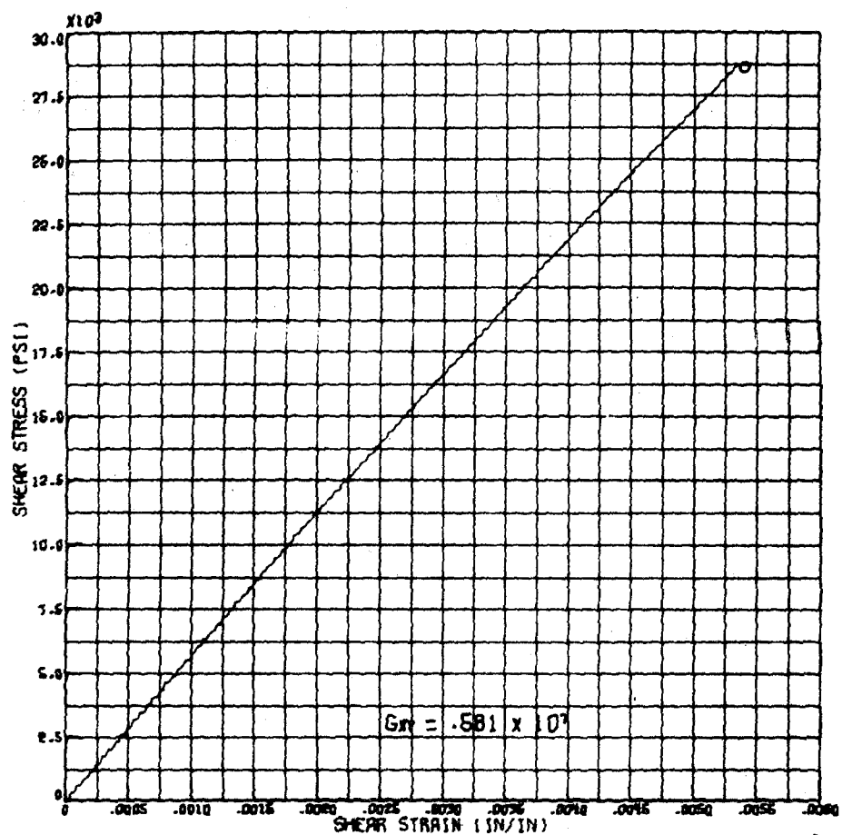
FIGURE 19B:-SHEAR RESPONSE OF TUBULAR SPECIMENS-CO/145/90° B/EP
