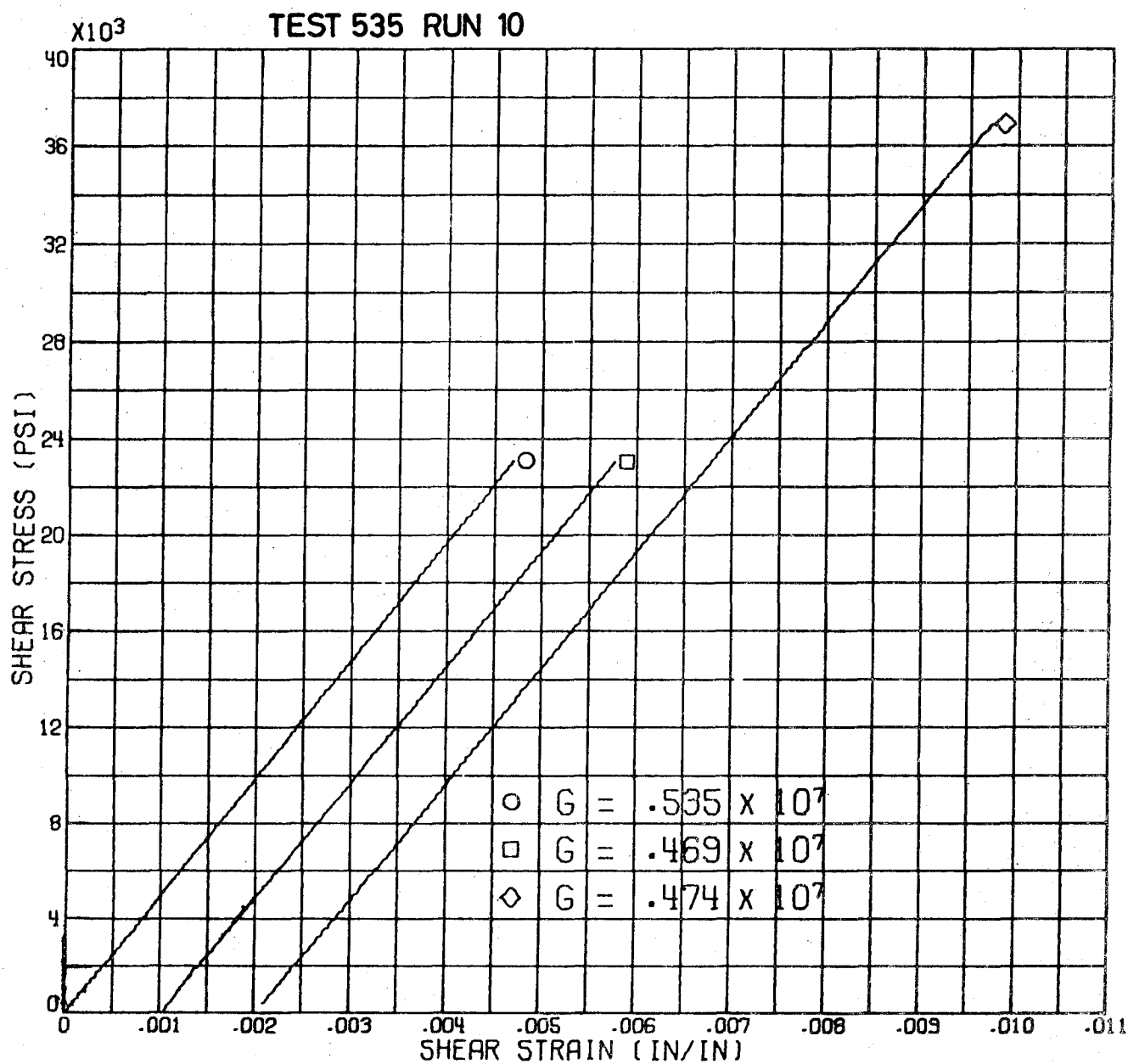
FIG. APA 2 II - INFLUENCE OF LOADING AND UNLOADING ON RESPONSE OF SHEAR TUBES-C \pm 30J GR/EP
