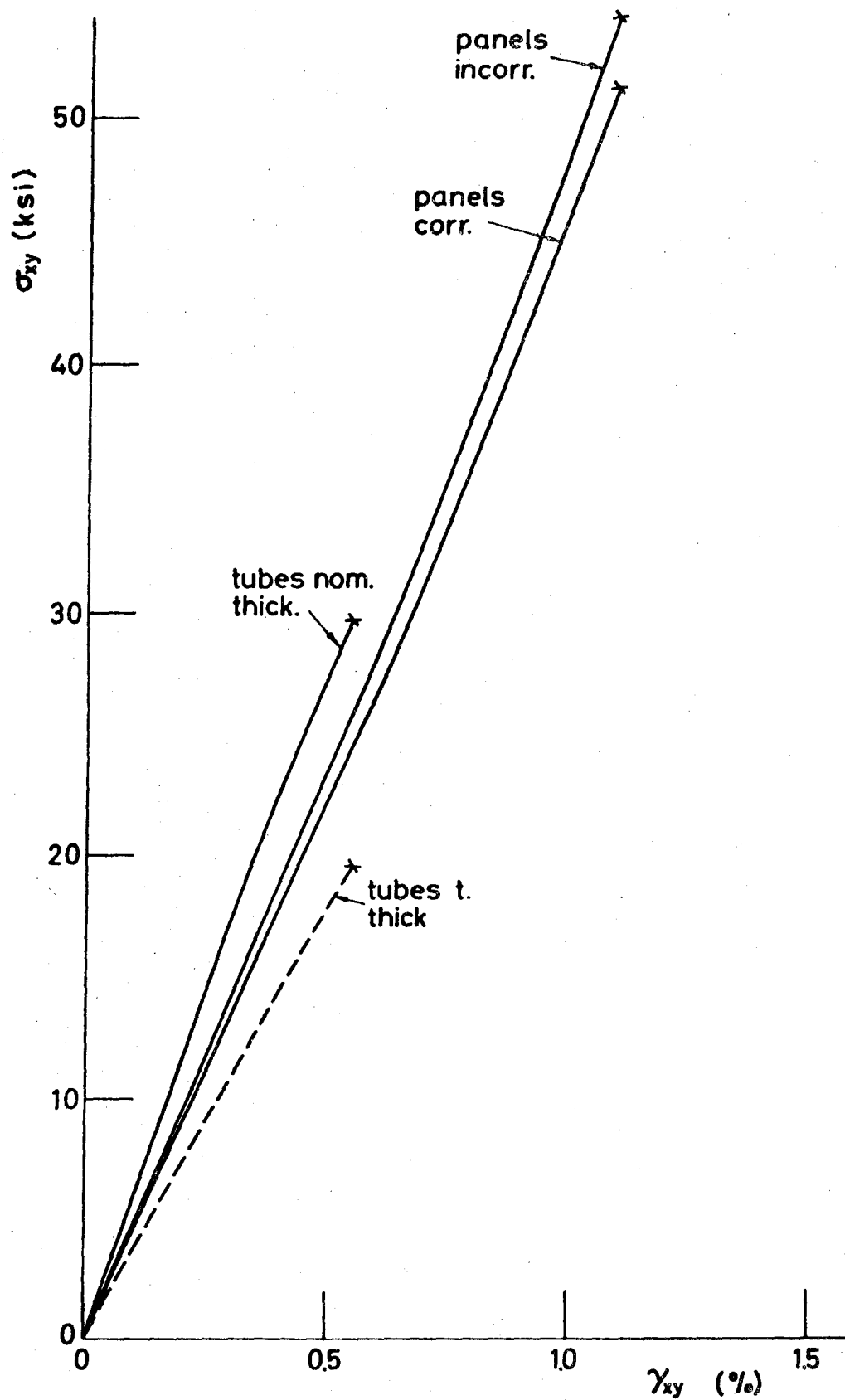
FIG. 19C SHEAR RESPONSE OF 0/±45/90° AVCO 5505/5.6 MIL BORON-EPOXY LAMINATES
