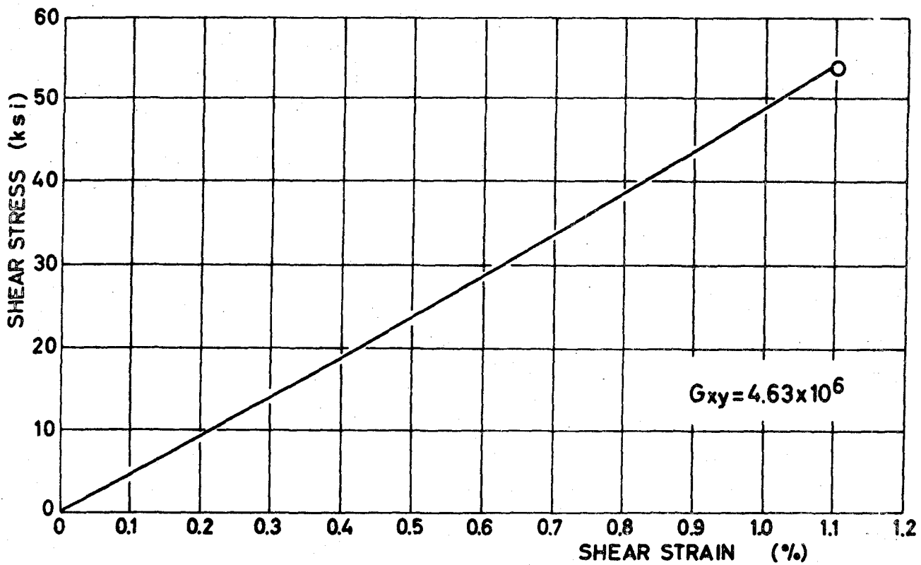
FIG. 19A SHEAR RESPONSE OF PLANAR SPECIMENS 0/±45/90° B/EP
