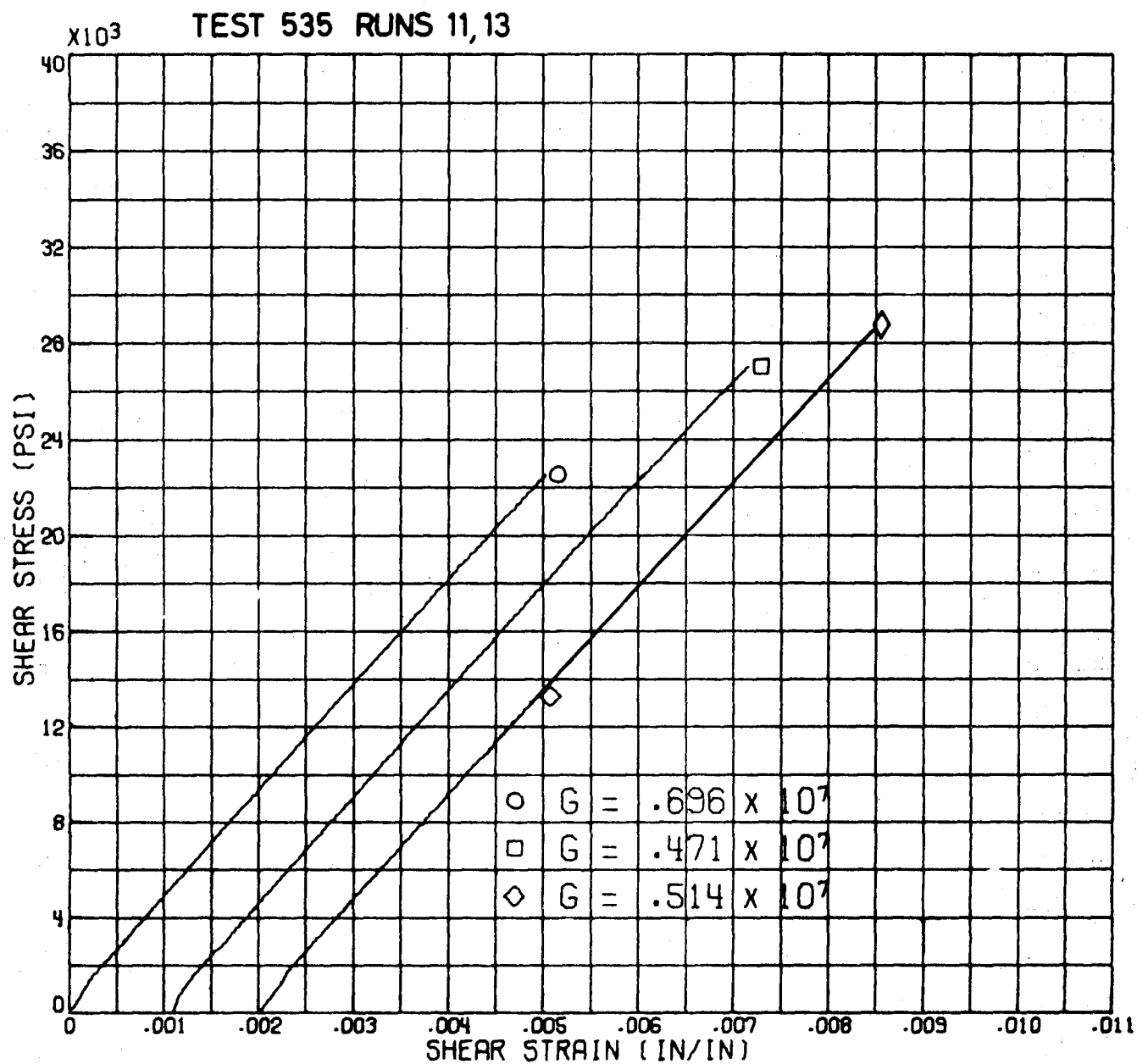
FIG. APA 2 III - INFLUENCE OF LOADING AND UNLOADING ON RESPONSE OF SHEAR TUBES-[±30] GR/EP
