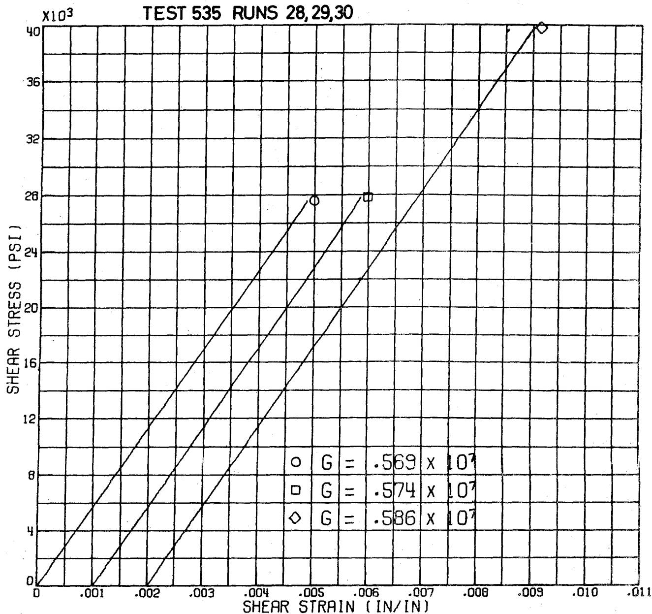
FIG. APA 3 - INFLUENCE OF LOADING AND UNLOADING ON RESPONSE OF SHEAR TUBES-[±45] GR/EP
