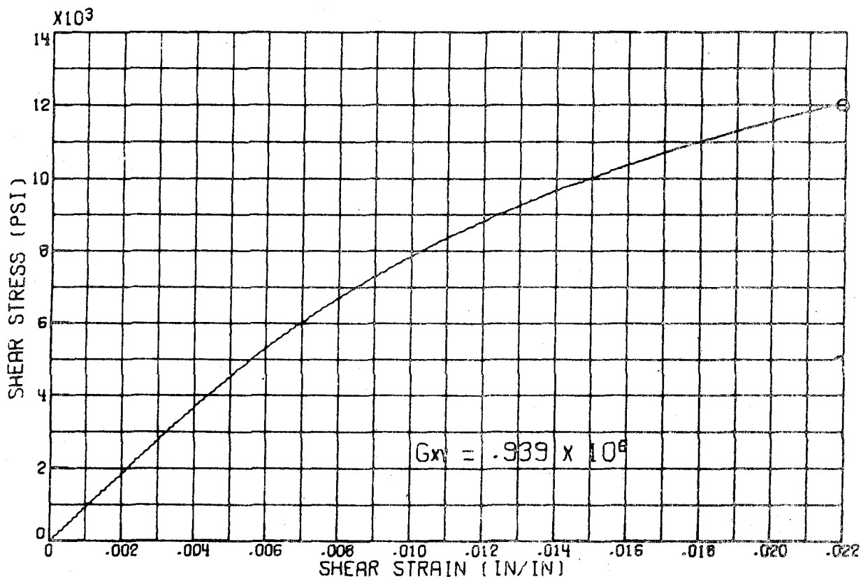
FIGURE 8B :-SHEAR RESPONSE OF TUBULAR SPECIMENS-[90°] GR/EP
