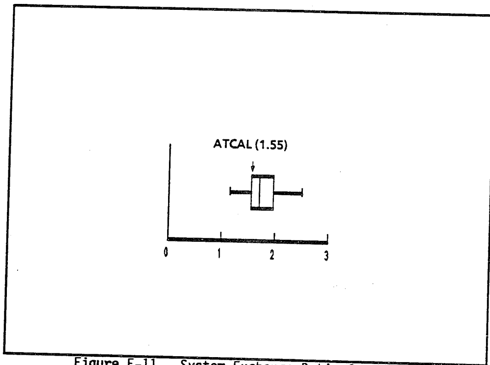
Figure E-11. System Exchange Ratio for MIAI, 7.0:1 Force Ratio
