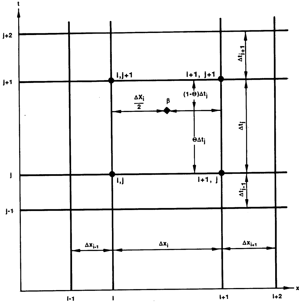
Figure 4. Numerical grid
