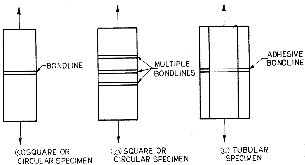
FIG. 5.2 ALTERNATE ADHESIVE BUTT JOINT SPECIMENS
