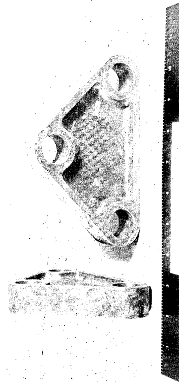
GRAPHITE/PMR-15 CHOPPED FIBER FITTINGS FIGURE 67
