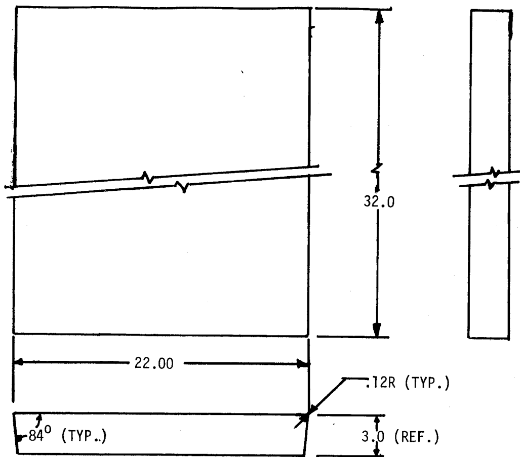
LAYUP MANDREL - END CLOSURE TASK H
