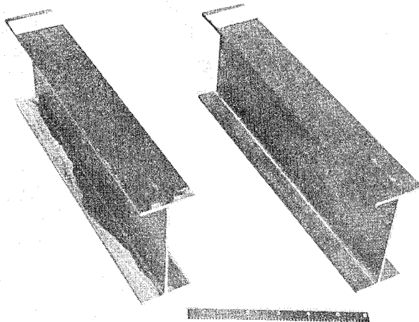
SECONDARY BONDED "I" STIFFENERS BEFORE POTTING
