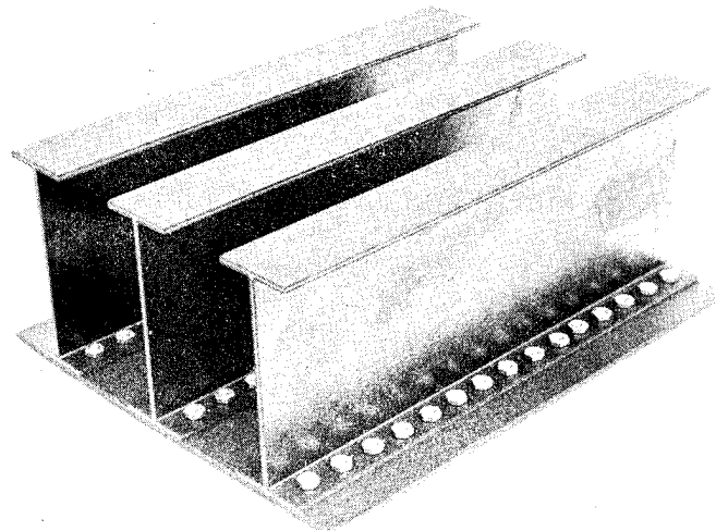
FIGURE 56 MECHANICALLY FASTENED "I" STIFFENED STRINGER PANEL
