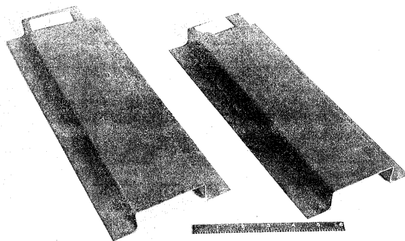
HAT SECTION STRUCTURAL ELEMENTS FIGURE 36
