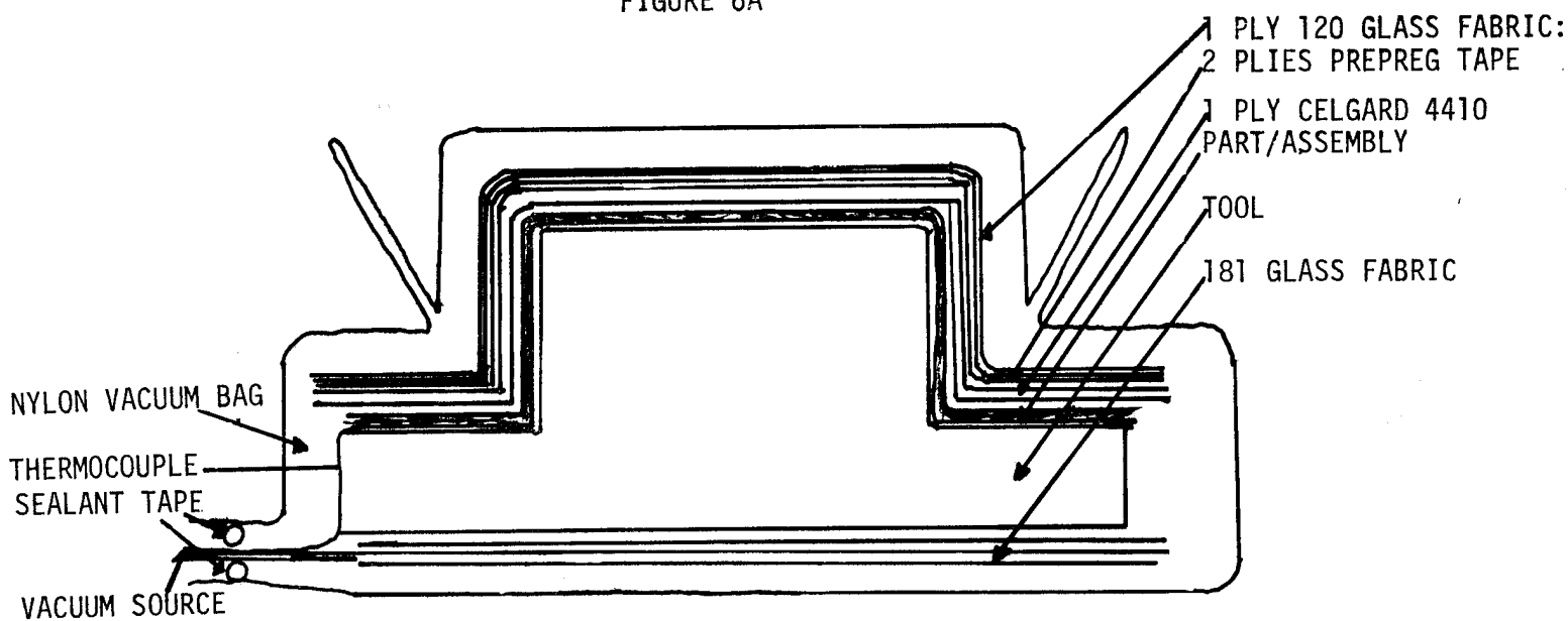
HAT SECTION LAYUP TO "B" STAGE PREPREG (D180-20545-4 CONDITION B PREPREG)
