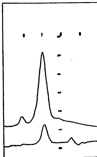
GEL PERMEATION CHROMATOGRAM FIGURE 7
