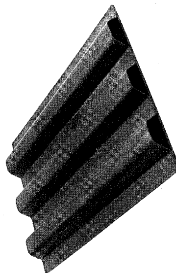
COCURED MULTIPLE HAT SECTION
