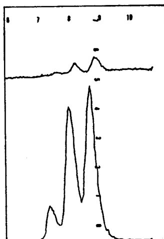
ADSORPTION CHROMATOGRAM FIGURE 9
