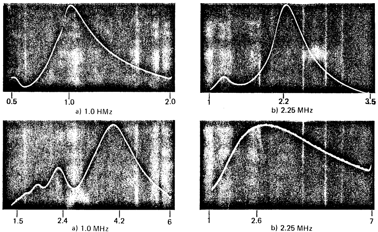
FIGURE 27 Frequency Response Curves of a Nortec 131 Ultrasonic Test Instrument at Various Frequencies (f) in Mega Hertz (MHz)
