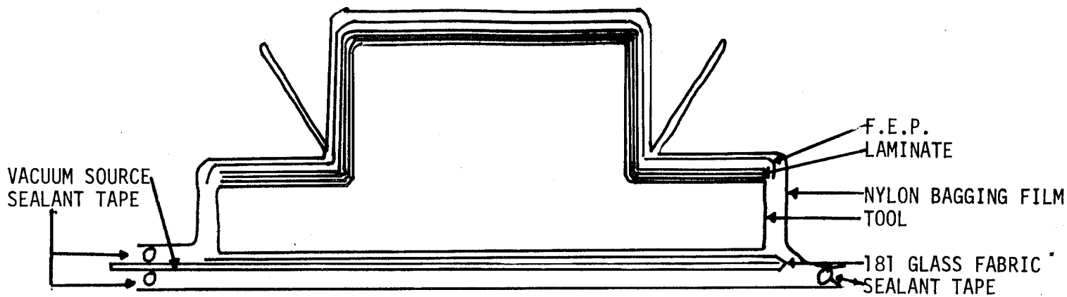
VACUUM BAG SCHEMATIC HAT SECTION LAYUP
