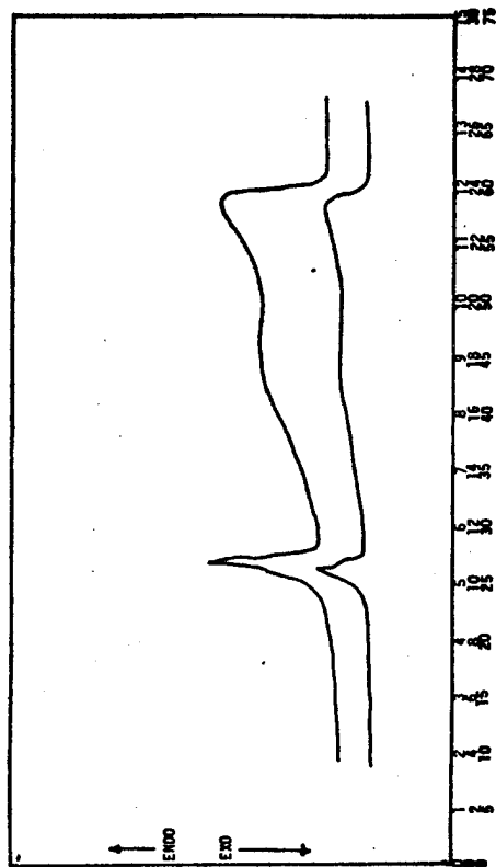
DSC ON COMPANY A NE MONOMER FIGURE 12
