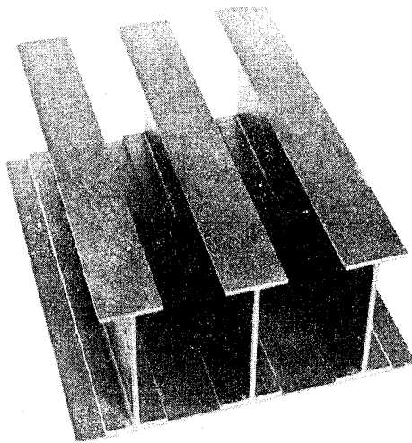
FIGURE 55 TASK E SECONDARY BONDED "I" STIFFENED STRINGER PANEL
