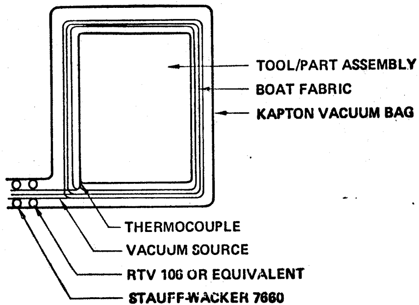
VACUUM BAG FOR "I" BEAM BONDING FIGURE 8B
