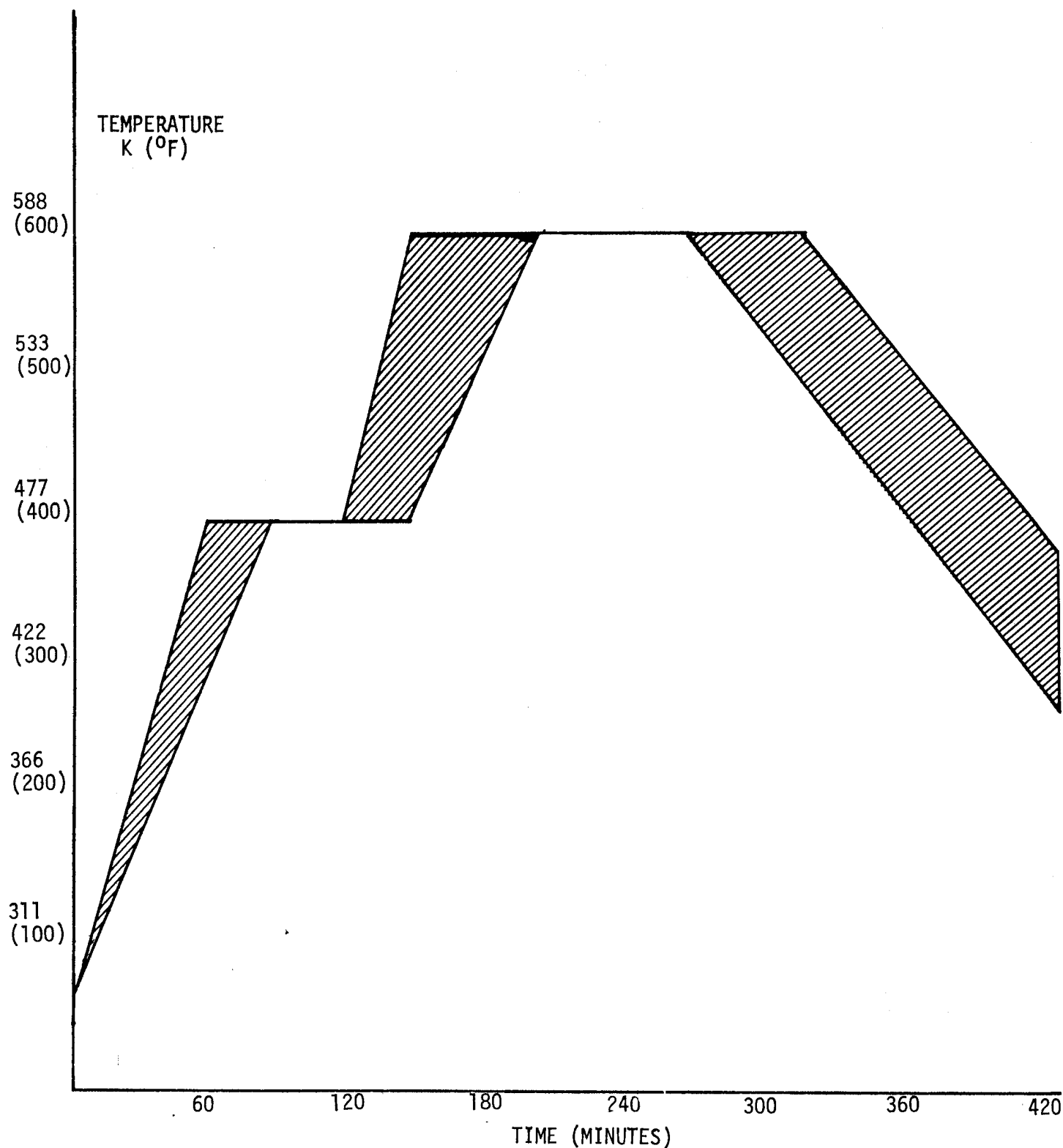
CURE CYCLE GRAPHITE/PMR-15 POLYIMIDE HONEYCOMB PANEL FIGURE 11
