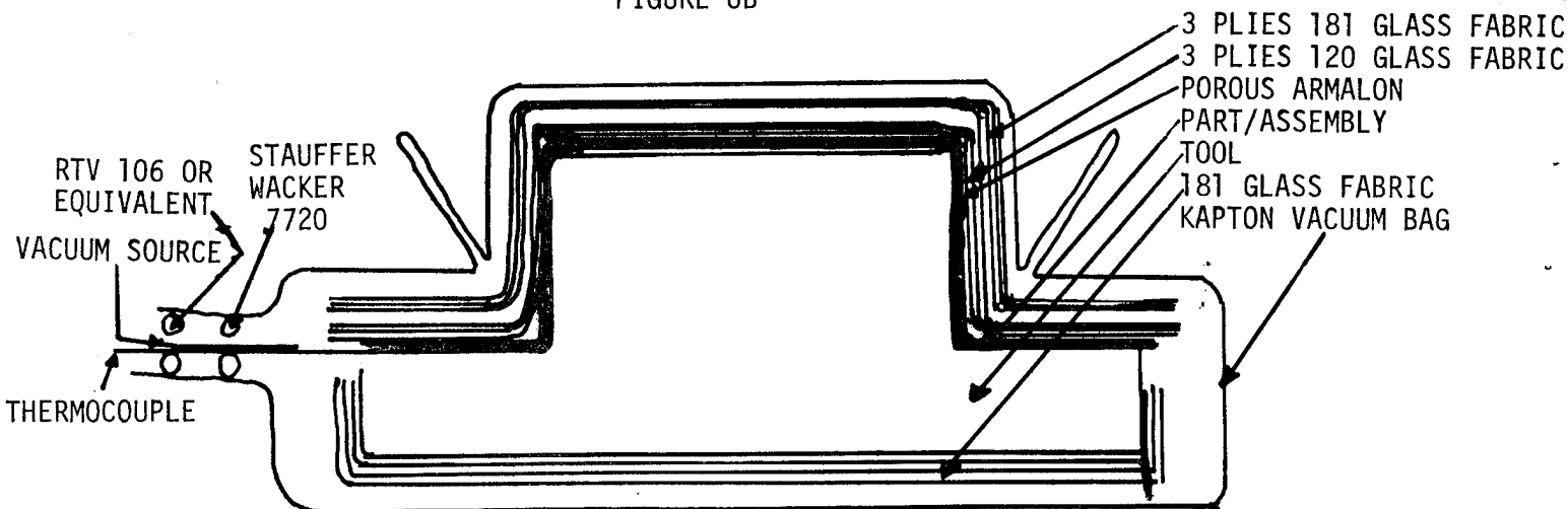
HAT SECTION KAPTON VACUUM BAG SCHEMATIC FIGURE 6C
