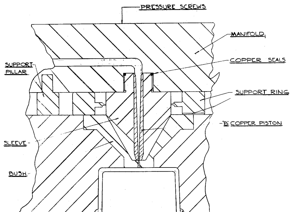
FIGURE 6: Piston Type Nozzle
