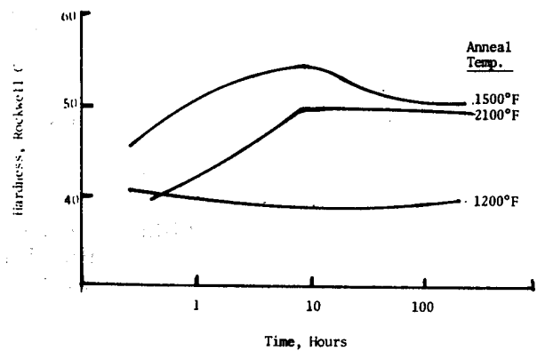
FIGURE 5: Effect of Aging at 900°F on Hardness After Initial Annealing At the Indicated Temperatures
