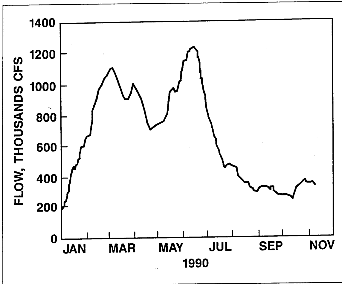
Figure 5. 1990 discharge hydrograph
