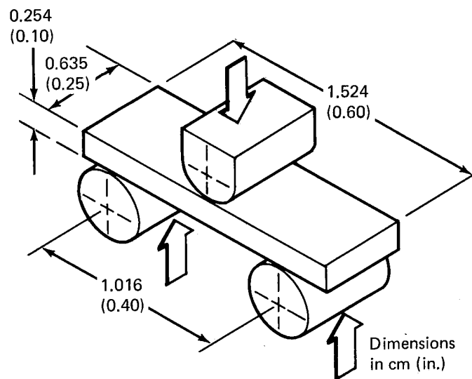
Figure 4. Short-Beam-Shear Test Specimen
