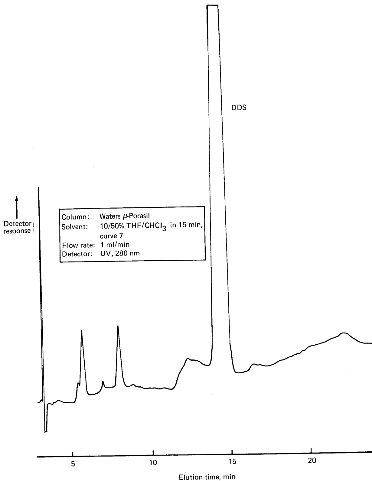
Figure 18. LC Chromatogram of DDS, Solvent: THF/ \text{CHCl}_3
