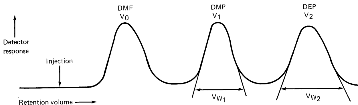
Figure A-1. Example LC Chromatogram for Column Calibration
