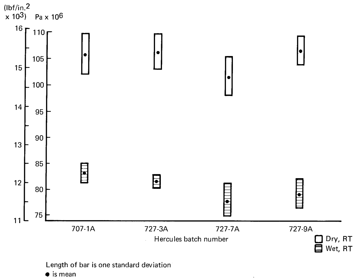
Figure 111. 0-deg Short-Beam-Shear Strength of Hercules Laminates
