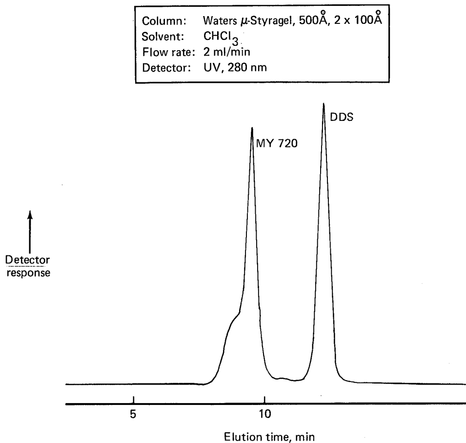
Figure 86. GPC Chromatogram of Narmco Neat Resin Batch 300, Solvent: \text{CHCl}_3 , Column: Waters \mu -Styragel-500Å, 2 x 100Å
