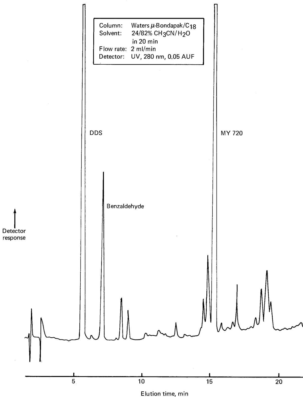
Figure 29. LC Chromatogram of Narmco Batch 286, Mobile Phase 1, Column: Waters \mu -Bondapak/C18
