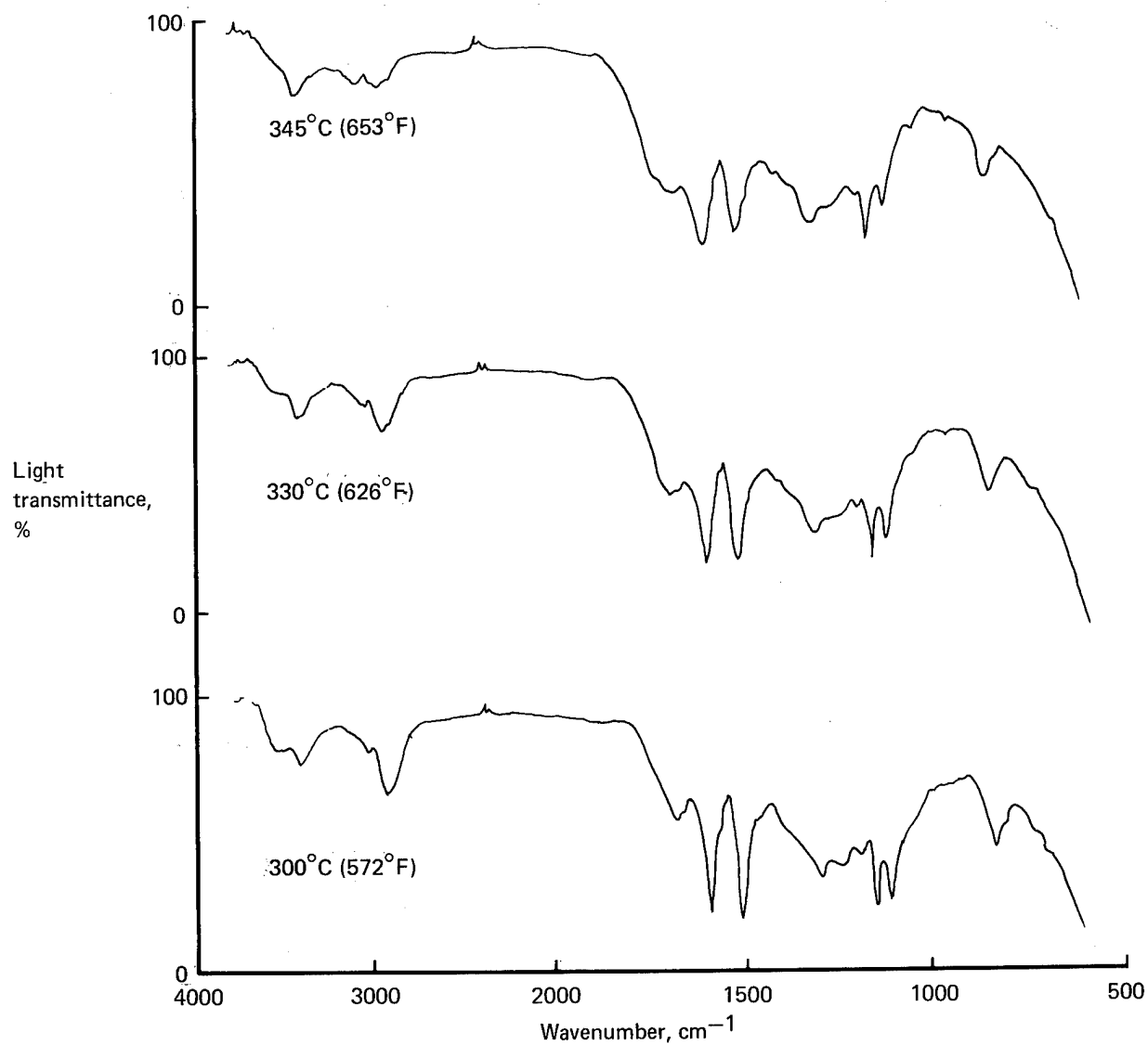
Figure 54. TSIR Spectra of Narmco Neat Resin Batch 300–300, 330, and 345°C (572, 626, and 653°F)
