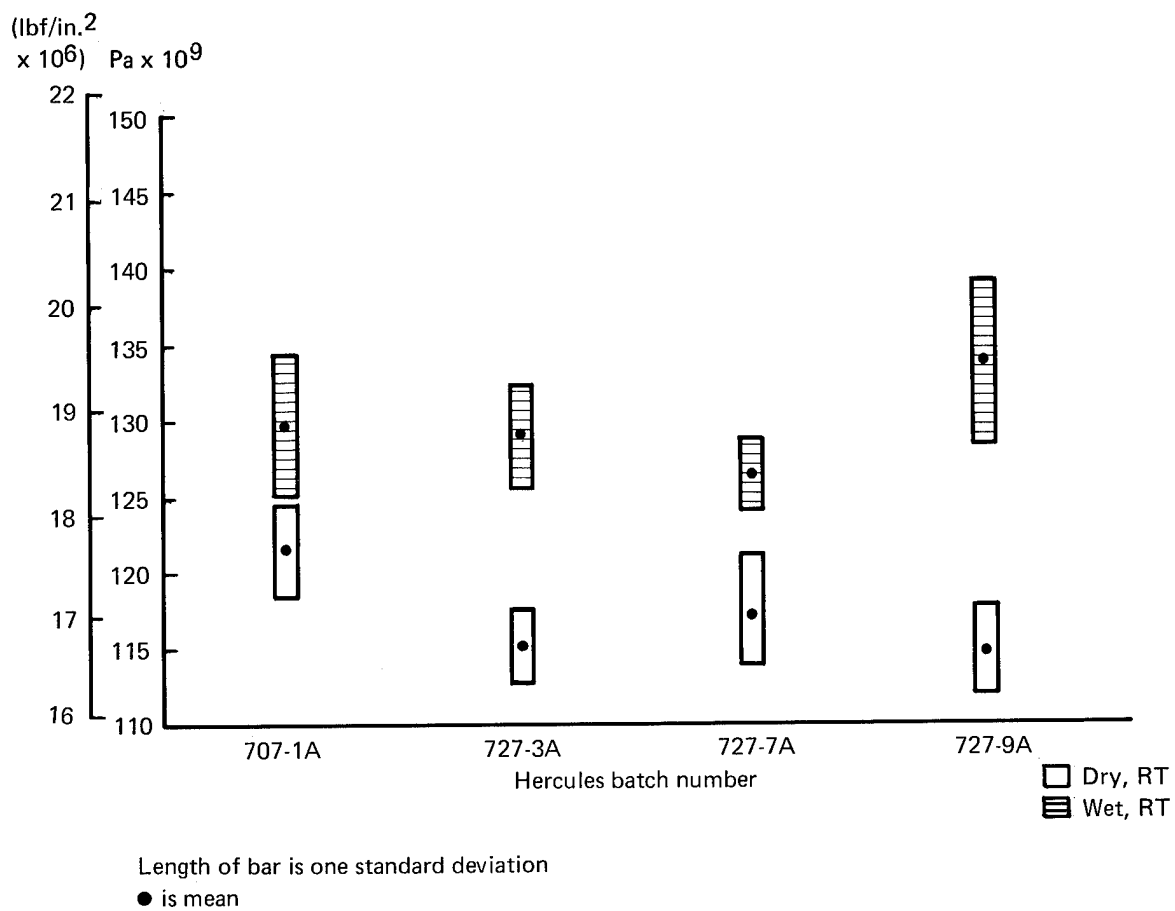
Figure 112. 0-deg Compression Modulus of Hercules Laminates
