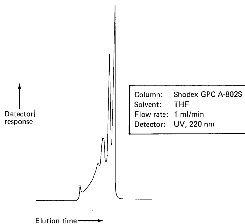
Figure 97. GPC Chromatogram of Narmco Prepreg Batch 1072, Round-Robin Participant H
