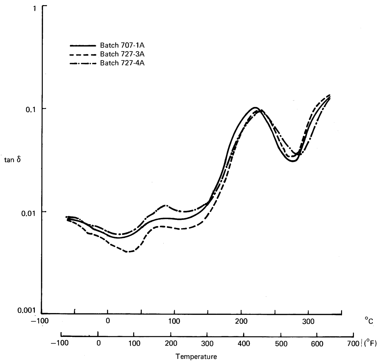
Figure 123. \tan \delta Versus Temperature, Hercules Laminates
