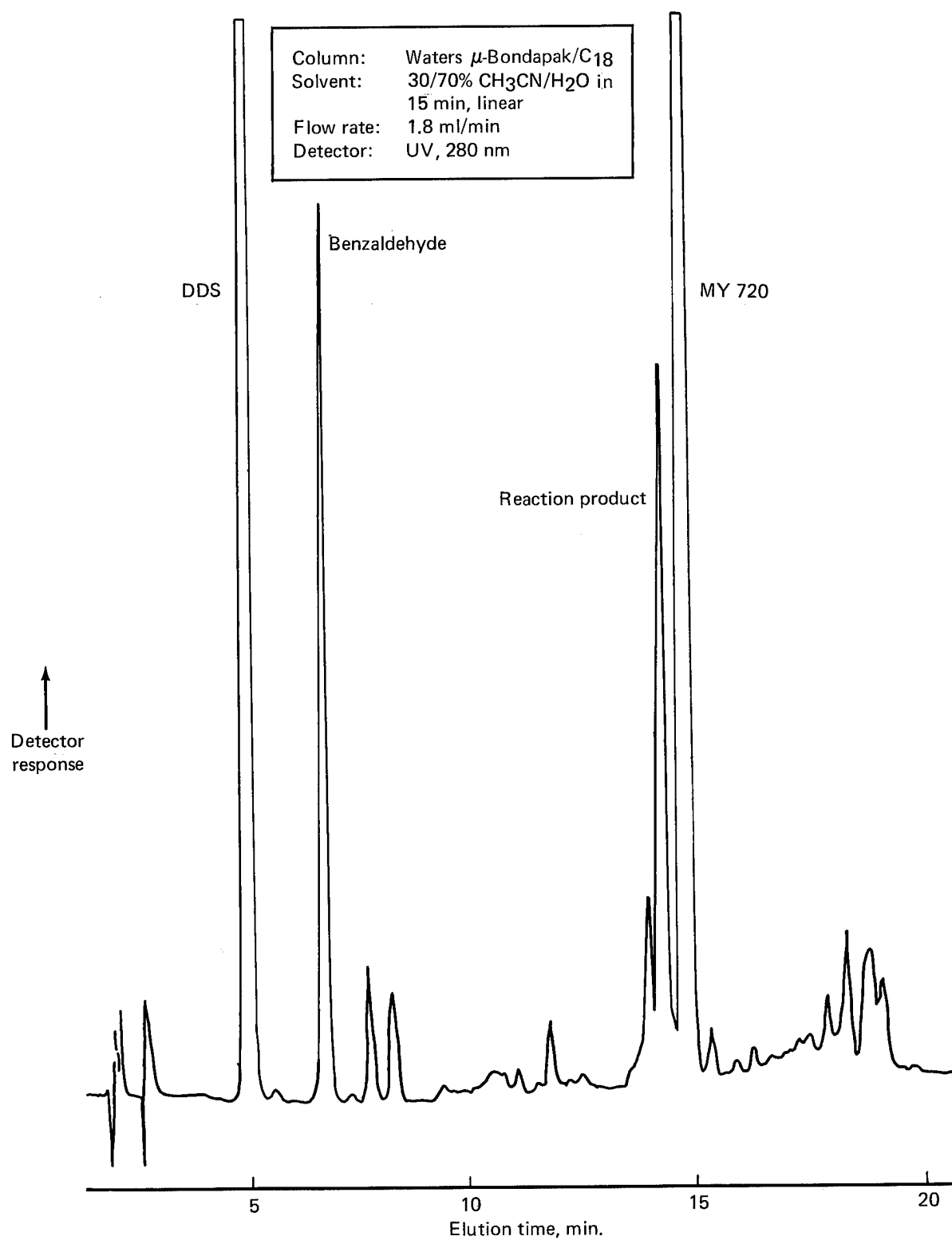
Figure 8. LC Chromatogram of Narmco Resin Matrix
