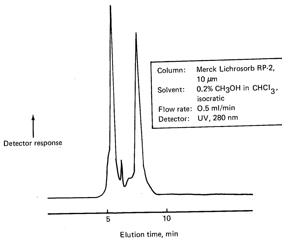
Figure 12. LC Chromatogram of Optimized TLC Mobile Phase
