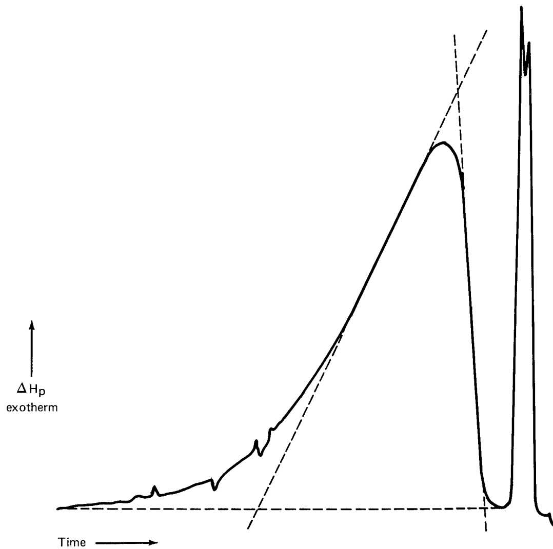
Figure 80. DSC Curve of Narmco Prepreg Batch 1072, Round-Robin Participant I
