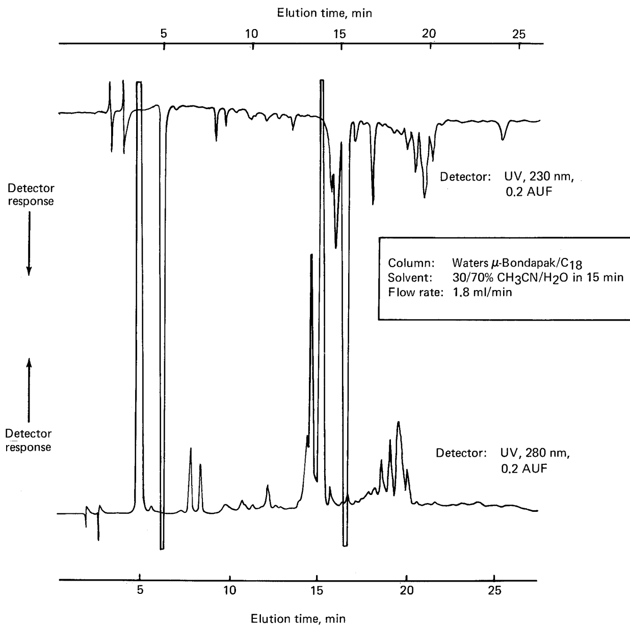
Figure 35. LC Chromatogram of Narmco Batch 286, Detector: UV, 230 nm
