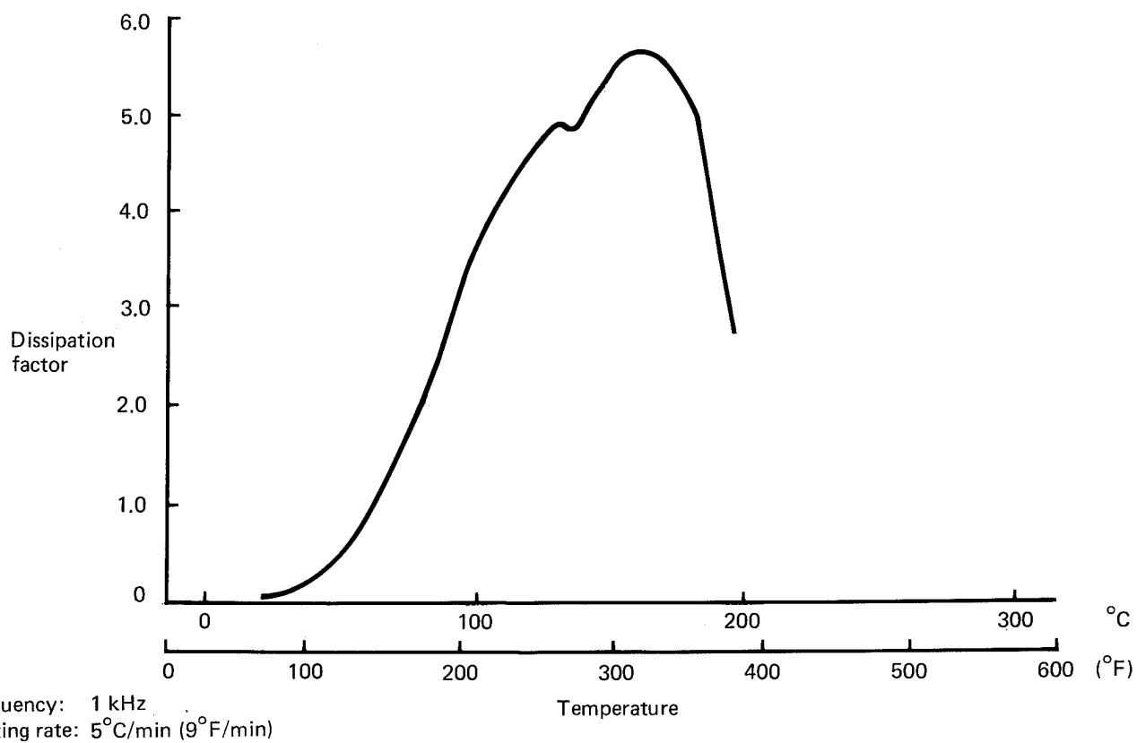
Figure 56. Results of Dielectric Analysis of Narmco Resin Batch 300
