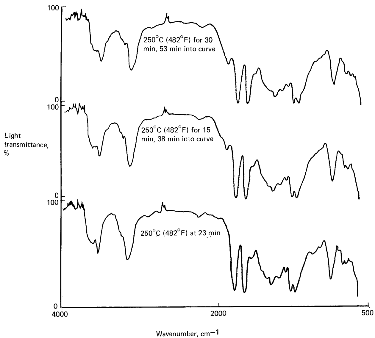
Figure 103. TSIR Spectra of Hercules Resin—250°C (482°F)
