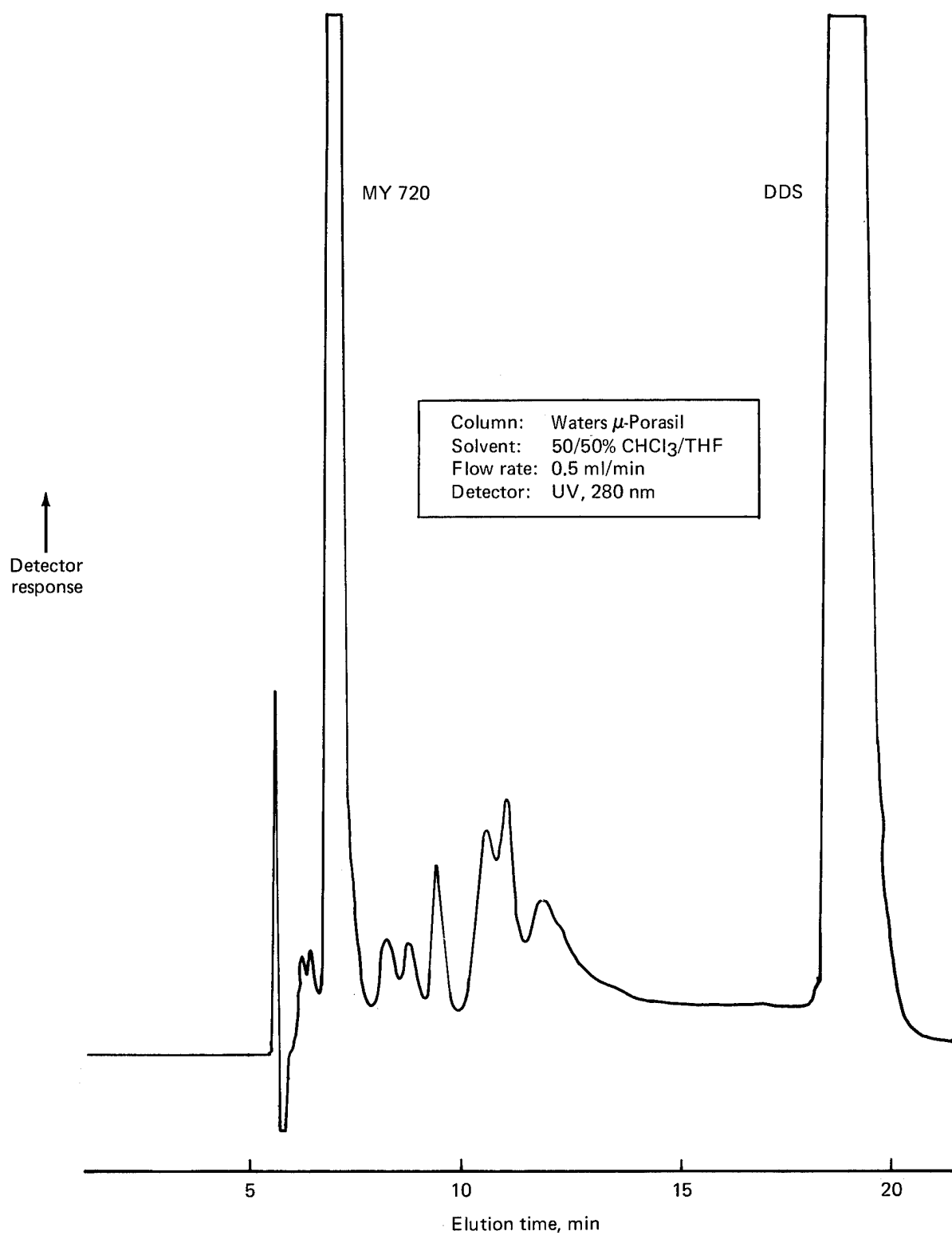
Figure 16. LC Chromatogram of Narmco Batch 286, Flow Rate: 0.5 ml/min
