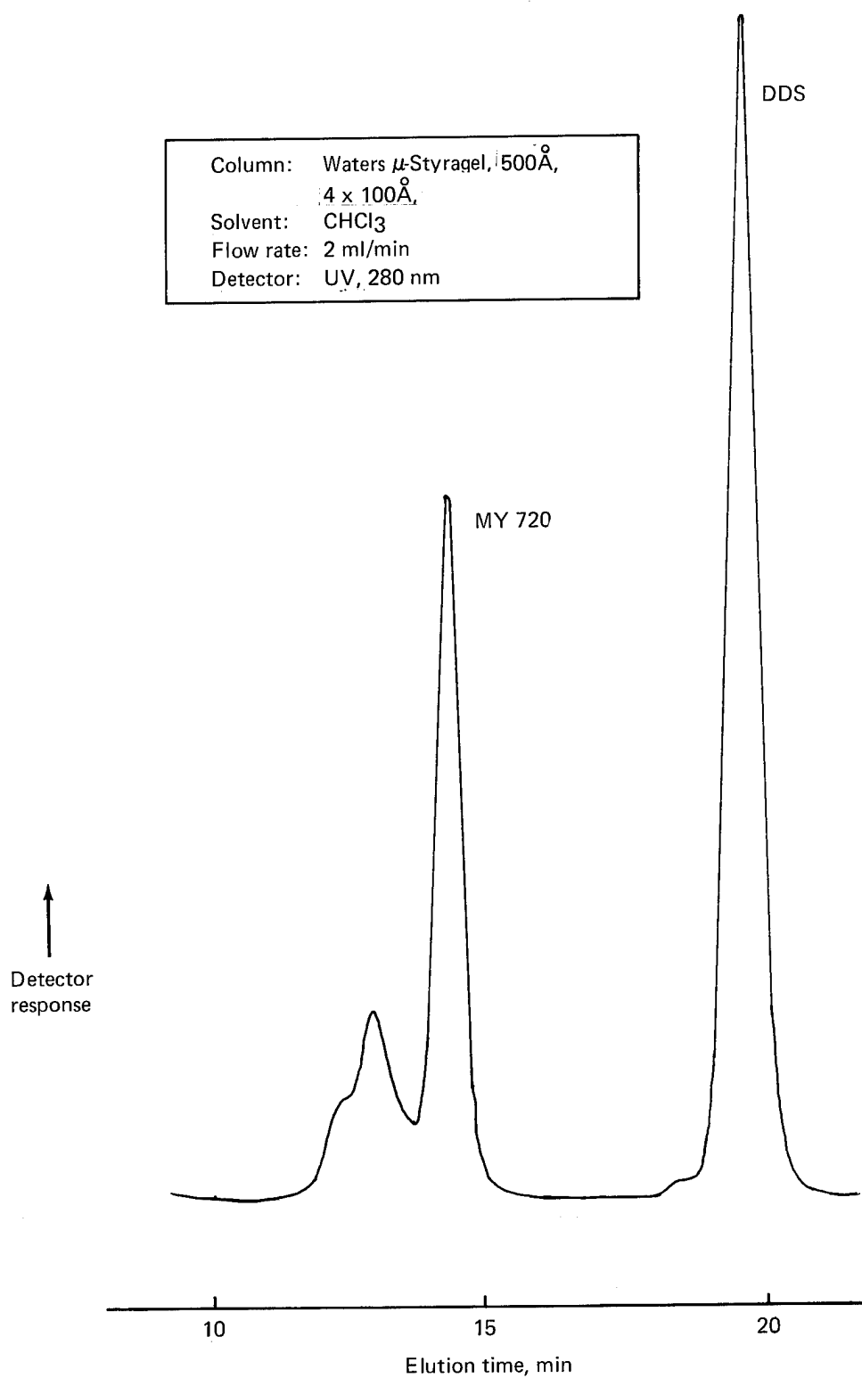
Figure 91. GPC Chromatogram of Narmco Neat Resin Batch 300, Solvent: \text{CHCl}_3 , Column: Waters \mu -Styragel—500Å, 4 x 100Å
