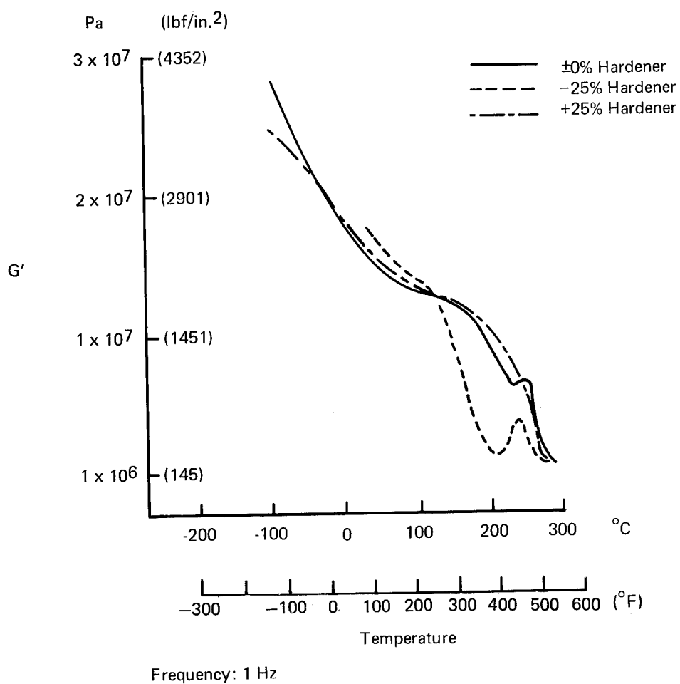
Figure 117. Elastic Modulus Versus Temperature, Narmco Matrix
