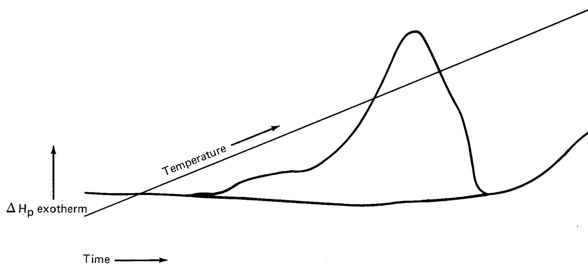
Figure 109. DSC Curve of Hercules Resin Batch 727-7A
