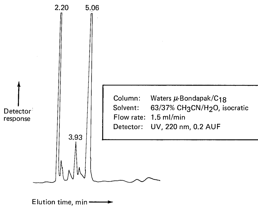
Figure 99. LC Chromatogram of Hercules Batch 707-1A, Using LC Round-Robin Procedure
