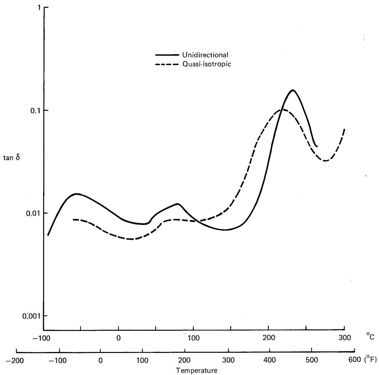
Figure 131. \tan \delta Versus Temperature, Hercules Laminates—Unidirectional and Quasi-Isotropic
