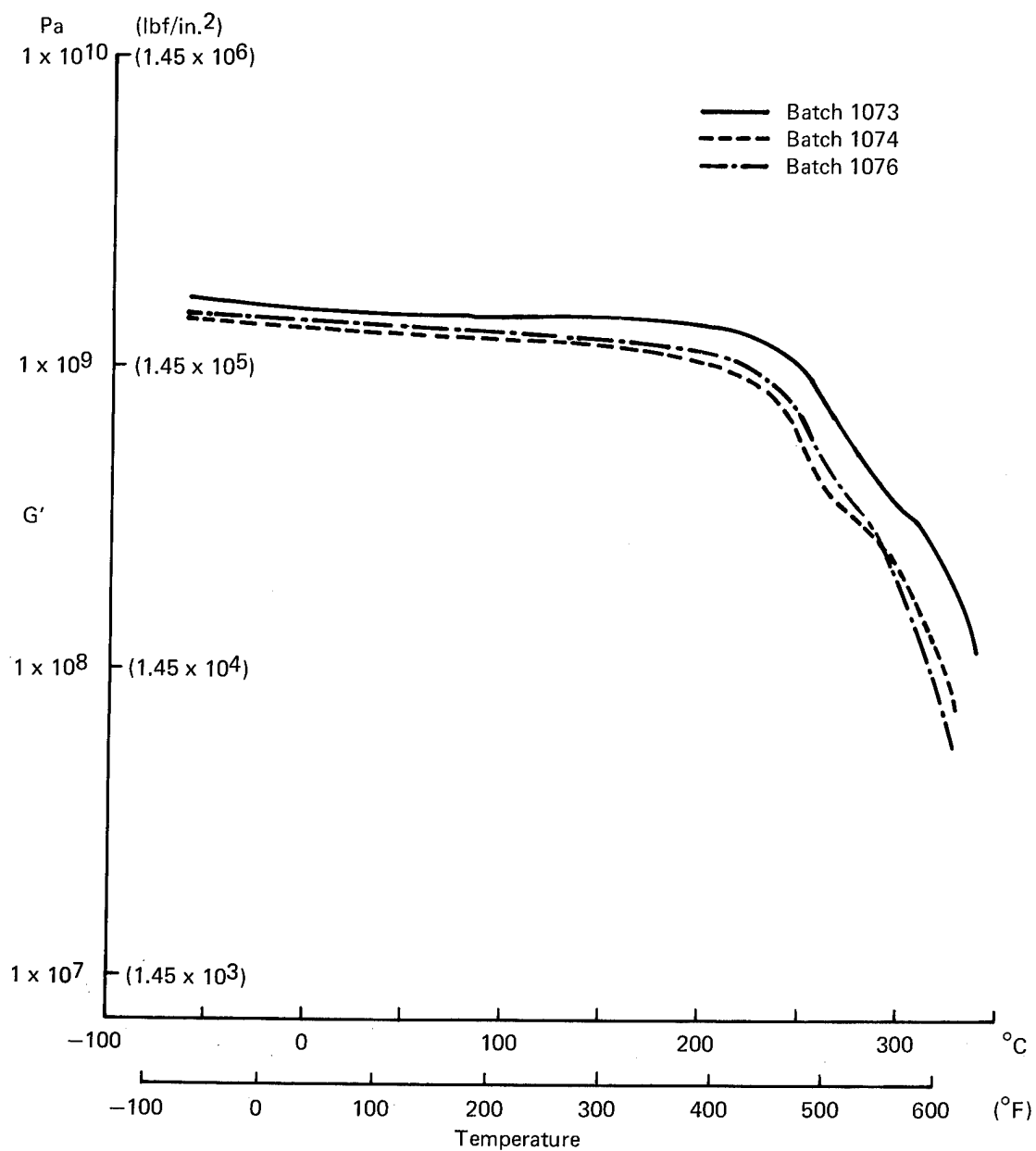
Figure 120. G' Versus Temperature, Narmco Laminates
