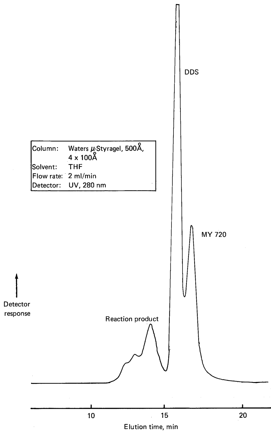
Figure 90. GPC Chromatogram of Narmco Neat Resin Batch 300, Solvent: THF, Column: Waters \mu -Styragel-500Å, 4 x 100Å
