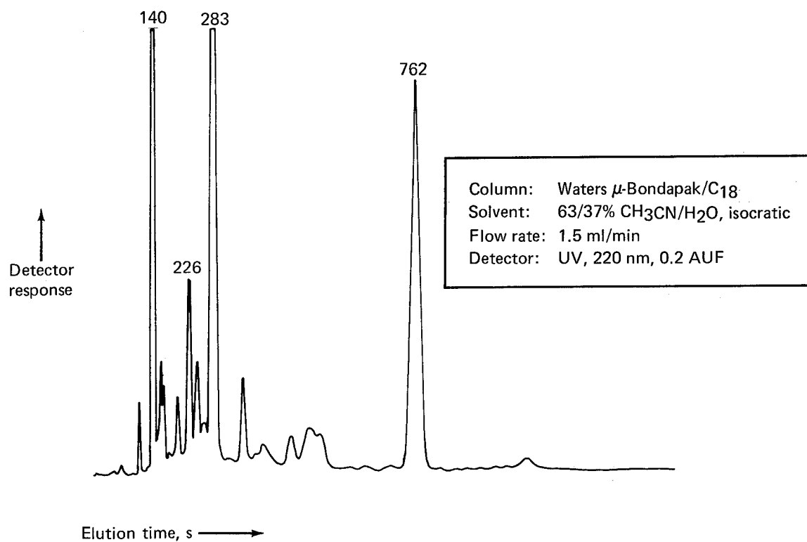
Figure 43. LC Chromatogram of Narmco Prepreg Batch 1072, Round-Robin Participant D
