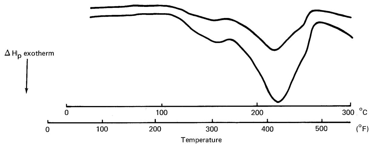
Figure 105. DSC Scan of Hercules Resin
