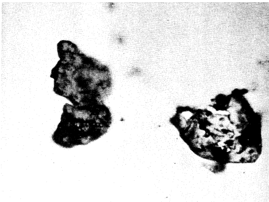
Figure 67. Contamination in Narmco Neat Resin Batch 300—Wear Metal
