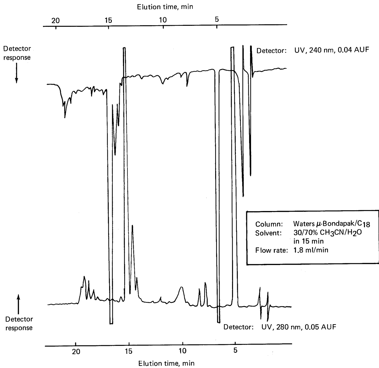
Figure 36. LC Chromatogram of Narmco Batch 286, Detector: UV, 240 nm
