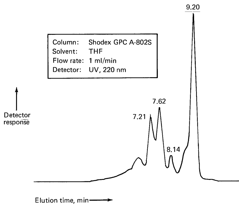
Figure 95. GPC Chromatogram of Narmco Prepreg Batch 1072, Round-Robin Participant E
