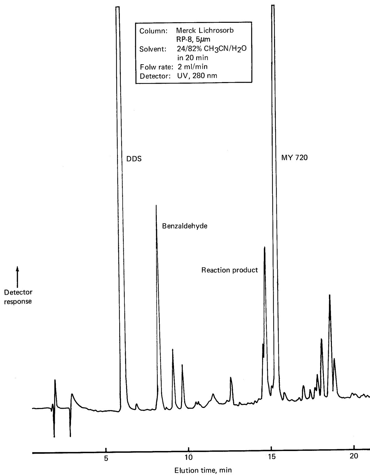
Figure 30. LC Chromatogram of Narmco Batch 286, Mobile Phase 1, Column: Merck Lichrosorb RP-8, 5 \mu m
