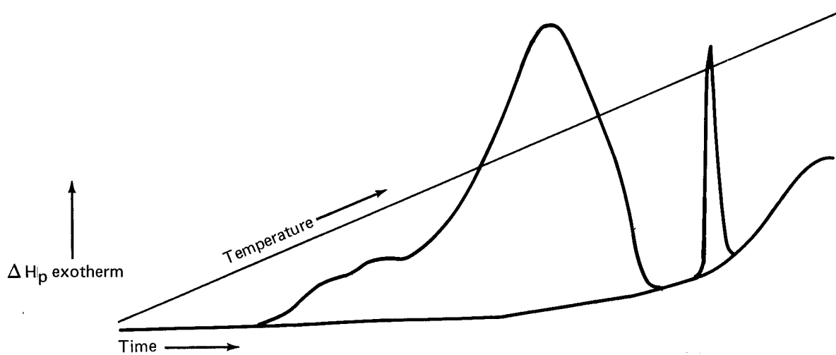
Figure 107. DSC Curve of Hercules Resin Batch 707-1A
