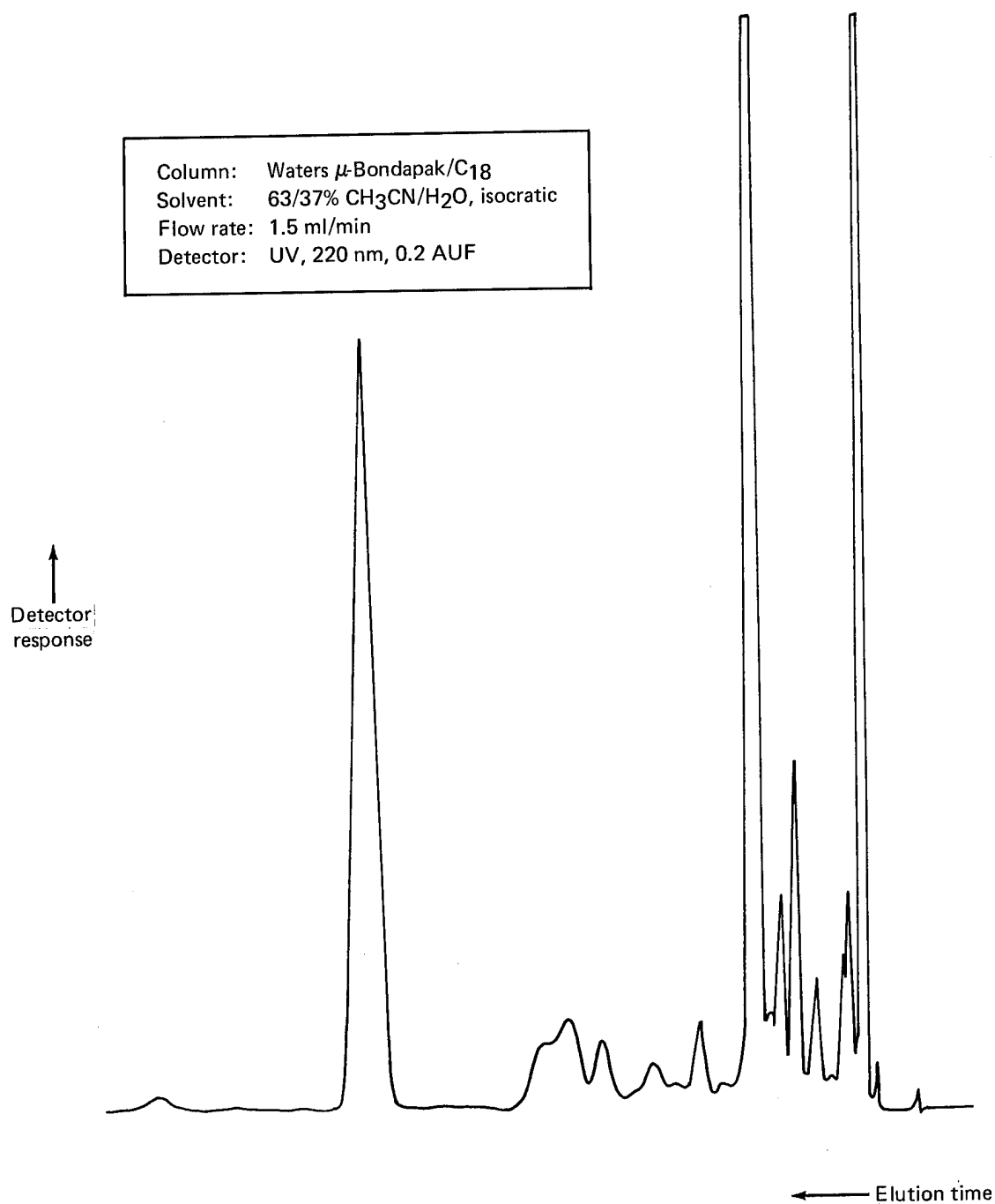
Figure 47. LC Chromatogram of Narmco Prepreg Batch 1072, Round-Robin Participant I
