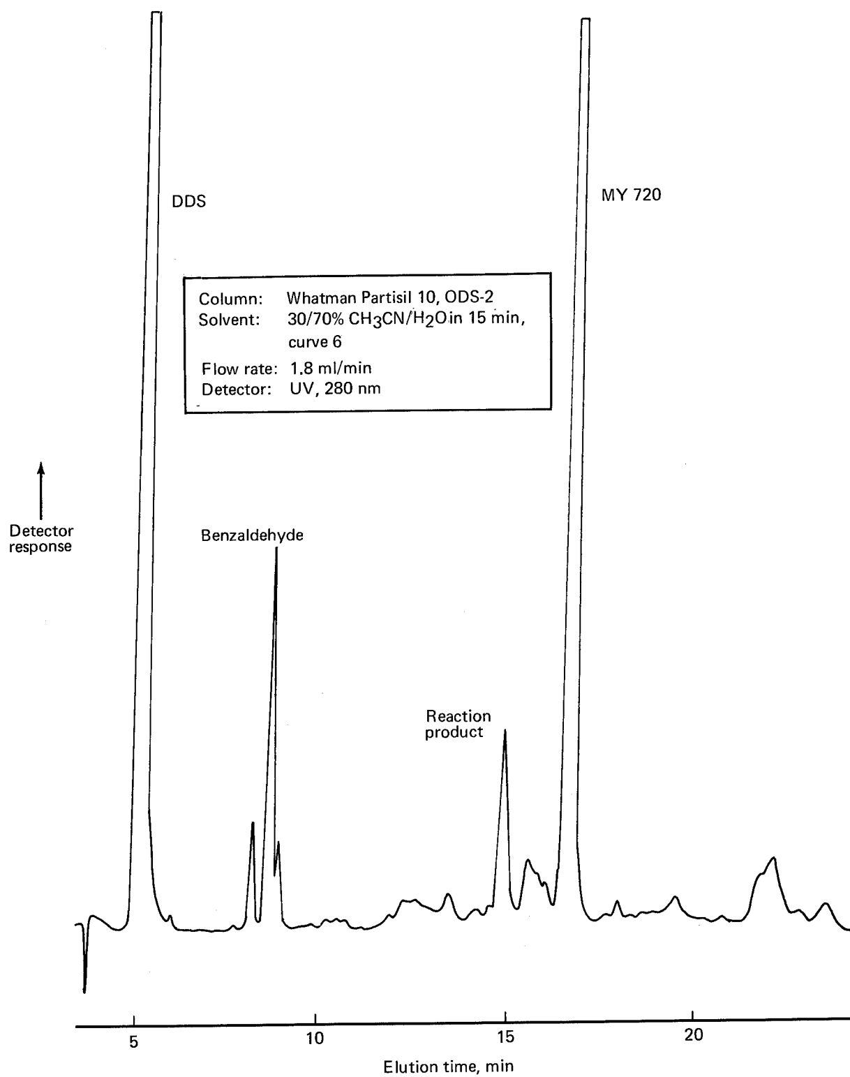
Figure 26. LC Chromatogram of Narmco Batch 286, Column: Whatman Partisil 10; ODS-2
