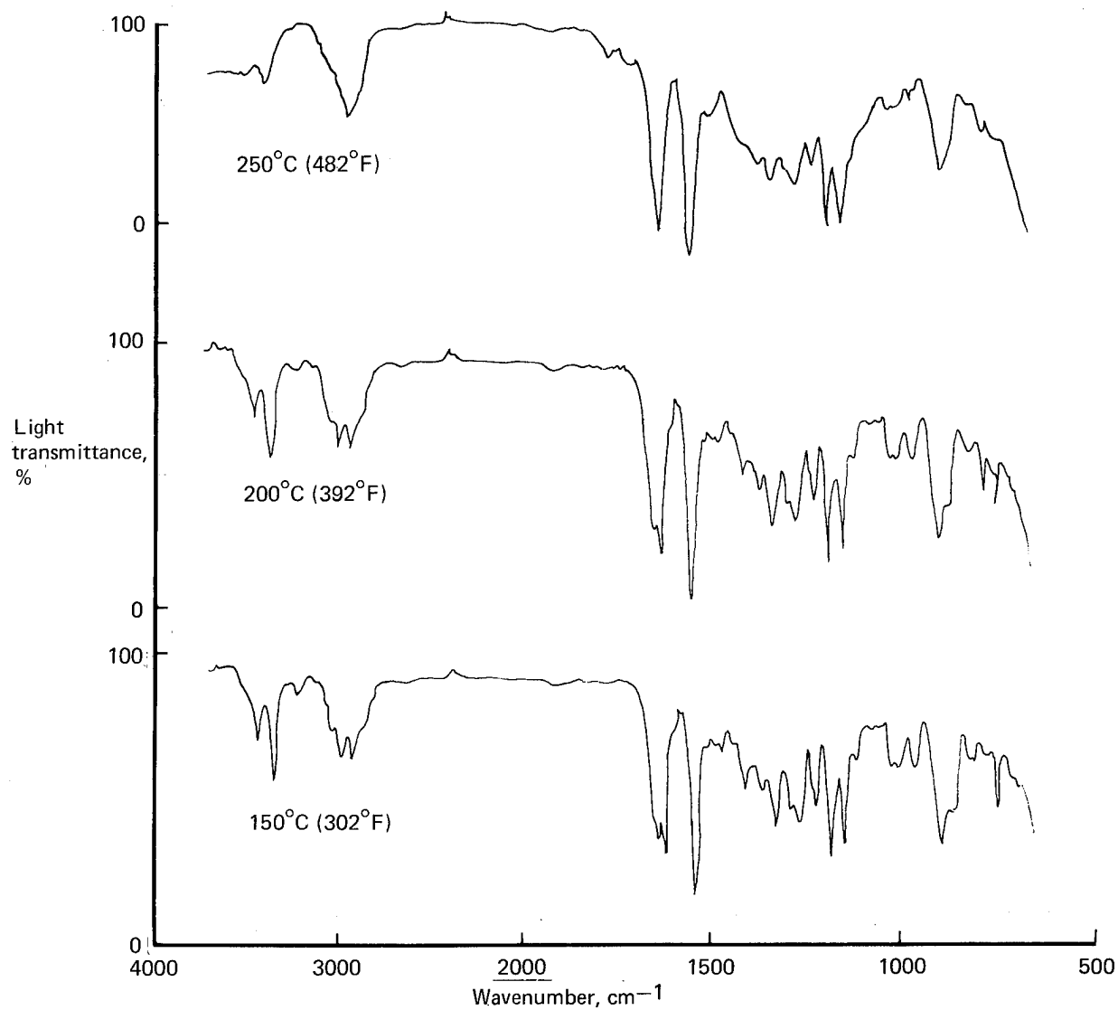
Figure 53. TSIR Spectra of Narmco Neat Resin Batch 300–150, 200, and 250°C (302, 392, and 482°F)
