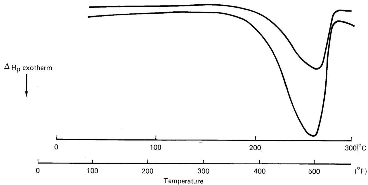
Figure 50. DSC Scan of Narmco Neat Resin Batch 300
