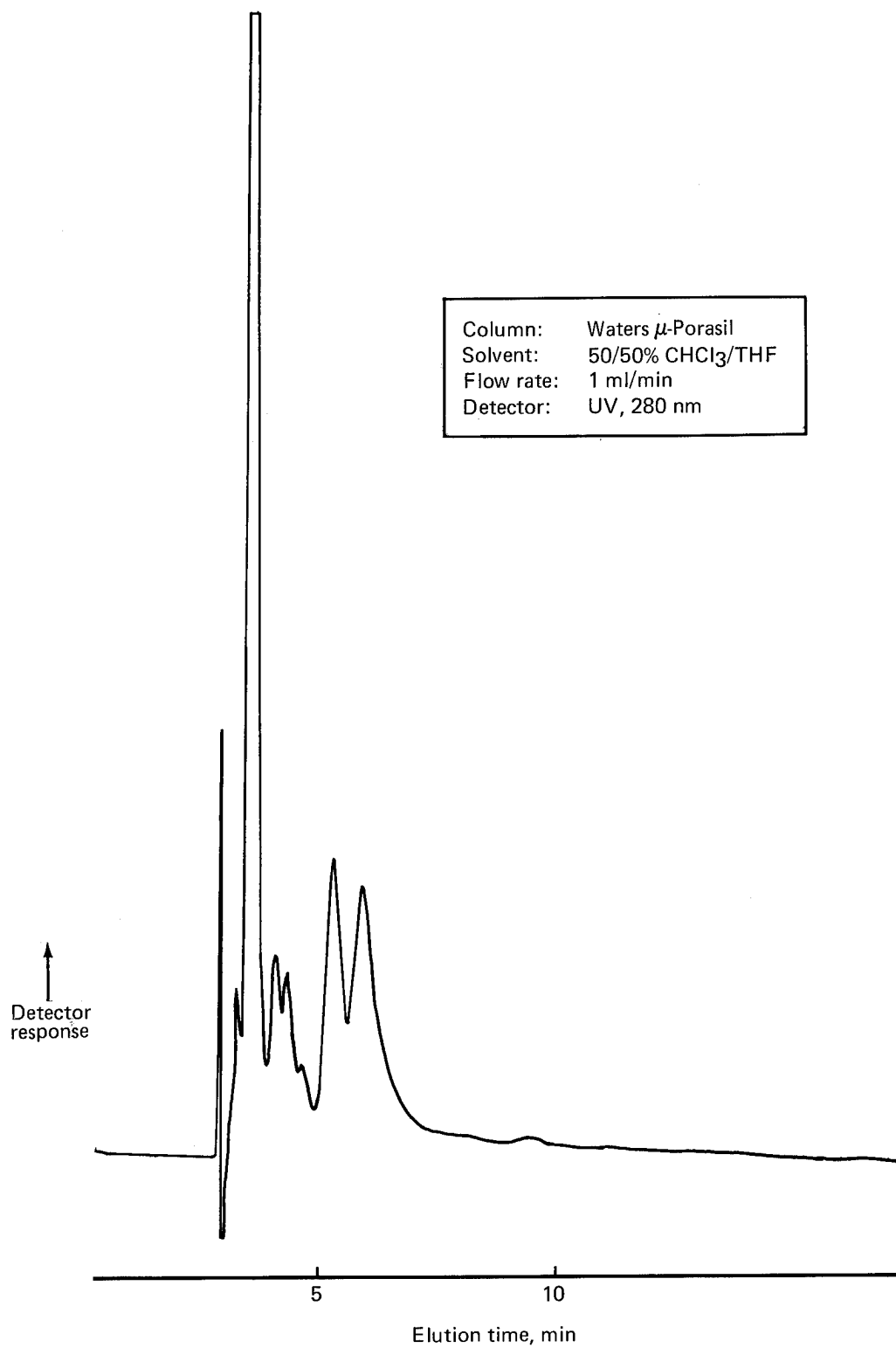
Figure 13. LC Chromatogram of MY 720
