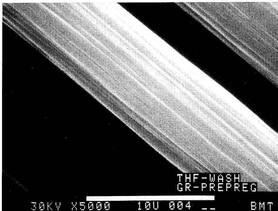
Figure 5. SEM Photomicrograph of Prepreg Fiber After THF Wash
