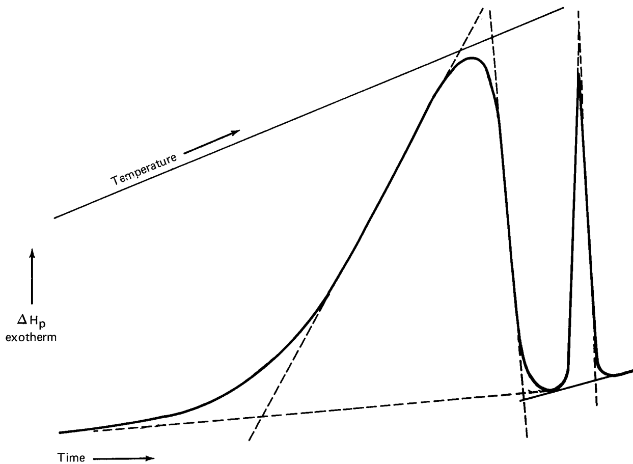
Figure 76. DSC Curve of Narmco Prepreg Batch 1072, Round-Robin Participant E
