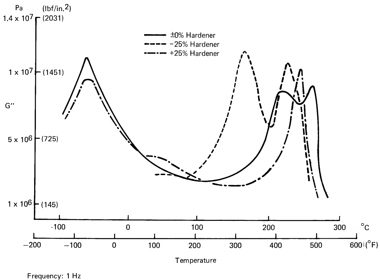
Figure 118. Viscous Modulus Versus Temperature, Narmco Matrix
