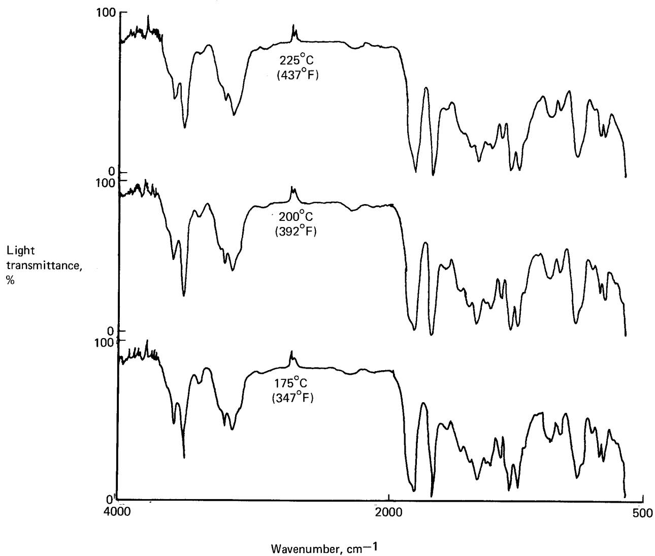
Figure 102. TSIR Spectra of Hercules Resin—175, 200, and 225°C (347, 392, and 437°F)
