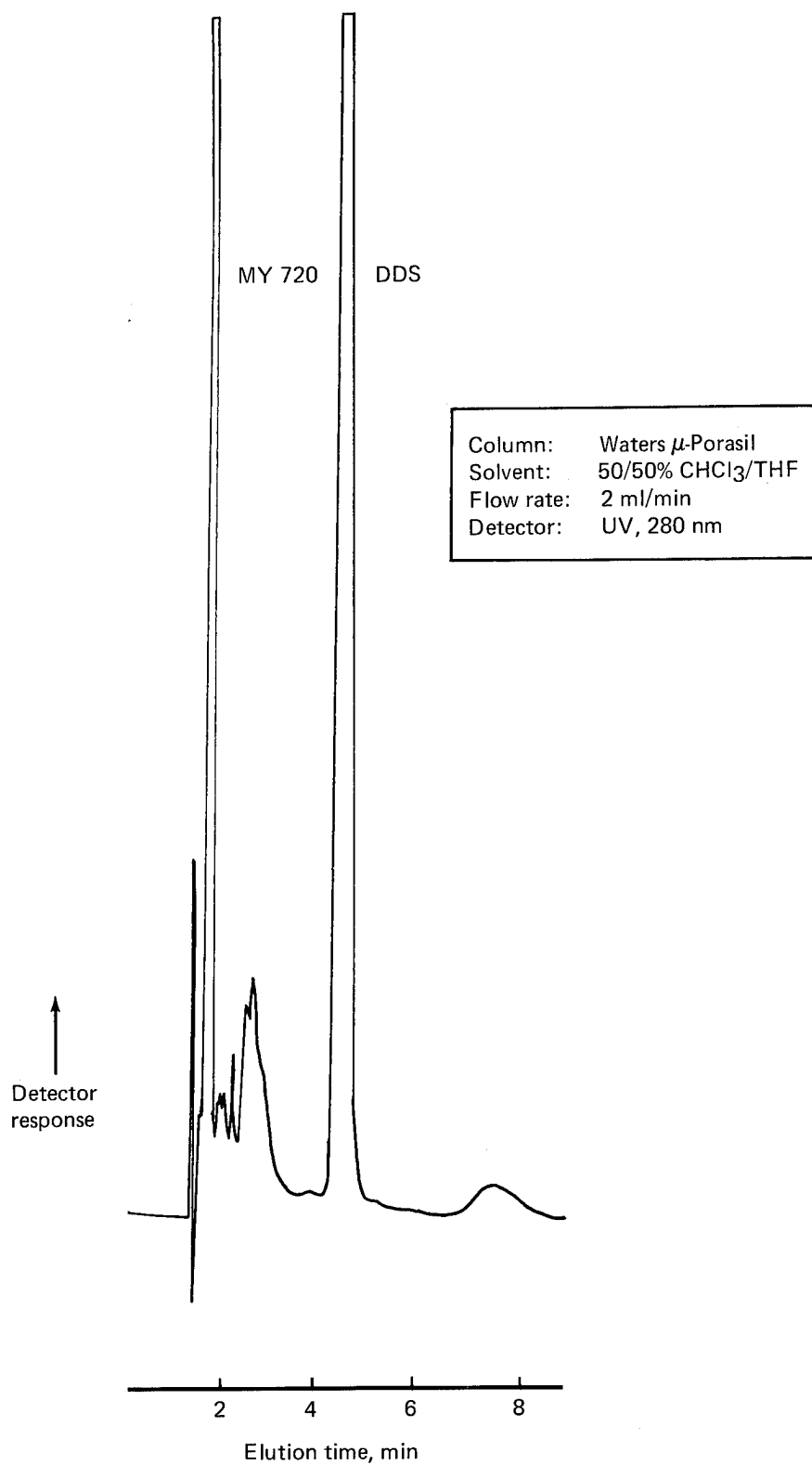
Figure 15. LC Chromatogram of Narmco Batch 286, Flow Rate: 2 ml/min
