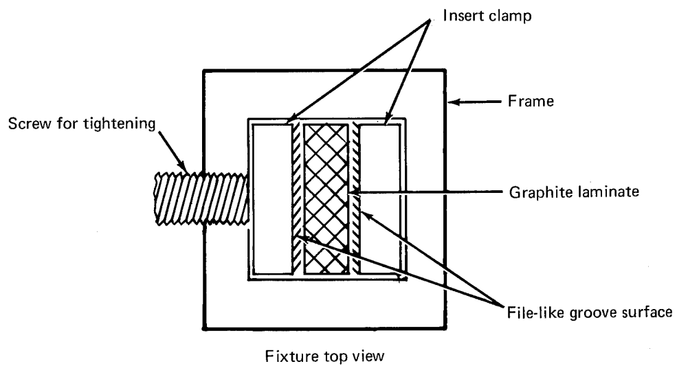
Figure 119. Fixture for DMA Testing of Epoxy Graphite Laminates
