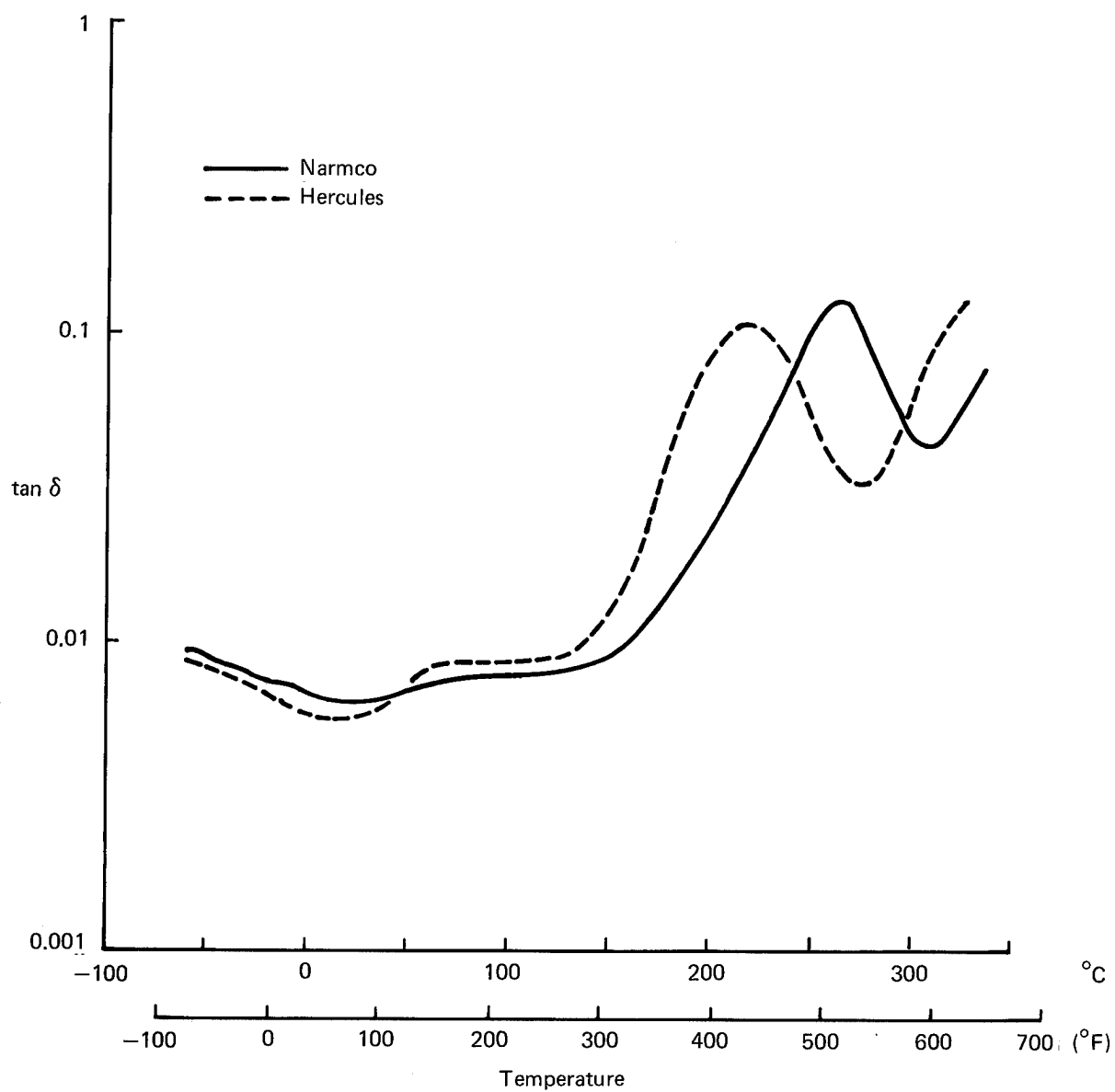
Figure 125. \tan \delta Versus Temperature, Narmco and Hercules Standard Batches
