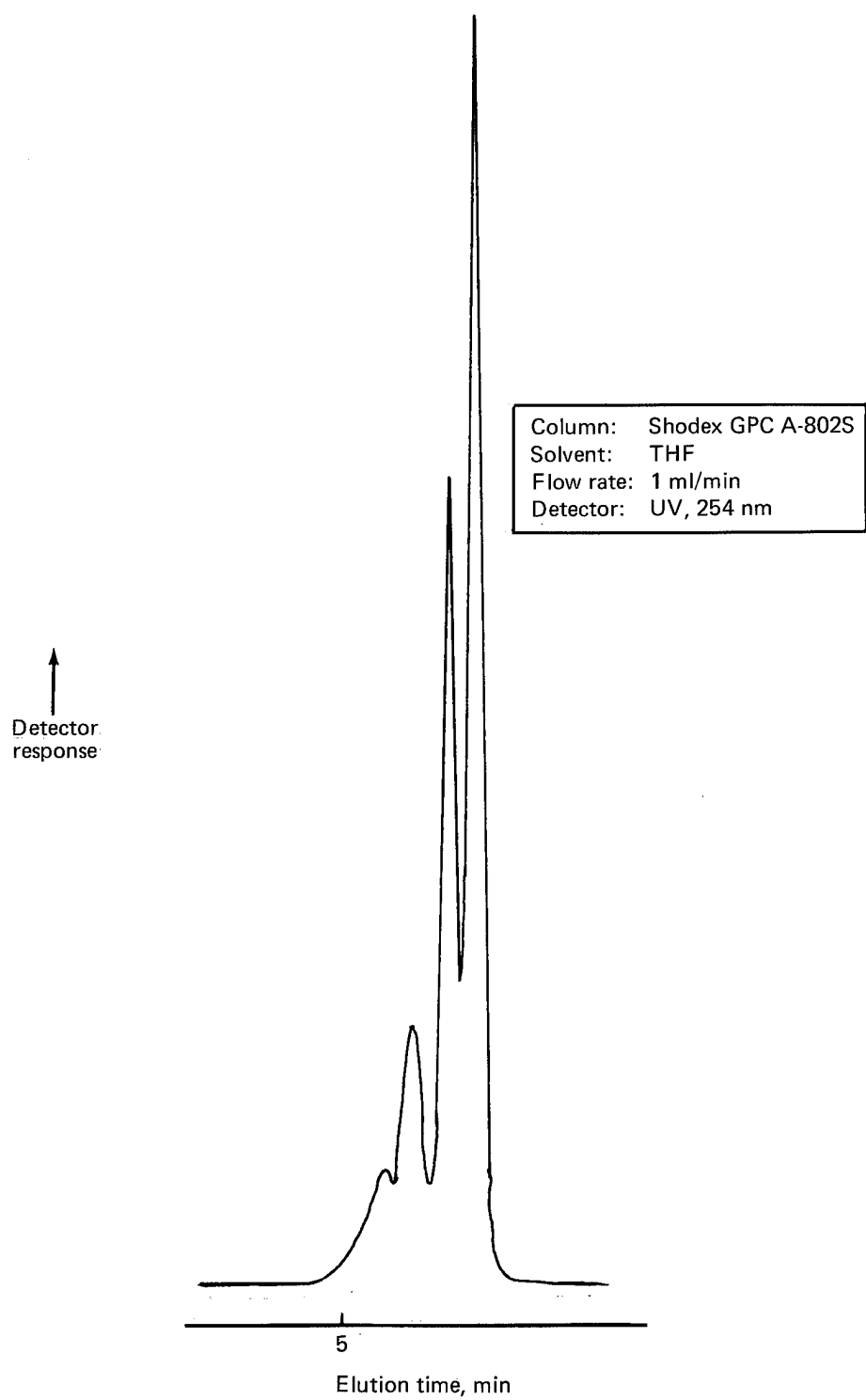
Figure 88. GPC Chromatogram of Narmco Neat Resin Batch 300, Flow Rate: 1 ml/min
