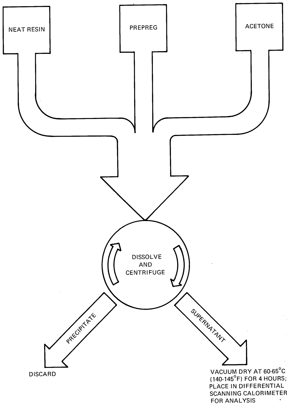
Figure 69. Optimized DSC Method Schematic
