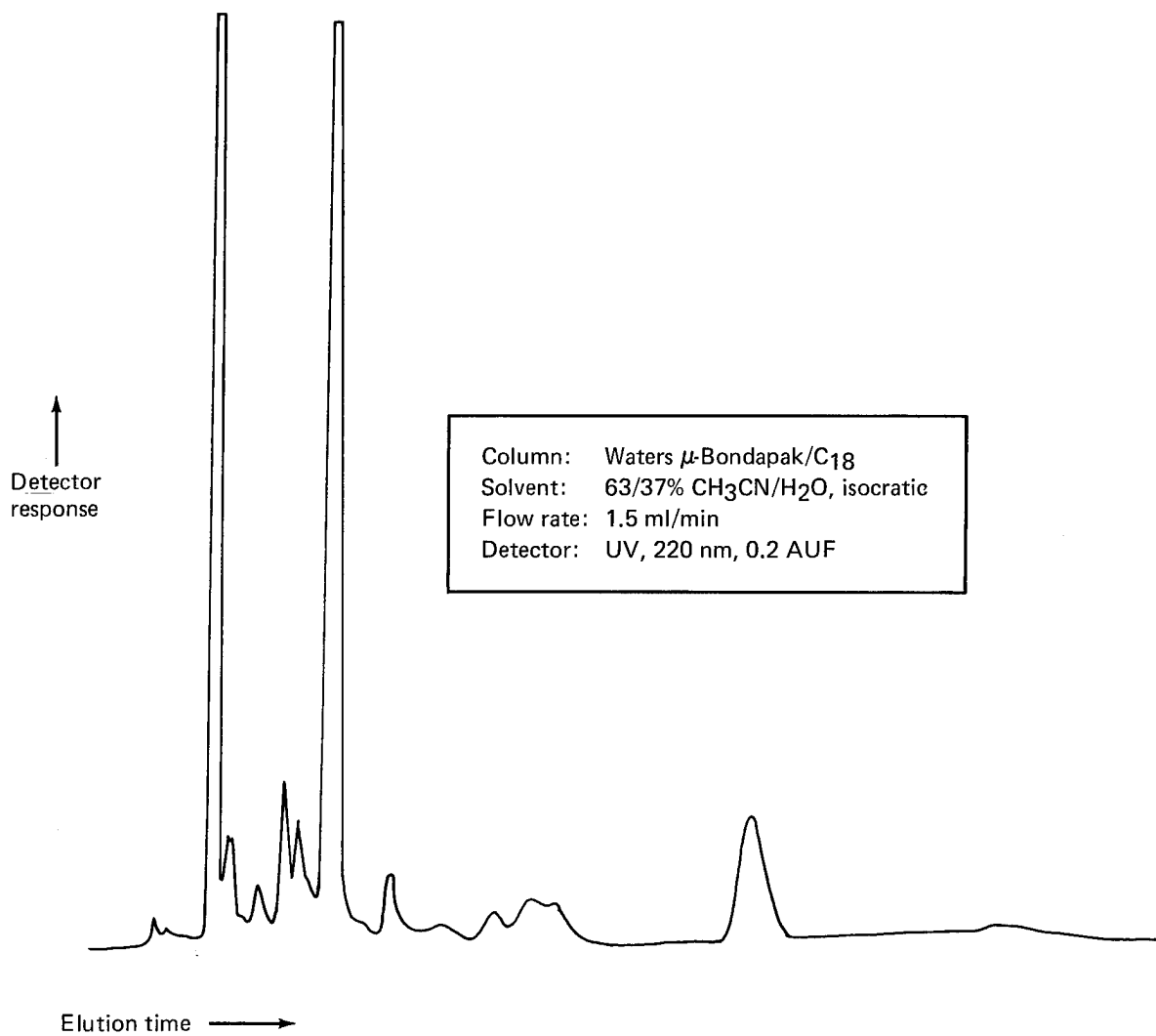
Figure 46. LC Chromatogram of Narmco Prepreg Batch 1072, Round-Robin Participant H
