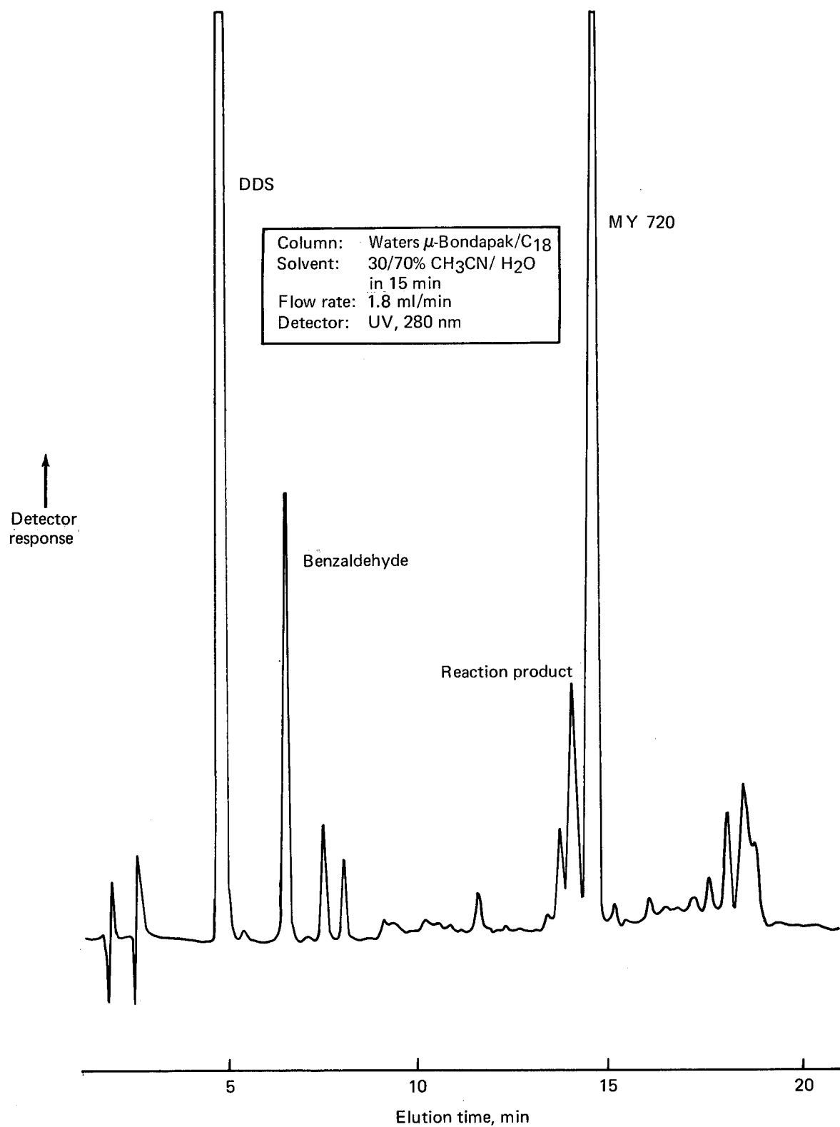
Figure 22. LC Chromatogram of Narmco Batch 286, Solvent: 30/70% CH 3 CN/H 2 O
