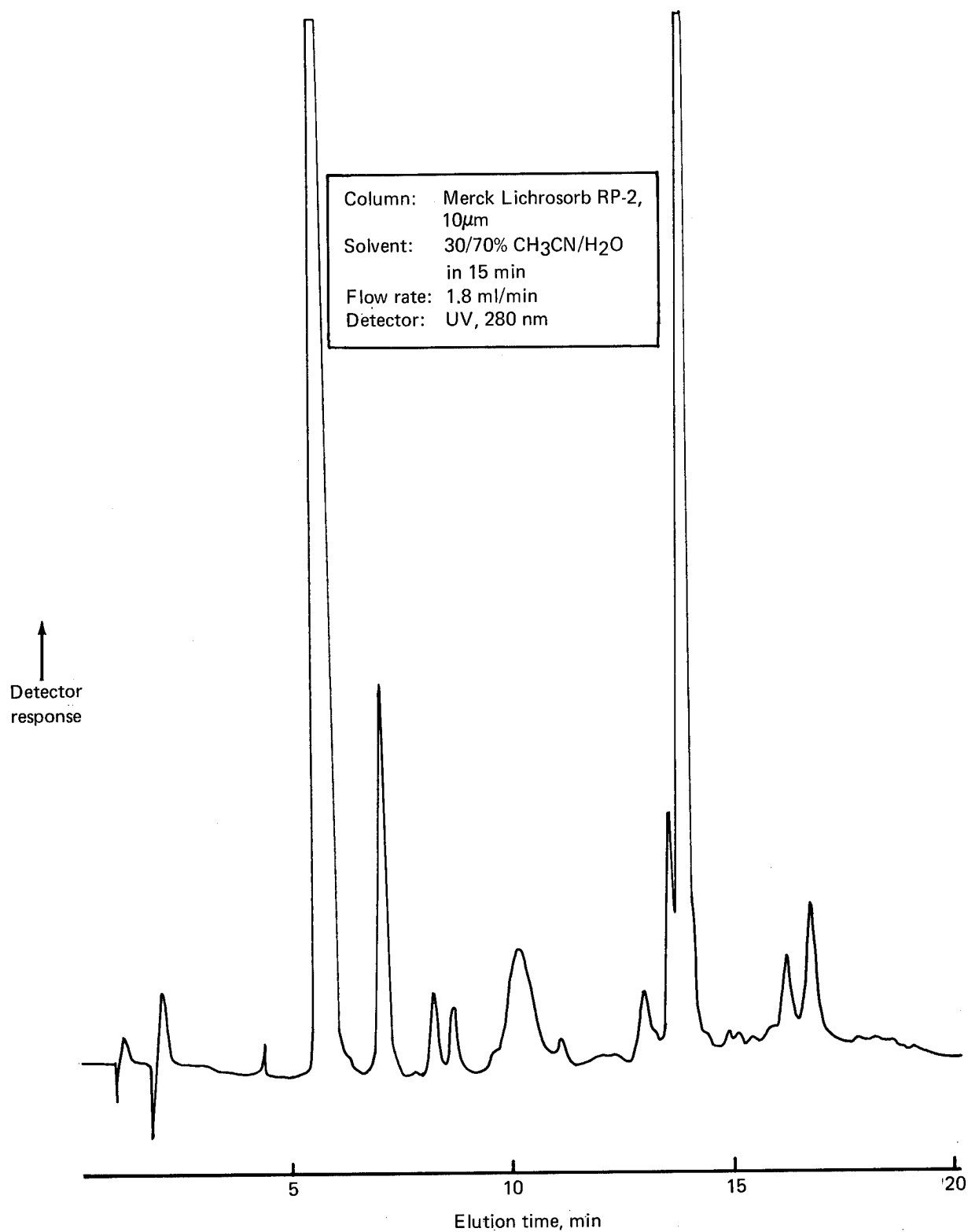
Figure 28. LC Chromatogram of Narmco Batch 286, Column: Merck Lichrosorb RP-2, 10 \mu m
