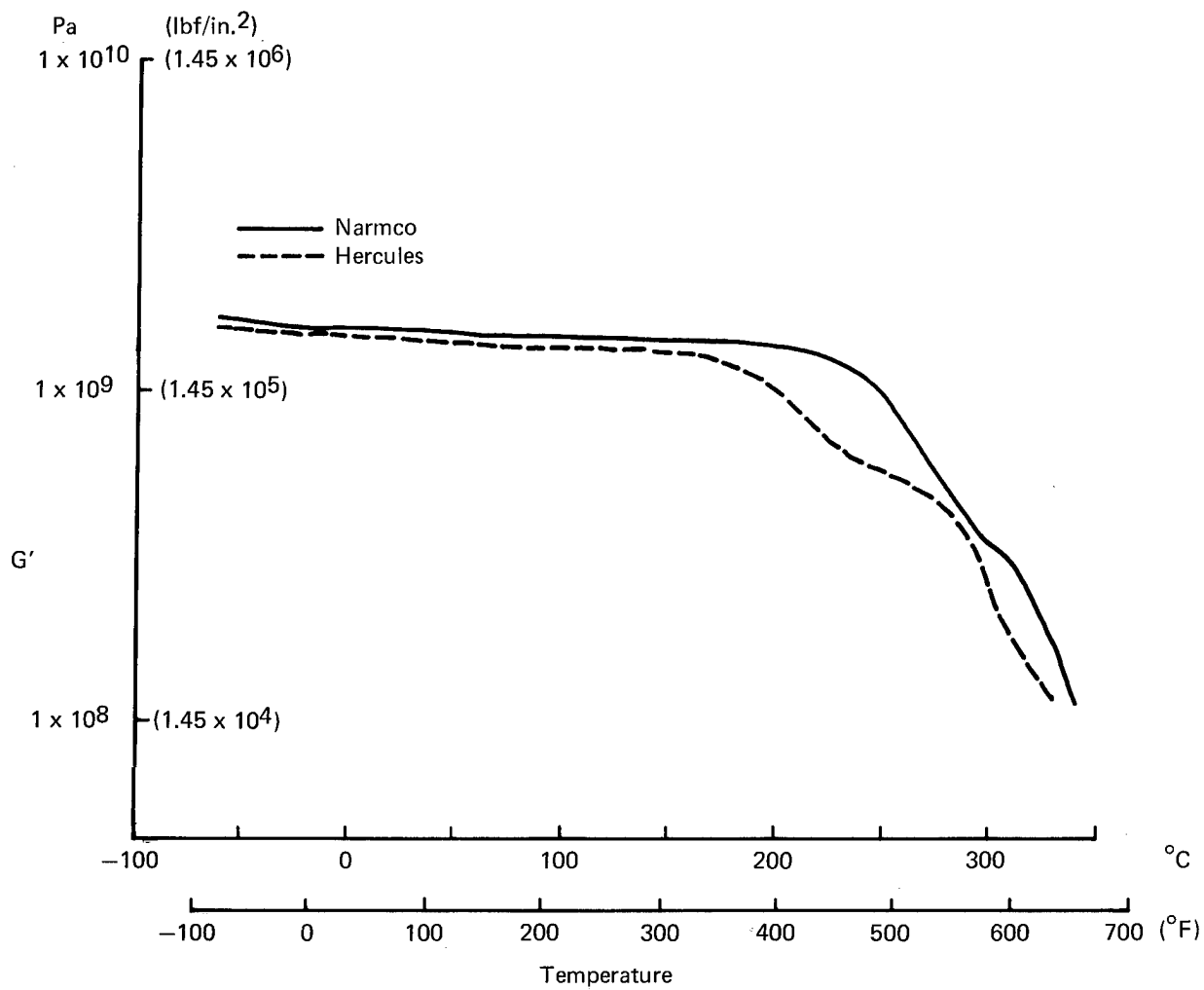
Figure 124. G' Versus Temperature, Narmco and Hercules Standard Batches
