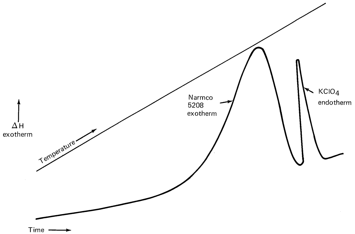
Figure A-2. Example DSC Curve—Resin and KClO 4 Standard
