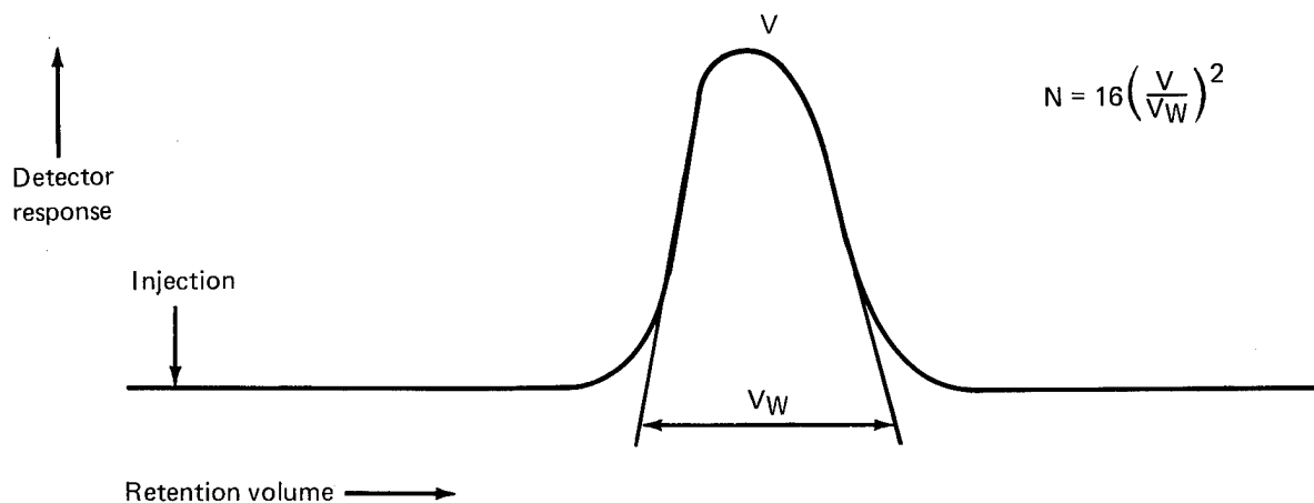
Figure A-4. Example GPC Chromatogram for Column Calibration
