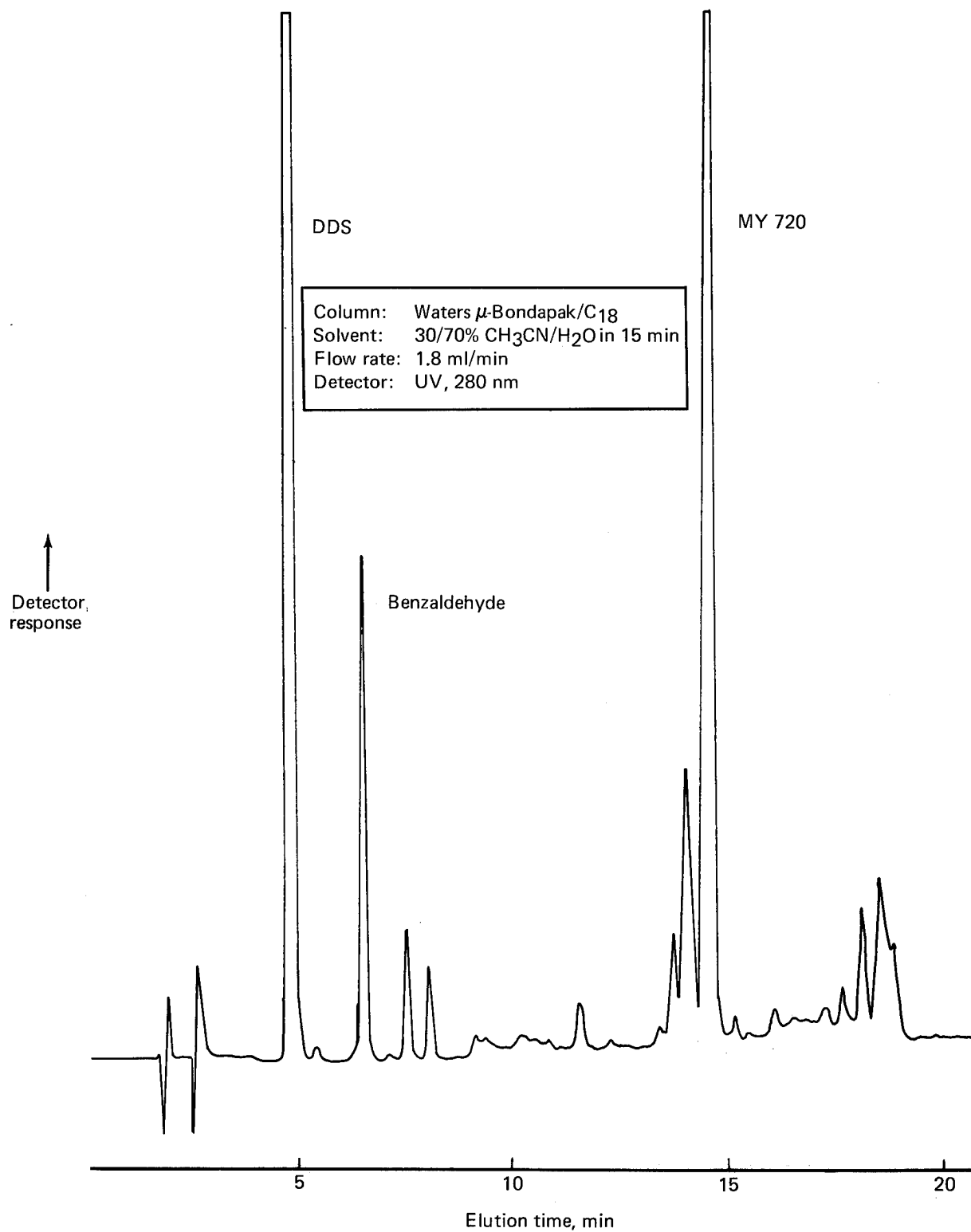
Figure 24. LC Chromatogram of Narmco Batch 286, Column: Waters \mu -Bondapak/C18
