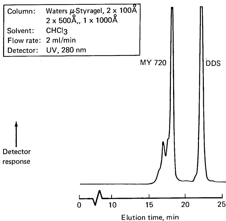
Figure 85. GPC Chromatogram of Narmco Neat Resin Batch 300, Solvent: \text{CHCl}_3 , Column: Waters \mu -Styragel—2 x 100Å, 2 x 500Å, 1 x 1000Å
