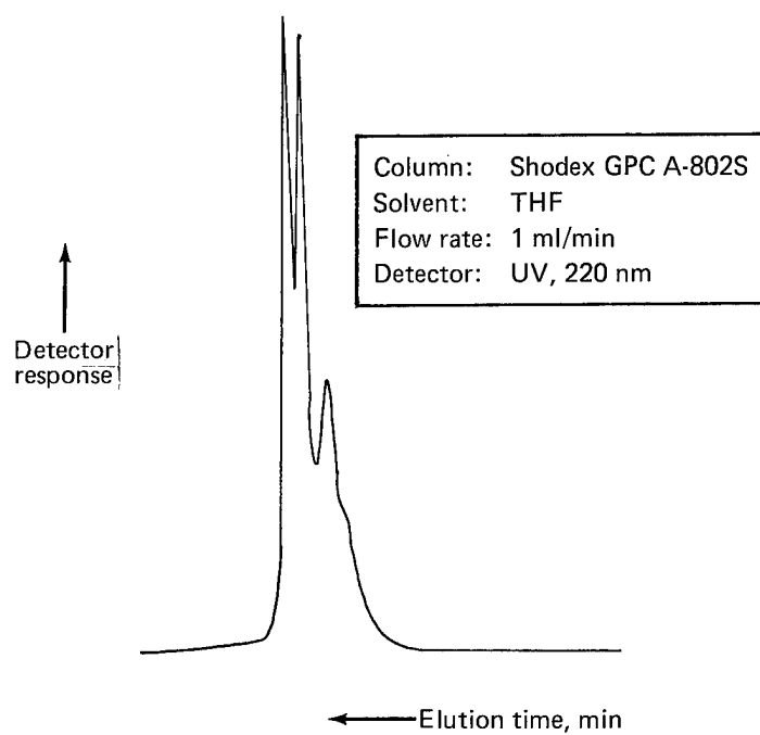
Figure 96. GPC Chromatogram of Narmco Prepreg Batch 1072, Round-Robin Participant F
