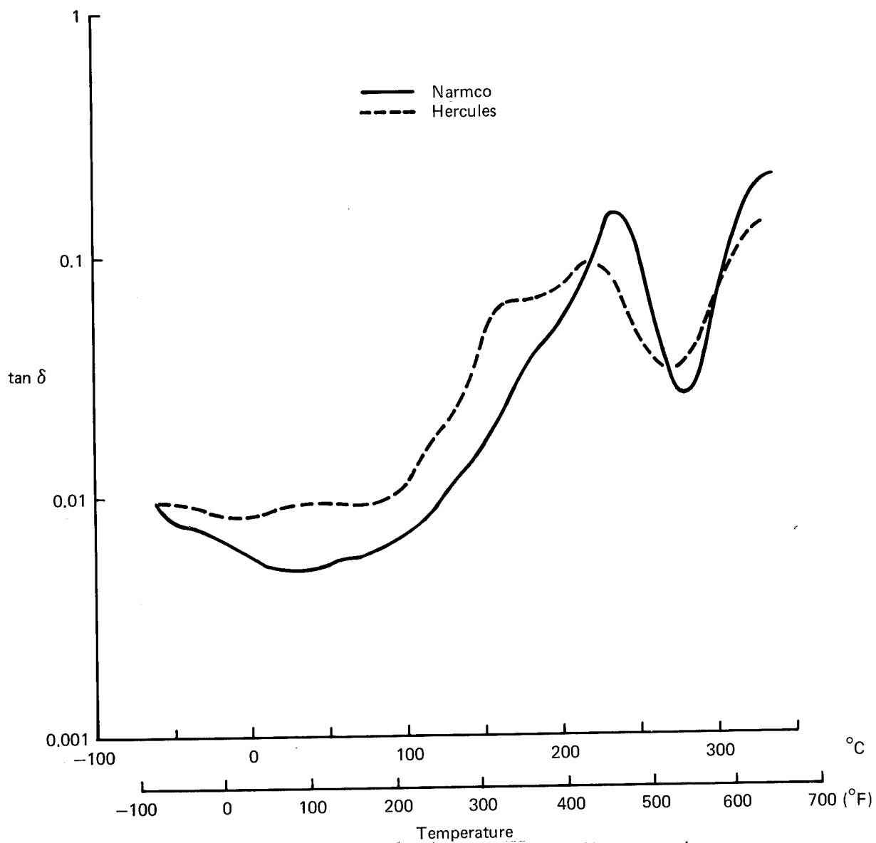
Figure 129. \tan \delta Versus Temperature, Narmco and Hercules Standard Batches, Humidity Exposed
