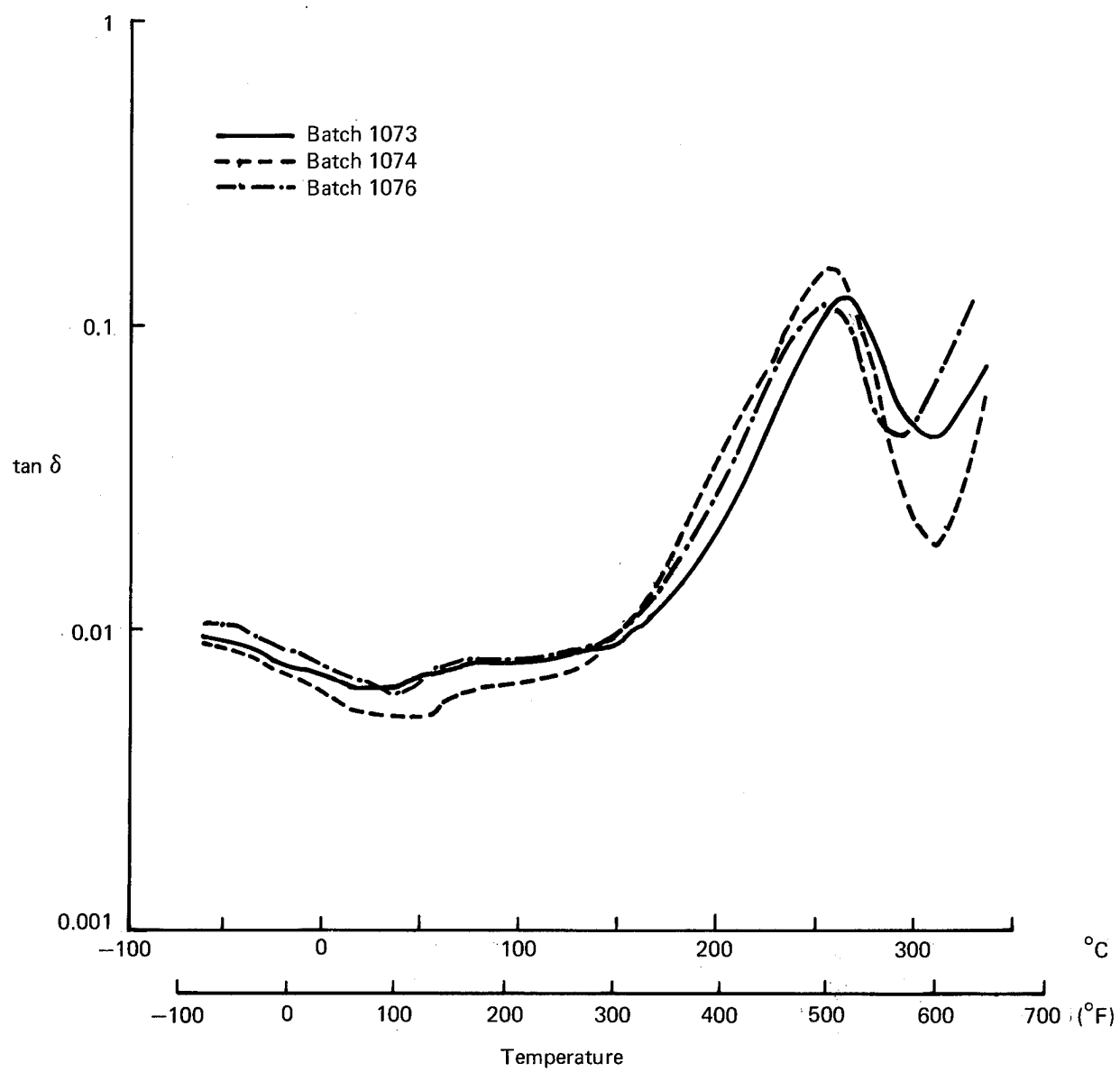
Figure 121. \tan \delta Versus Temperature, Narmco Laminates
