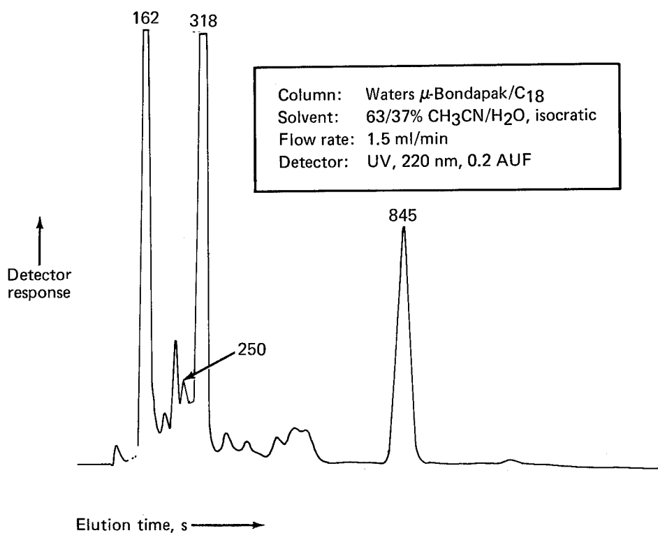
Figure 41. LC Chromatogram of Narmco Prepreg Batch 1072, Round-Robin Participant B
