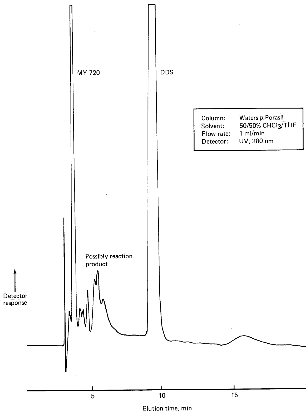
Figure 14. LC Chromatogram of Narmco Batch 286, Flow Rate: 1 ml/min
