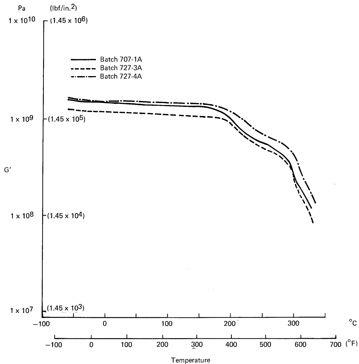
Figure 122. G' Versus Temperature, Hercules Laminates
