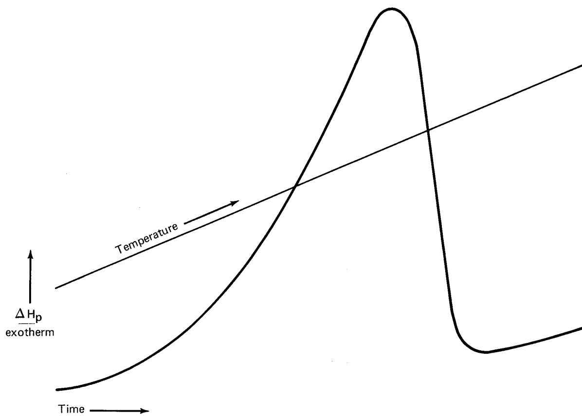
Figure 81. DSC Curve of Narmco Prepreg Batch 1072, Round-Robin Participant J
