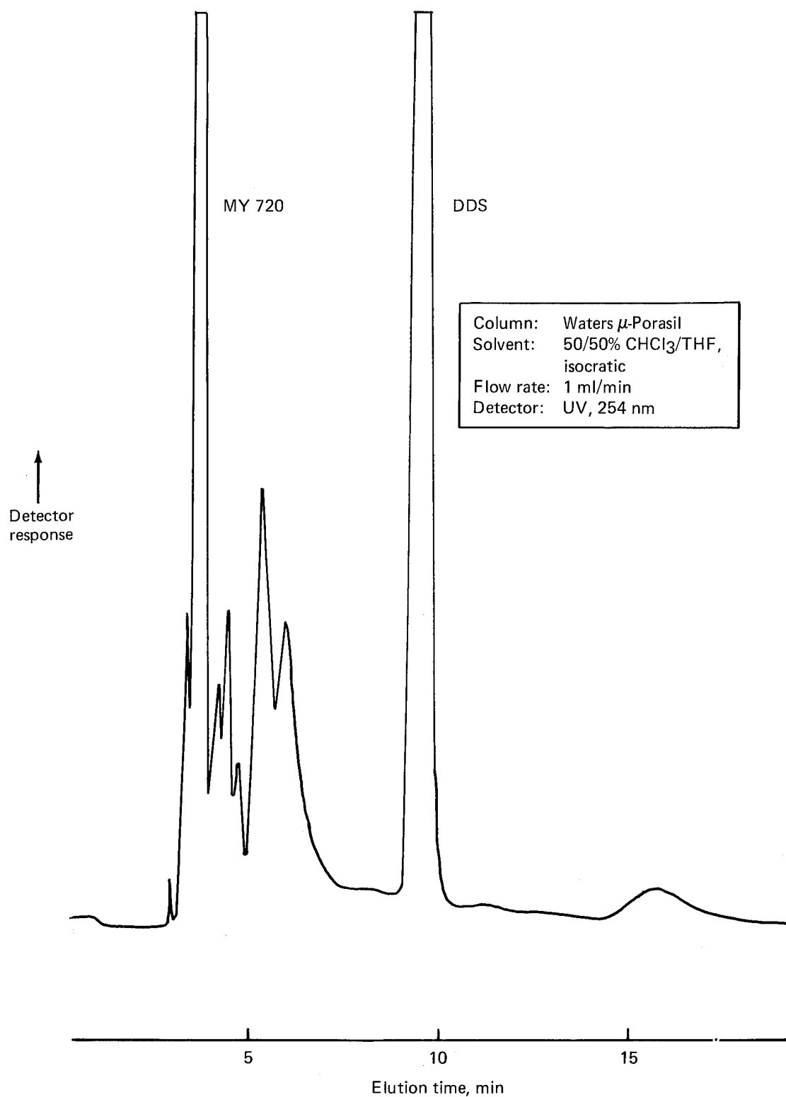
Figure 17. LC Chromatogram of Narmco Batch 286, Detector: UV, 254 nm
