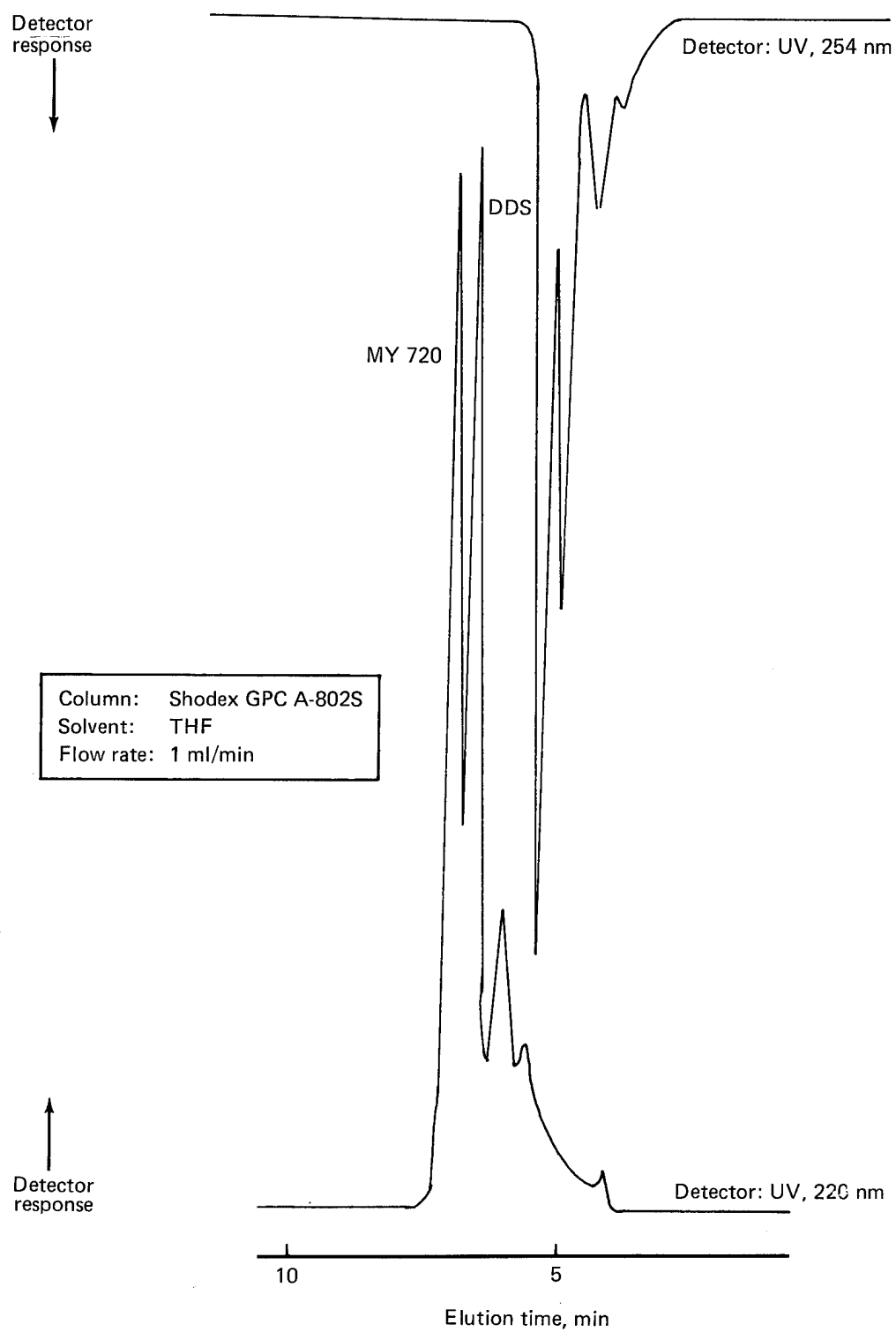
Figure 89. GPC Chromatogram of Narmco Neat Resin Batch 300, Detector: UV, 220 nm
