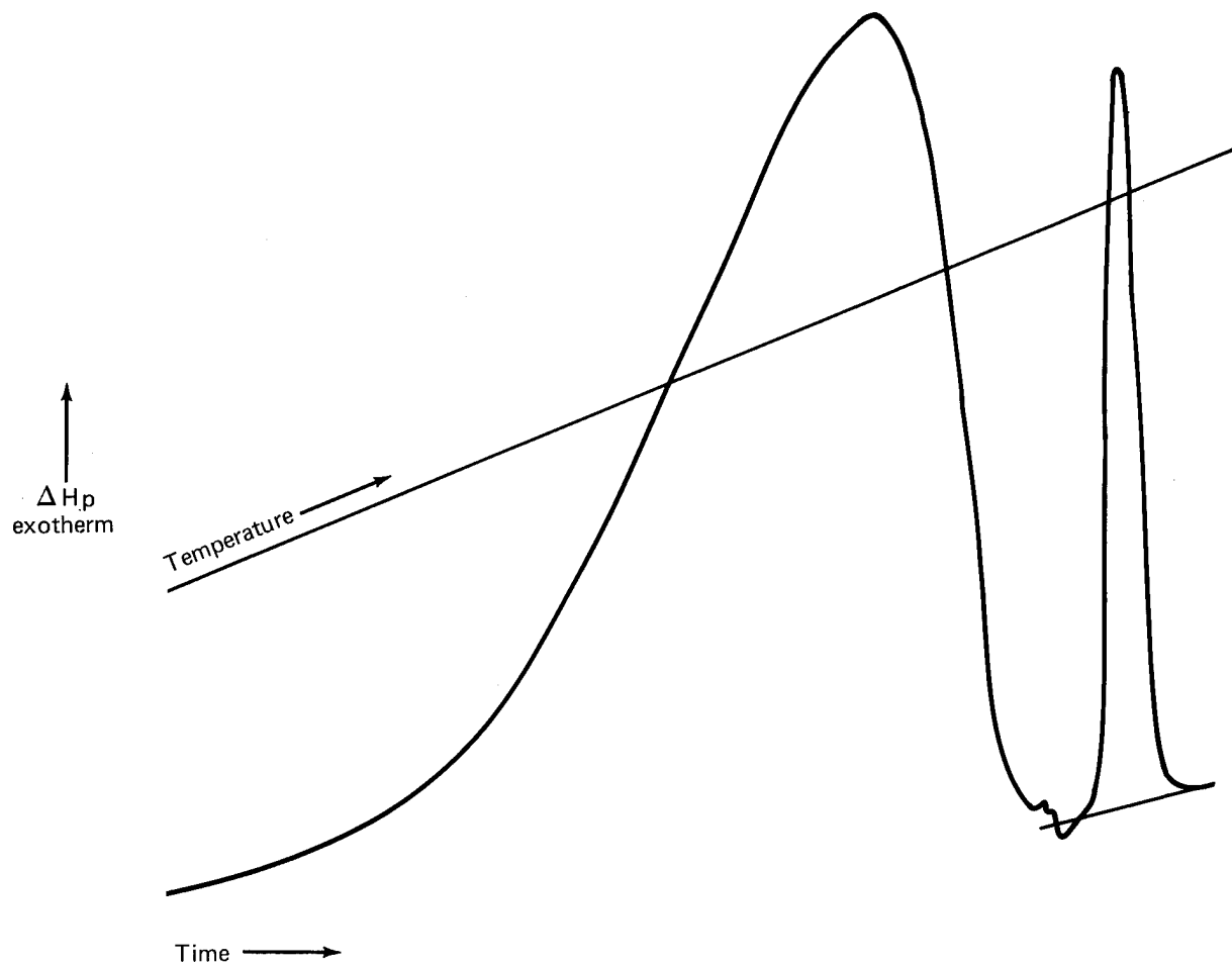
Figure 72. DSC Curve of Narmco Prepreg Batch 1072, Round-Robin Participant A
