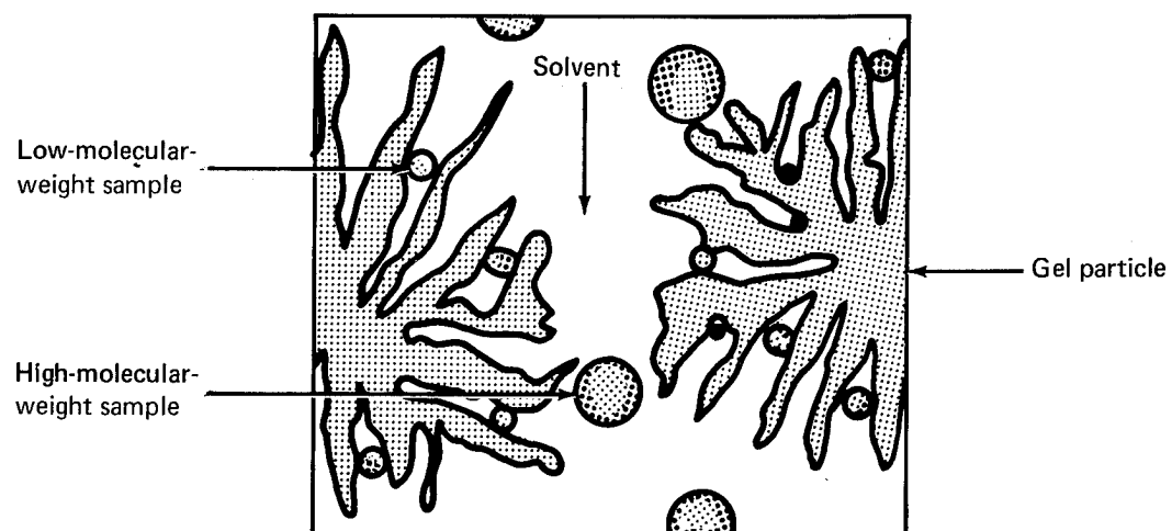
Figure 82. Diagram of GPC Technique
