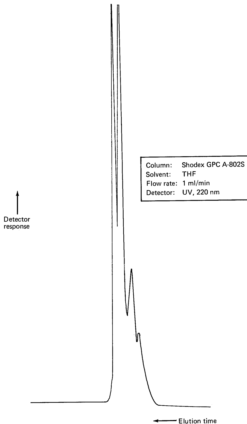
Figure 110. GPC Chromatogram of Hercules Batch 707-1A, Using GPC Round-Robin Procedure
