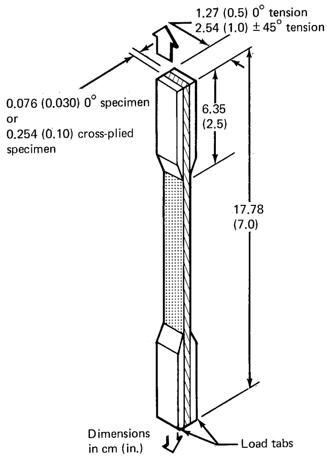
Figure 3. Tension Test Specimen
