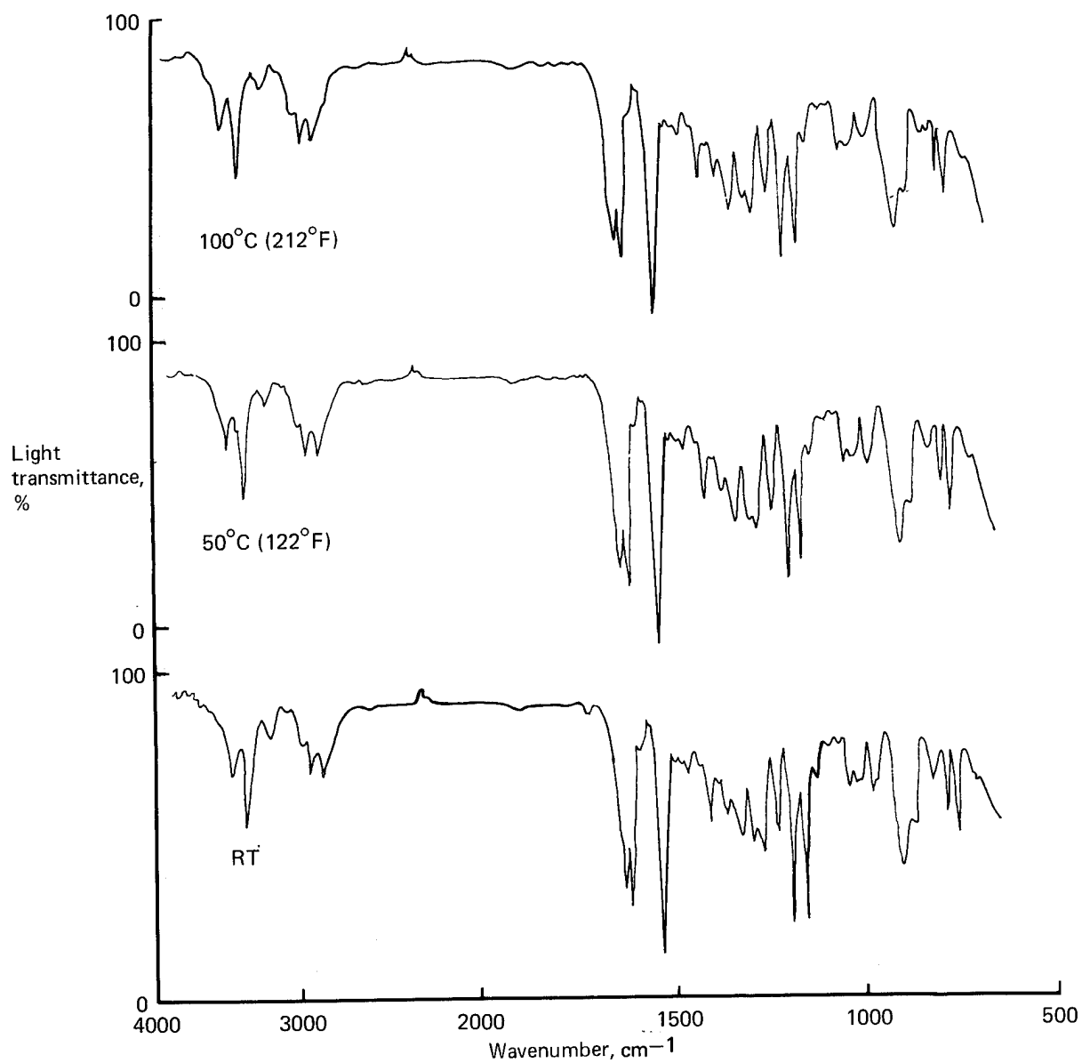
Figure 52. TSIR Spectra of Narmco Neat Resin Batch 300—RT, 50°C, and 100°C (RT, 122°F, and 212°F)
