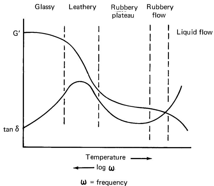
Figure 115. Typical Dynamic Mechanical Response
