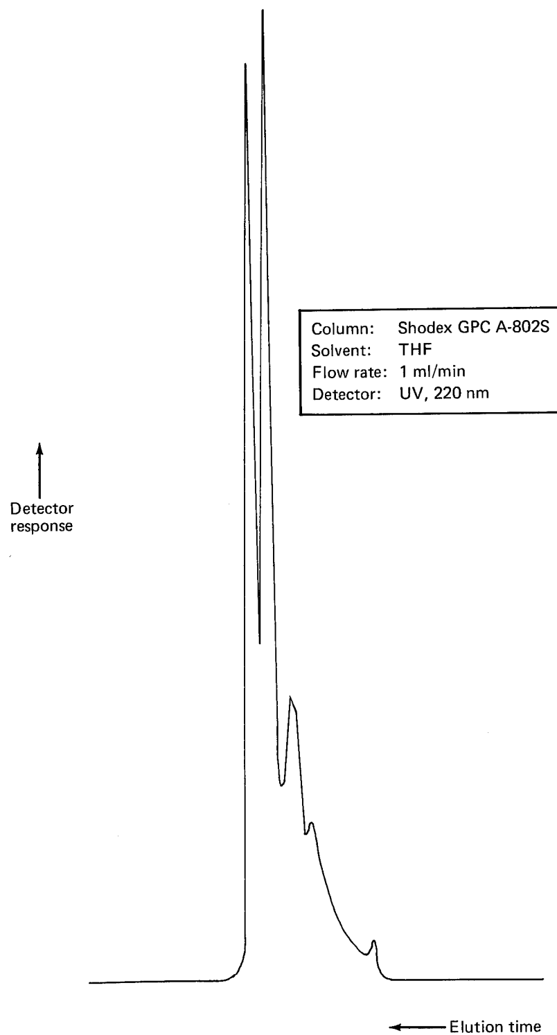
Figure 98. GPC Chromatogram of Narmco Prepreg Batch 1072, Round-Robin Participant I
