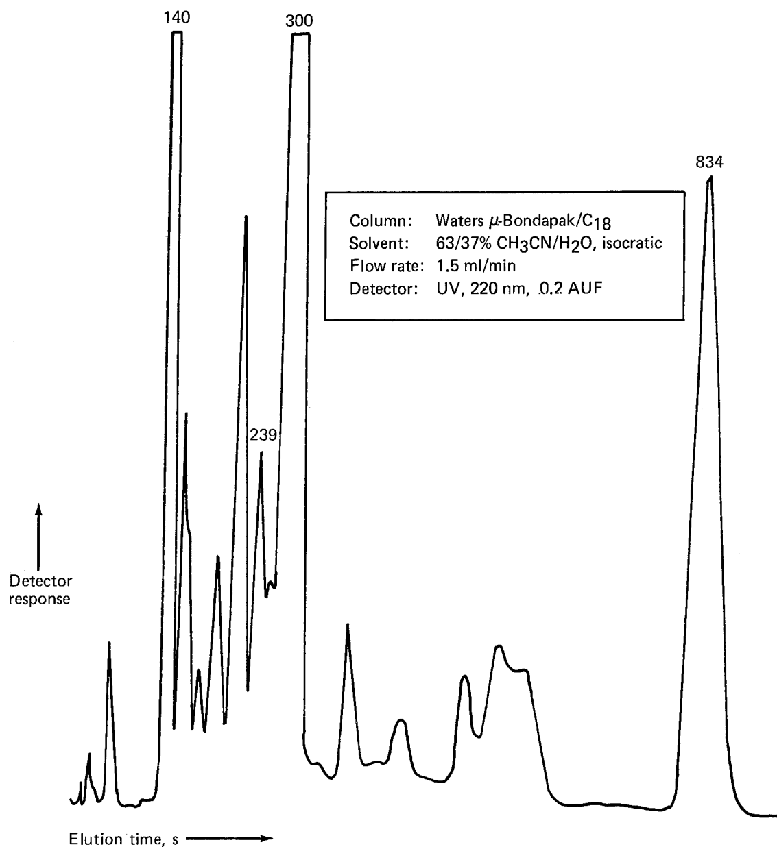
Figure 48. LC Chromatogram of Narmco Prepreg Batch 1072, Round-Robin Participant J
