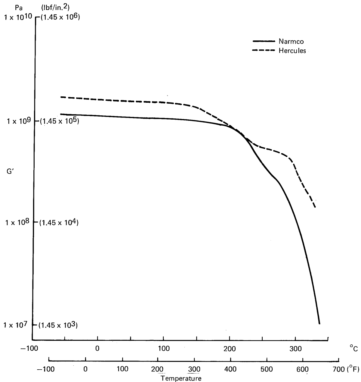
Figure 128. G' Versus Temperature, Narmco and Hercules Standard Batches, Humidity Exposed
