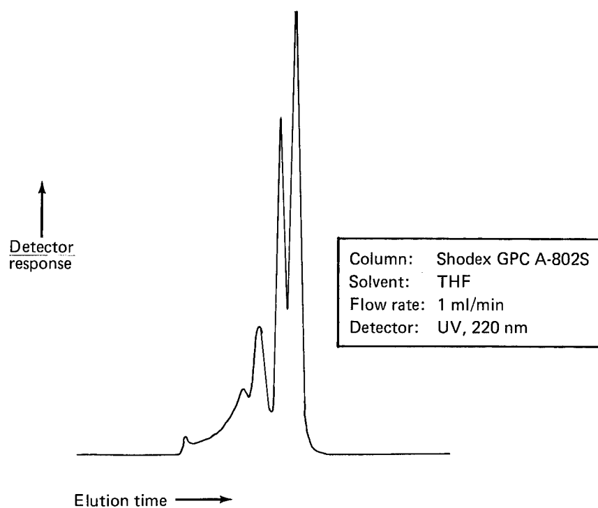
Figure 94. GPC Chromatogram of Narmco Prepreg Batch 1072, Round-Robin Participant D
