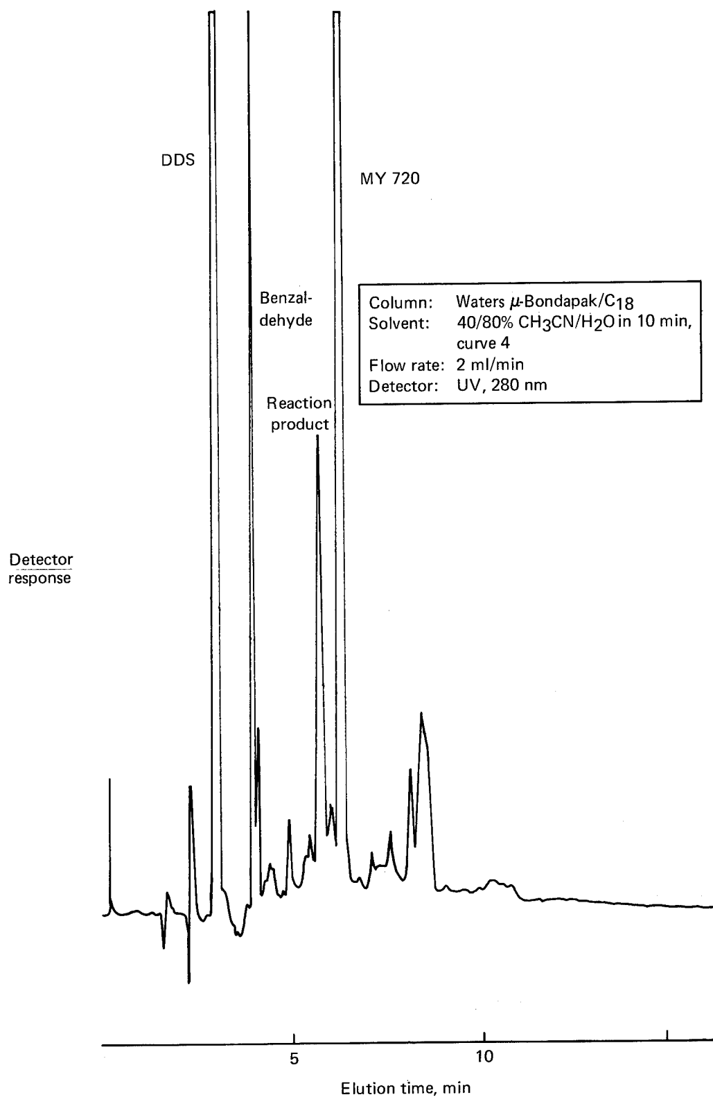
Figure 23. LC Chromatogram of Narmco Batch 286, Solvent: 40/80% CH 3 CN/H 2 O
