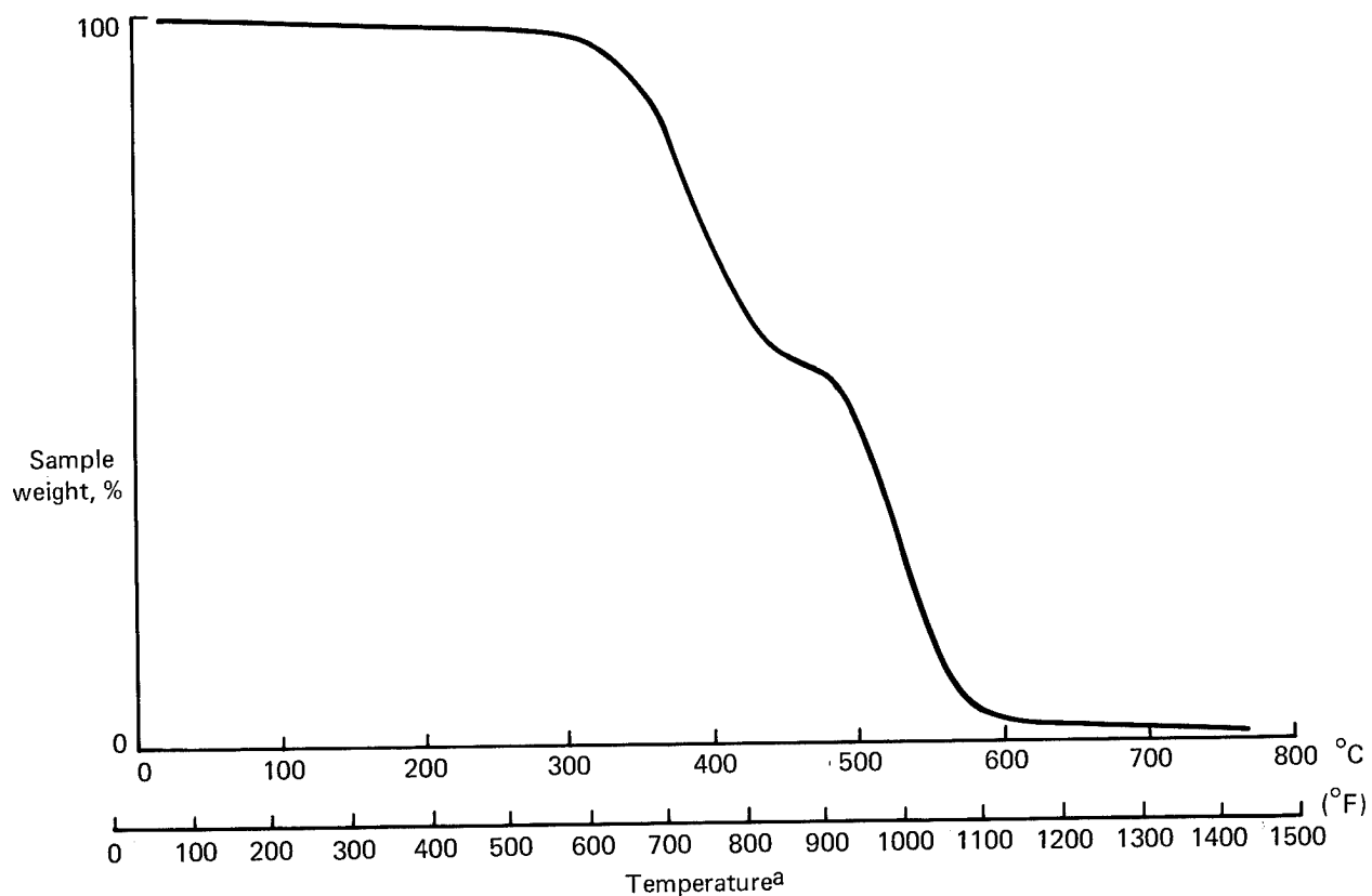
Figure 106. TGA Scan of Hercules Resin
