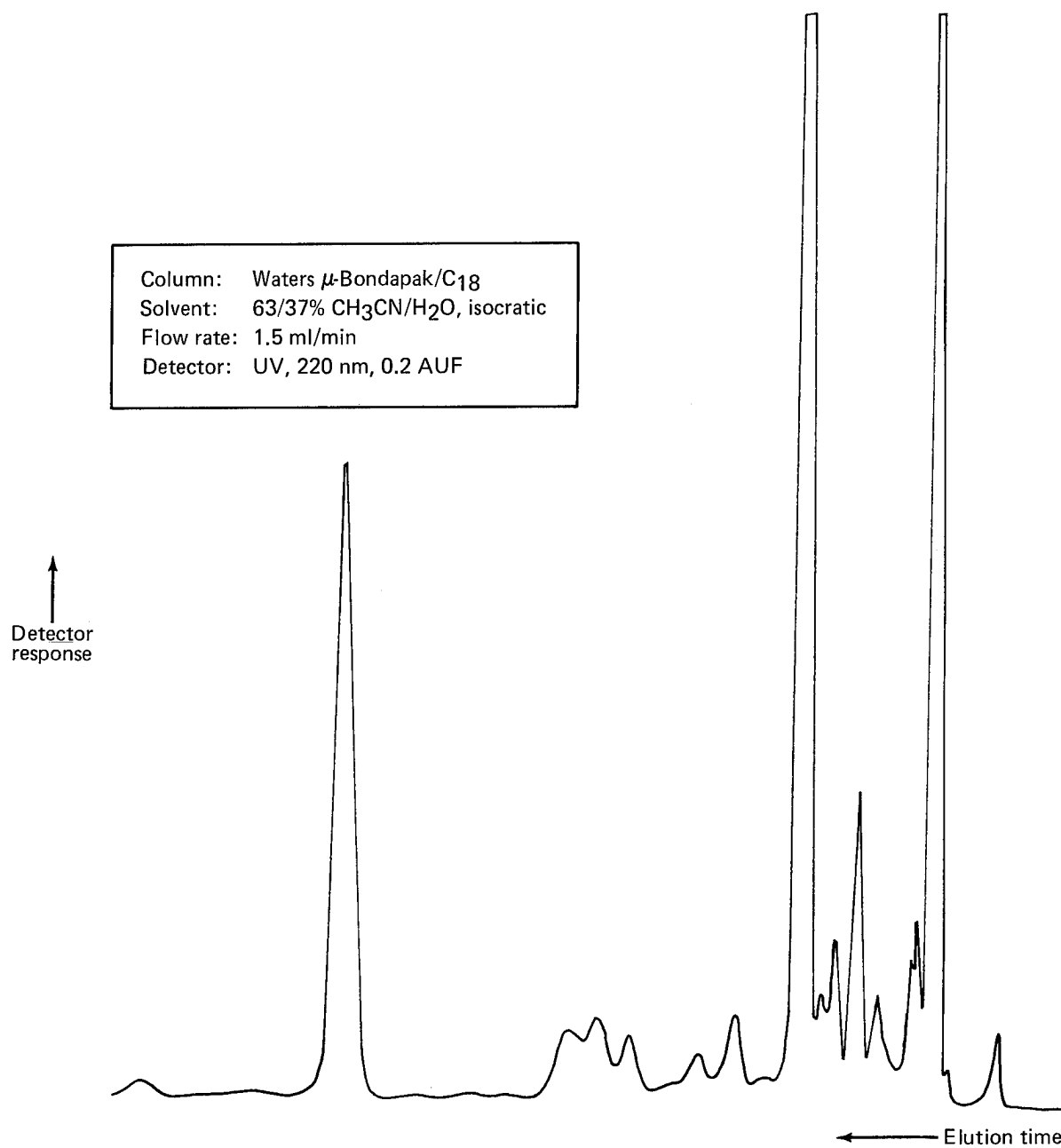
Figure 40. LC Chromatogram of Narmco Prepreg Batch 1072, Round-Robin Participant A
