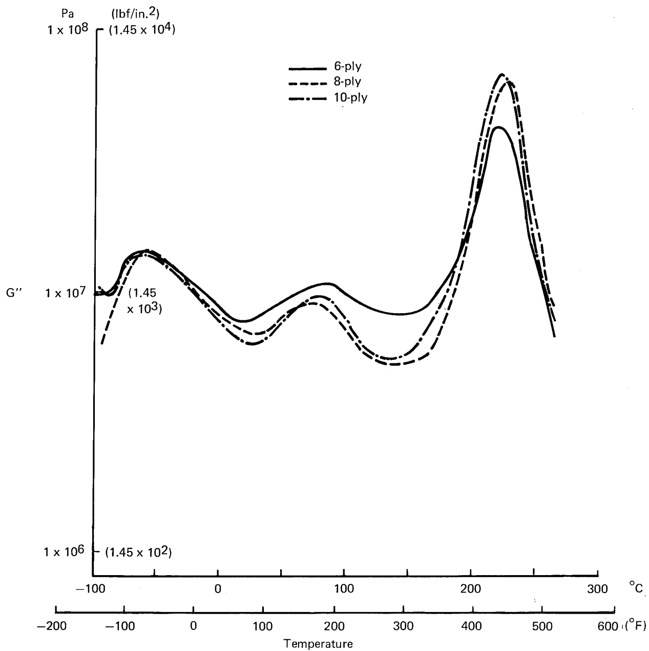
Figure 130. G'' Versus Temperature, Hercules Laminates—6, 8, and 10 Plies
