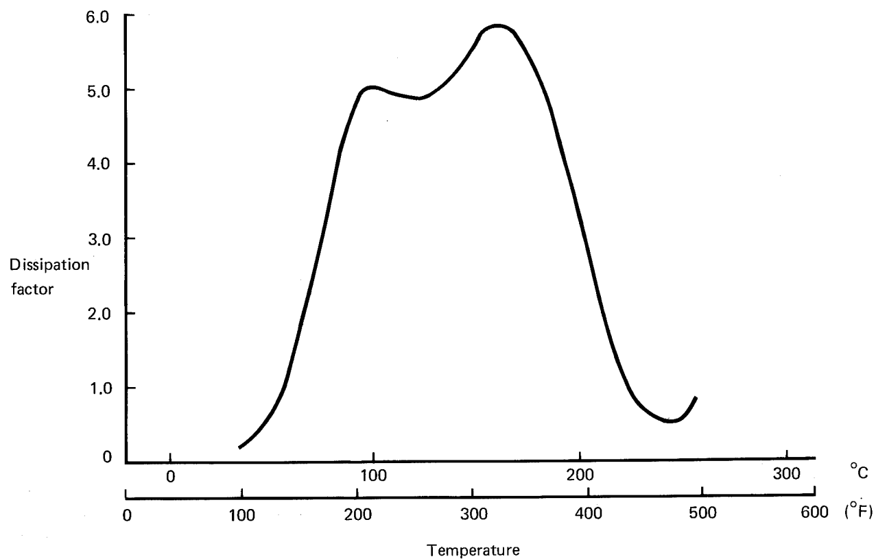
Figure 57. Results of Dielectric Analysis of Narmco Resin Batch 298
