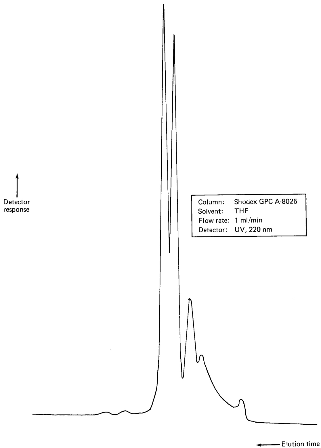
Figure 92. GPC Chromatogram of Narmco Prepreg Batch 1072, Round-Robin Participant A
