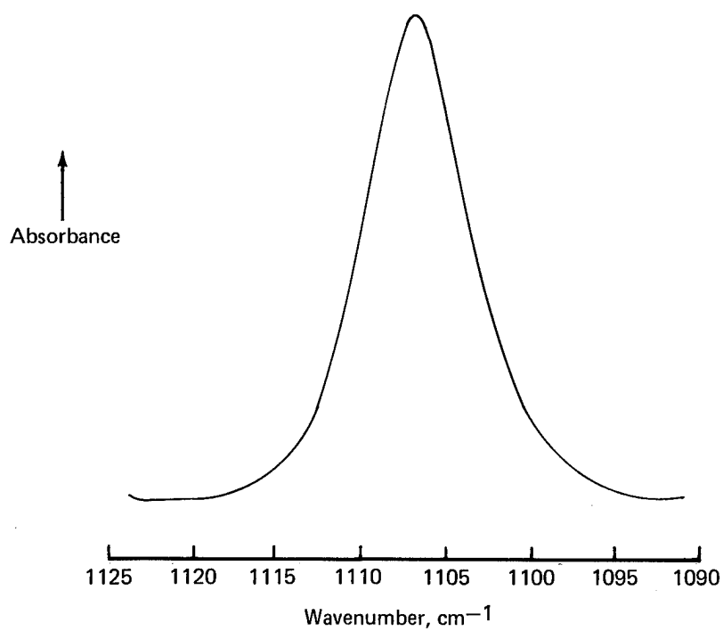
Figure 39. Determination of DDS Concentration by FTIR
