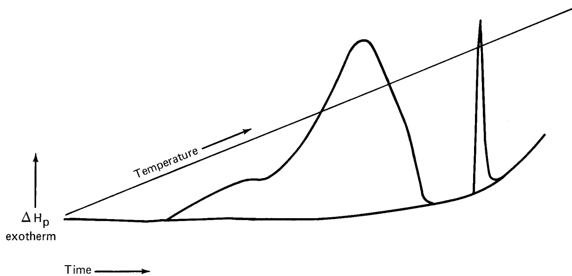
Figure 108. DSC Curve of Hercules Resin Batch 727-3A
