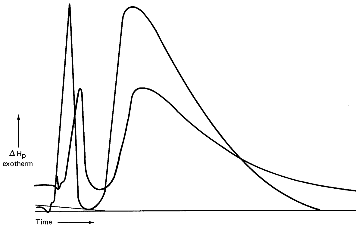
Figure 75. DSC Curve of Narmco Prepreg Batch 1072, Round-Robin Participant D
