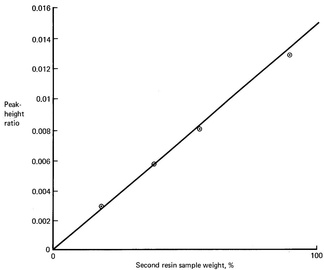
Figure 38. Calibration Curve of Second Resin
