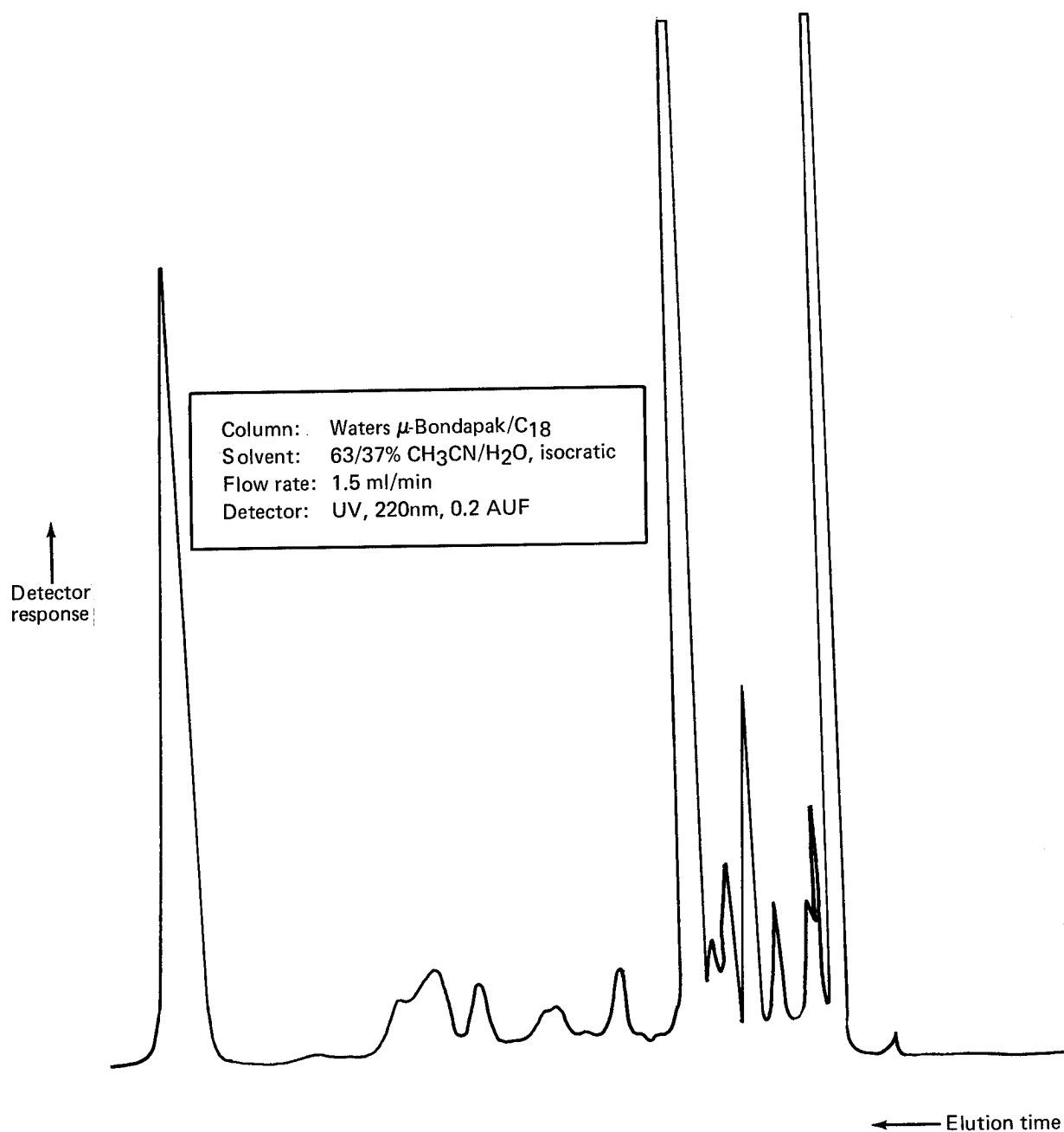
Figure 45. LC Chromatogram of Narmco Prepreg Batch 1072, Round-Robin Participant F
