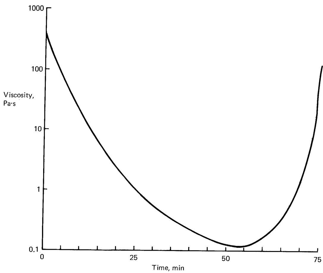
Figure 132. Viscosity Versus Time, Narmco Resin Batch 293
