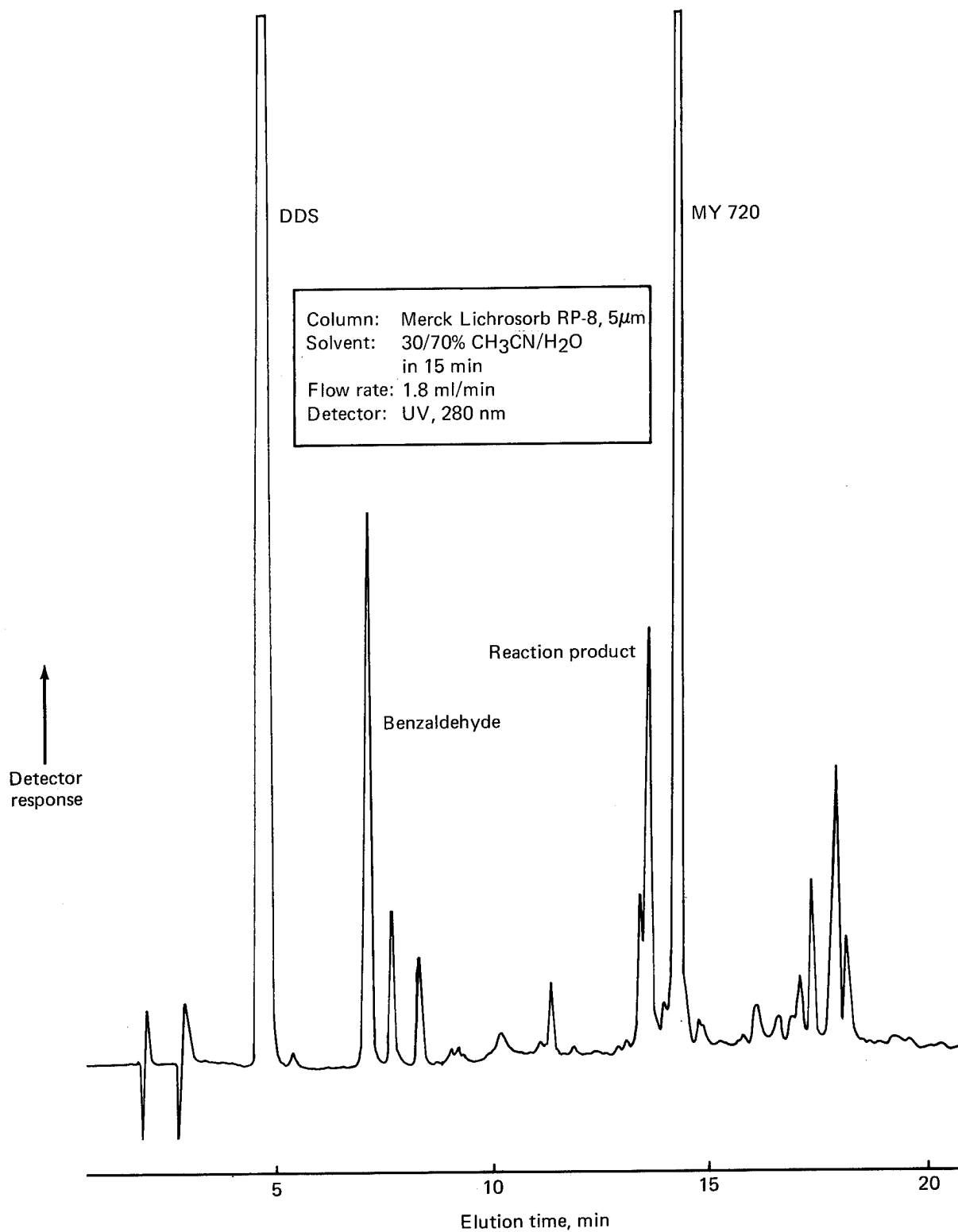
Figure 25. LC Chromatogram of Narmco Batch 286, Column: Merck Lichrosorb RP-8, 5 \mu m
