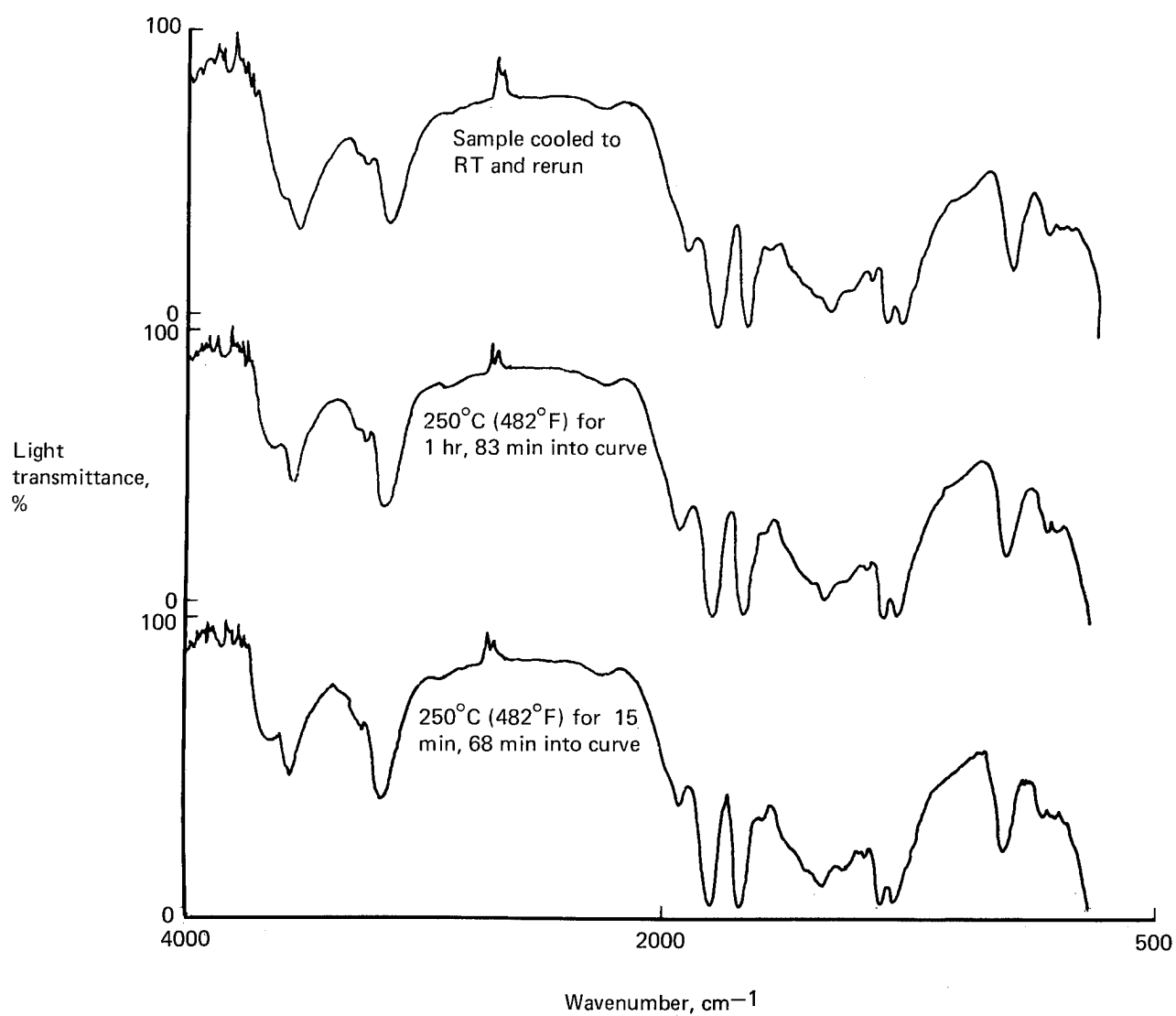
Figure 104. TSIR Spectra of Hercules Resin—RT and 250°C (RT and 482°F)
