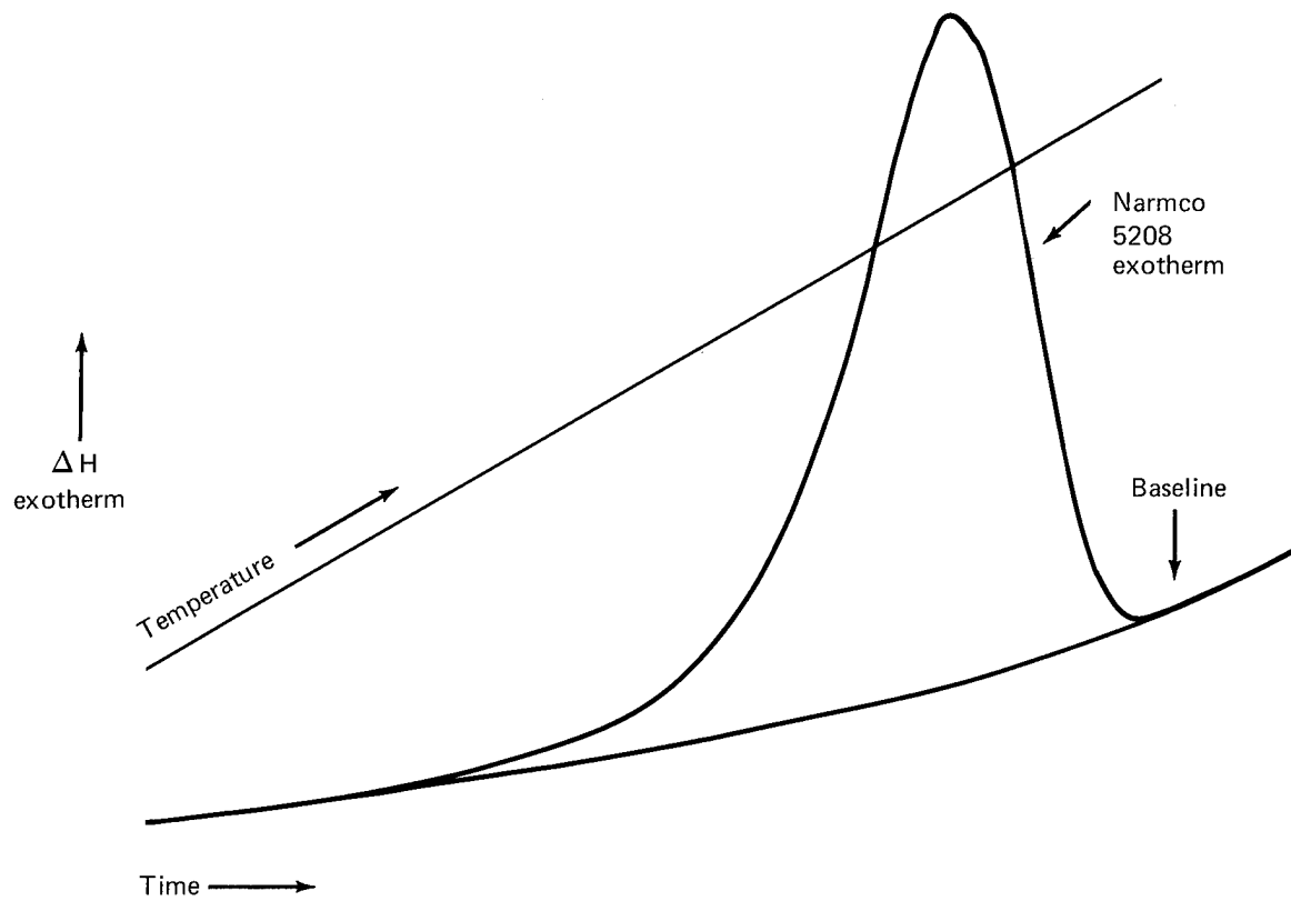
Figure A-3. Example DSC Curve—Resin and Baseline
