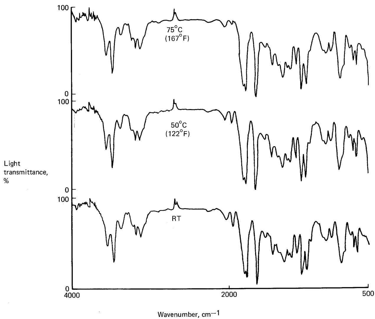
Figure 100. TSIR Spectra of Hercules Resin—RT, 50°C, and 75°C (RT, 122°F, and 167°F)
