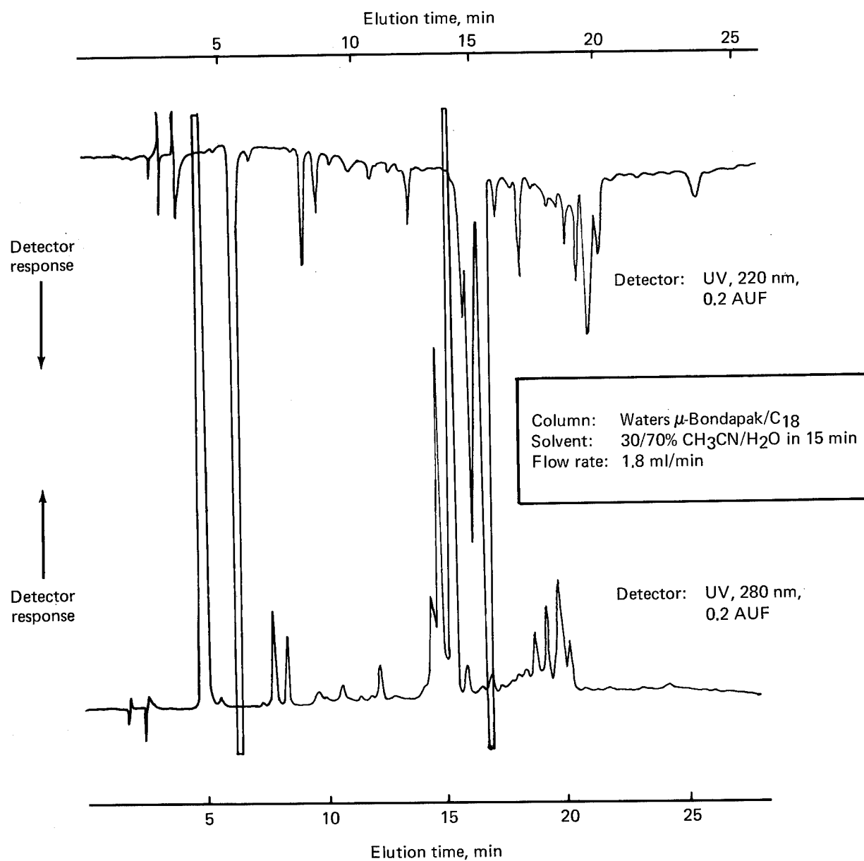
Figure 34. LC Chromatogram of Narmco Batch 286, Detector: UV, 220 nm
