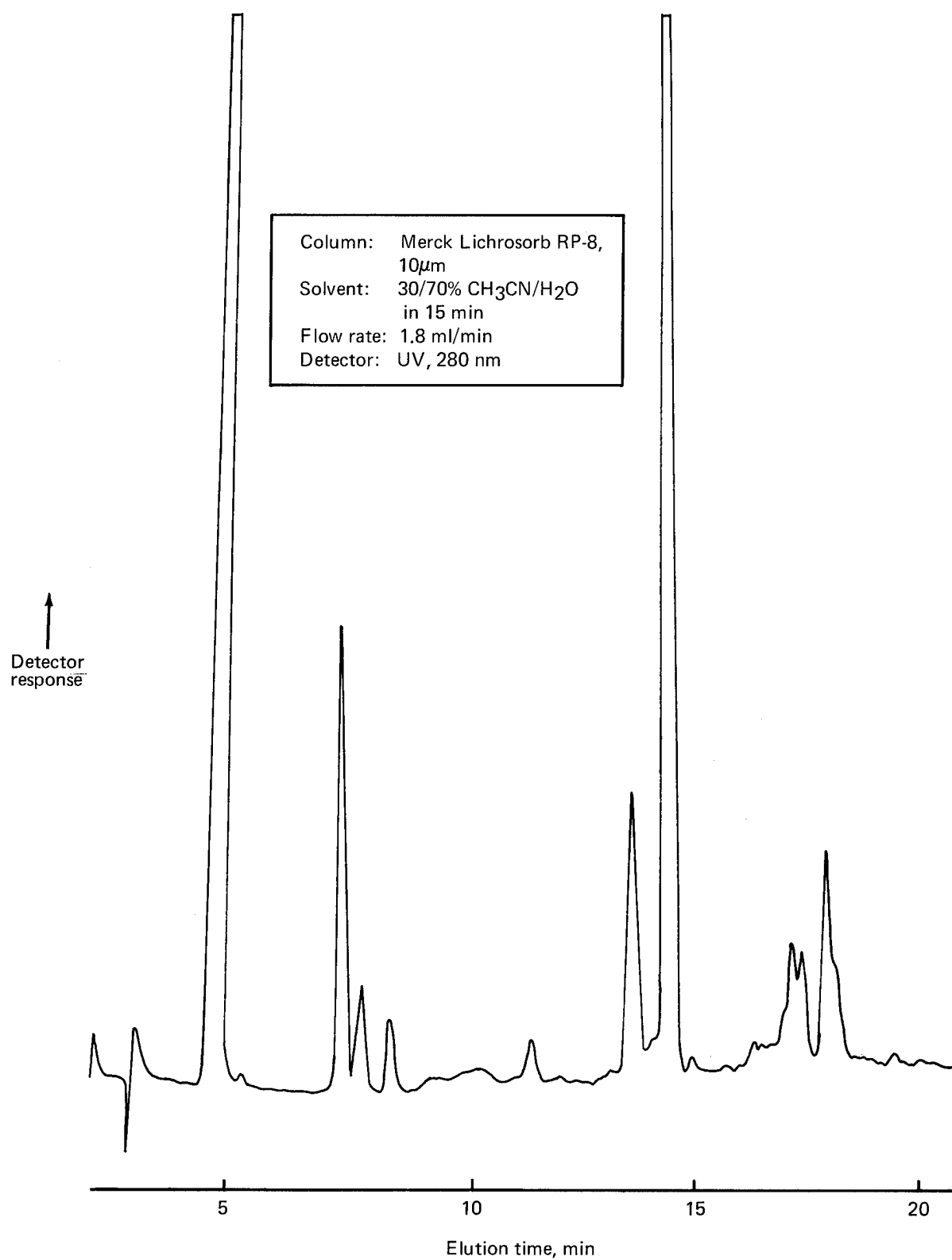
Figure 27. LC Chromatogram of Narmco Batch 286, Column: Merck Lichrosorb RP-8, 10µm
