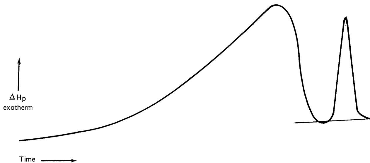
Figure 78. DSC Curve of Narmco Prepreg Batch 1072, Round-Robin Participant G
