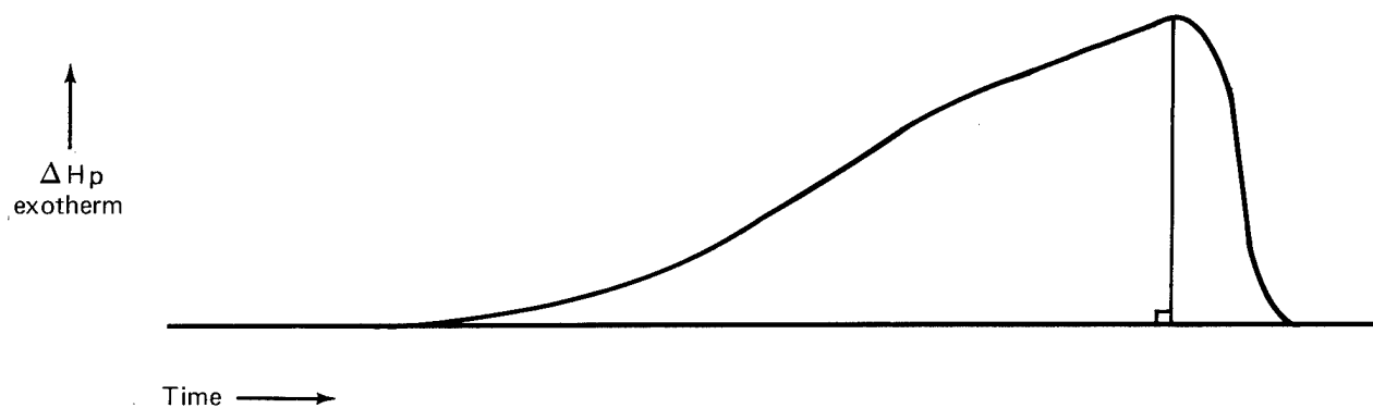
Figure 71. Symmetry Evaluation of DSC Curve for Narmco Resin Batch 286
