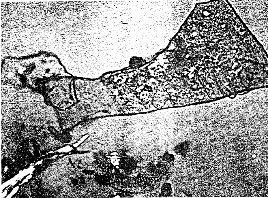
Figure 61. Contamination in Narmco Neat Resin Batch 300—Acetone-Insoluble Resin, Diatom
