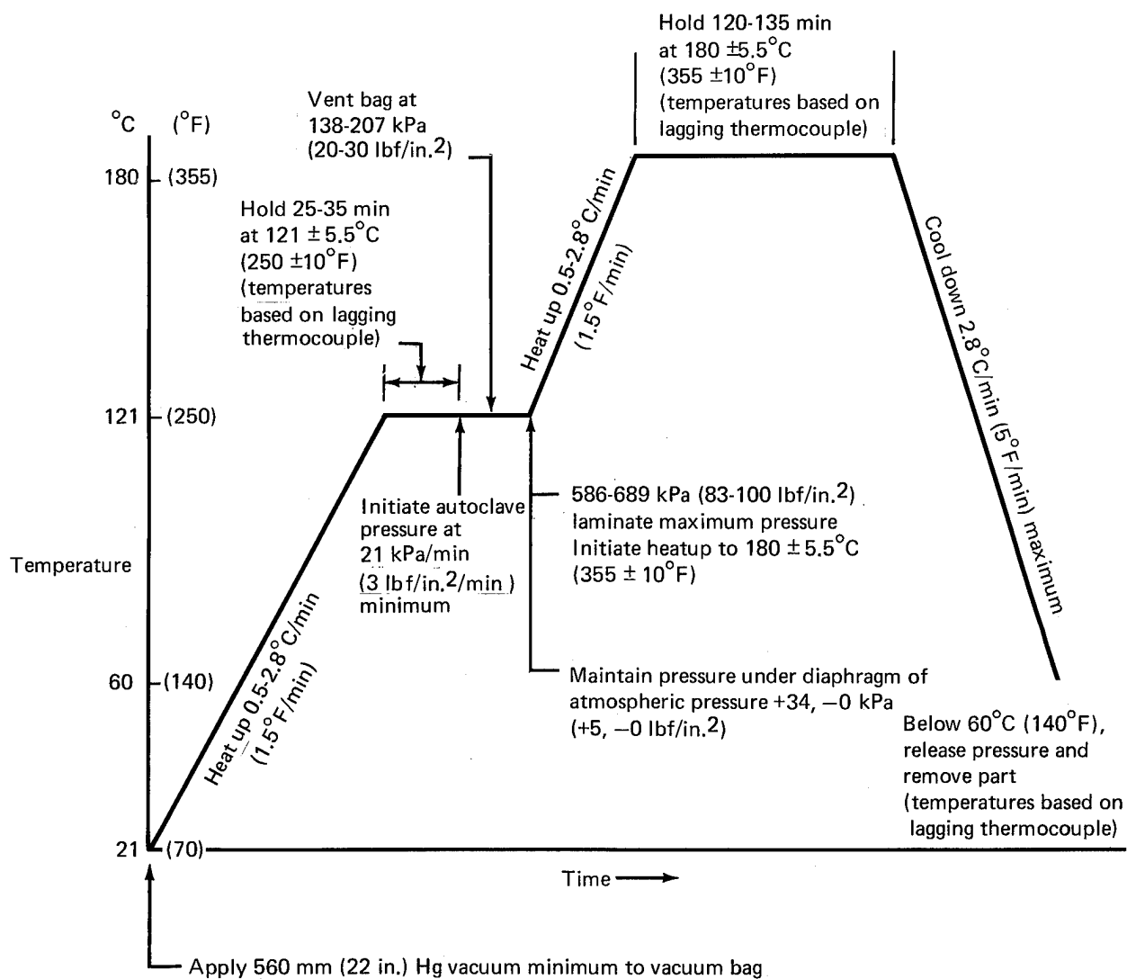
Figure 2. Lamine Cure Cycle
