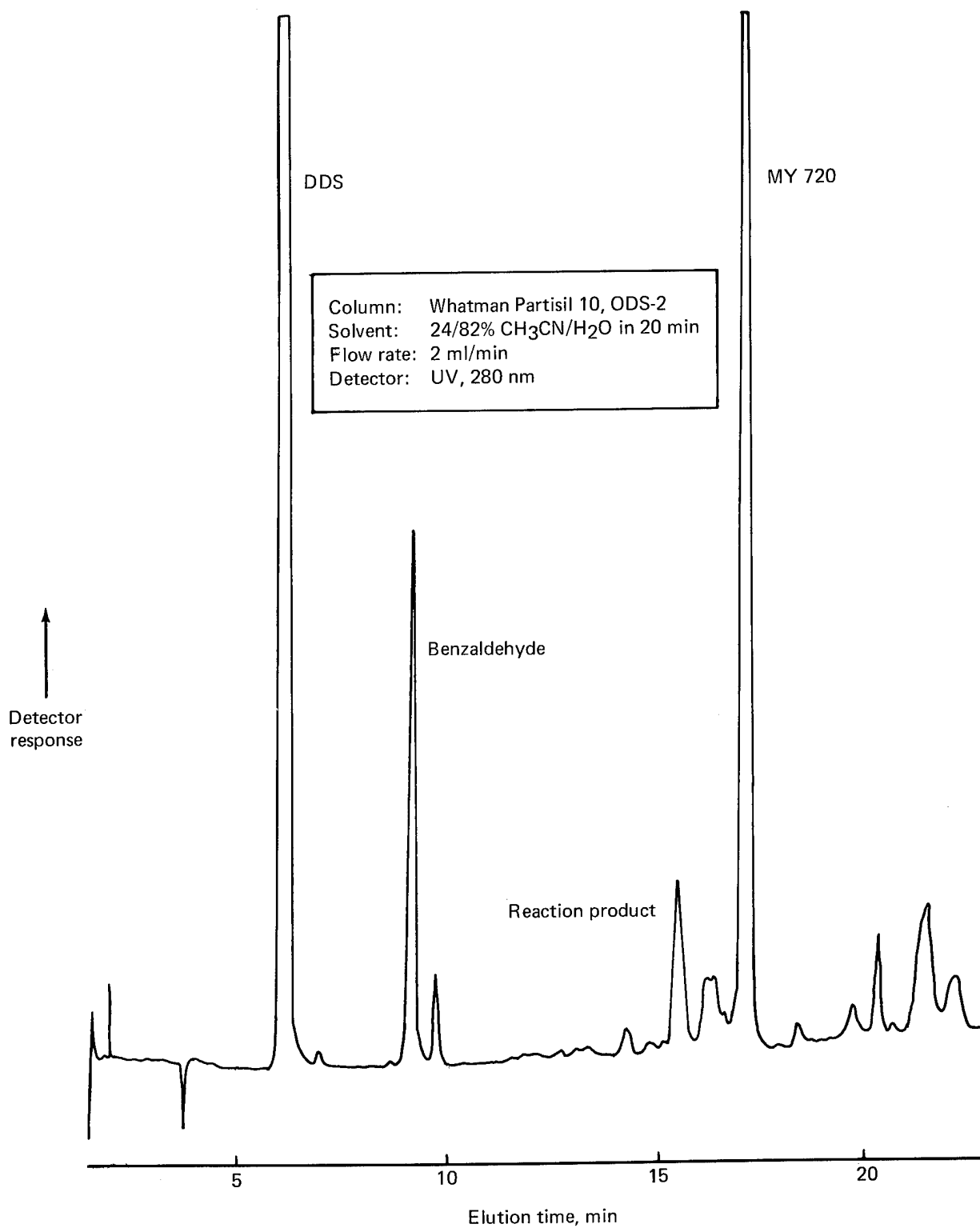
Figure 31. LC Chromatogram of Narmco Batch 286, Mobile Phase 1, Column: Whatman Partisil 10, ODS-2
