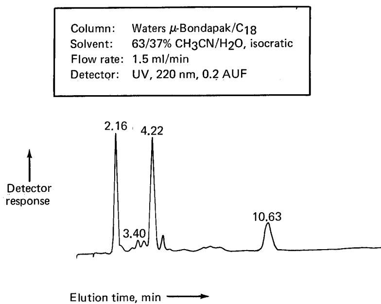
Figure 44. LC Chromatogram of Narmco Propreg Batch 1072, Round-Robin Participant E
