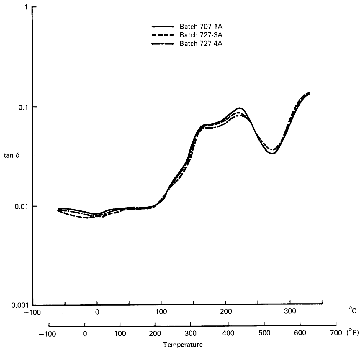
Figure 127. \tan \delta Versus Temperature, Hercules Laminates, Humidity Exposed
