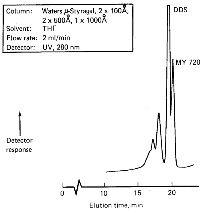
Figure 84. GPC Chromatogram of Narmco Neat Resin Batch 300, Solvent: THF, Column: Waters \mu -Styragel—2 x 100Å, 2 x 500 Å, 1 x 1000Å
