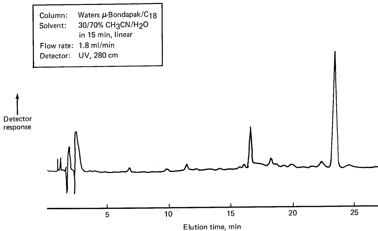
Figure 7. LC Chromatogram of T300 Fiber Finish
