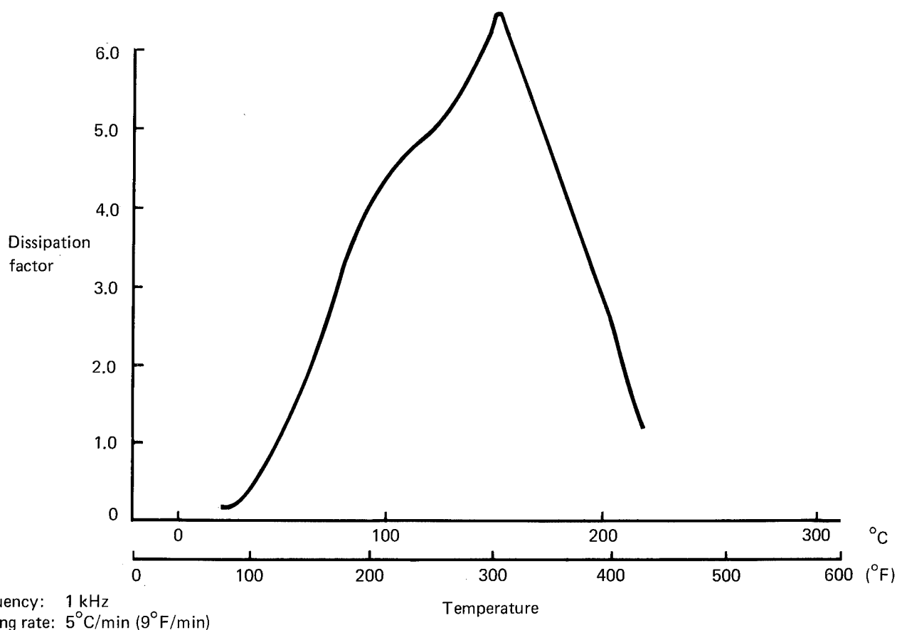
Figure 55. Results of Dielectric Analysis of Narmco Resin Batch 286
