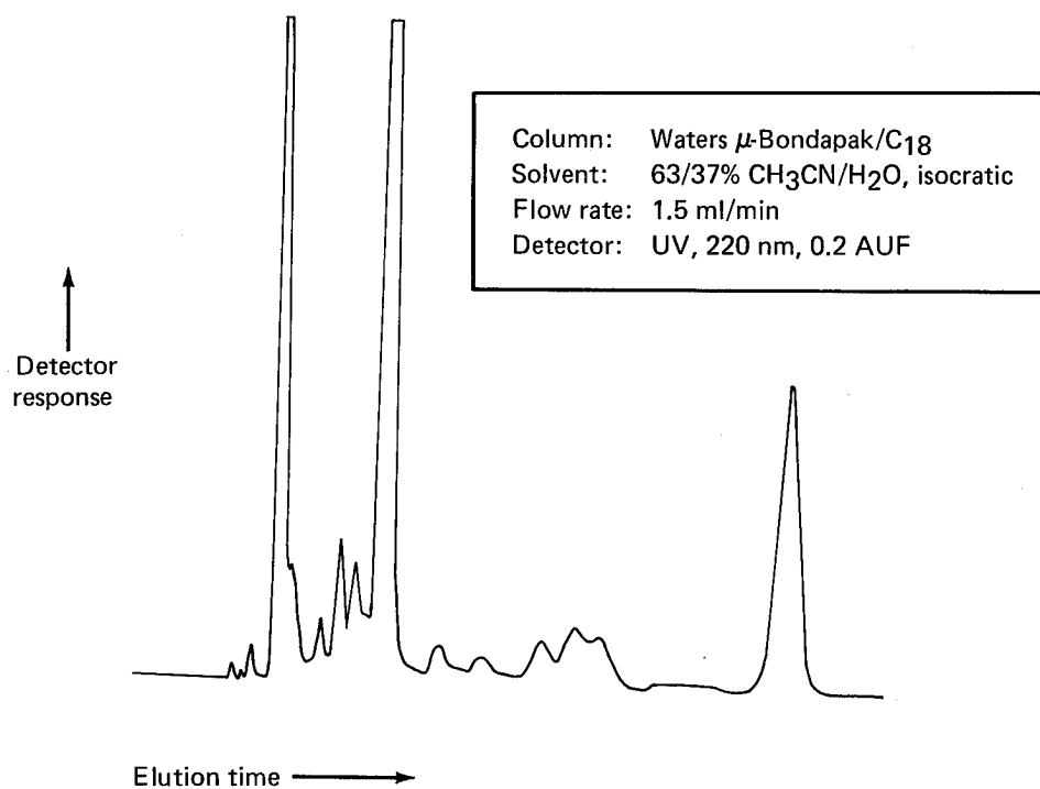
Figure 42. LC Chromatogram of Narmco Prepreg Batch 1072, Round-Robin Participant C
