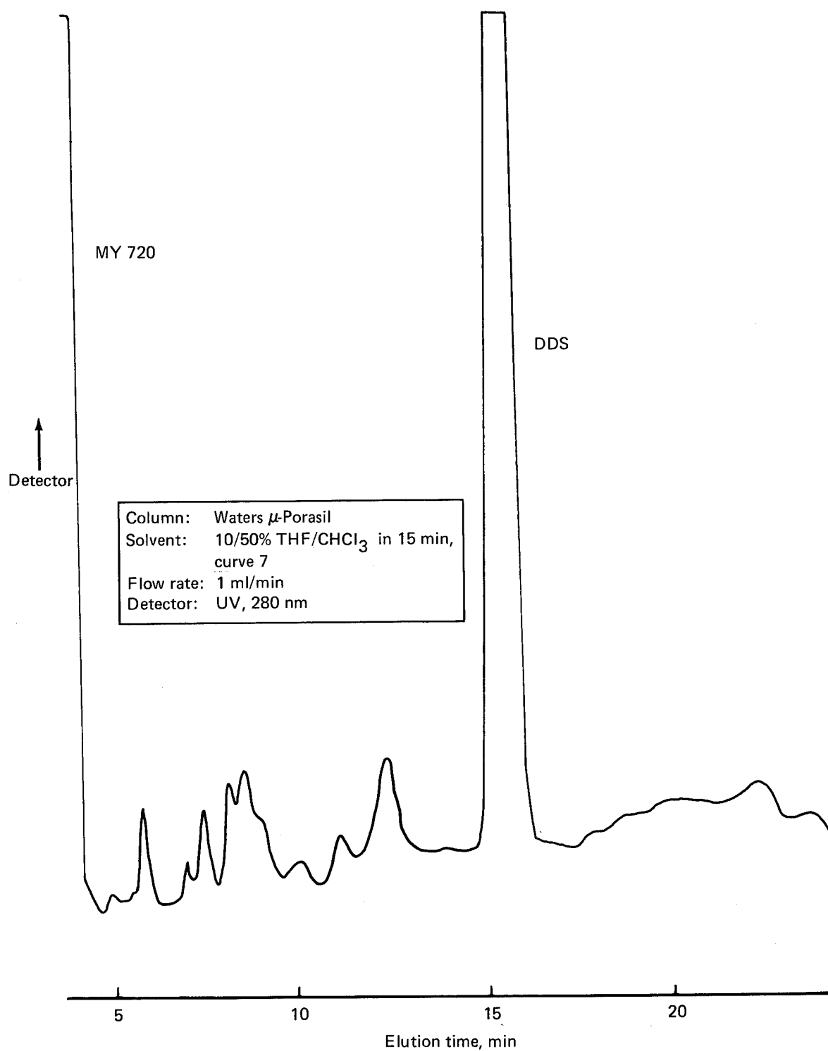
Figure 20. LC Chromatogram of Narmco Batch 286, Solvent: THF/ \text{CHCl}_3
