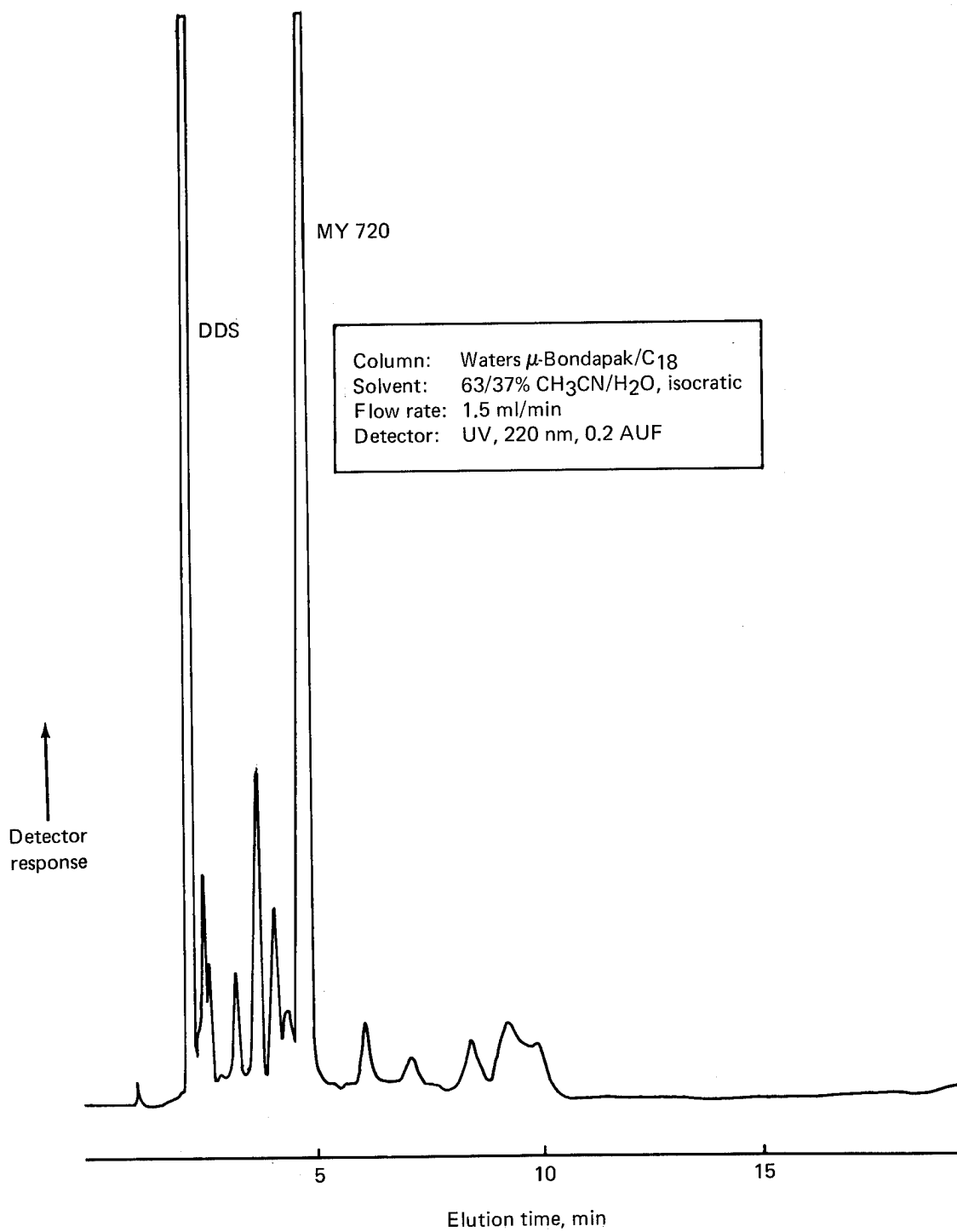
Figure 32. LC Chromatogram of Narmco Batch 286, Isocratic Solvent, Column: Waters \mu -Bondapak/C18
