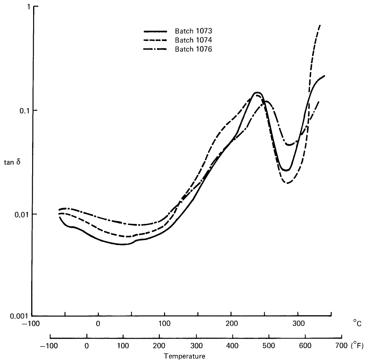
Figure 126. \tan \delta Versus Temperature, Narmco Laminates, Humidity Exposed
