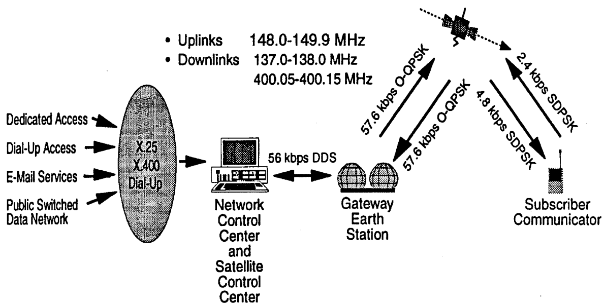
Figure 2. ORBCOMM system architecture. After Ref. [6].
