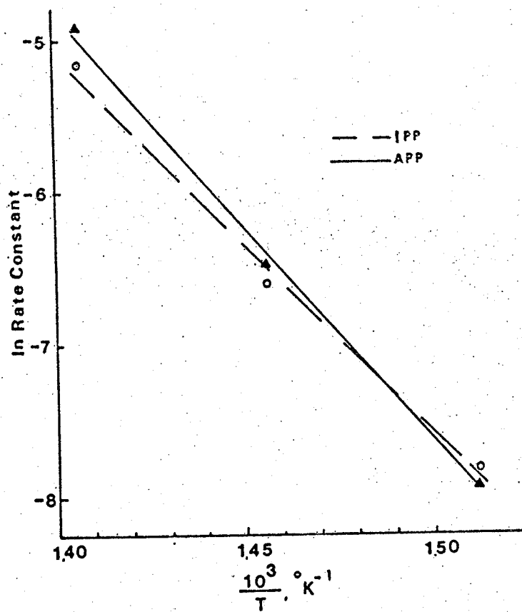
Fig. 5 Arrhenius plot for pyrolysis of AFP and IPP in helium
