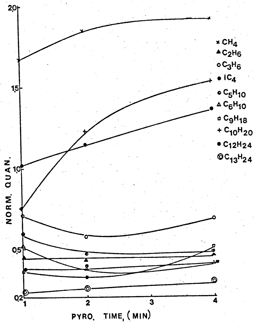
Fig. 6 Absolute normalized product distributions of pyrolysis of Sample A and IPP in helium at 438^\circ\text{C} as a function of pyrolysis time
