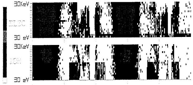
Figure 4: ESA Output showing full return of Low Energy Ion Spectra on 6/19/95 - plot on left shows 30sec averaged electron & ion data - plot above shows raw counts over same interval
