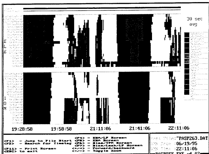
Figure 4: ESA Output showing full return of Low Energy Ion Spectra on 6/19/95 - plot on left shows 30sec averaged electron & ion data - plot above shows raw counts over same interval
