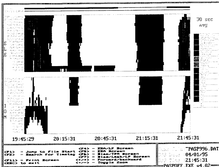
Figure 3: ESA Output showing partial return of Low Energy Ion Spectra - plot on left shows 30sec averaged electron & ion data - plot above shows raw counts over same interval
