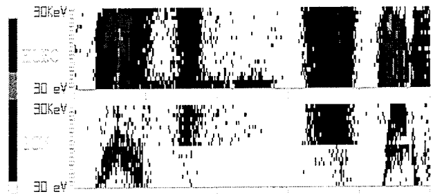
Figure 3: ESA Output showing partial return of Low Energy Ion Spectra - plot on left shows 30sec averaged electron & ion data - plot above shows raw counts over same interval
