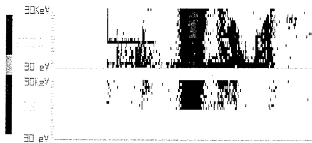
Figure 2: ESA Output showing loss of Low Energy Ion Data - plot on left shows 30sec averaged electron & ion data - plot above shows raw counts over same interval
