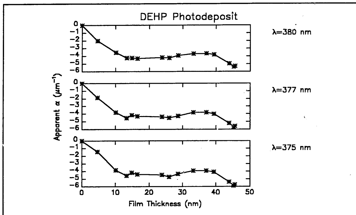
Figure C18c Computed values of \alpha ; for photochemically deposited films of dioctyl phthalate (DEHP). (Ultraviolet wavelength range)
