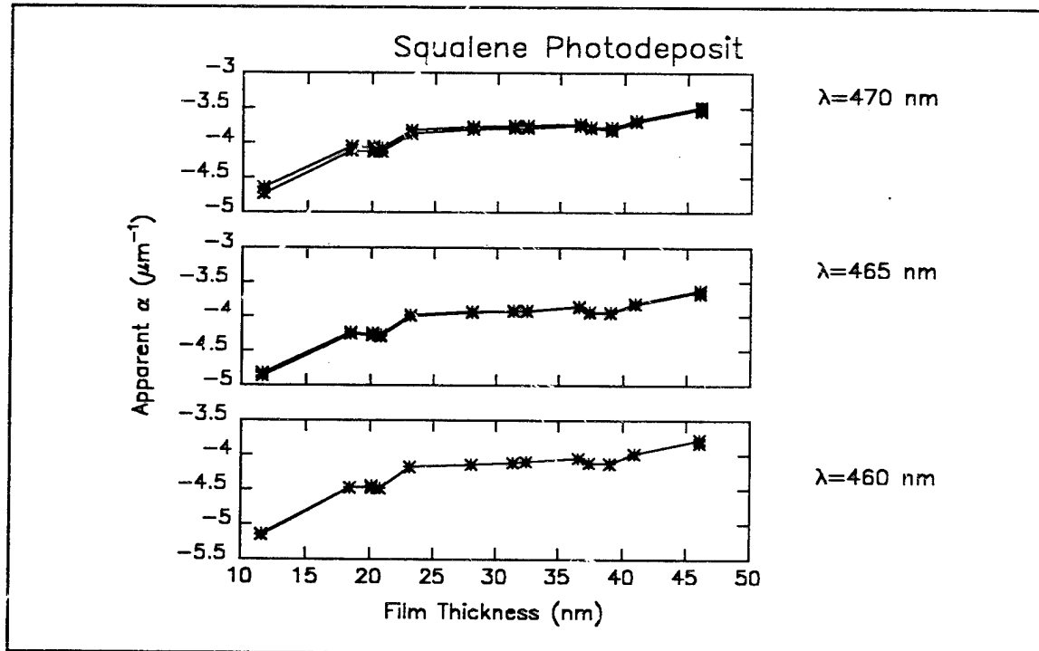
Figure D18p Computed values of \alpha_j for photochemically deposited films of Squalene. (Visible wavelength range)
