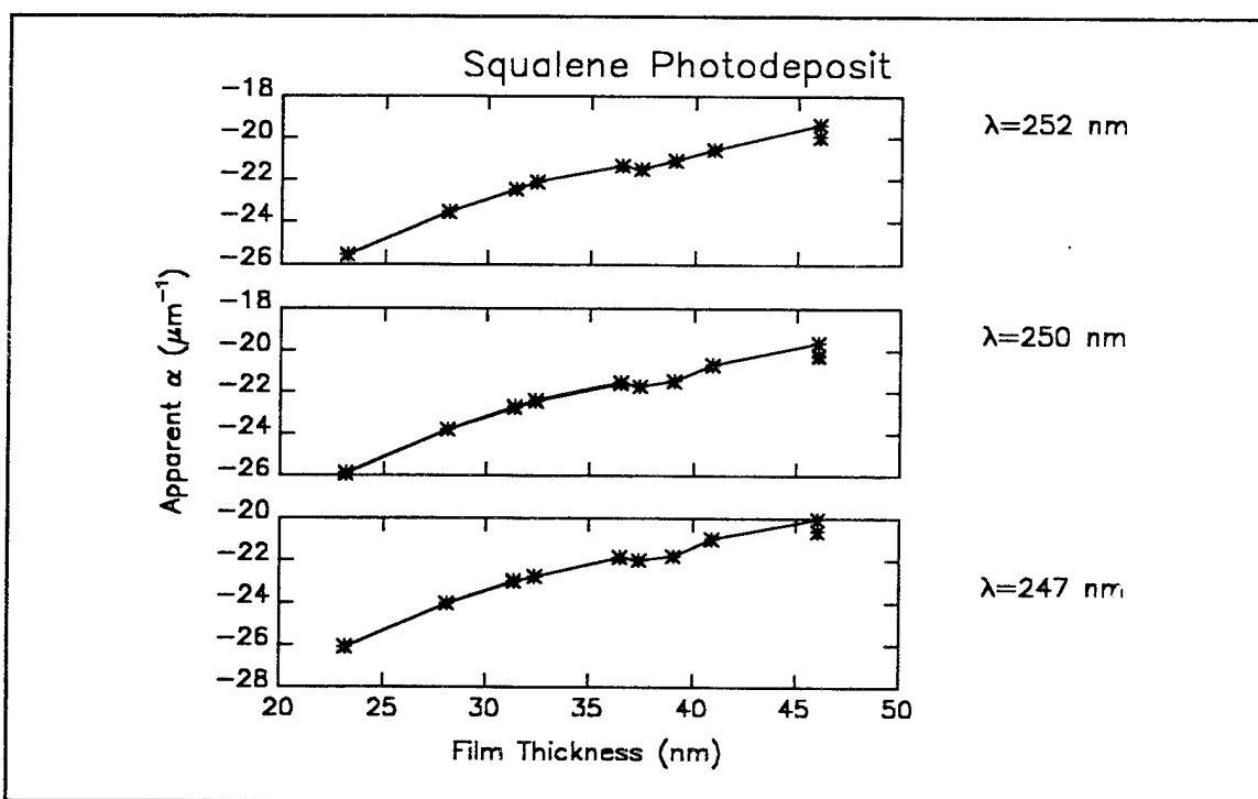
Figure D19t Computed values of \alpha_i for photochemically deposited films of Squalene. (Ultraviolet wavelength range)
