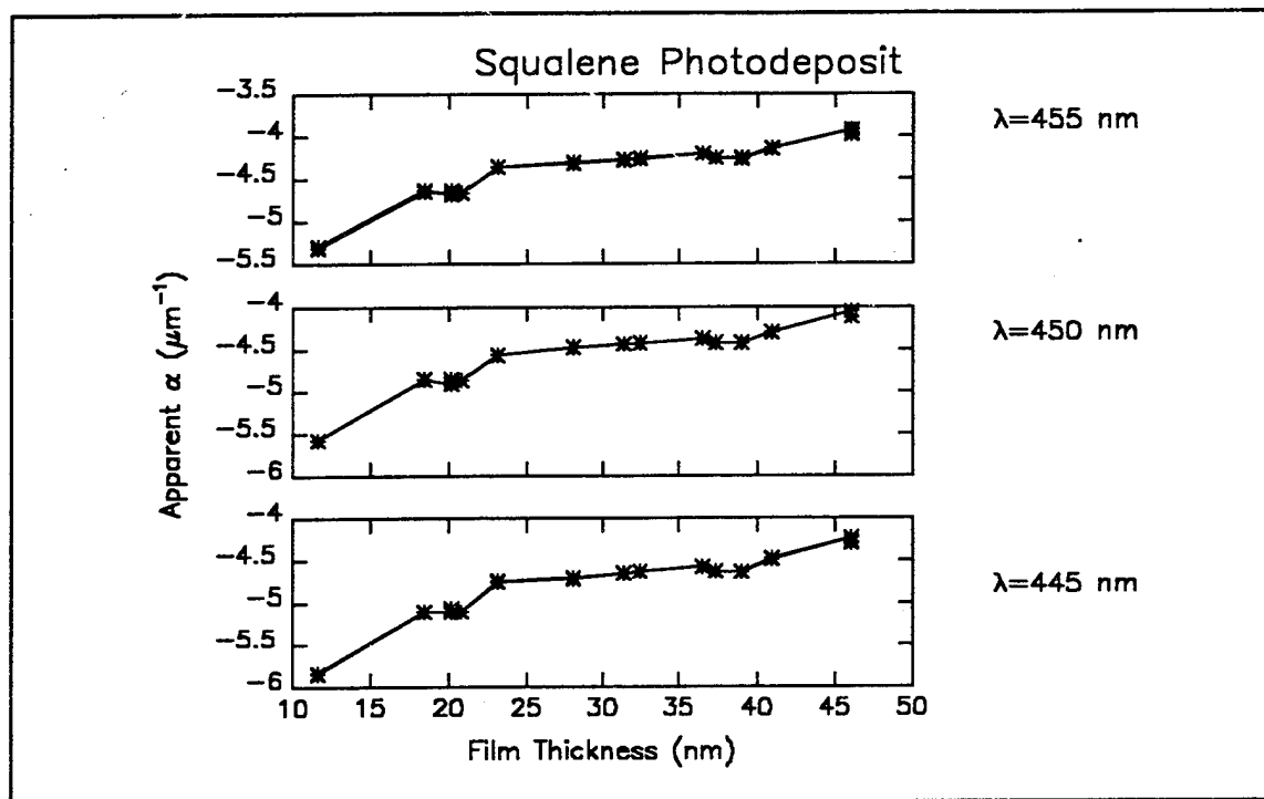
Figure D18q Computed values of \alpha_i for photochemically deposited films of Squalene. (Visible wavelength range)
