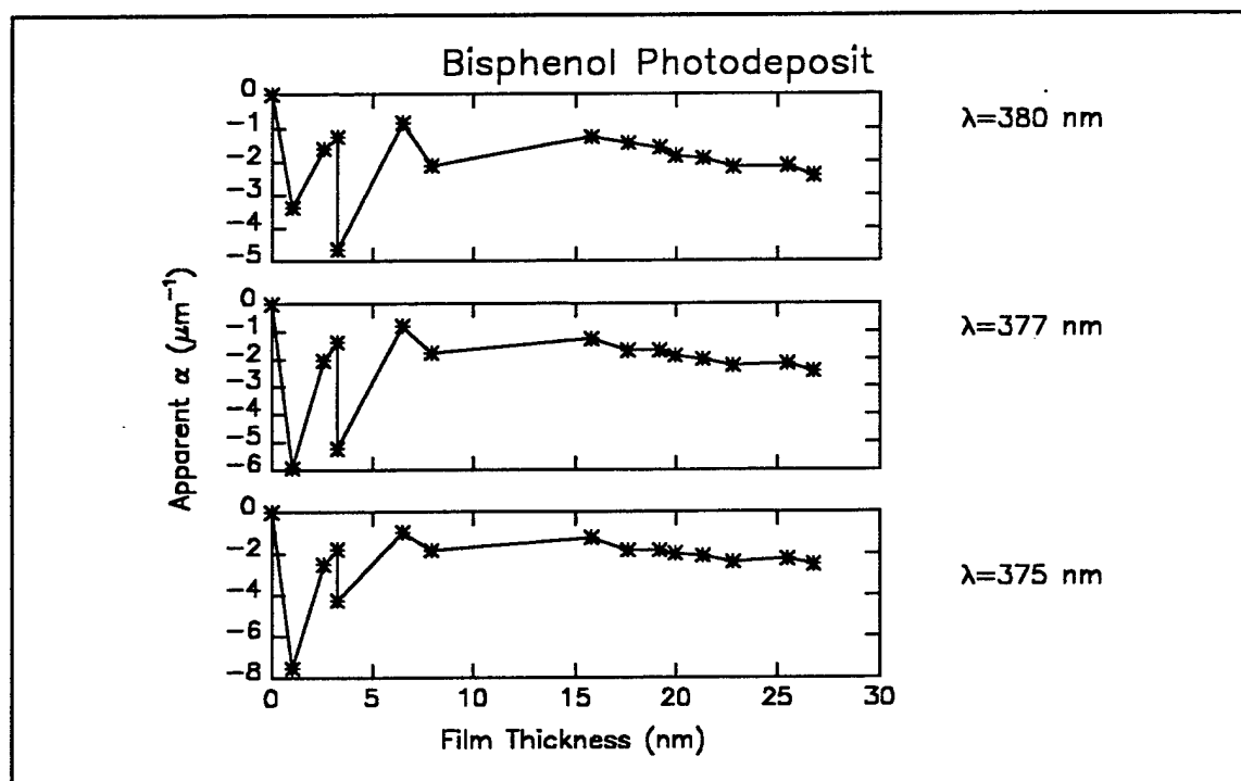
Figure A17c Computed values of \alpha_i for the Bisphenol photodeposit, visible range.
