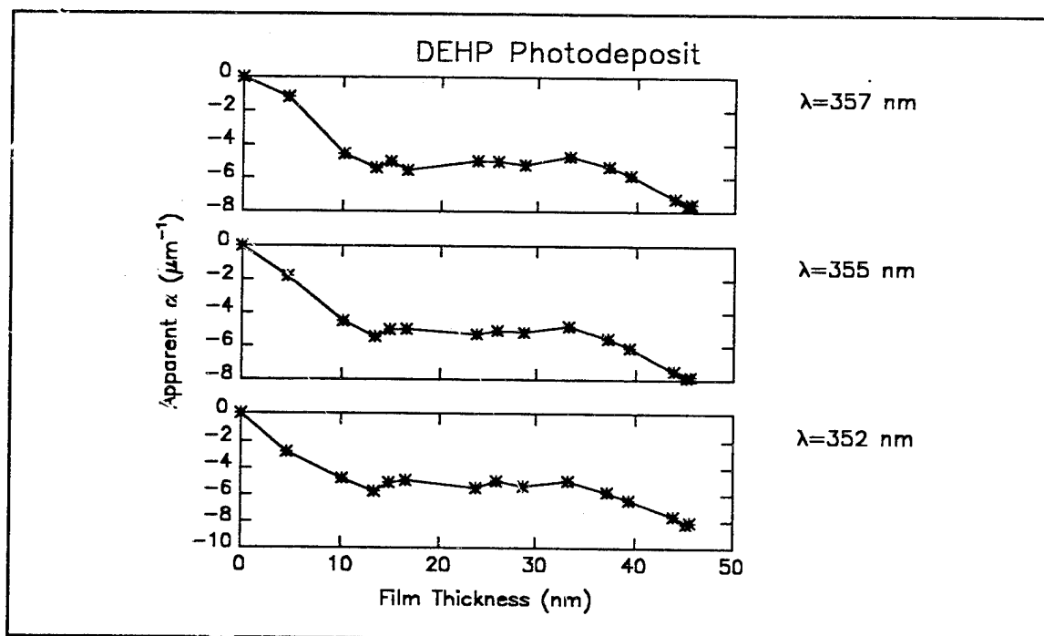
Figure C18f Computed values of \alpha_j for photochemically deposited films of dioctyl phthalate (DEHP). (Ultraviolet wavelength range)
