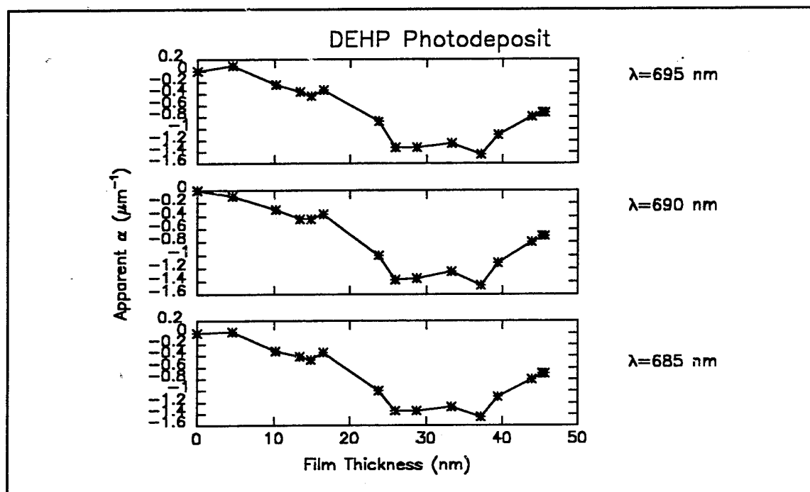
Figure C17a Computed values of \alpha_i for photochemically deposited films of dioctyl phthalate (DEHP). (Visible wavelength range)
