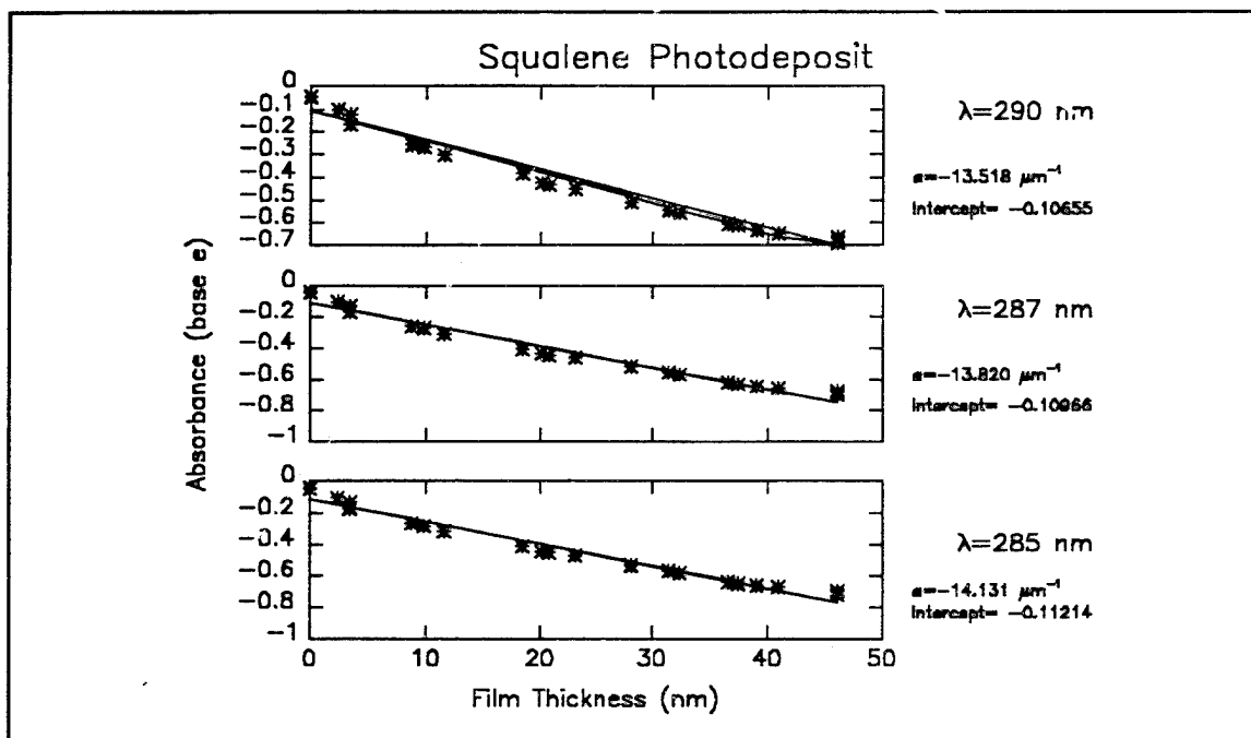
Figure D15o Fits of measured transmission spectra of the Squalene photodeposit to the Beer-Lambert absorption law. (Ultraviolet wavelength range)
