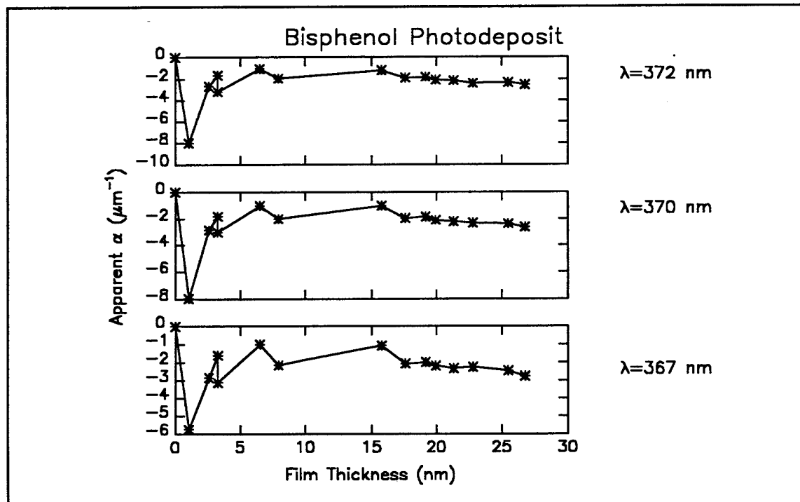
Figure A17d Computed values of \alpha_i for the Bisphenol photodeposit, visible range.
