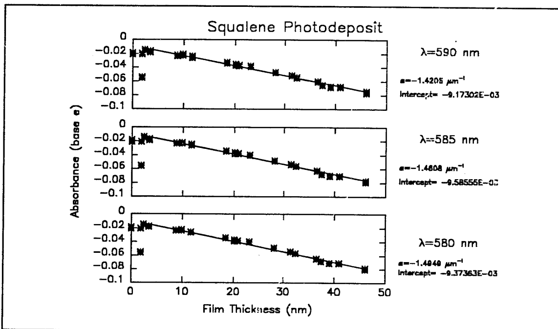
Figure D14h Fits of measured transmission spectra of the Squalene photodeposit to the Beer-Lambert absorption law. (Visible wavelength range)
