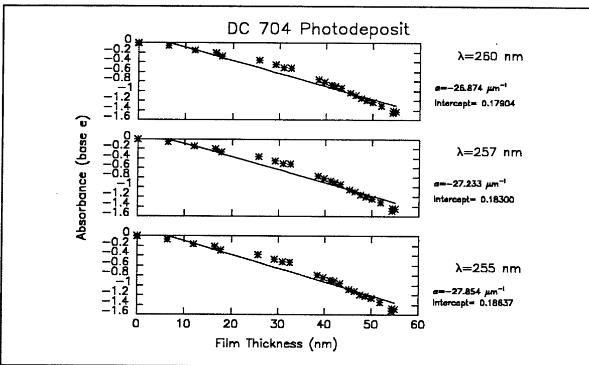
Figure B17s. Fits of measured transmission spectra to the Beer-Lambert absorption law. (Ultraviolet wavelength range)
