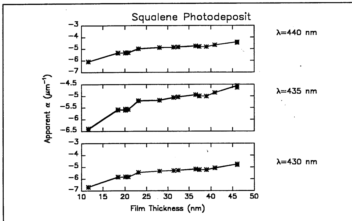
Figure D18r Computed values of \alpha_i for photochemically deposited films of Squalene. (Visible wavelength range)
