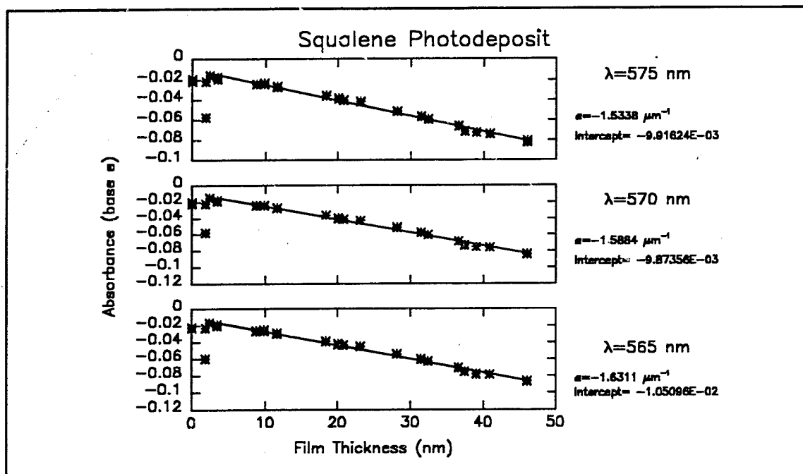
Figure D14i Fits of measured transmission spectra of the Squalene photodeposit to the Beer-Lambert absorption law. (Visible wavelength range)
