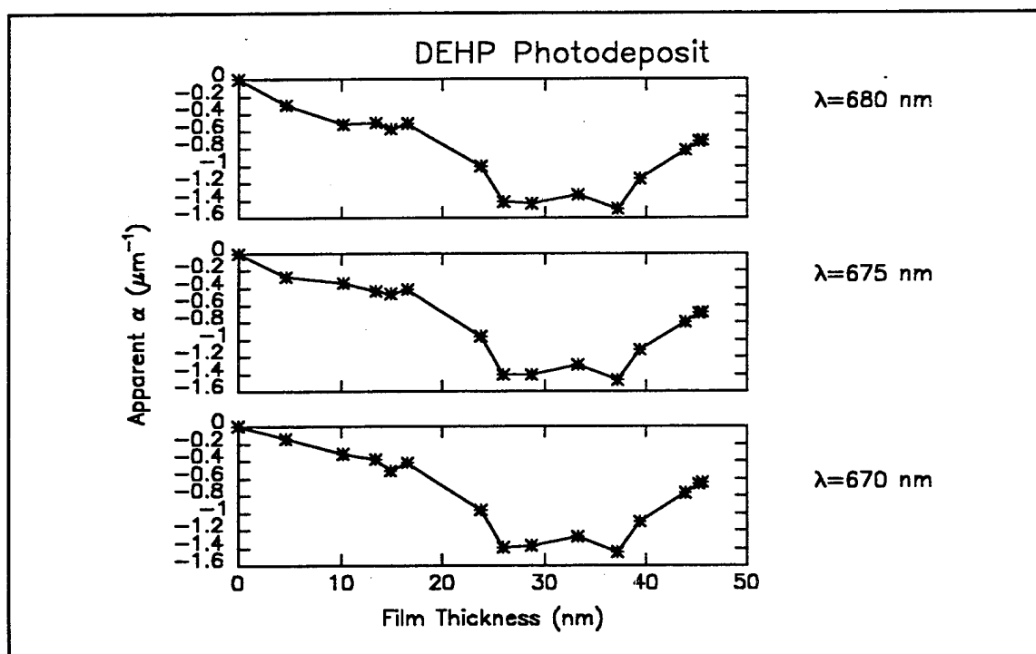
Figure C17b Computed values of \alpha_i for photochemically deposited films of dioctyl phthalate (DEHP). (Visible wavelength range)
