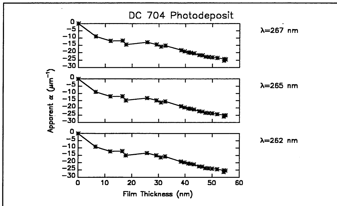
Figure B21r. Computed values of \alpha_i for photochemically deposited films of DC704. Ultraviolet wavelength range
