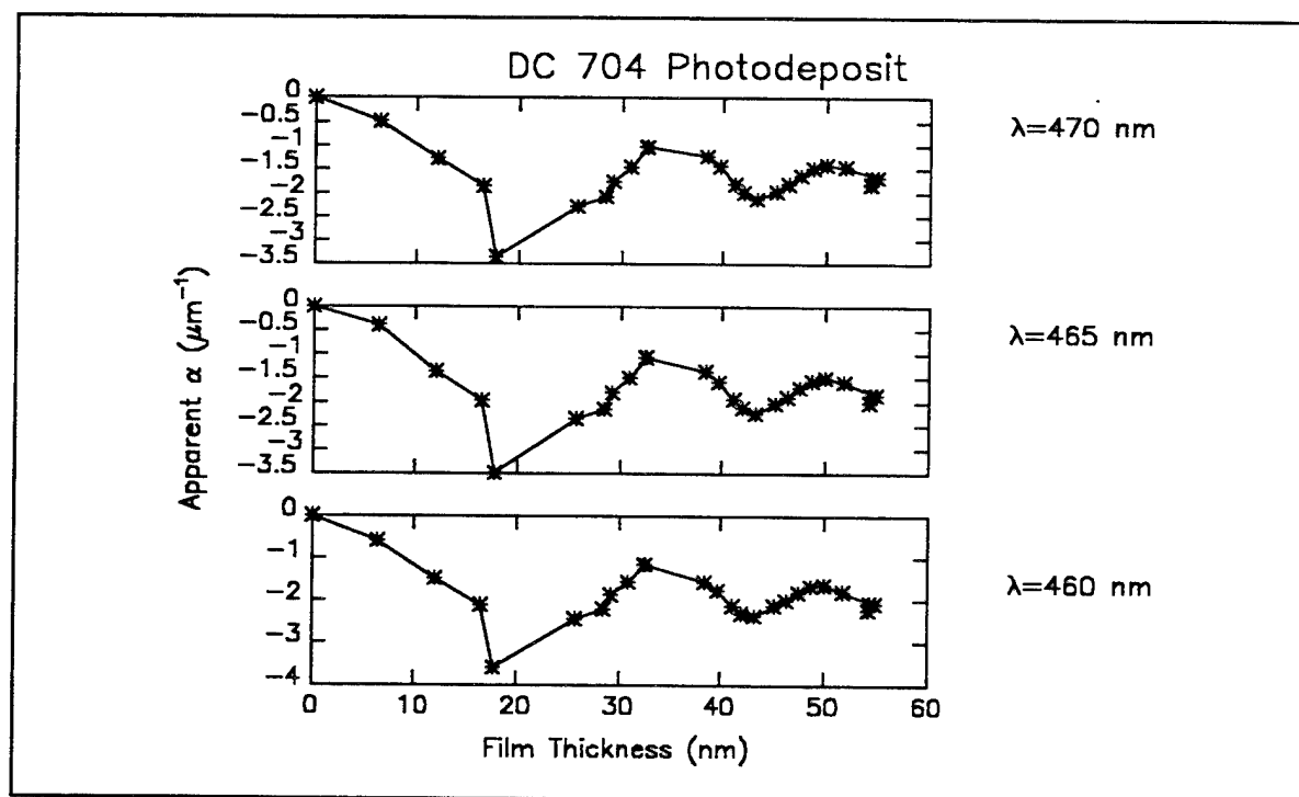
Figure B20p Computed values of \alpha_j for photochemically deposited DC 704 (see eq. B2).
