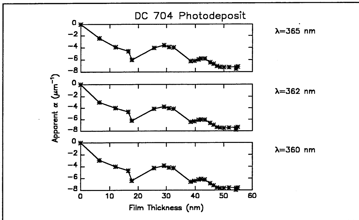
Figure B21e. Computed values of \alpha_j for photochemically deposited films of DC704. Ultraviolet wavelength range
