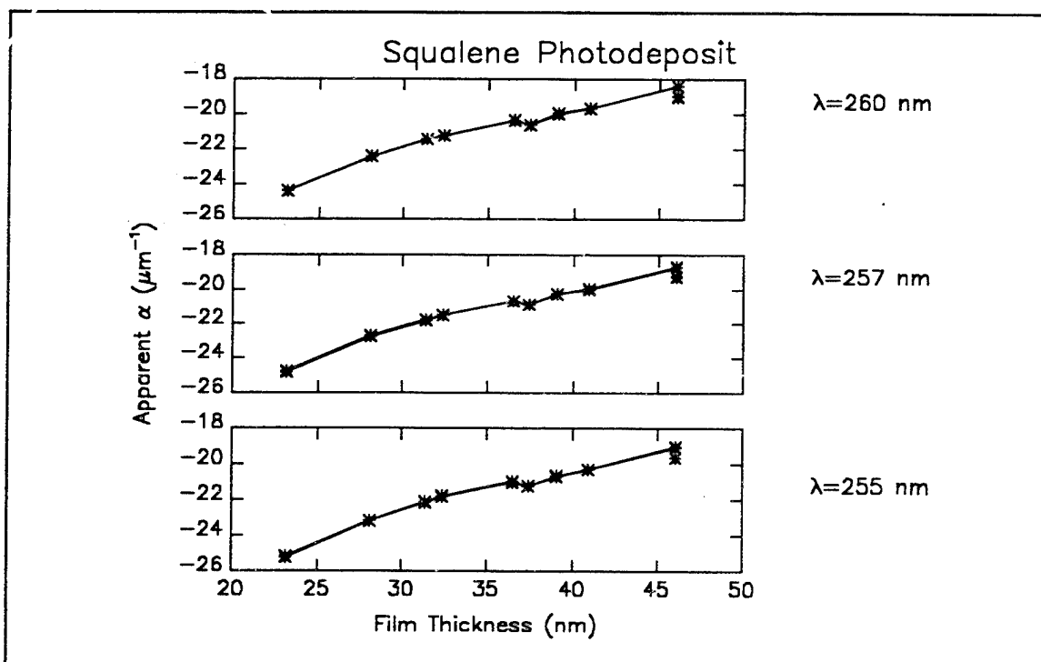
Figure D19s Computed values of \alpha_i for photochemically deposited films of Squalene. (Ultraviolet wavelength range)
