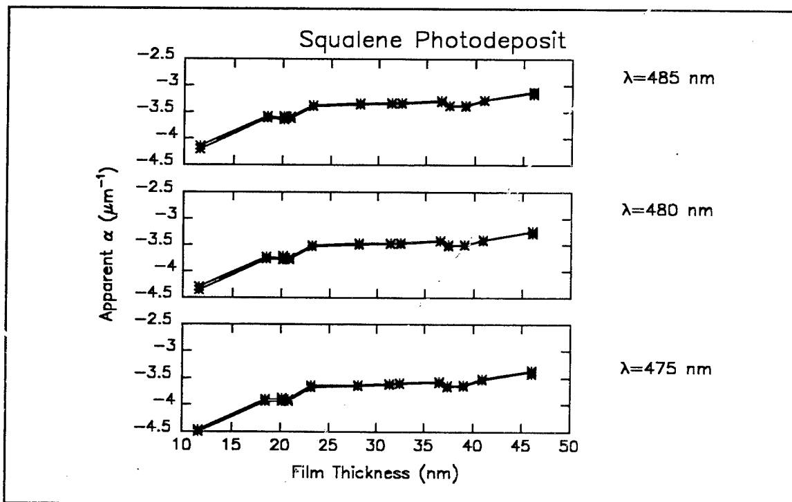
Figure D18o Computed values of \alpha_j for photochemically deposited films of Squalene. (Visible wavelength range)
