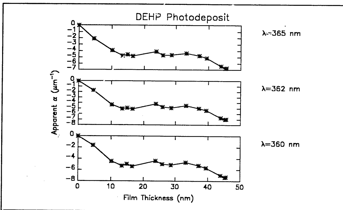
Figure C18e Computed values of \alpha_j for photochemically deposited films of dioctyl phthalate (DEHP). (Ultraviolet wavelength range)
