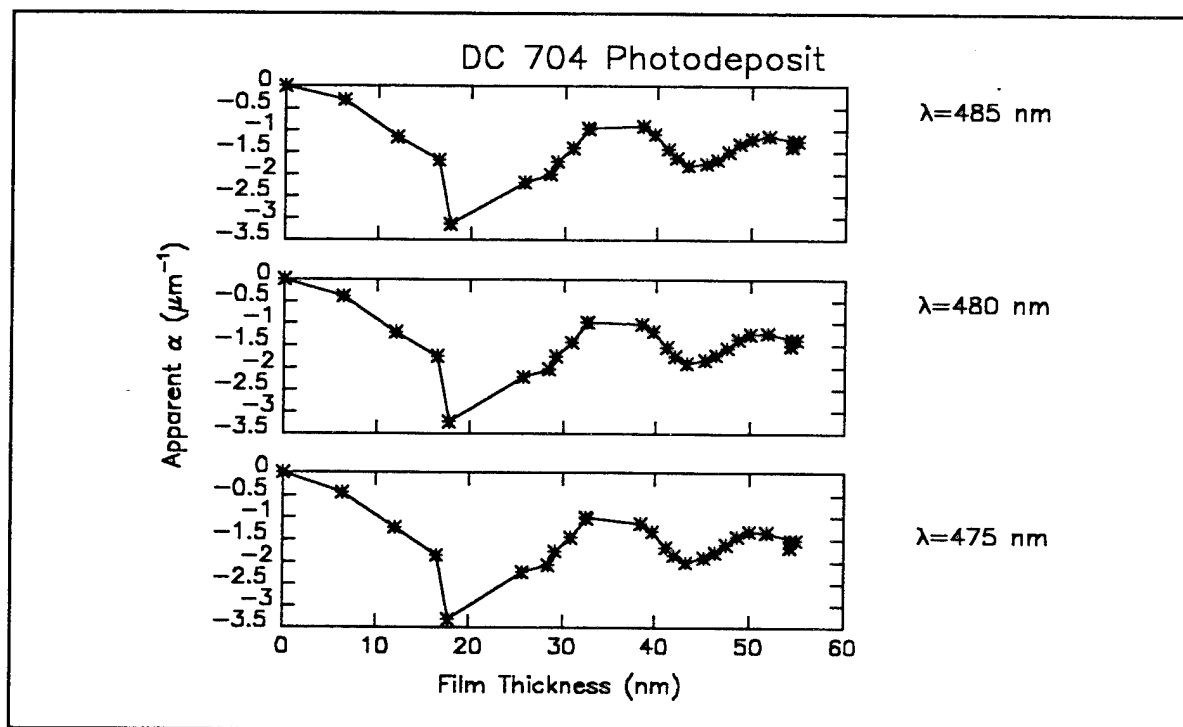
Figure B20o Computed values of \alpha_j for photochemically deposited DC 704 (see eq. B2).
