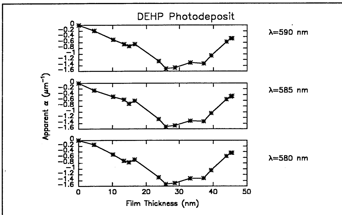
Figure C17h Computed values of \alpha_i for photochemically deposited films of dioctyl phthalate (DEHP). (Visible wavelength range)
