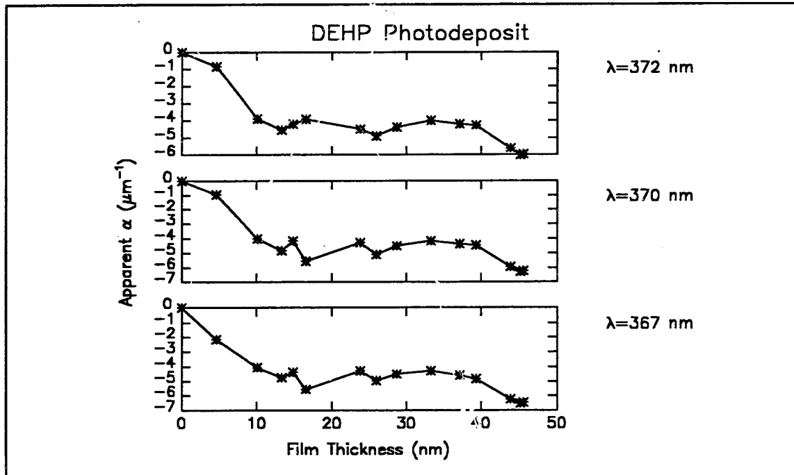
Figure C18d Computed values of \alpha ; for photochemically deposited films of dioctyl phthalate (DEHP). (Ultraviolet wavelength range)
