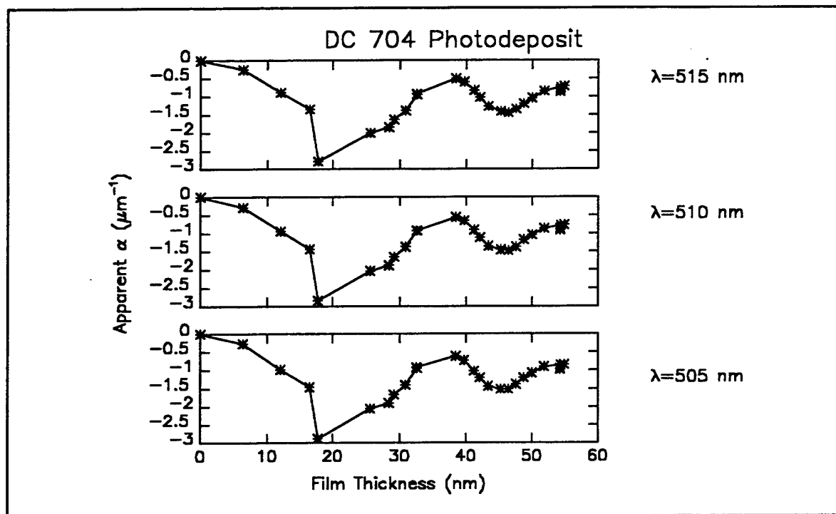
Figure B20m Computed values of \alpha_i for photochemically deposited DC 704 (see eq. B2).
