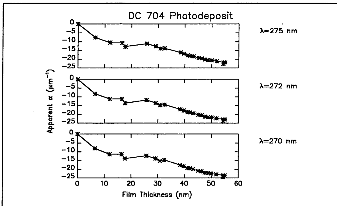
Figure B21q. Computed values of \alpha_i for photochemically deposited films of DC704. Ultraviolet wavelength range
