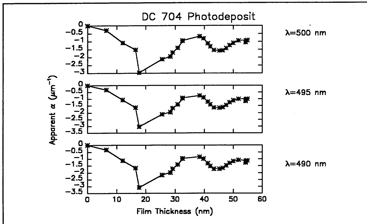
Figure B20n Computed values of \alpha_i for photochemically deposited DC 704 (see eq. B2).
