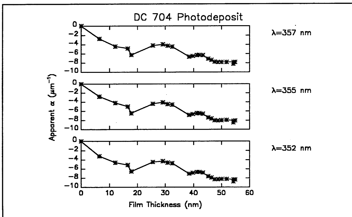
Figure B21f. Computed values of \alpha_j for photochemically deposited films of DC704. Ultraviolet wavelength range
