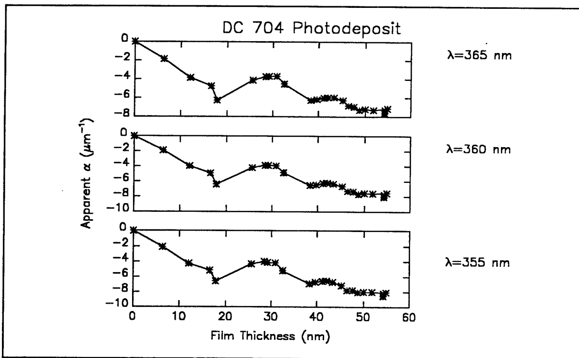
Figure B20w Computed values of \alpha_j for photochemically deposited DC 704 (see eq. B2).
