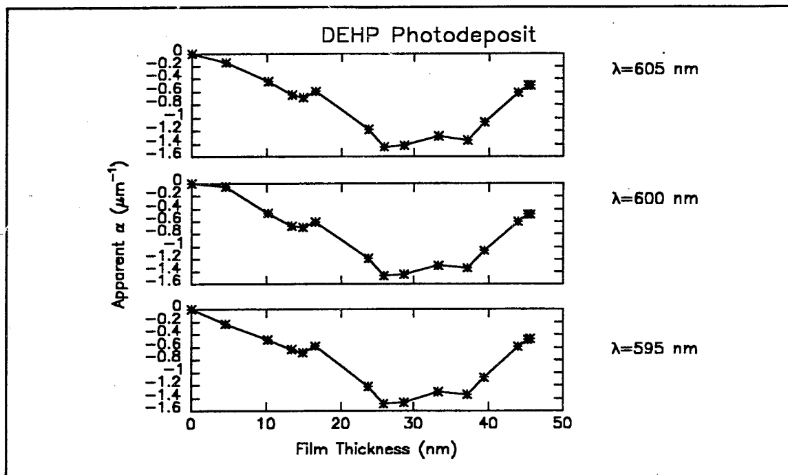
Figure C17g Computed values of \alpha_i for photochemically deposited films of dioctyl phthalate (DEHP). (Visible wavelength range)
